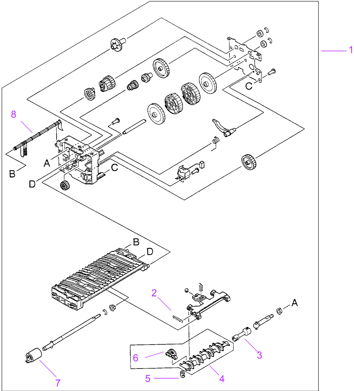
Figure 8-19 Paper Pickup Drive Assembly
