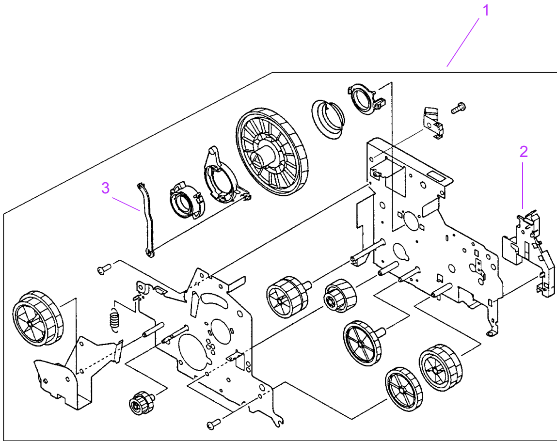
Figure 8-9 Printer Drive Assembly
