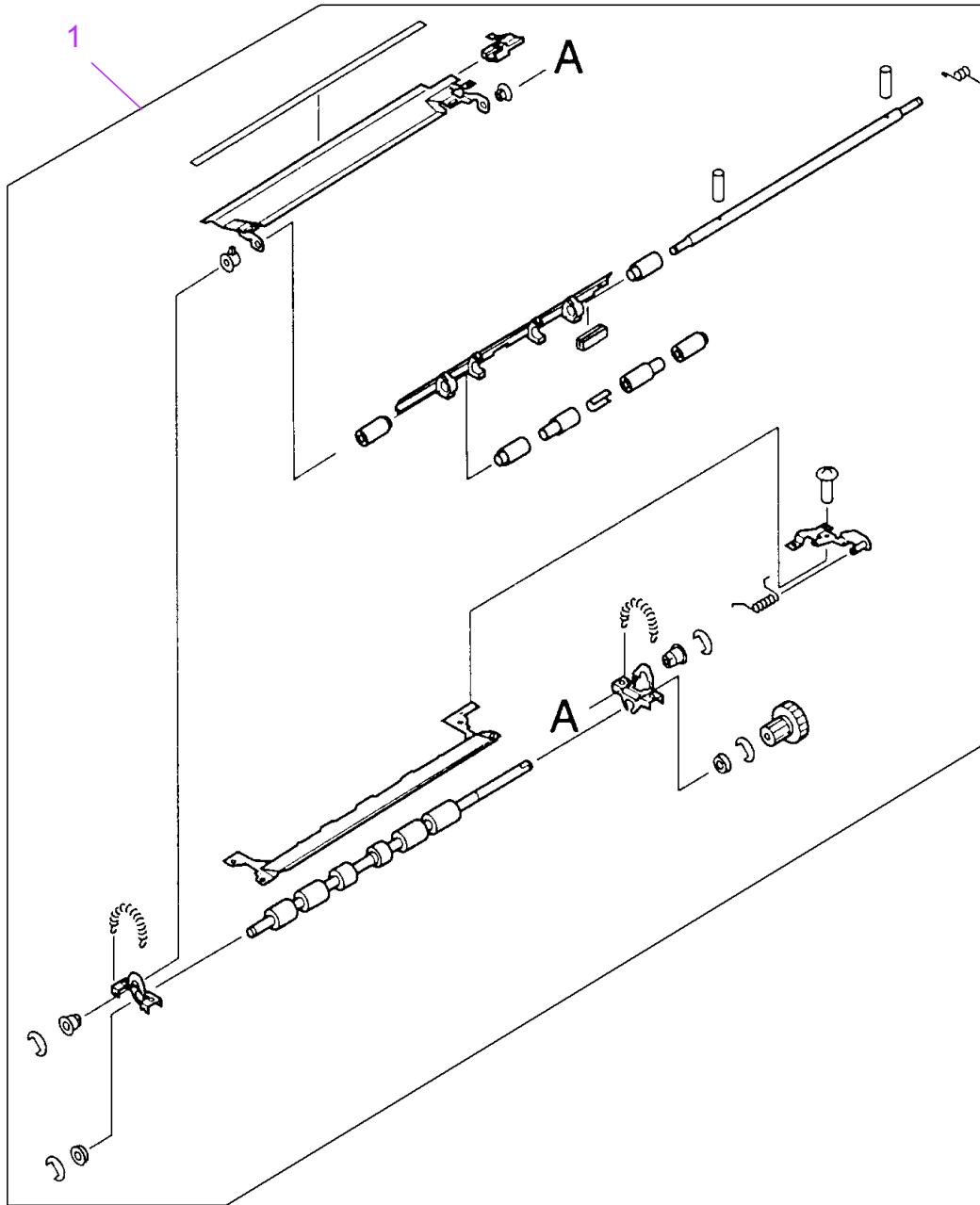
Figure 8-13 Registration Assembly
