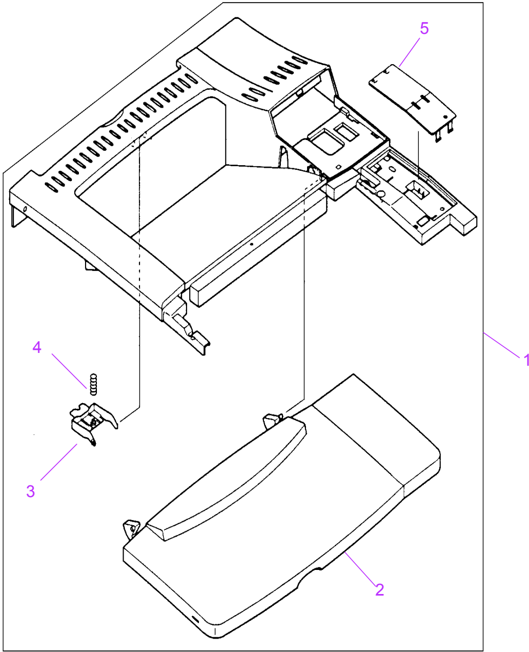
Figure 8-3 Top Cover Assembly
