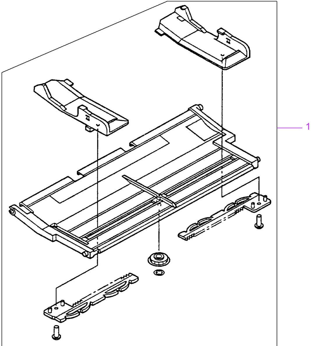
Figure 8-11 Tray 1 Assembly
