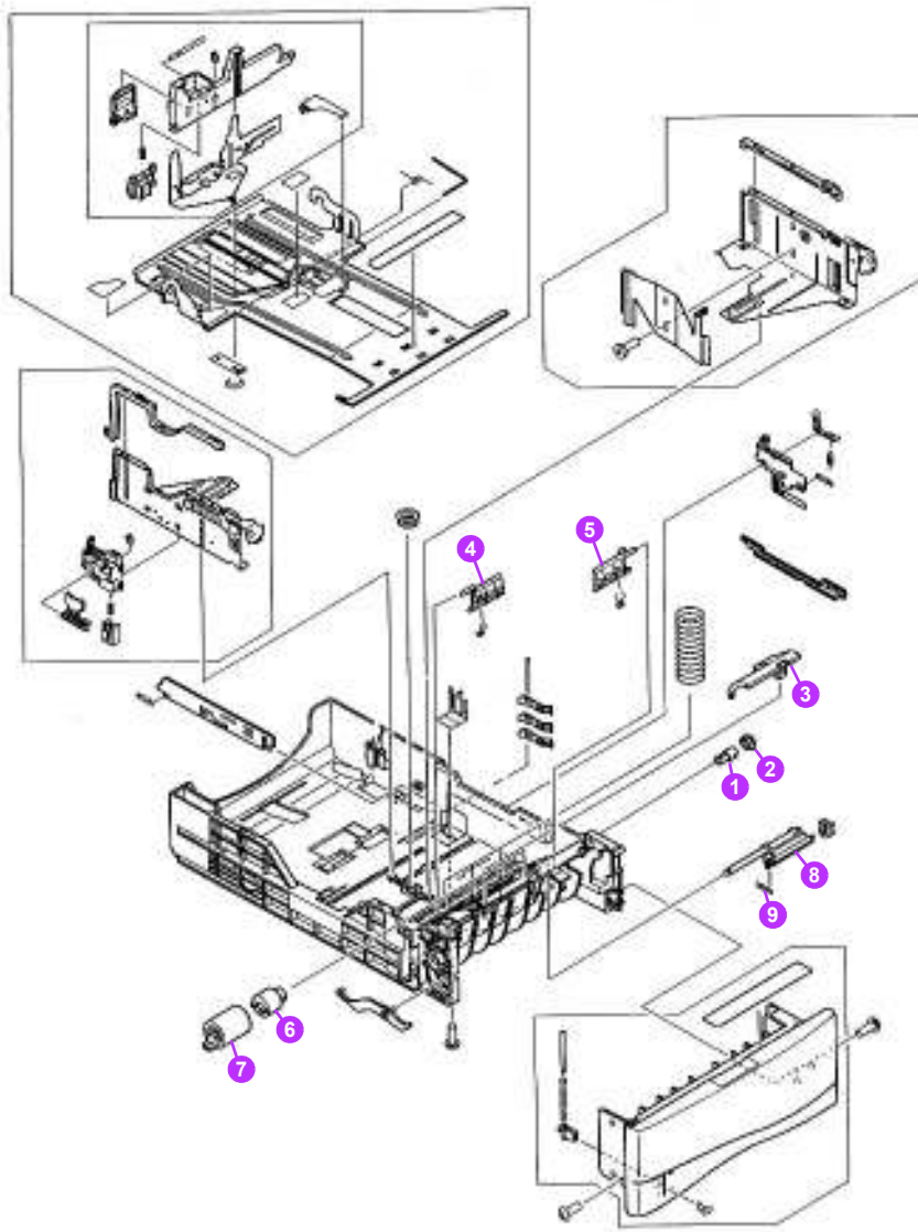
Figure 137. 500-sheet tray
