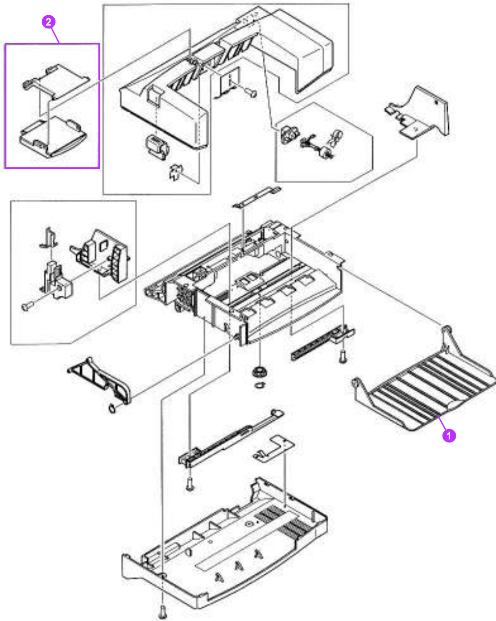
Figure 138. Envelope feeder
