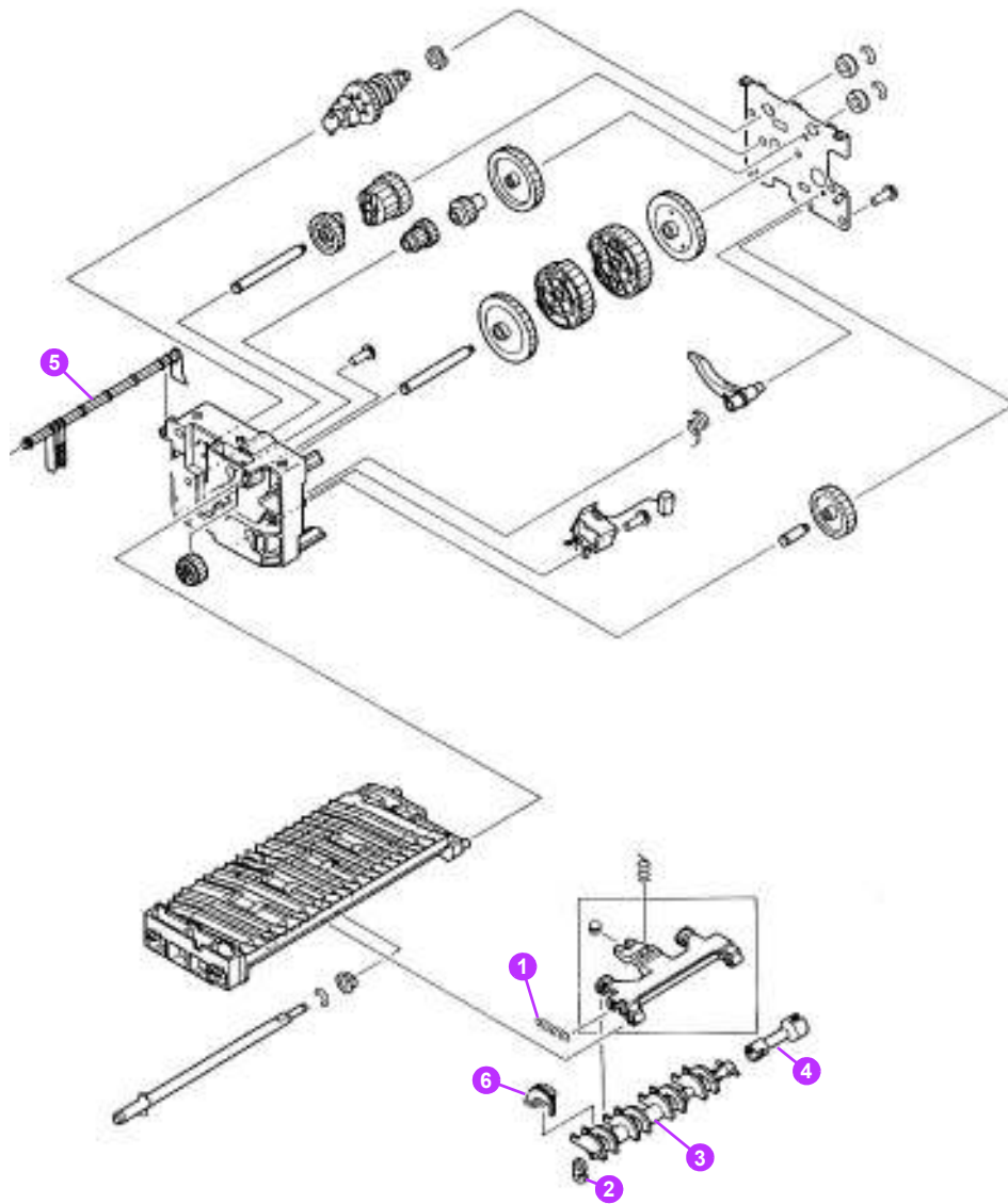
Figure 129. Tray 2 paper pickup guide assembly
