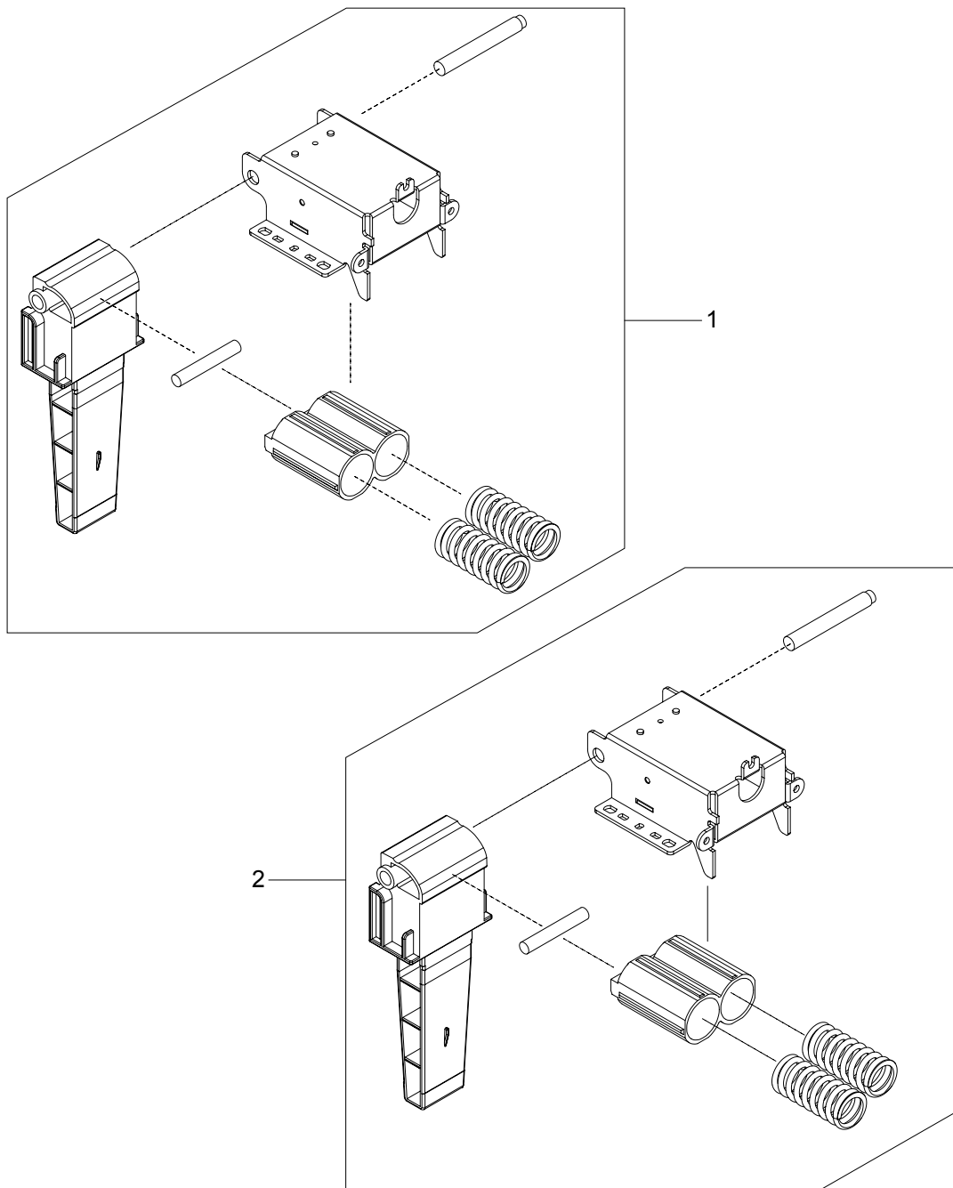
Figure 8-32 ADF internal components (2 of 3)
