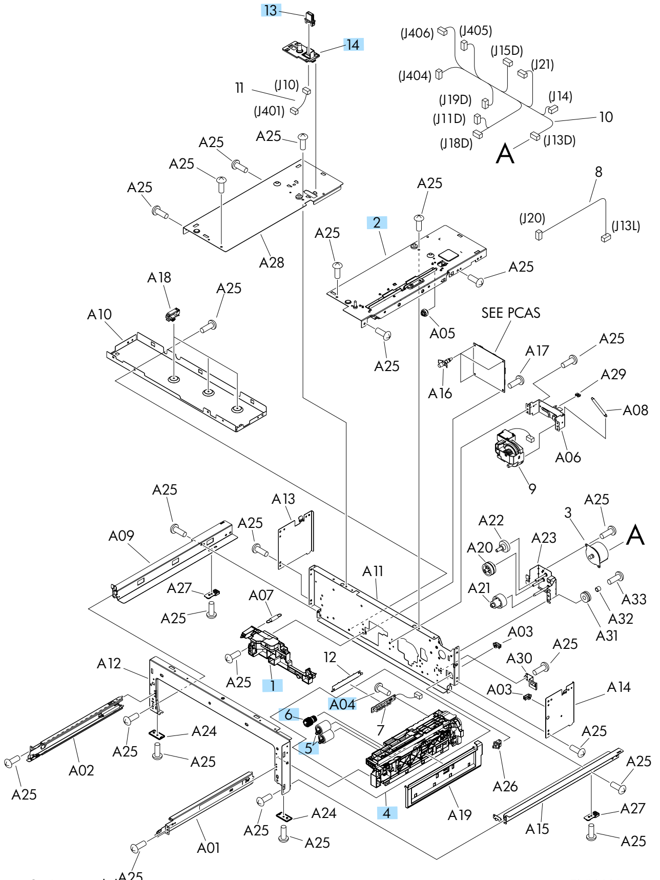
Figure 2-22 Paper feeder main body
