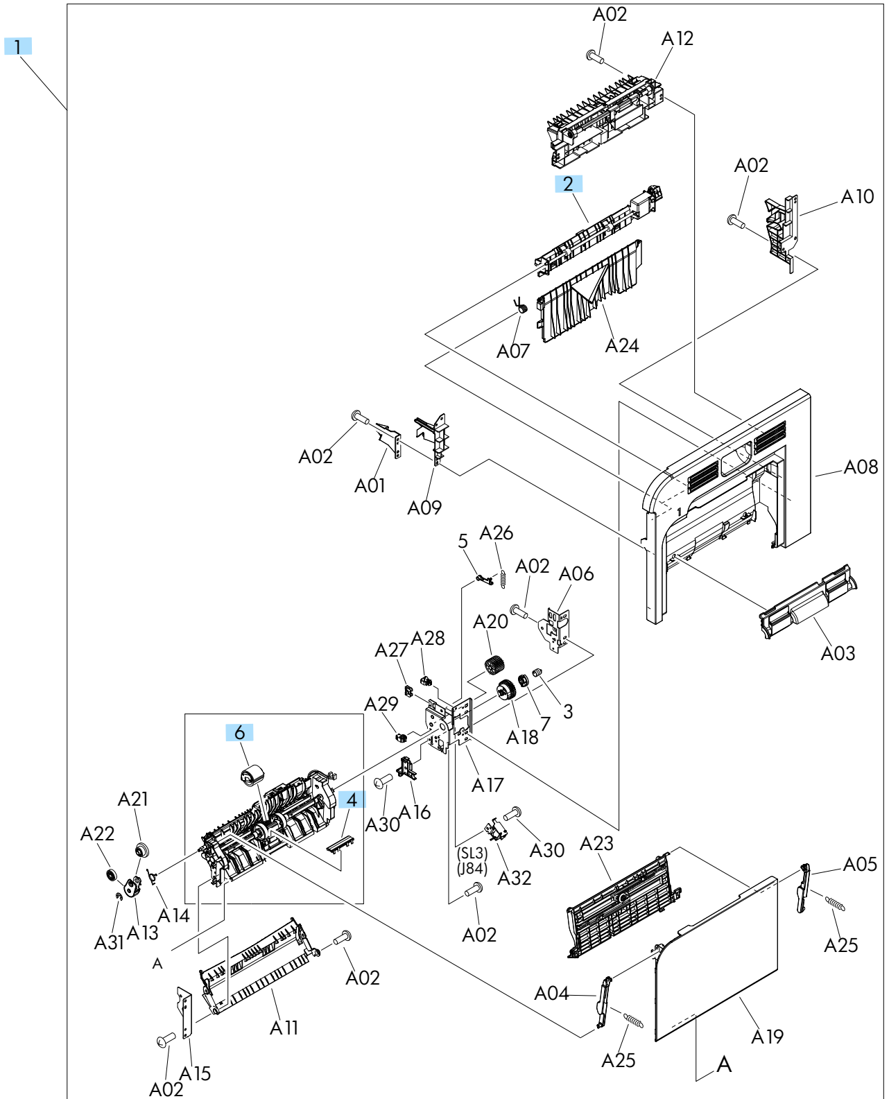
Figure 2-10 Right-door assembly
