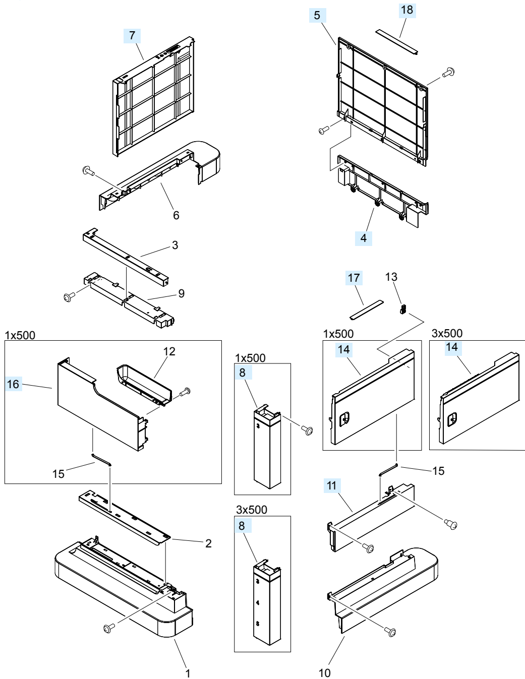
Figure 4-25 Covers (1x500/3x500)
