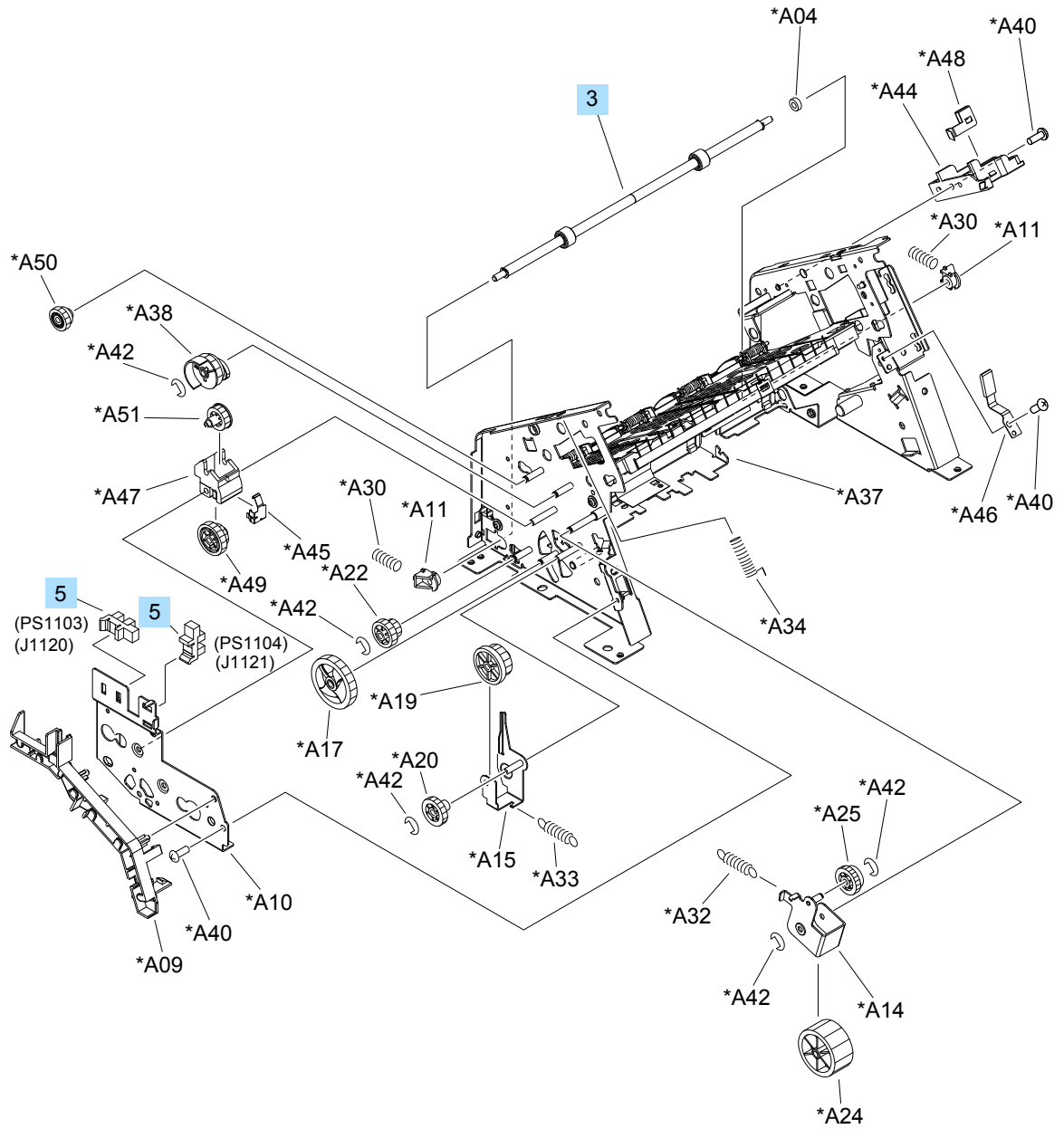
Figure 4-41 Stapler/Stacker middle assembly (2 of 2; S/S)
