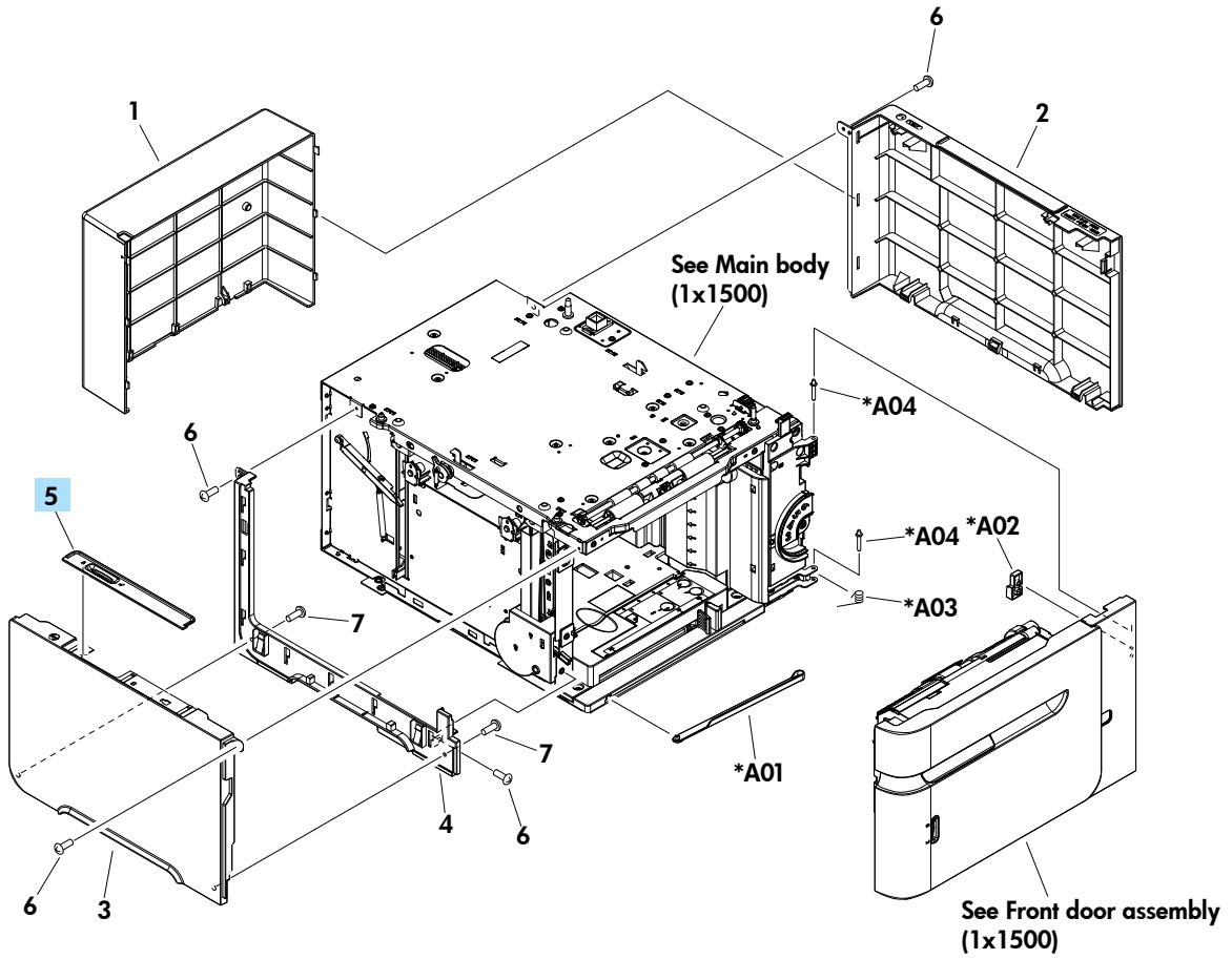
Figure 4-21 Covers (1x1500)
