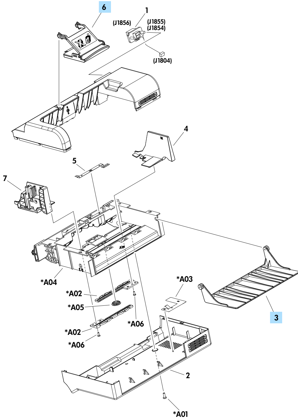
Figure 4-29 Covers (envelope feeder)
