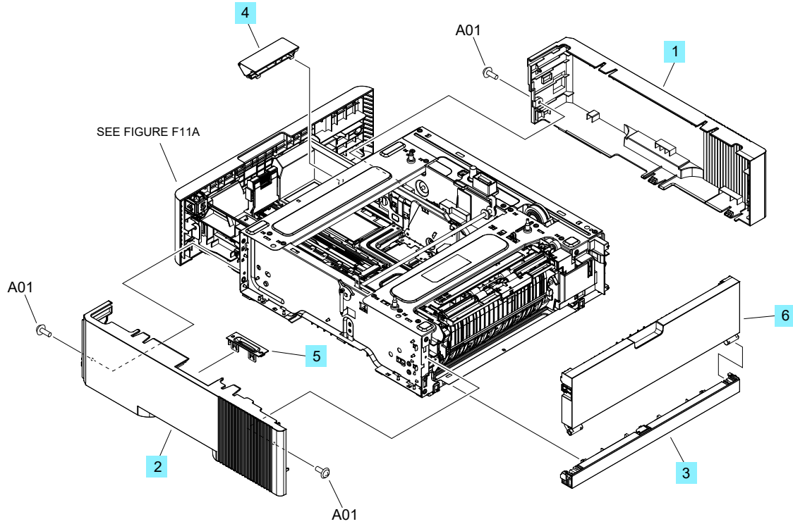
Figure 2-15 550-sheet paper feeder covers (M607, M608, M609)
