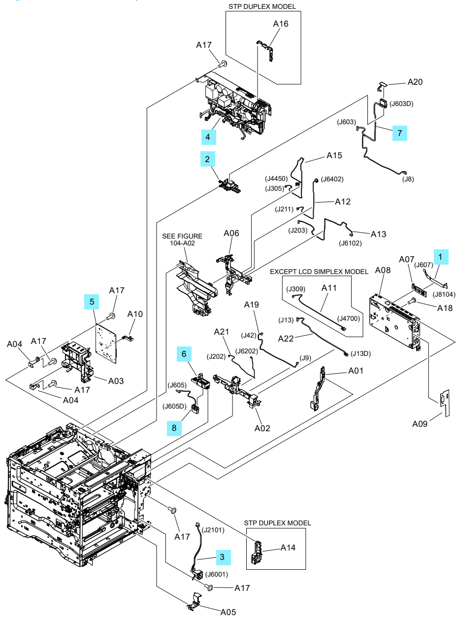
Figure 2-8 Internal components 5 of 6 (M607, M608, M609)
