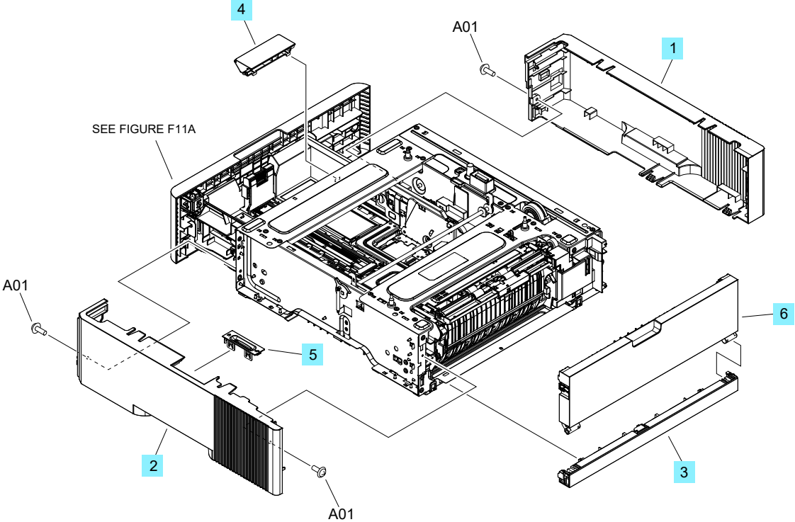
Figure 2-19 Envelope feeder covers (M607, M608, M609)
