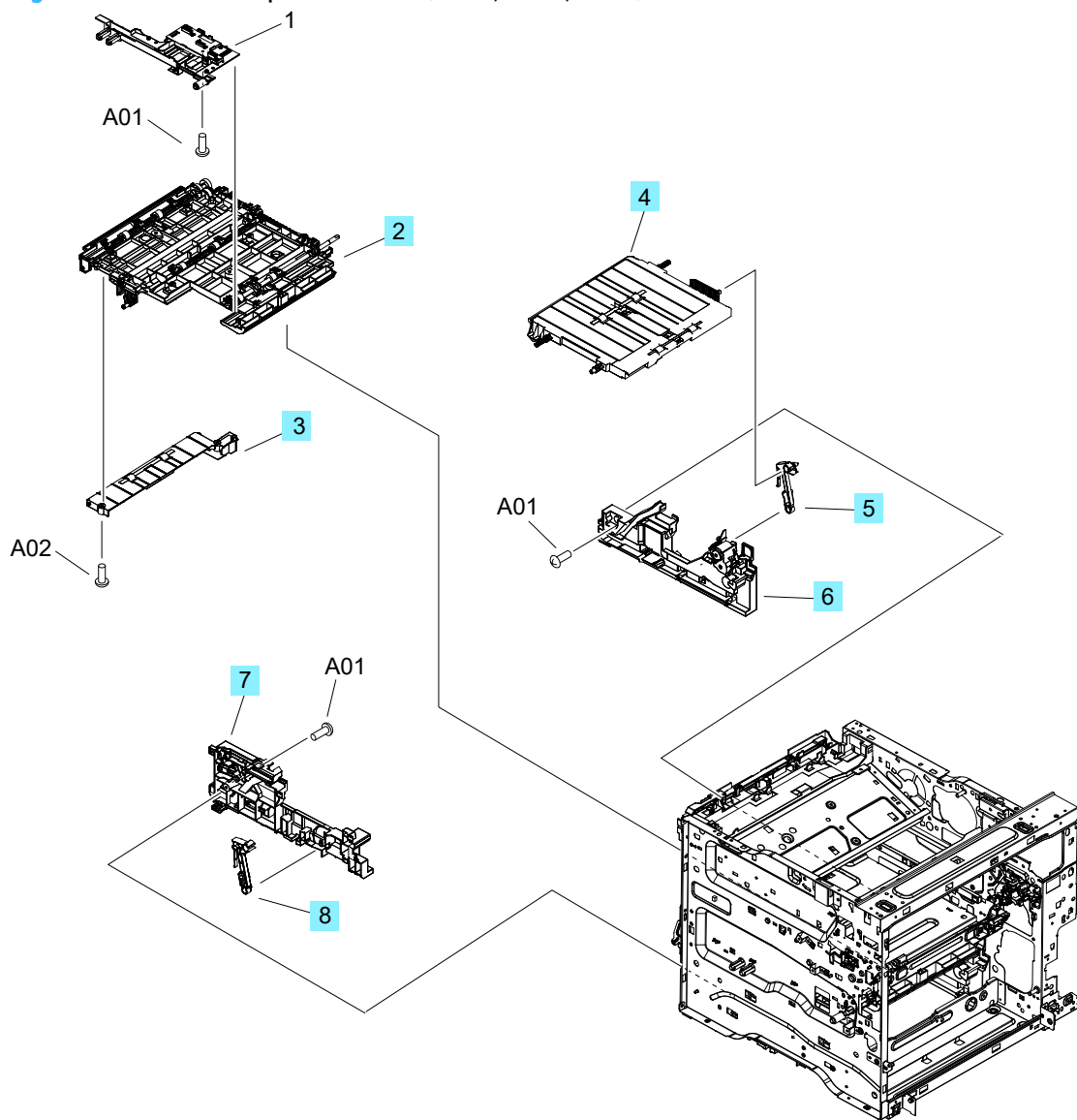
Figure 2-9 Internal components 6 of 6 (M607, M608, M609)
