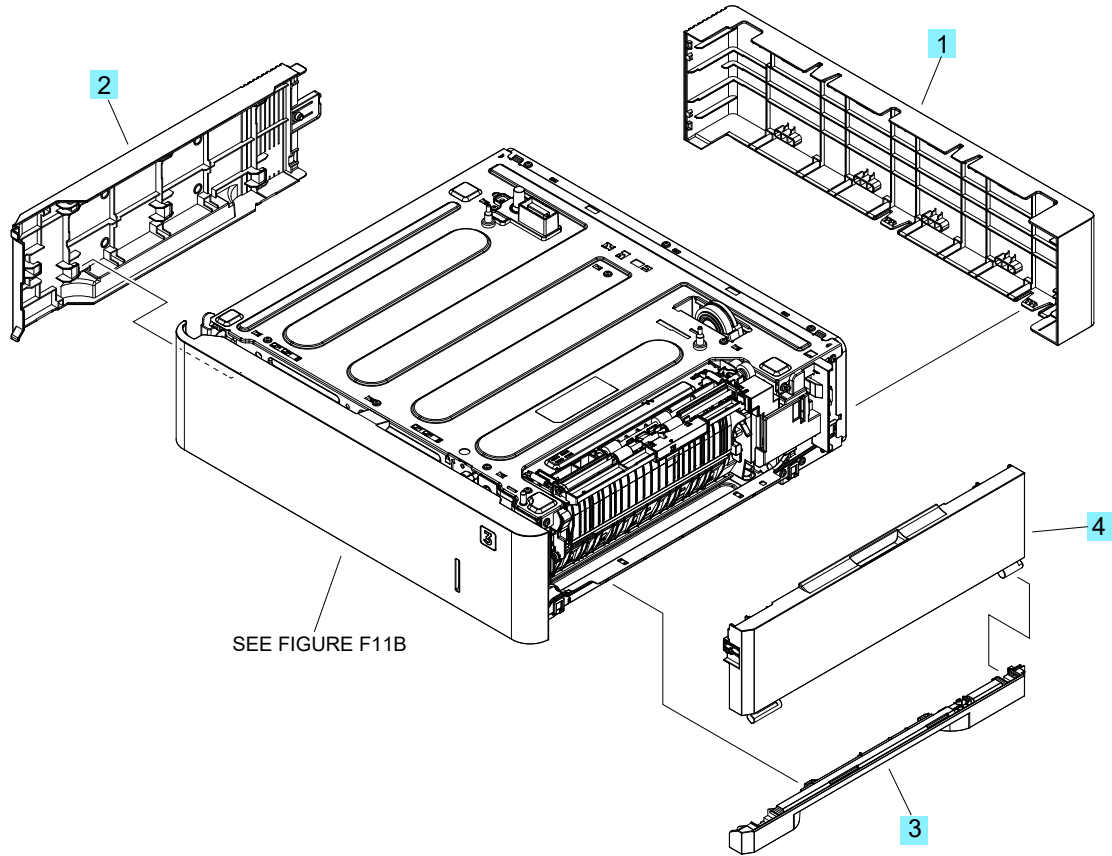
Figure 2-17 550-sheet paper feeder covers (M631, M632, M633)
