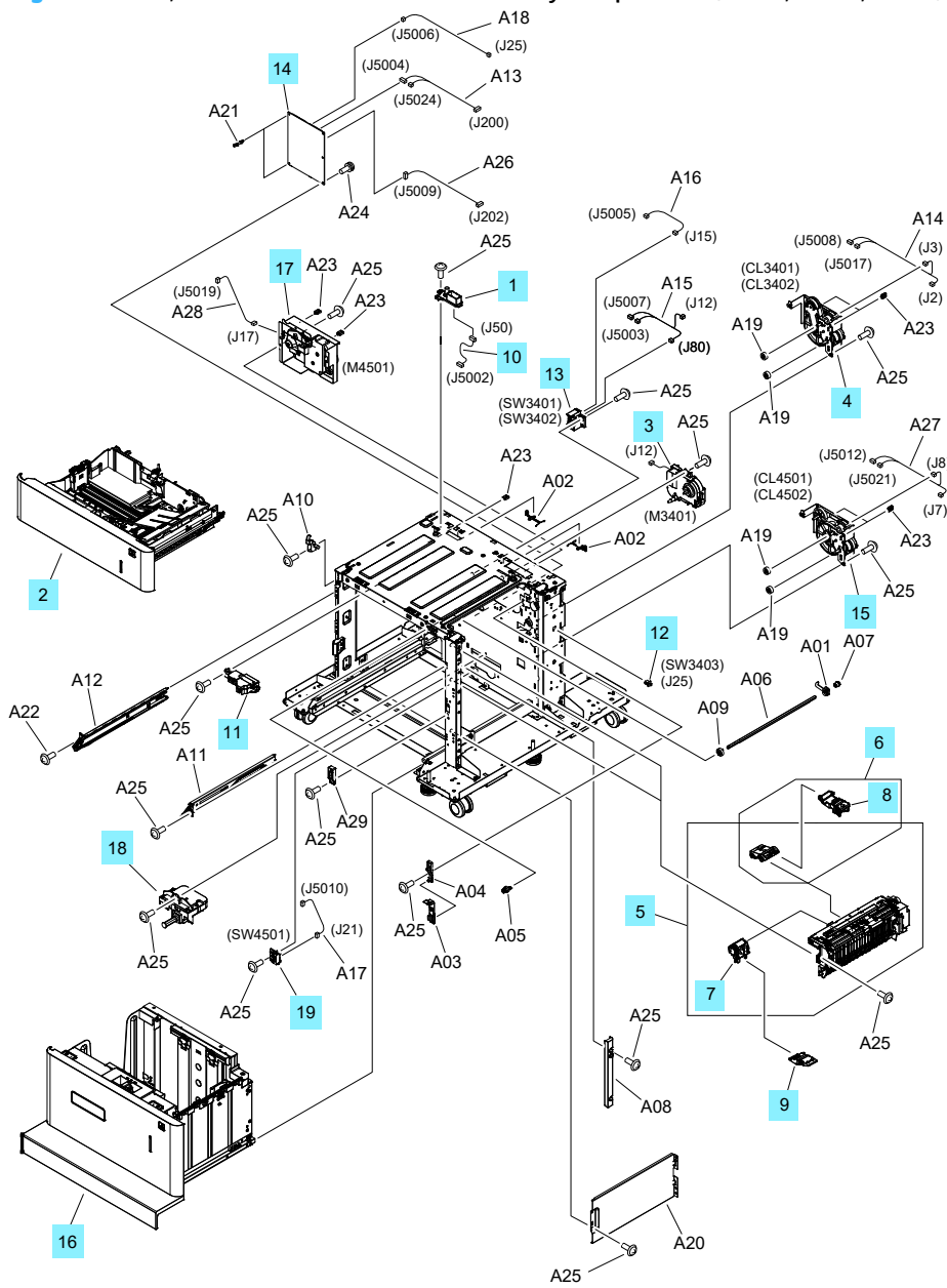
Figure 2-28 2,550 Sheet feeder stand main body components (M631, M632, M633)
