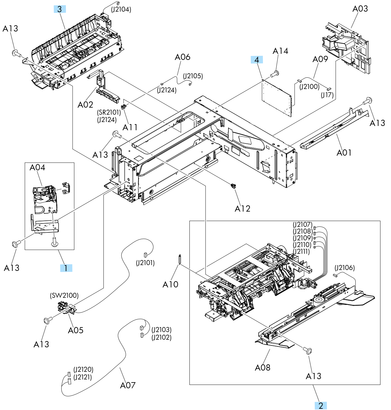
Figure 2-26 Stapler/stacker components
