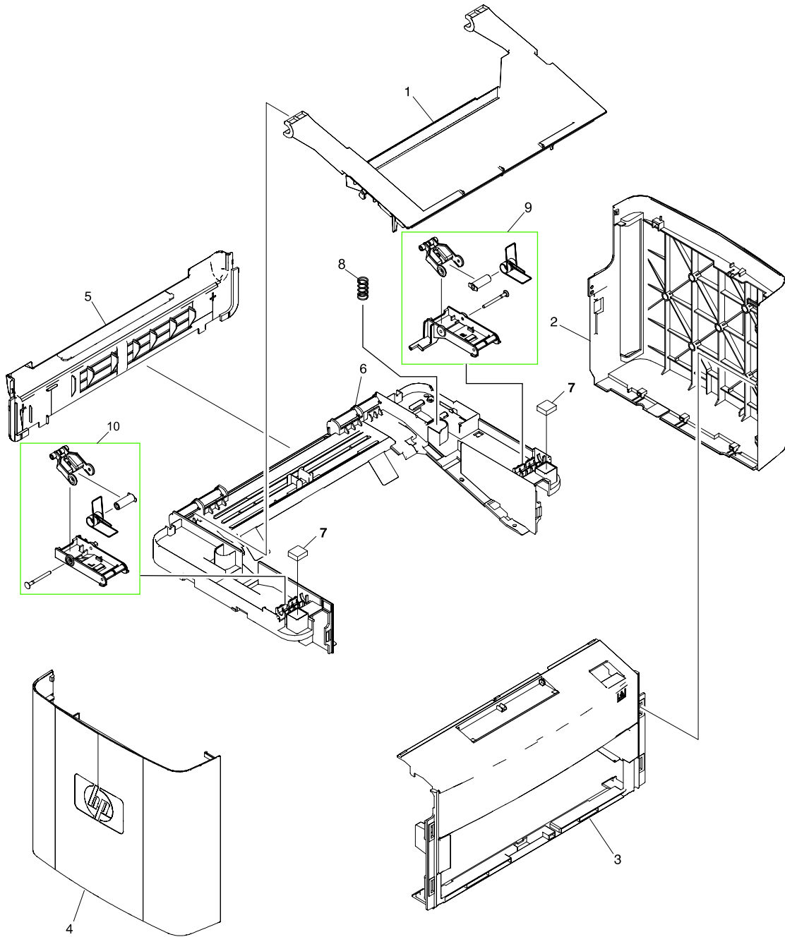
Figure 8-5 External covers
