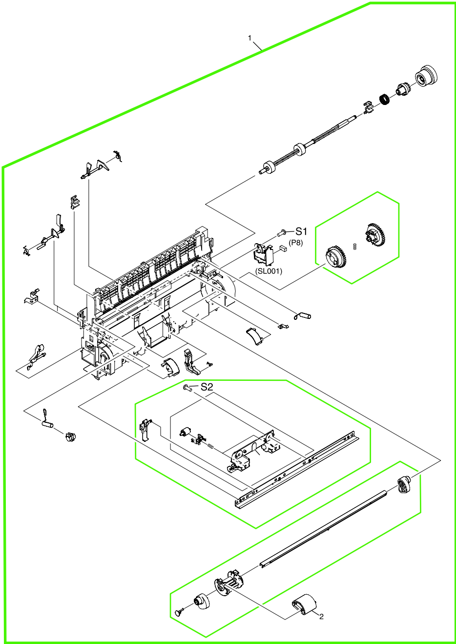
Figure 8-9 Paper-pickup assembly
