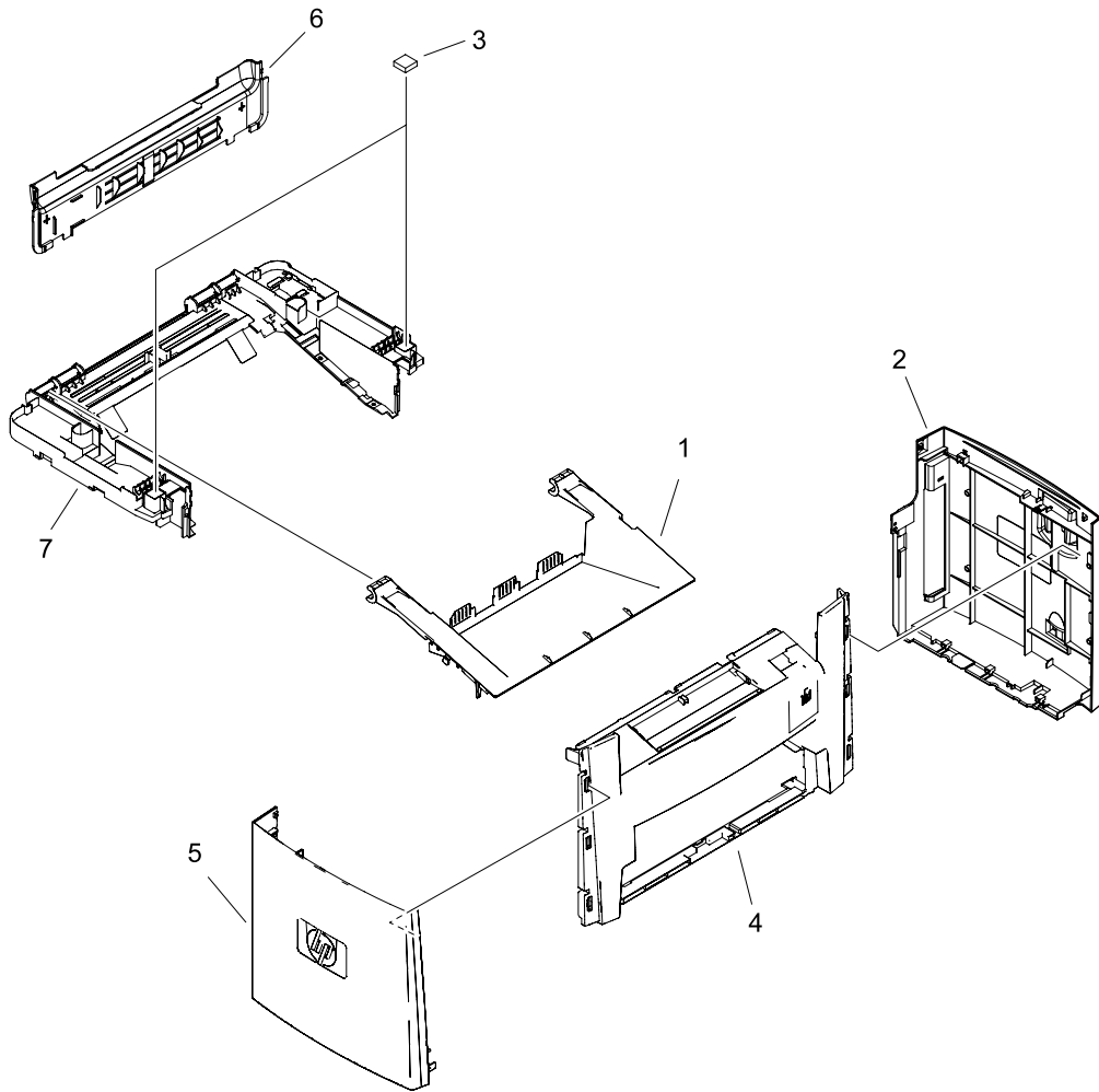
Figure 8-6 External covers
