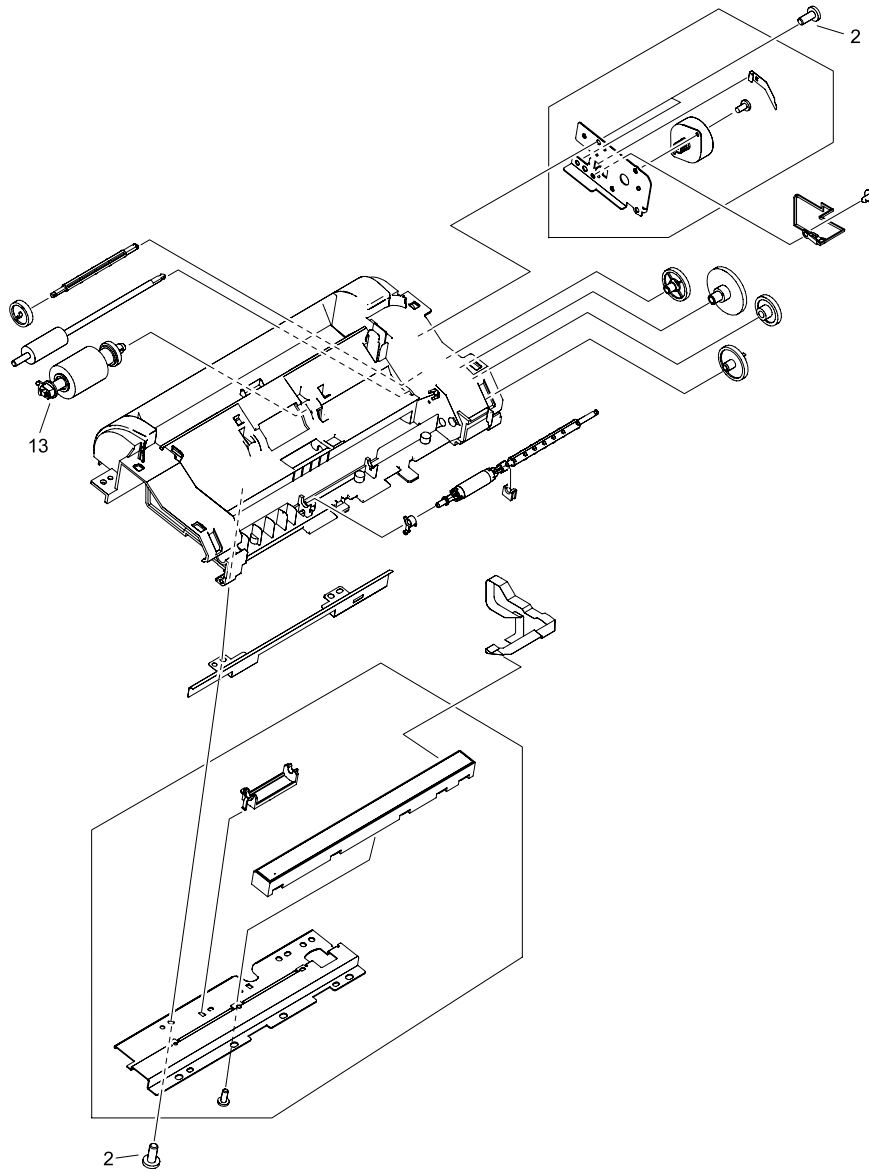
Figure 8-3 Frame assembly
