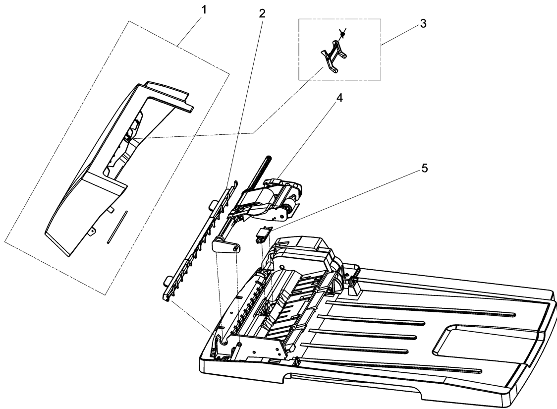
Figure 7-14 ADF components
