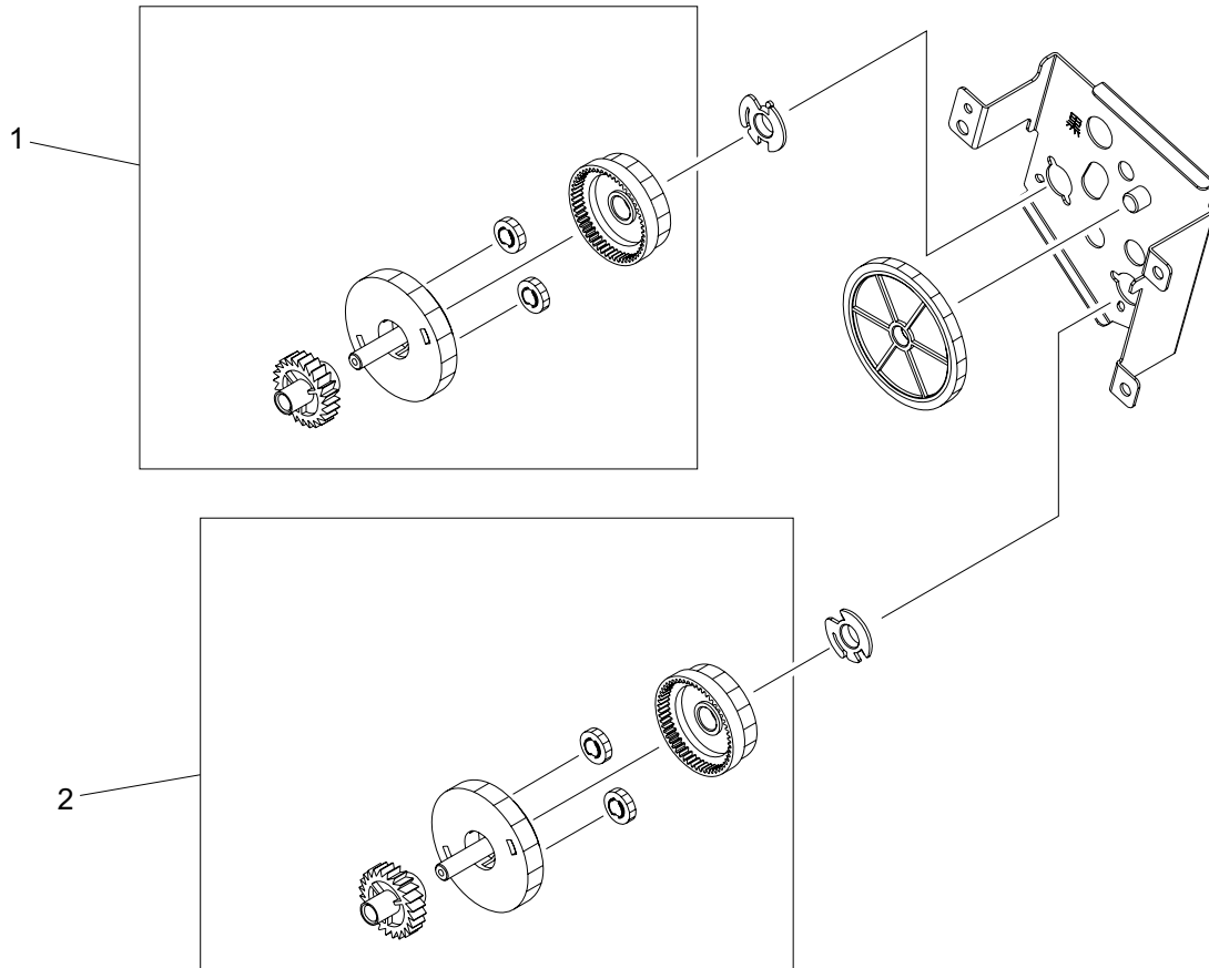
Figure 7-25 Duplexing-drive assembly
