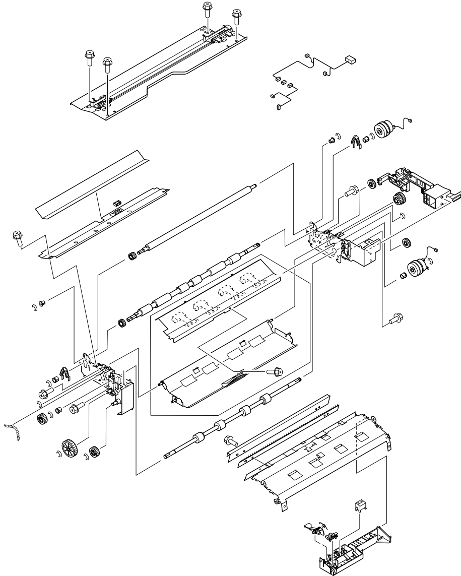
Figure 8-27 Registration assembly
