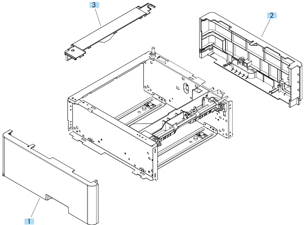
Figure 2-11 Paper feeder covers
