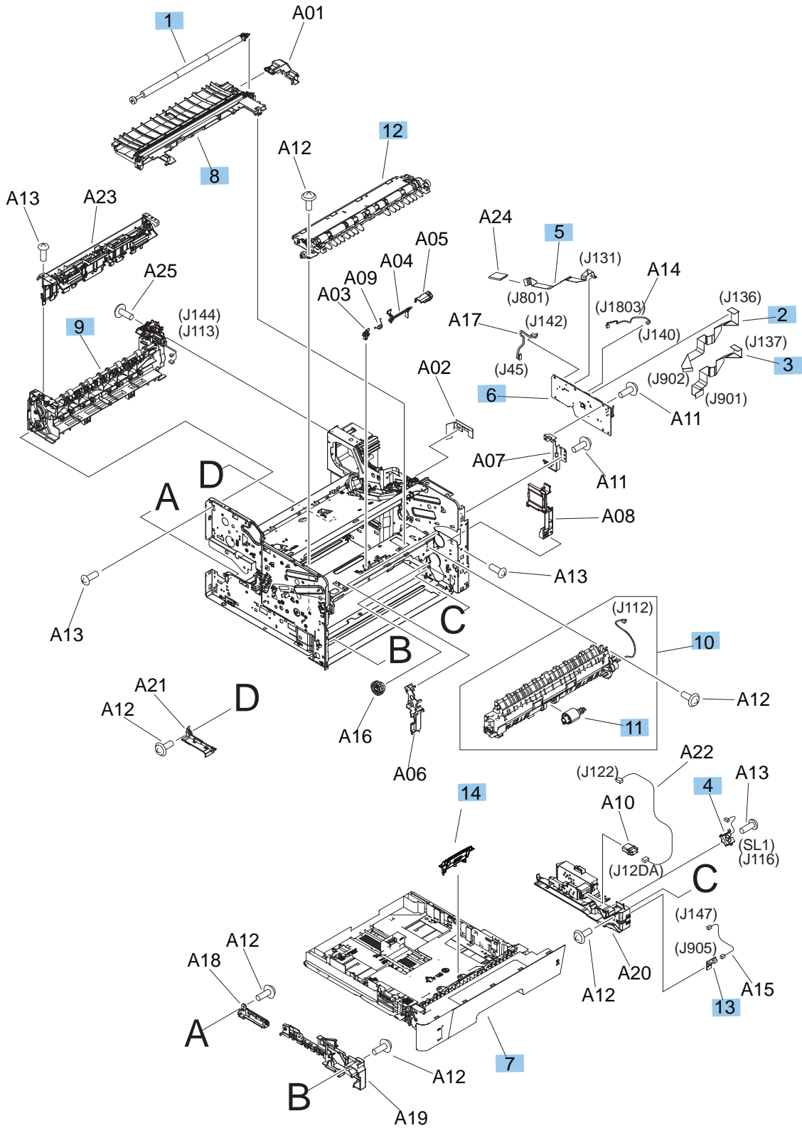
Figure 2-7 Internal components (1 of 3)
