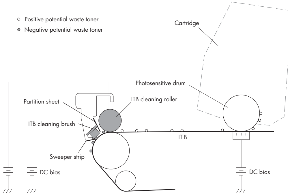
Figure 1-17 ITB cleaning
