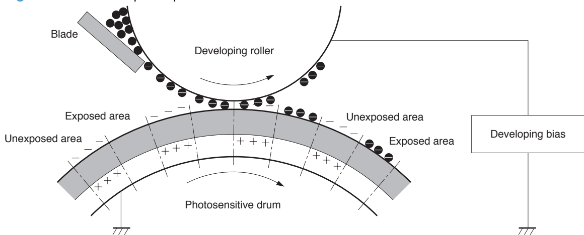
Figure 1-17 Development process
