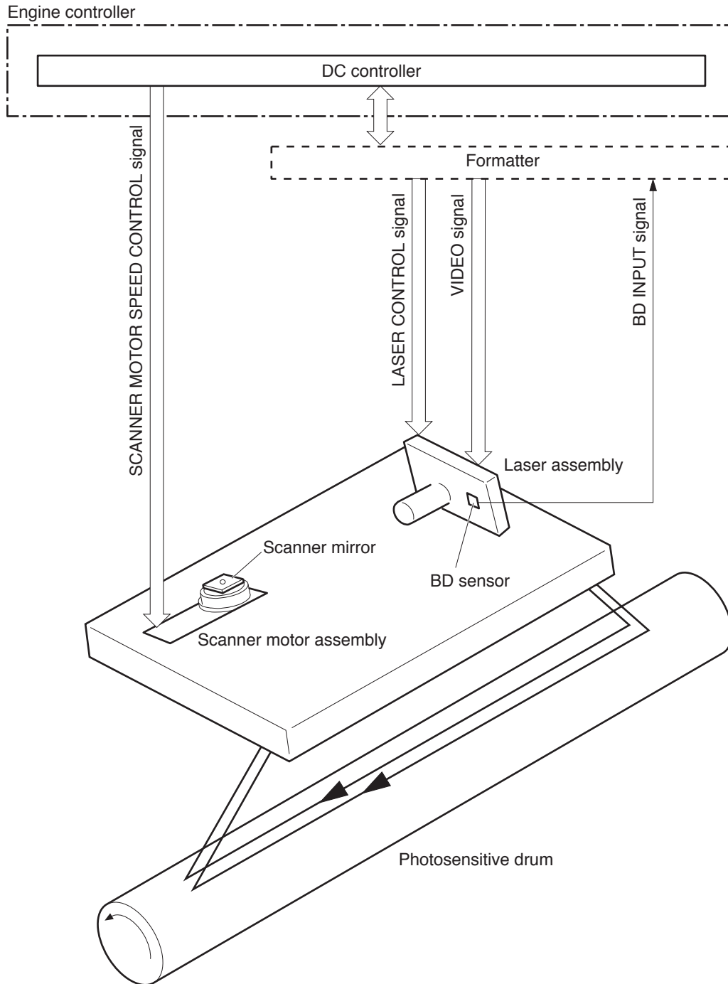
Figure 1-12 Laser scanner system
