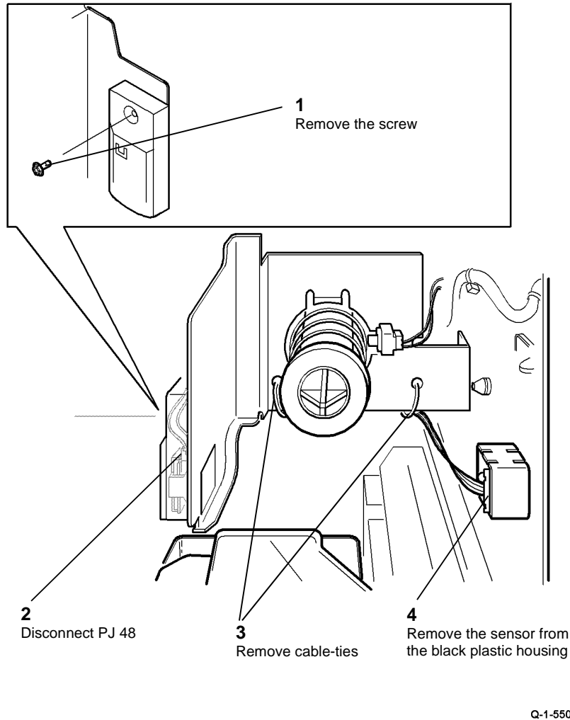
Figure 1 Waste toner full sensor
