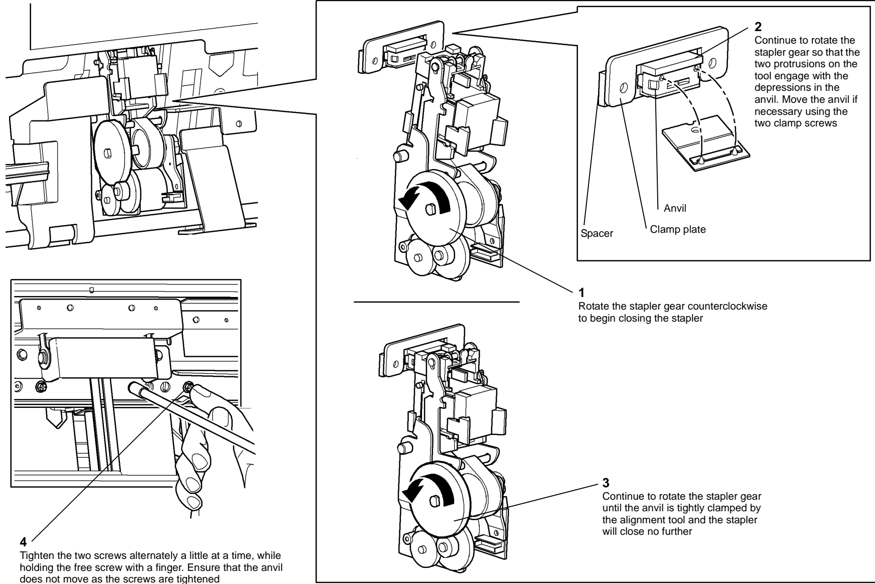
Figure 3 Closing the stapler
