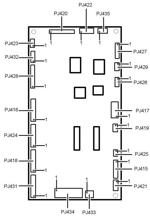
Figure 16 HCSS PWB
