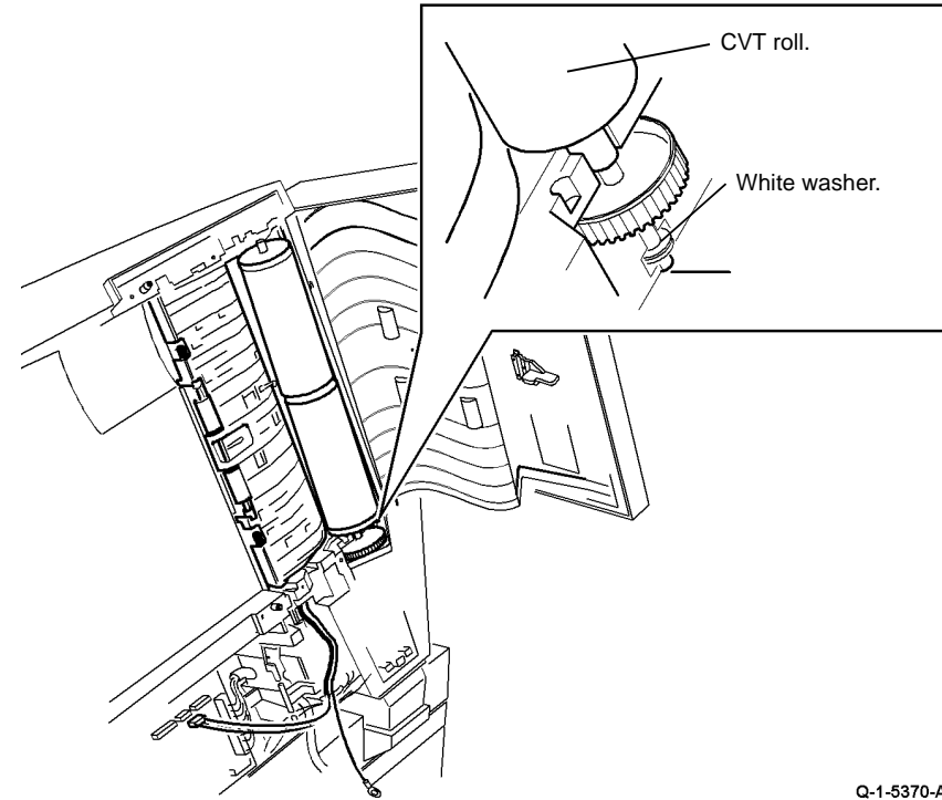
Figure 4 Replacement
