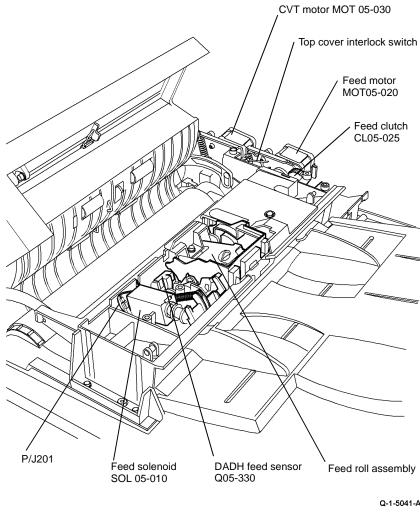
Figure 1 Component location
