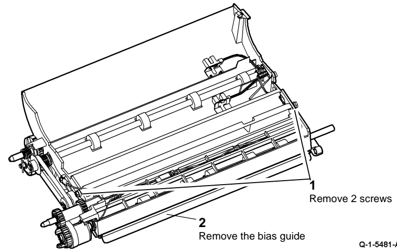
Figure 2 Lower bias guide
