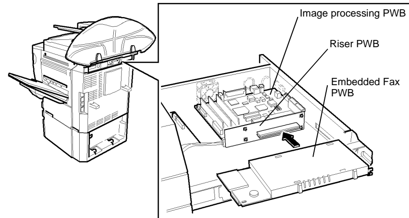
Figure 1 Component location
