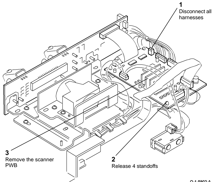
Figure 1 Scanner PWB
