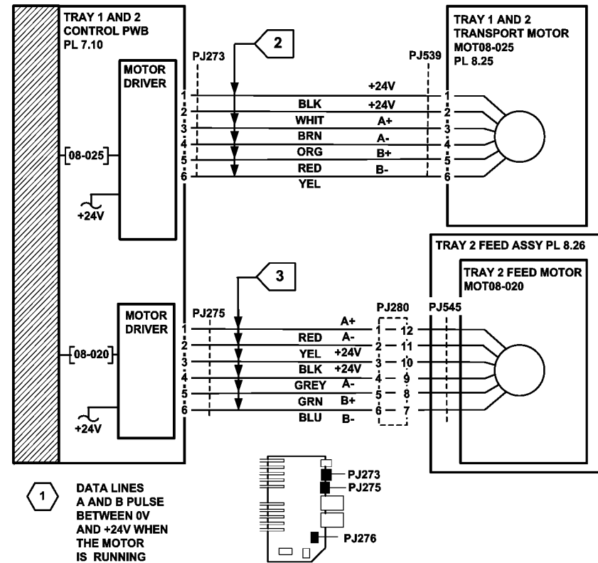
TRAY 1 AND 2 CONTROL PWB
