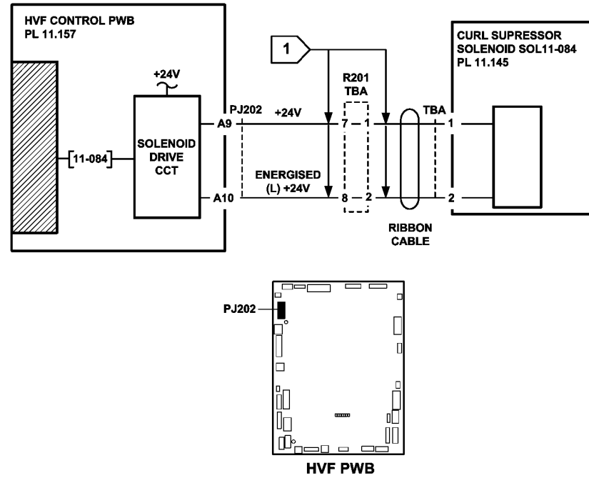
Figure 2 Circuit diagram
