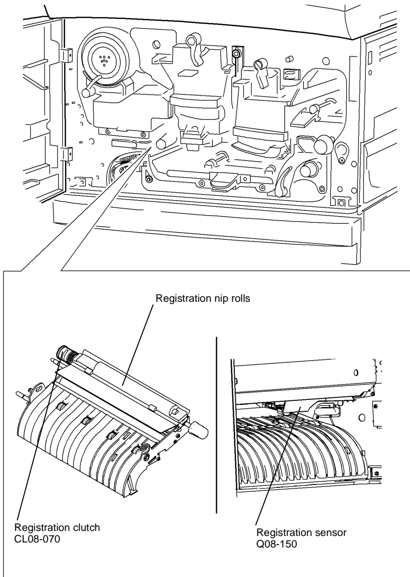
Figure 2 Component location
