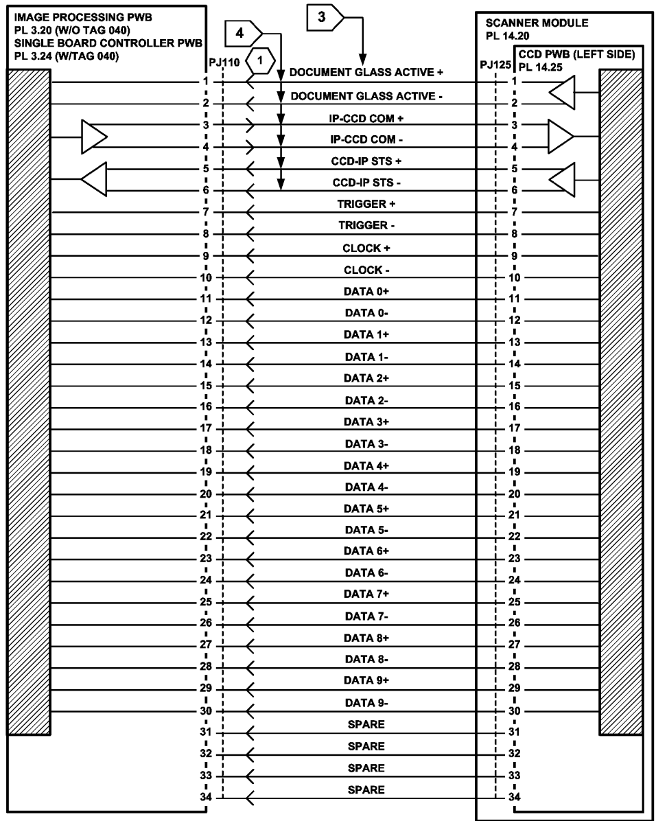
Figure 2 Circuit diagram
