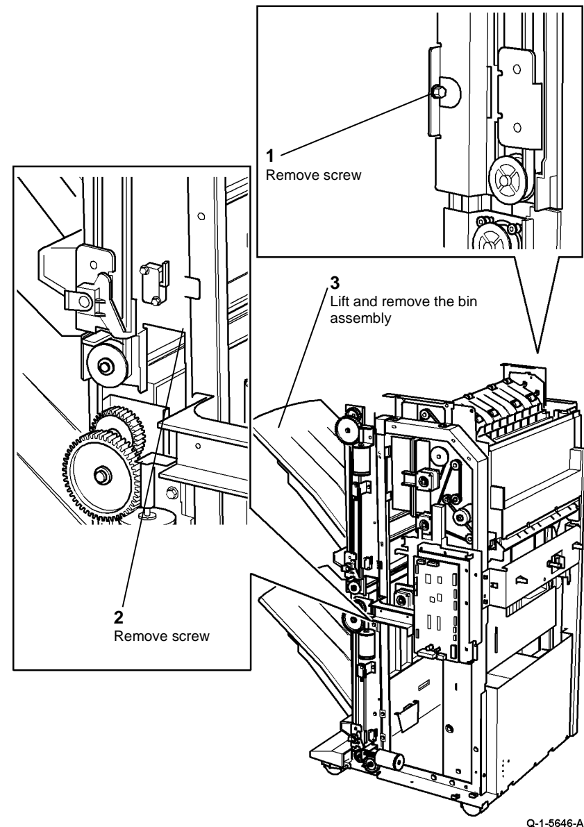
Figure 1 Bin 1 assembly removal
