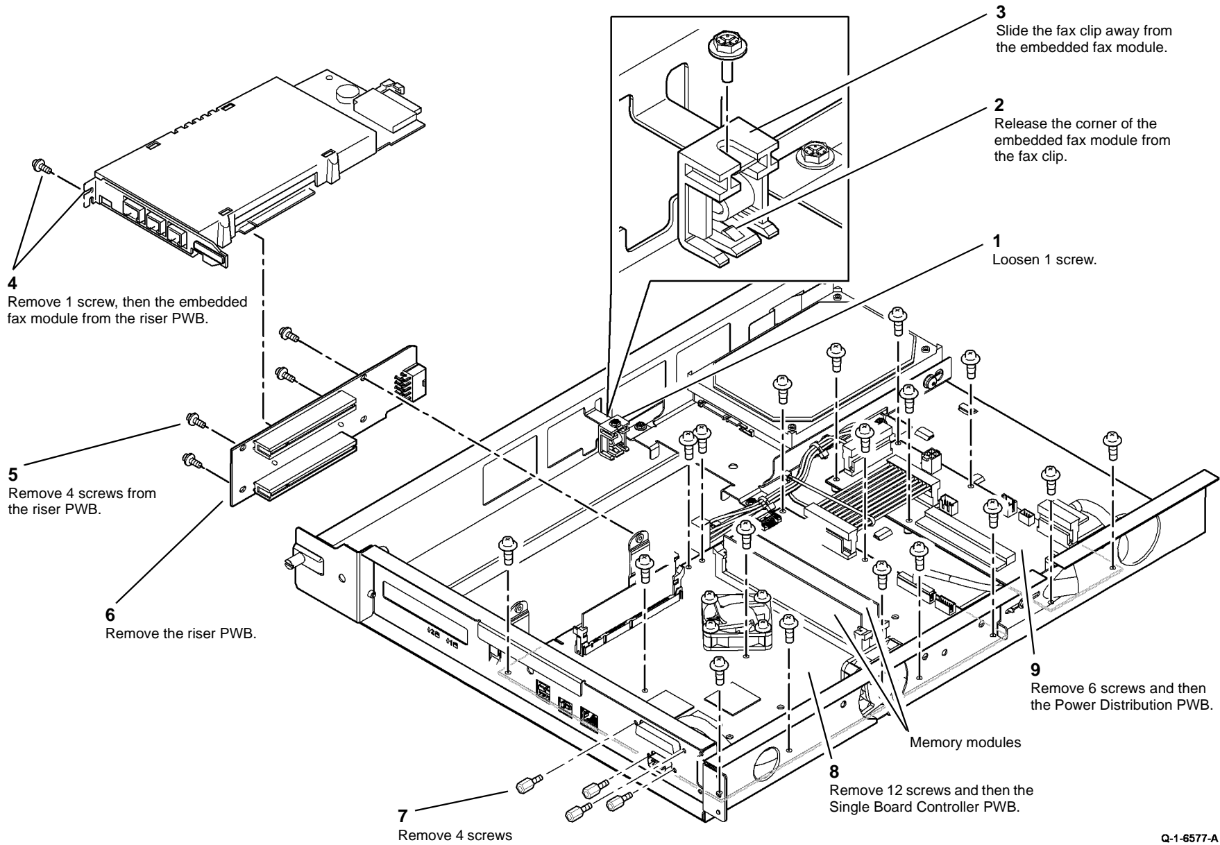
Figure 1 Image processing module
