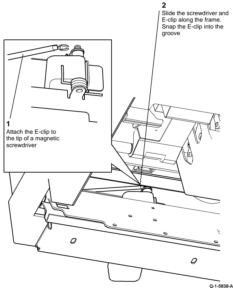
Figure 6 E-clip insertion
