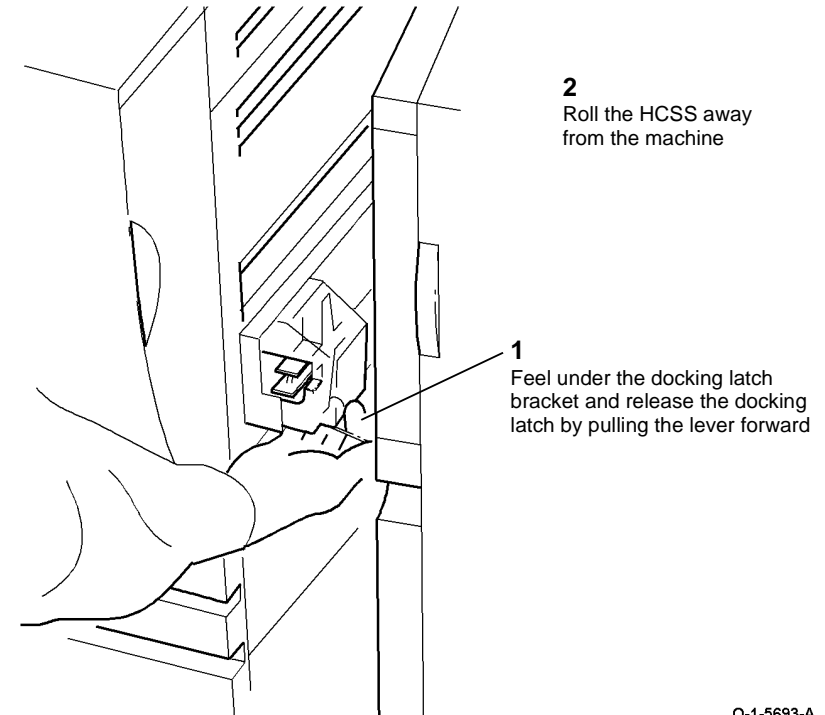
Figure 1 Docking latch location
