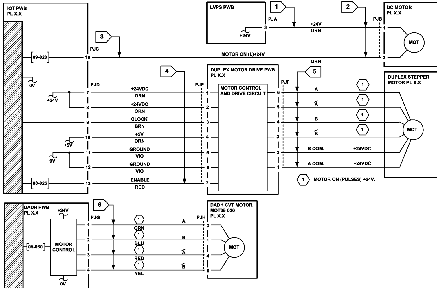
Figure 1 Circuit diagram
