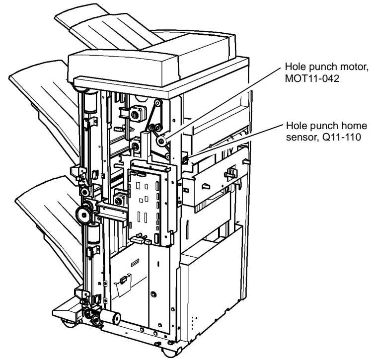
Figure 1 Component location
