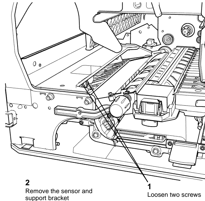
Figure 2 Remove sensor and bracket
