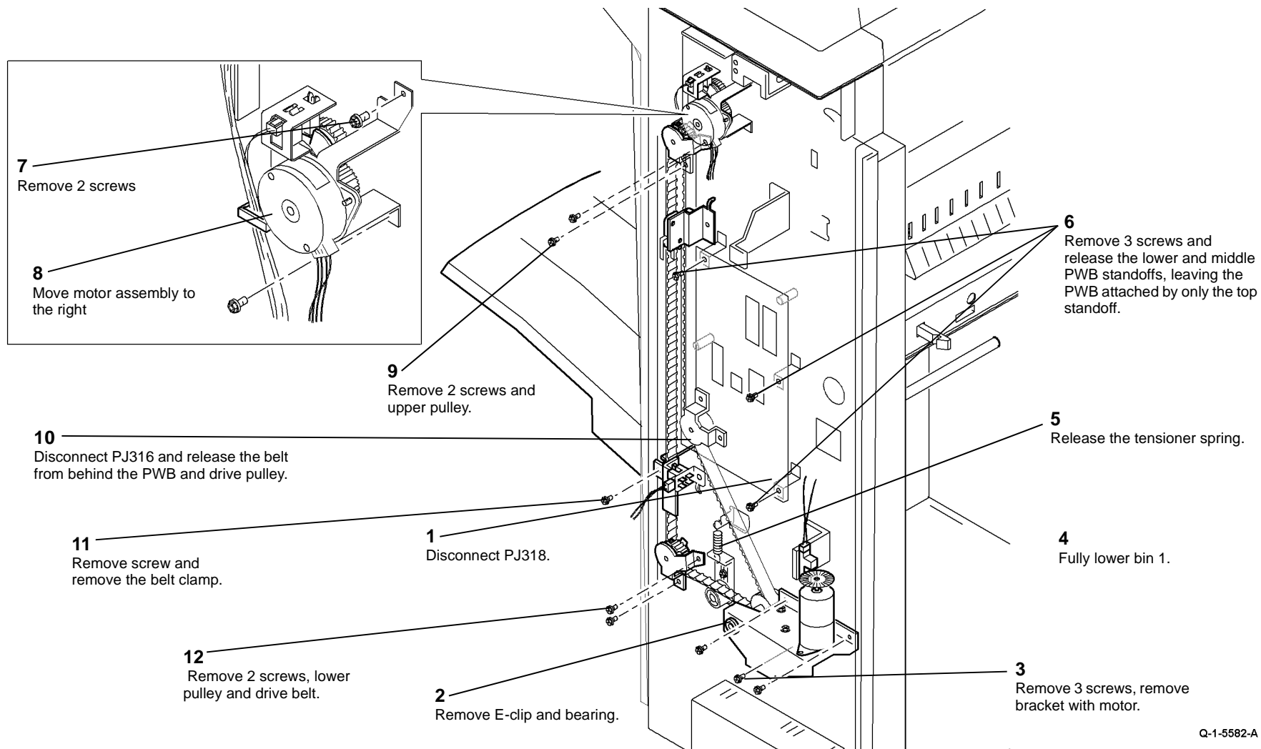
Figure 1 Bin 1 drive belt (rear)
