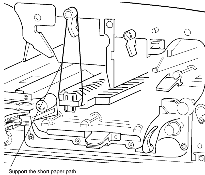
Figure 7 Short paper path assembly
