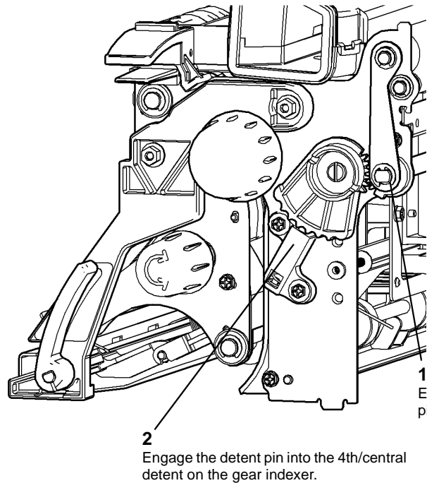
Figure 8 Initial setup of the gear indexer
