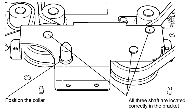
Figure 4 Main drive module support bracket
