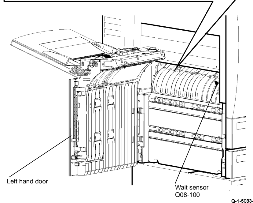
Figure 1 Component location
