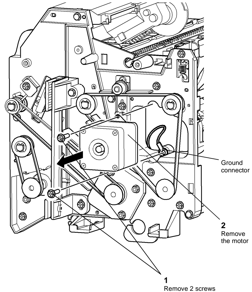
Figure 1 Motor removal
