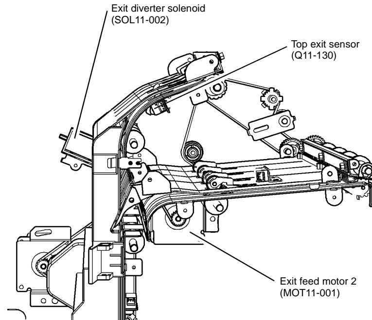
Figure 1 Component location
