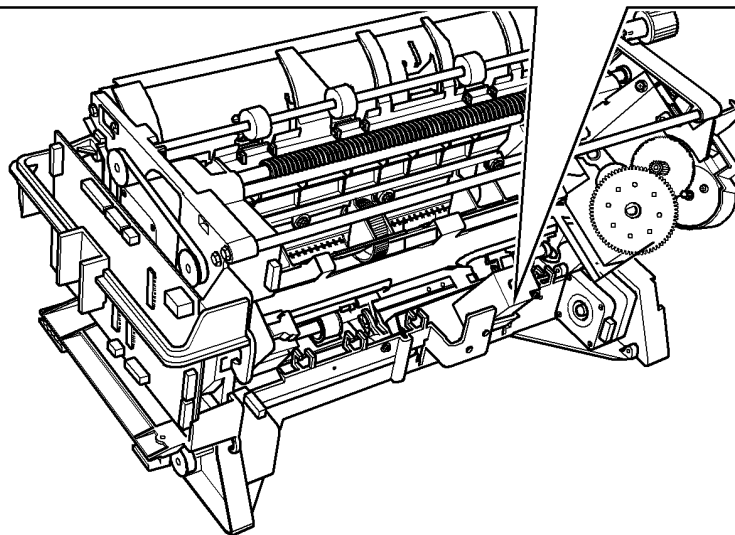
Figure 1 Removal
