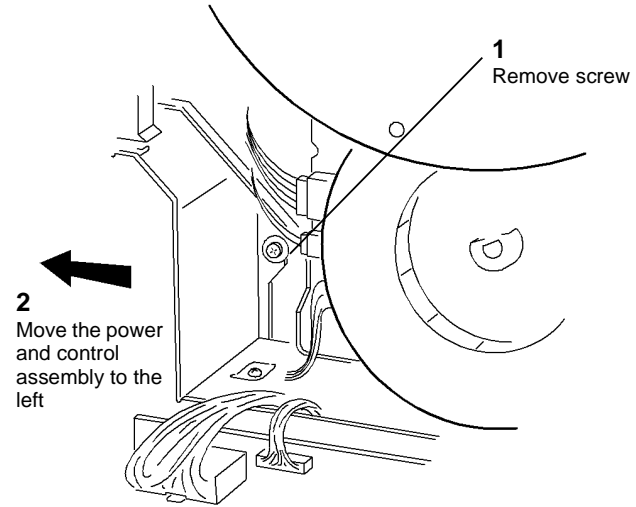
Figure 3 Power and control assembly
