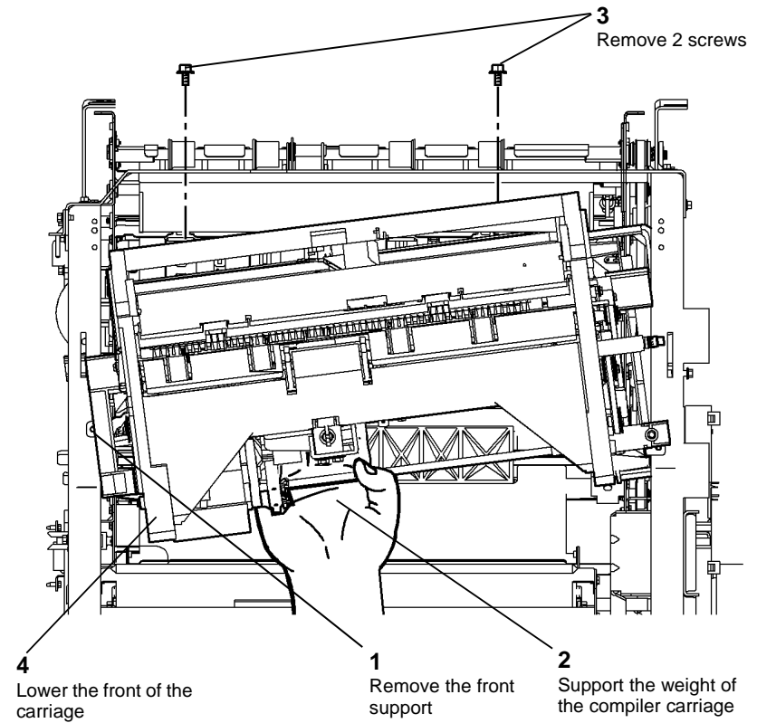
Figure 1 Carriage position
