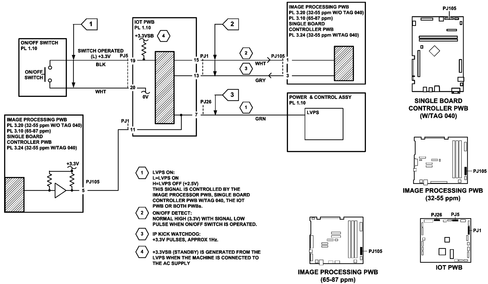
Figure 1 Circuit diagram
