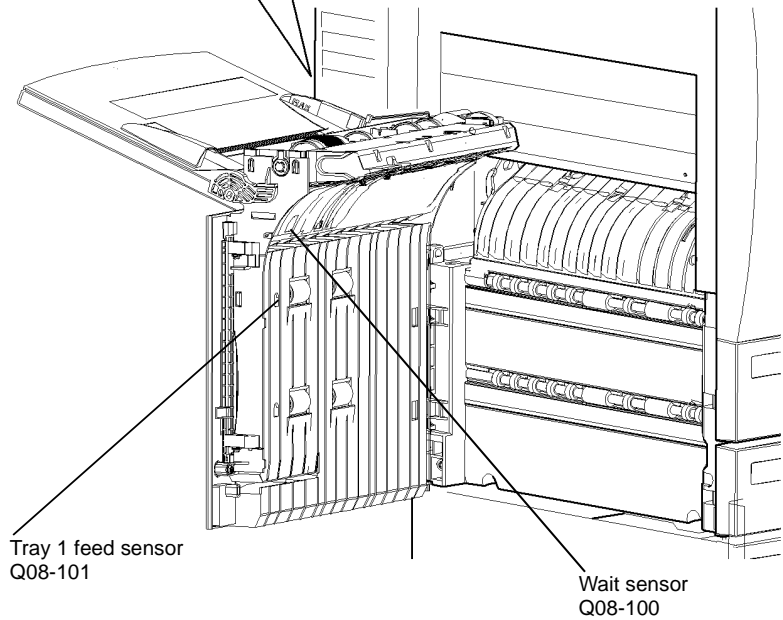
Figure 1 Component location
