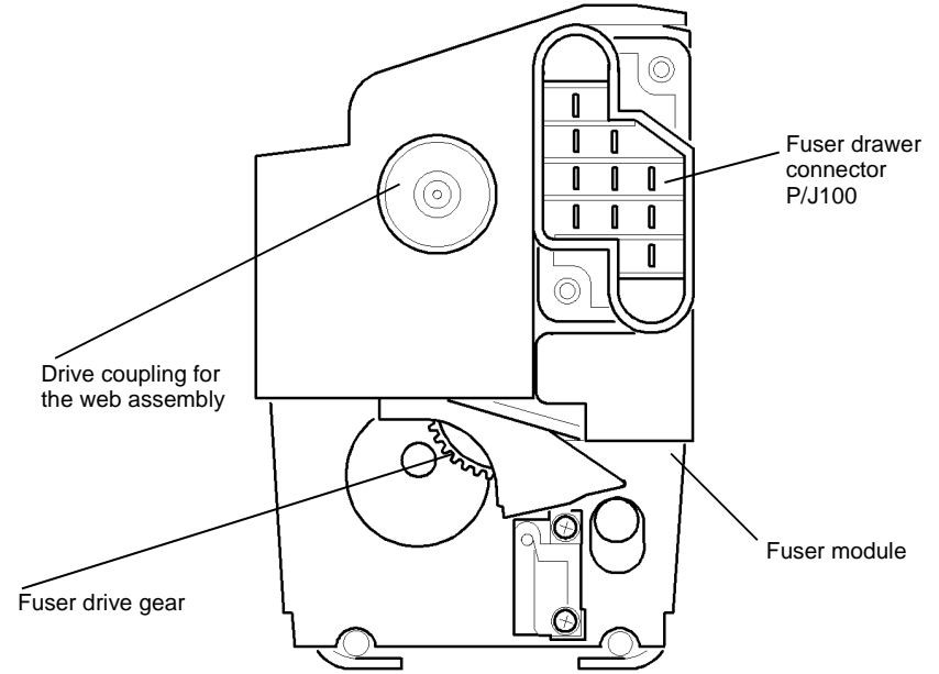
Figure 2 Component location
