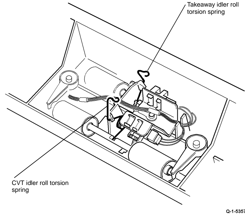
Figure 2 Torsion springs
