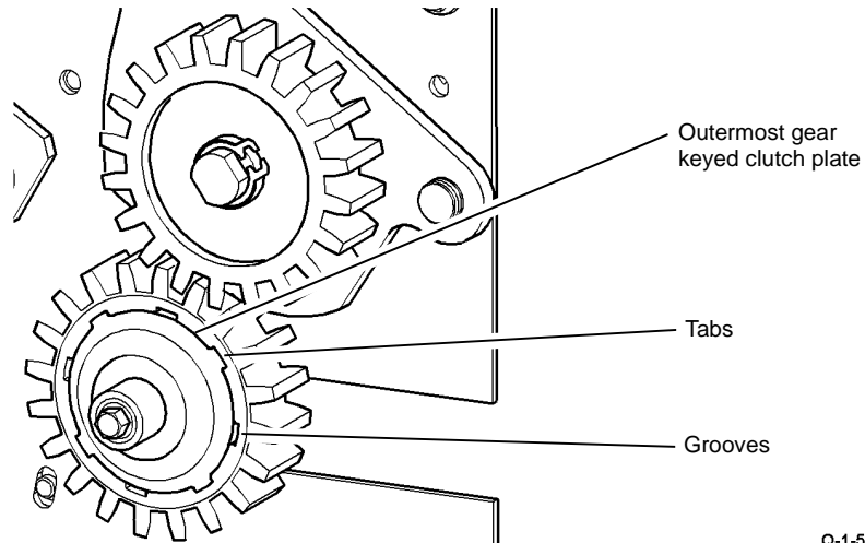
Figure 7 Outermost gear keyed clutch plate
