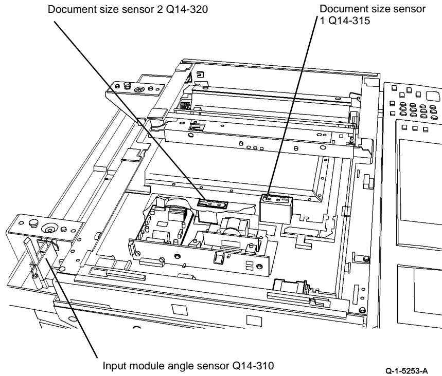
Figure 1 Component location
