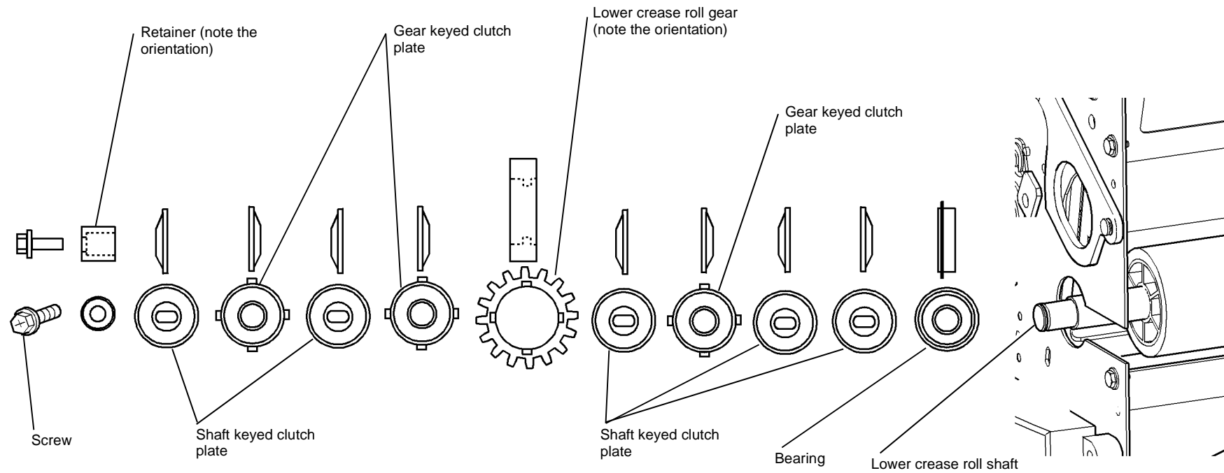
Figure 6 Clutch components
