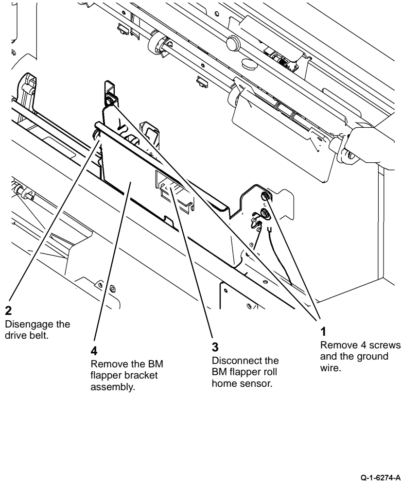
Figure 1 Remove the BM flapper bracket
