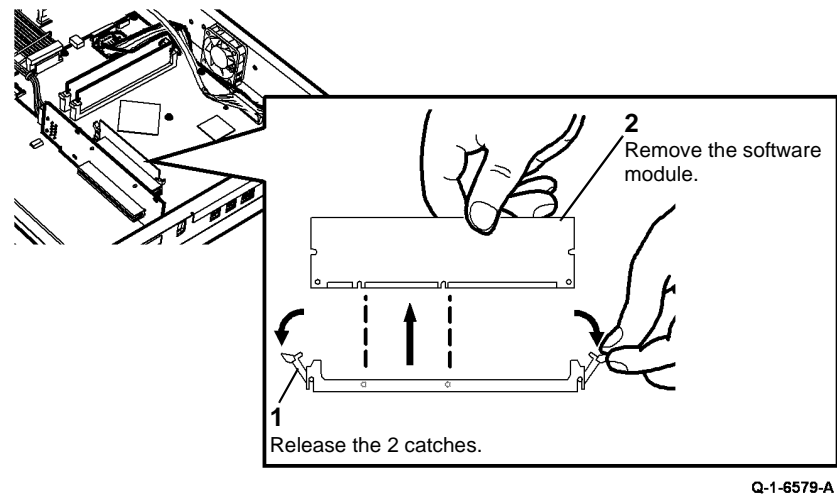
Figure 2 Software module removal W/TAG 040
