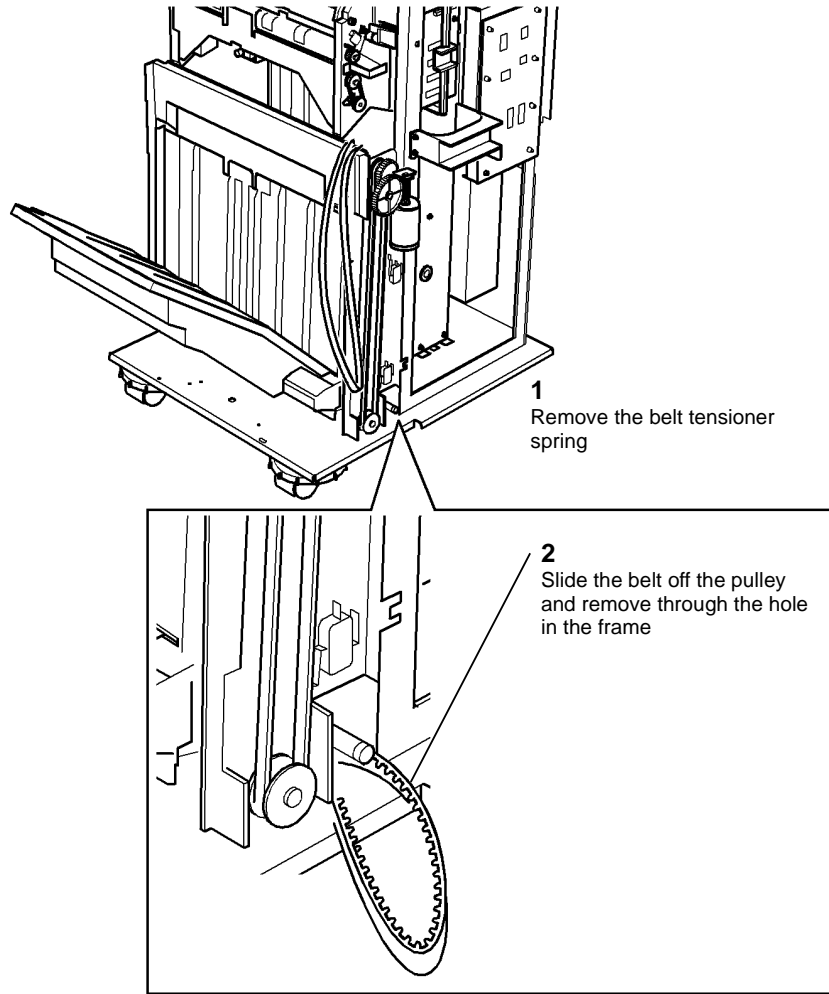
Figure 7 Elevator belt removal
