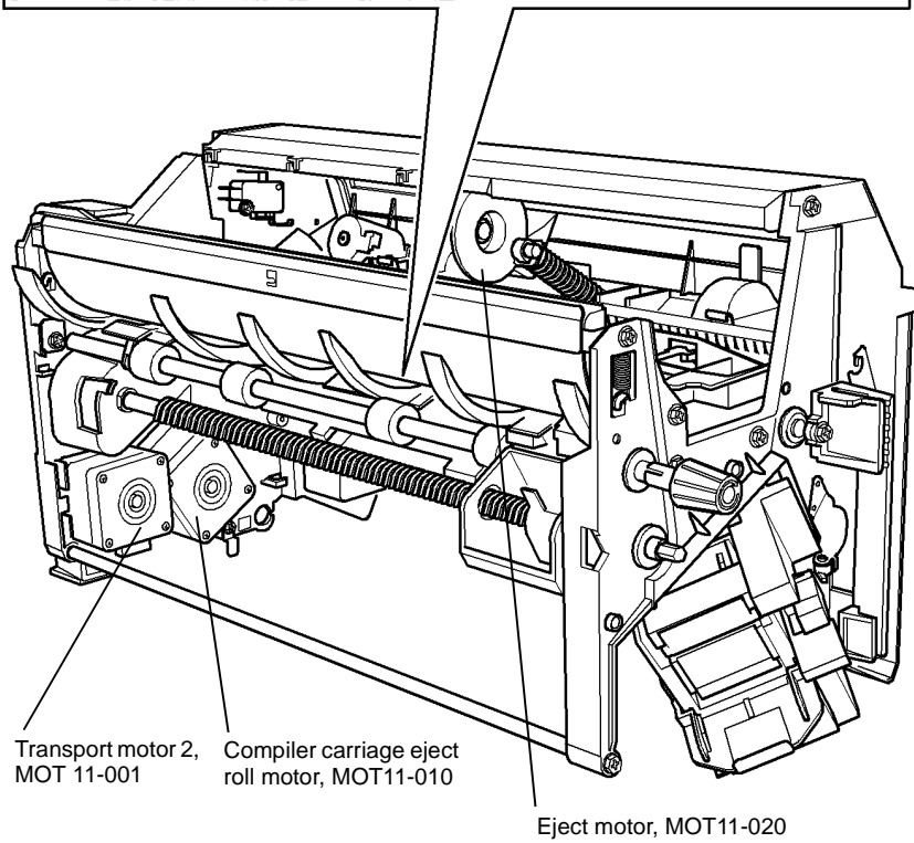
Figure 1 Component location
