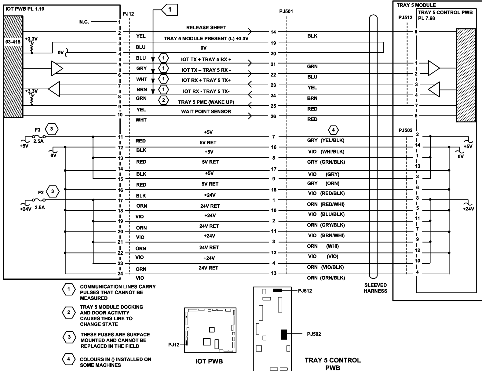
Figure 1 Circuit diagram
