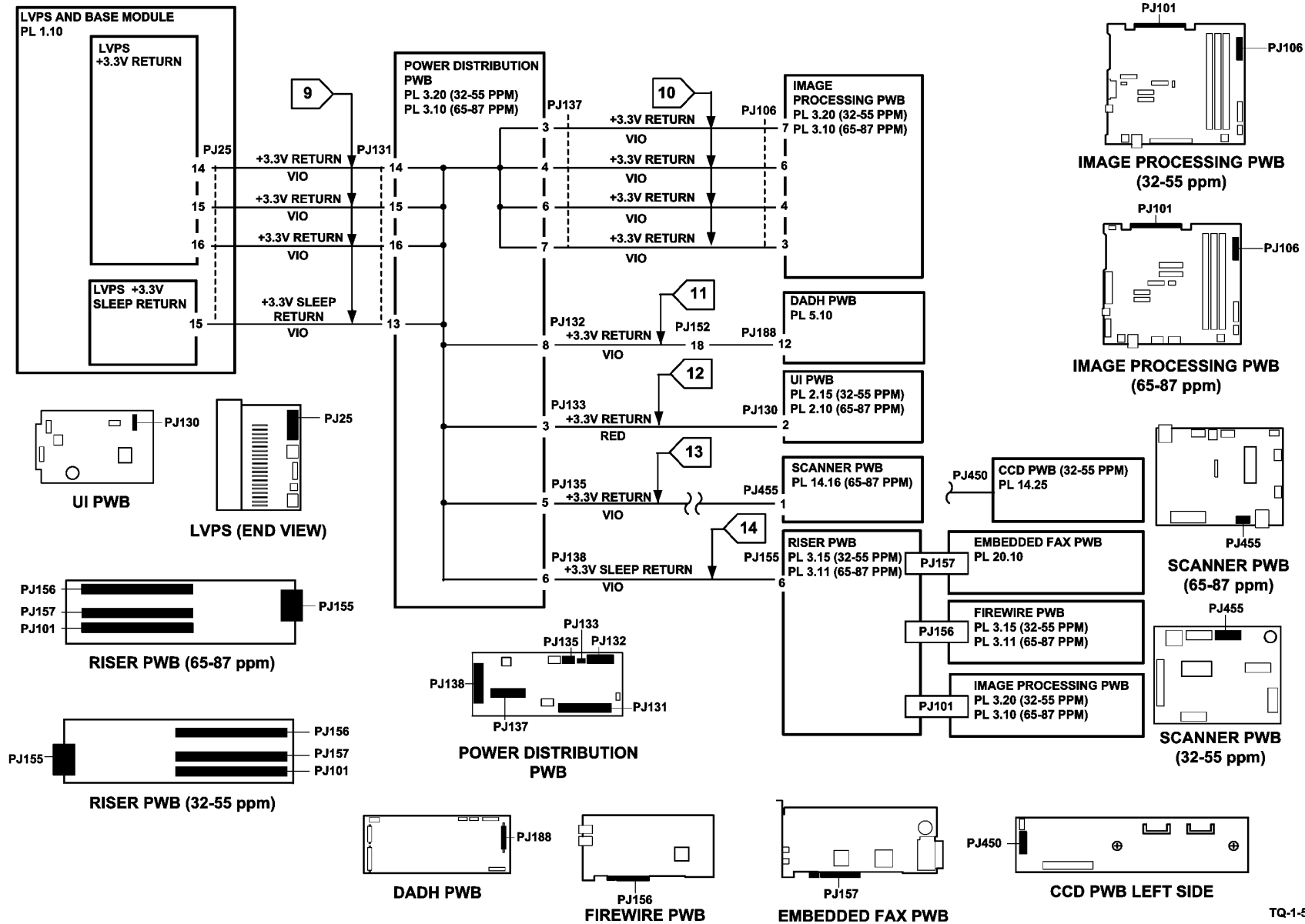
Figure 2 3.3V Return W/OTAG 040
