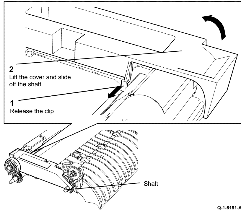
Figure 3 Remove the cover
