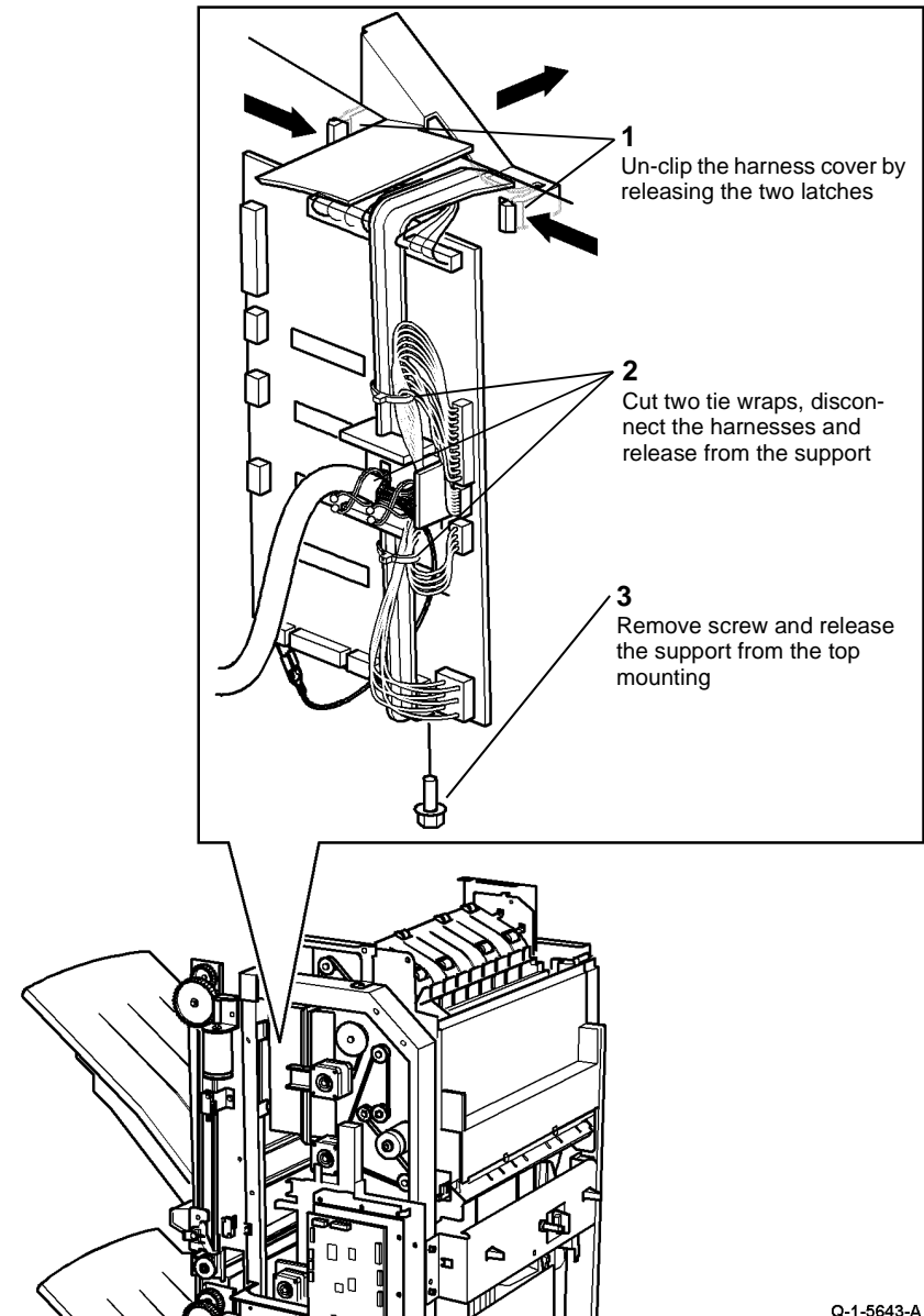
Figure 1 Harness cover and support
