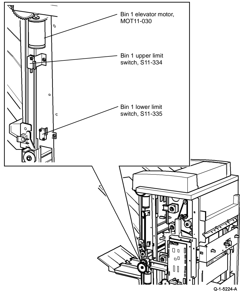
Figure 1 Component location
