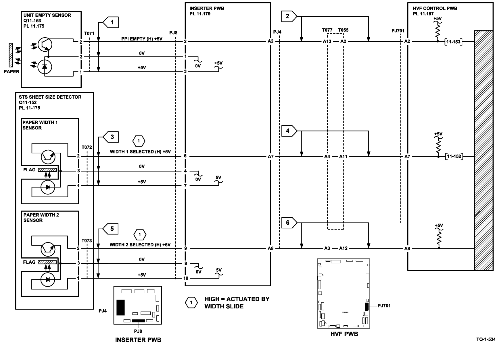
Figure 3 Circuit diagram
