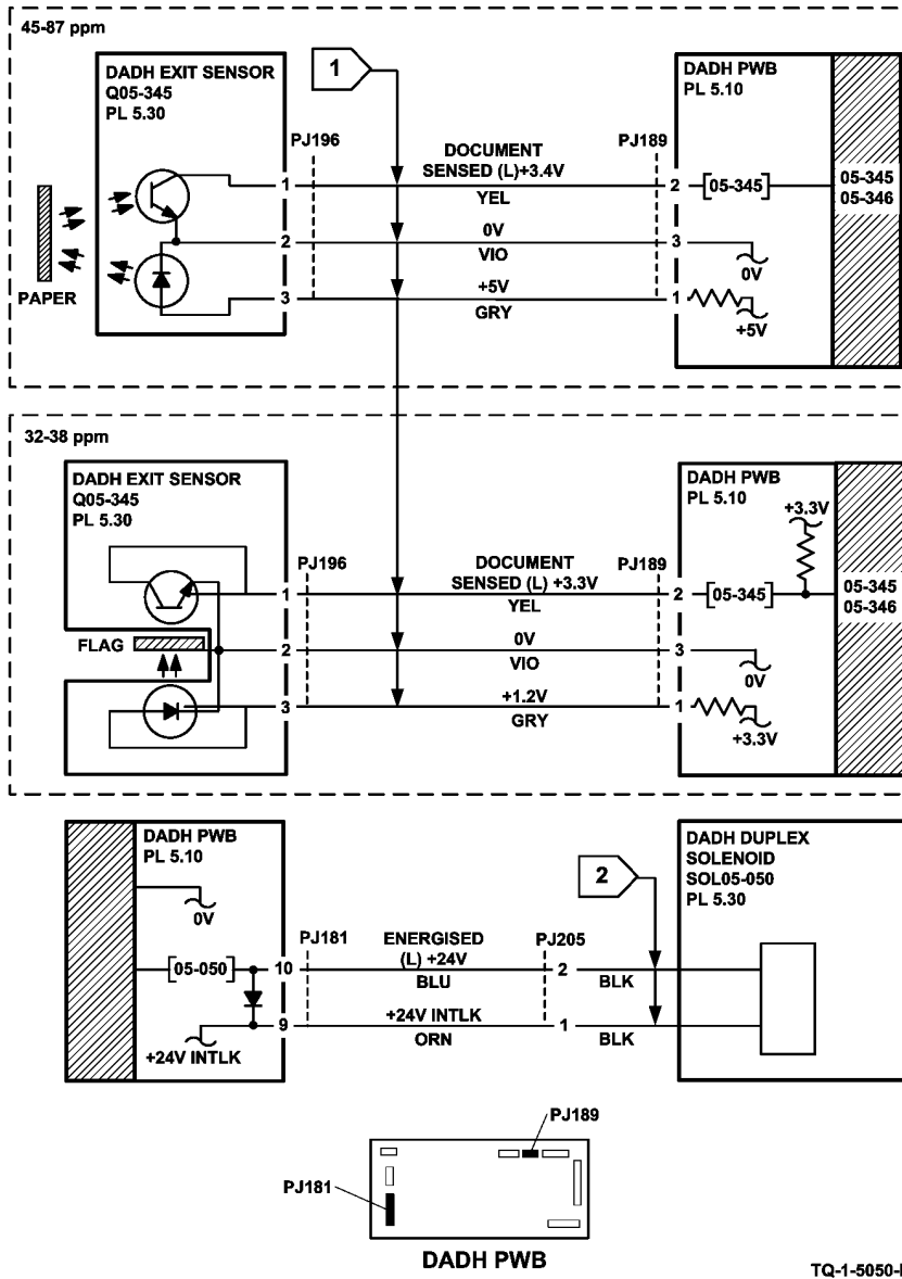
Figure 4 Circuit diagram
