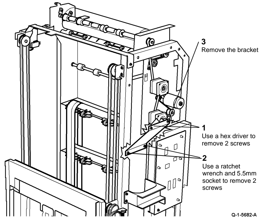
Figure 3 bracket removal
