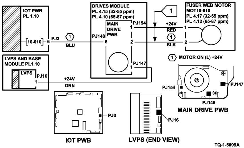
Figure 3 Circuit diagram
