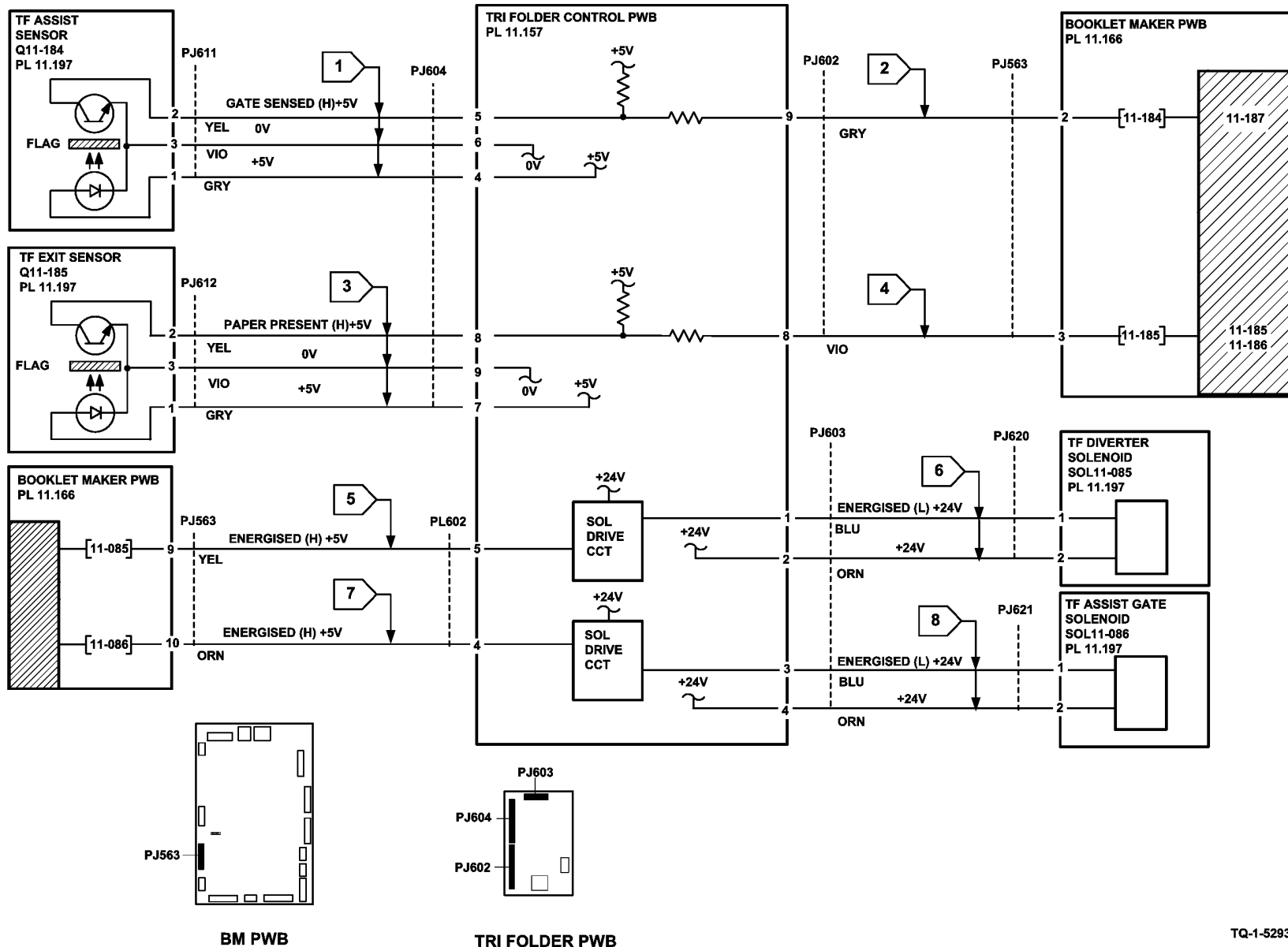
Figure 4 Circuit diagram
