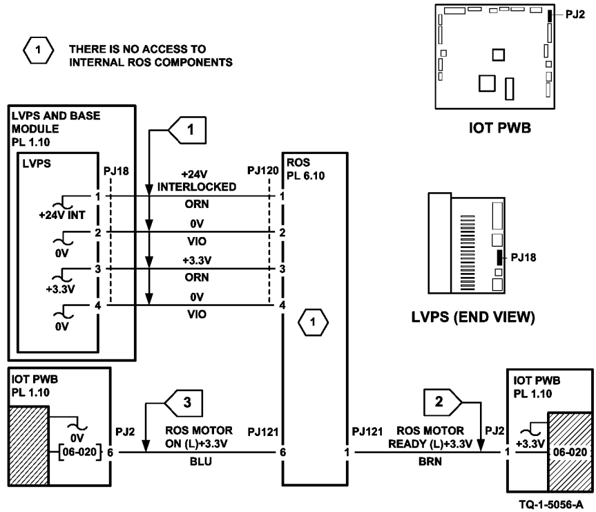
Figure 2 Circuit diagram
