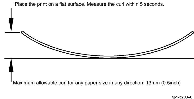
Figure 1 Curl height measurement
