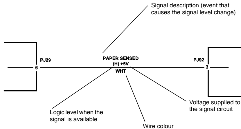
Figure 1 Signal Nomenclature
