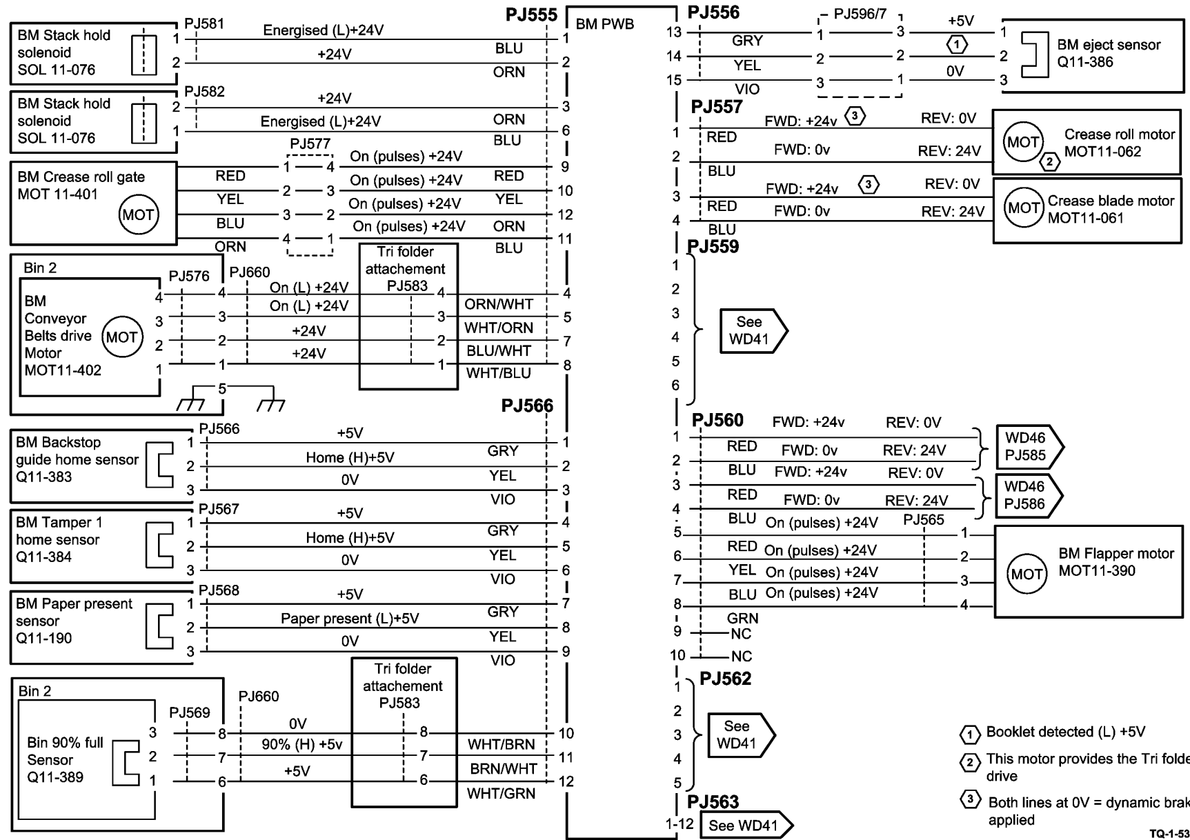
Figure 47 Wiring Diagram 47
