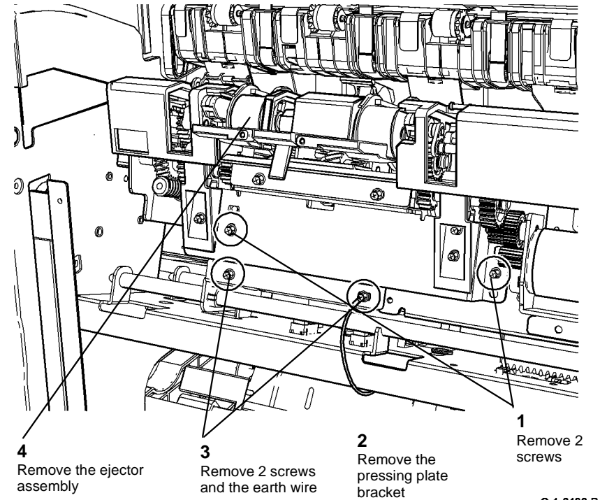
Figure 2 Ejector Assembly
