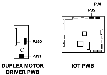
Figure 2 Circuit diagram
