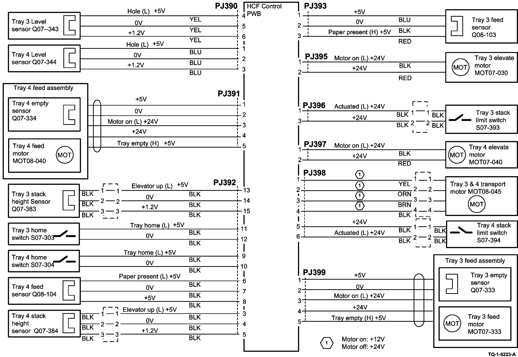
Figure 14 Wiring Diagram 14
