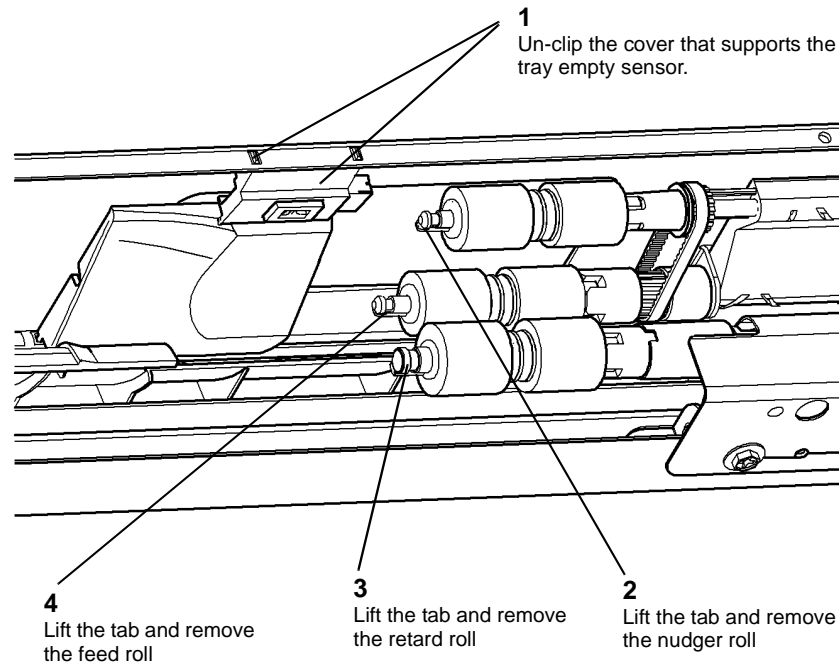
Figure 1 Remove the feed rolls
