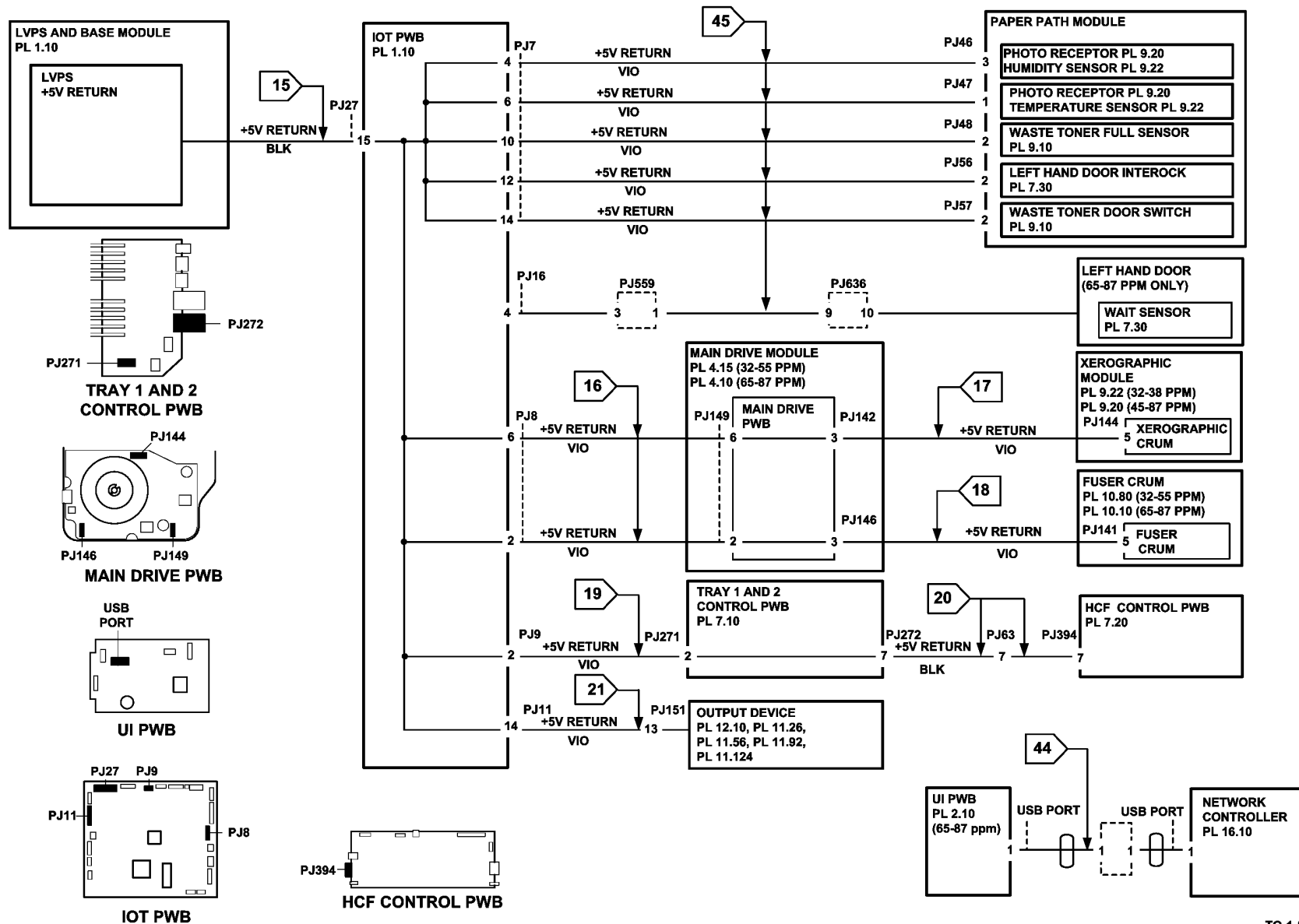
Figure 4 5V Return
