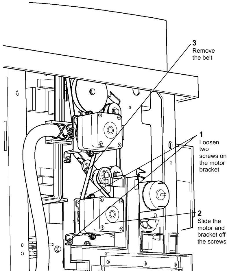
Figure 2 Belt removal
