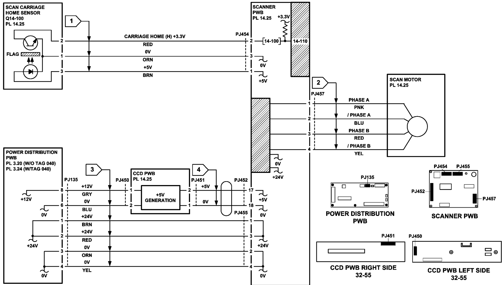
Figure 3 Circuit diagram
