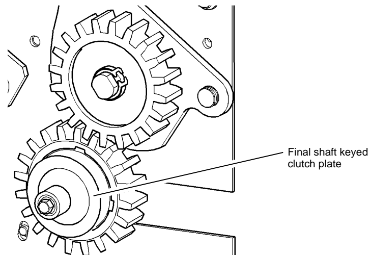
Figure 8 Outermost gear keyed clutch plate
