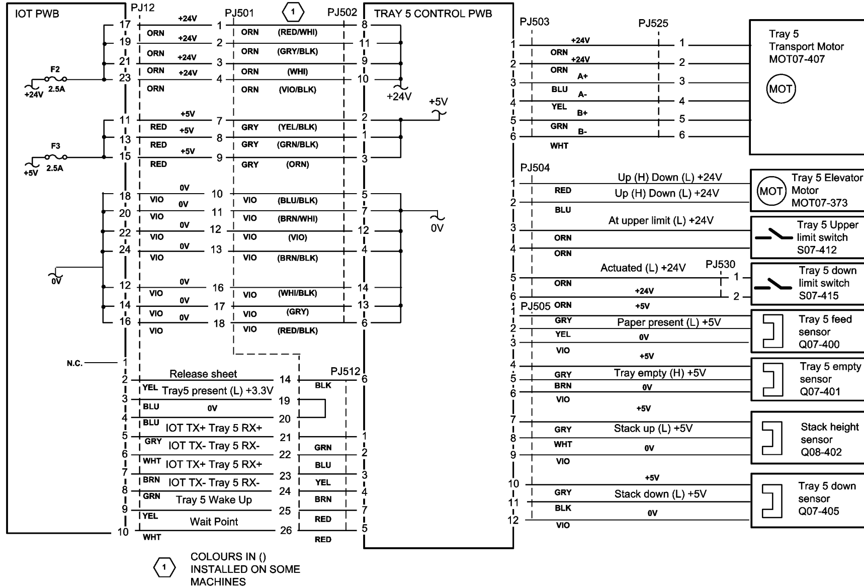
Figure 38 Wiring Diagram 38
