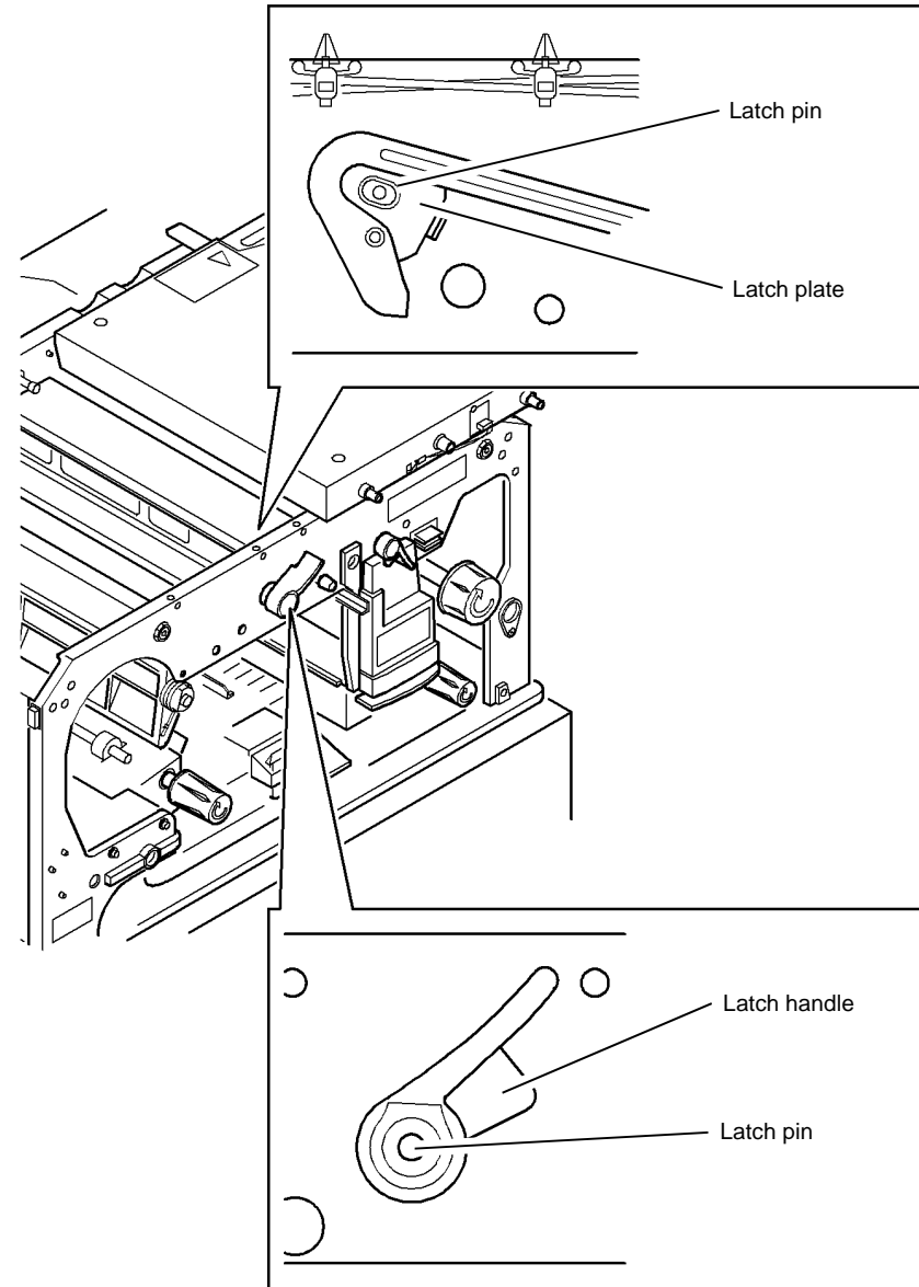
Figure 4 Latch alignment
