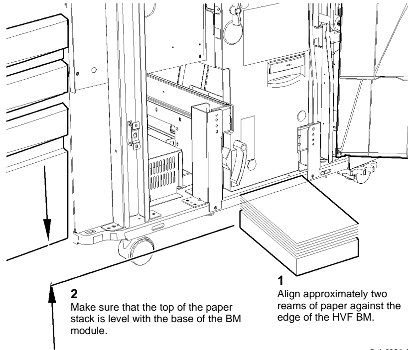
Figure 3 Preparation
