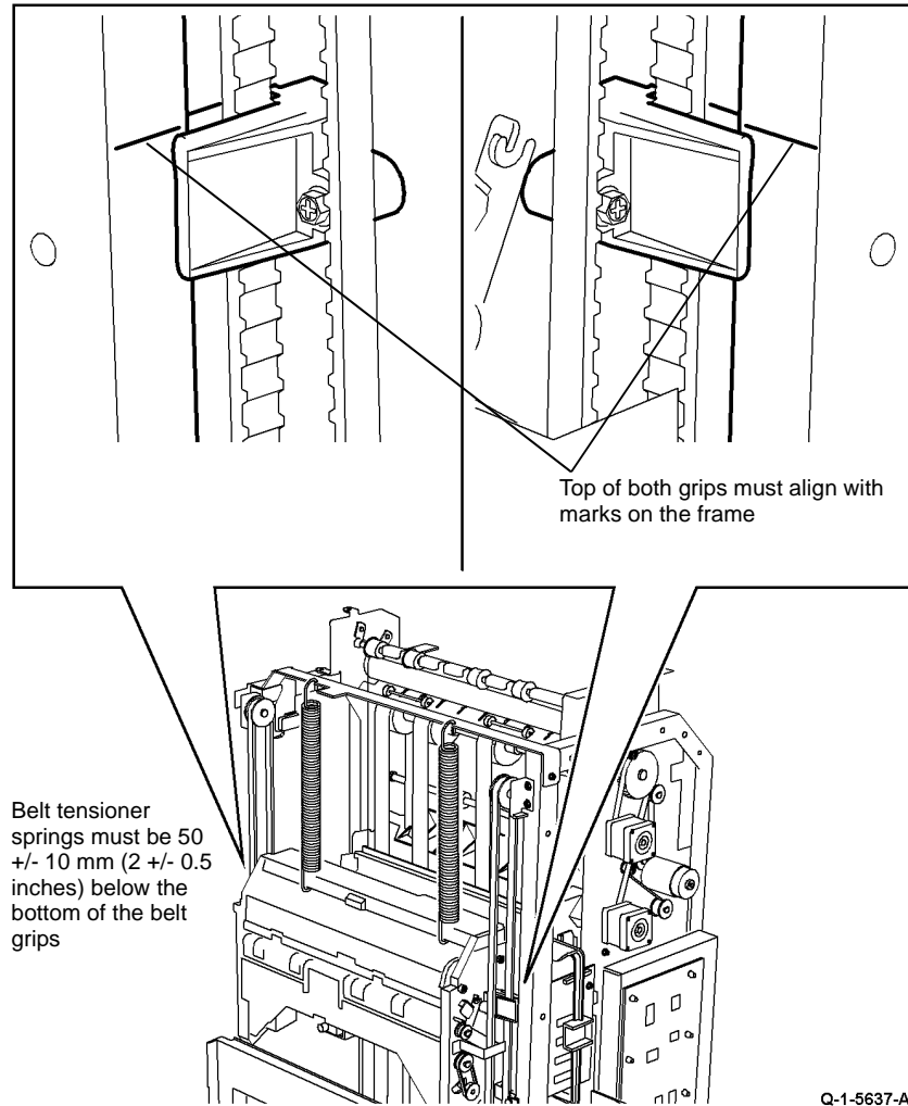
Figure 8 Carriage alignment
