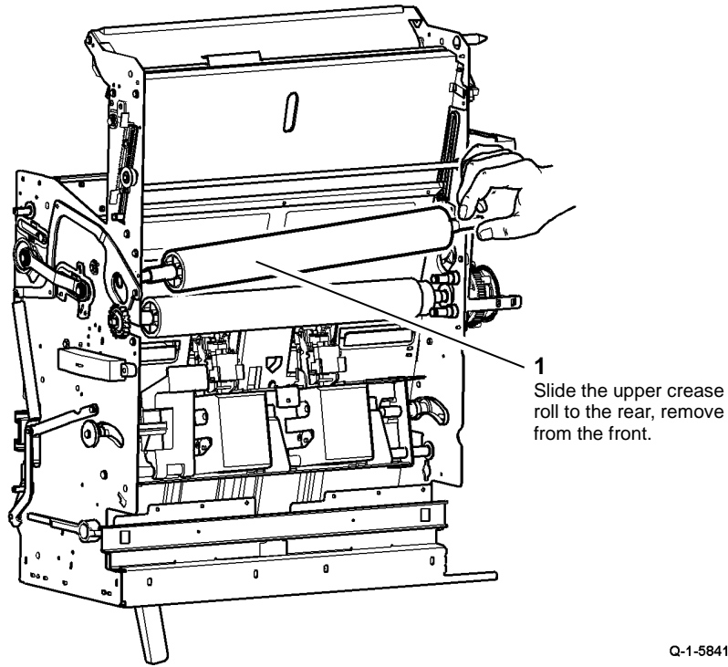
Figure 3 Upper crease roll removal
