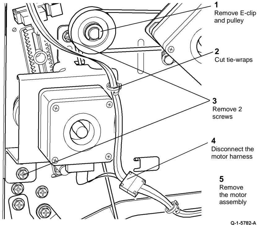
Figure 1 Motor assembly removal
