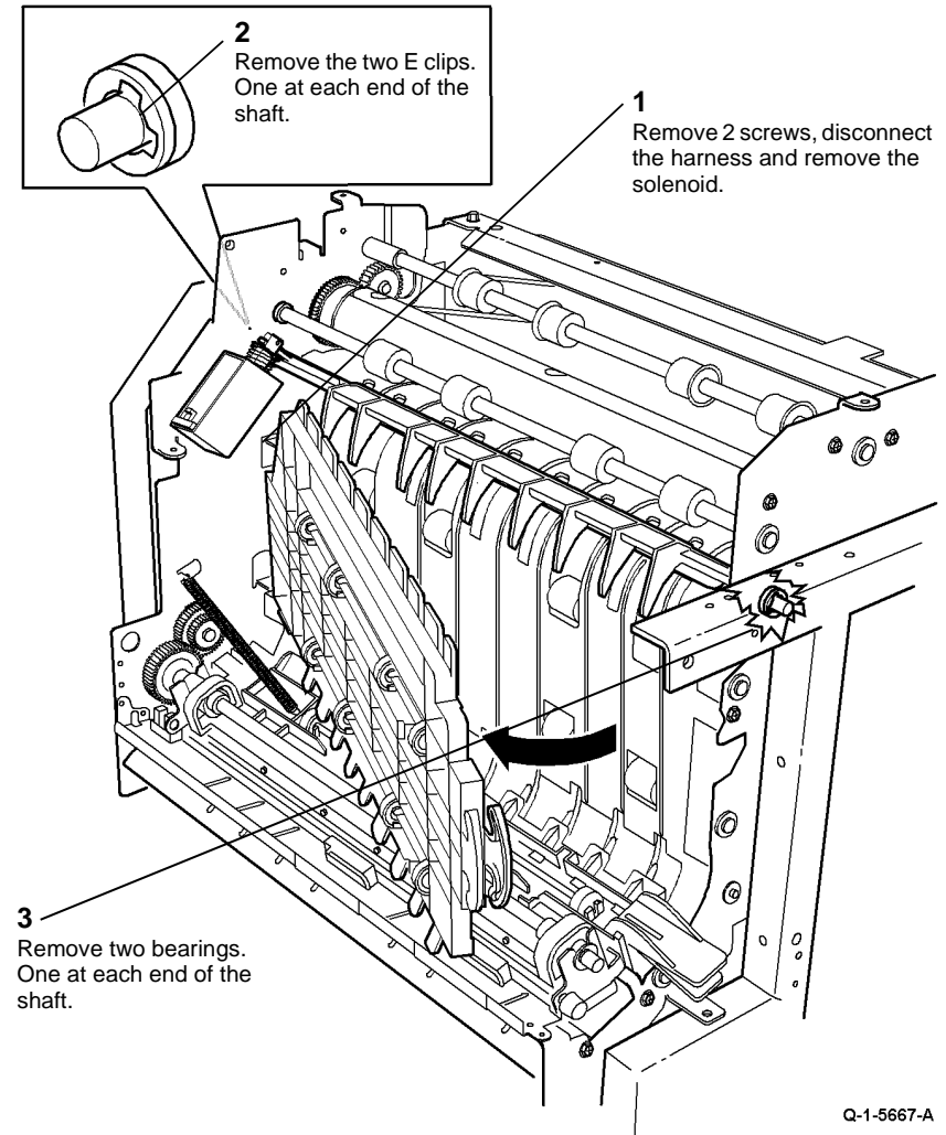
Figure 1 Preparation
