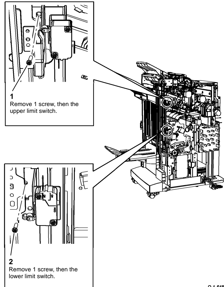
Figure 1 Bin 1 limit switches removal
