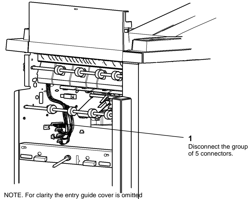
Figure 1 Harness disconnection
