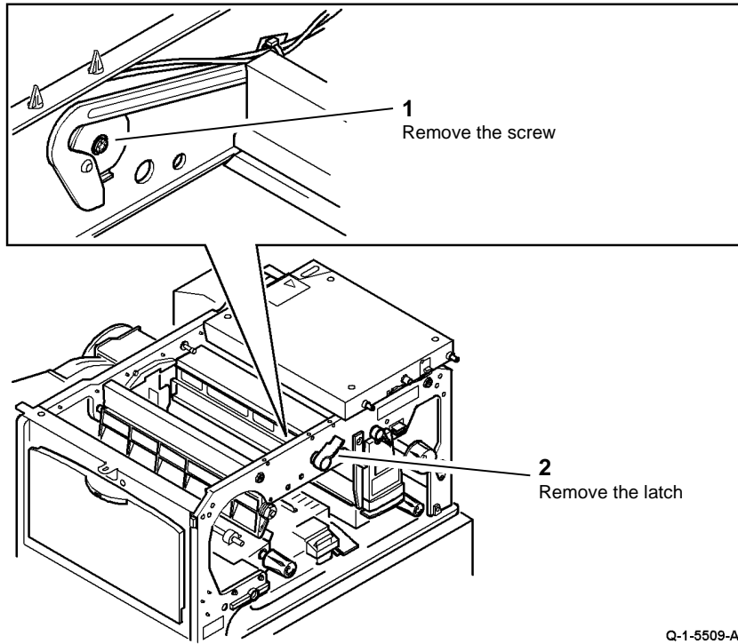
Figure 3 Remove the latch
