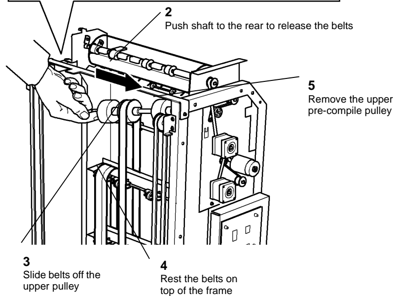
Figure 2 Release belts
