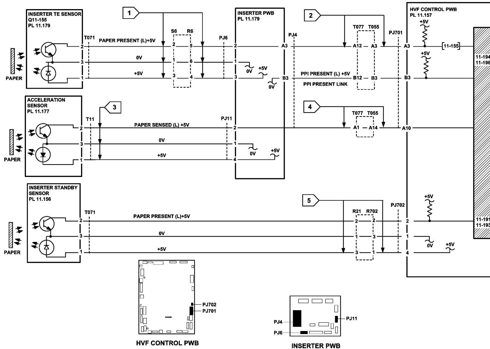
Figure 2 Circuit diagram
