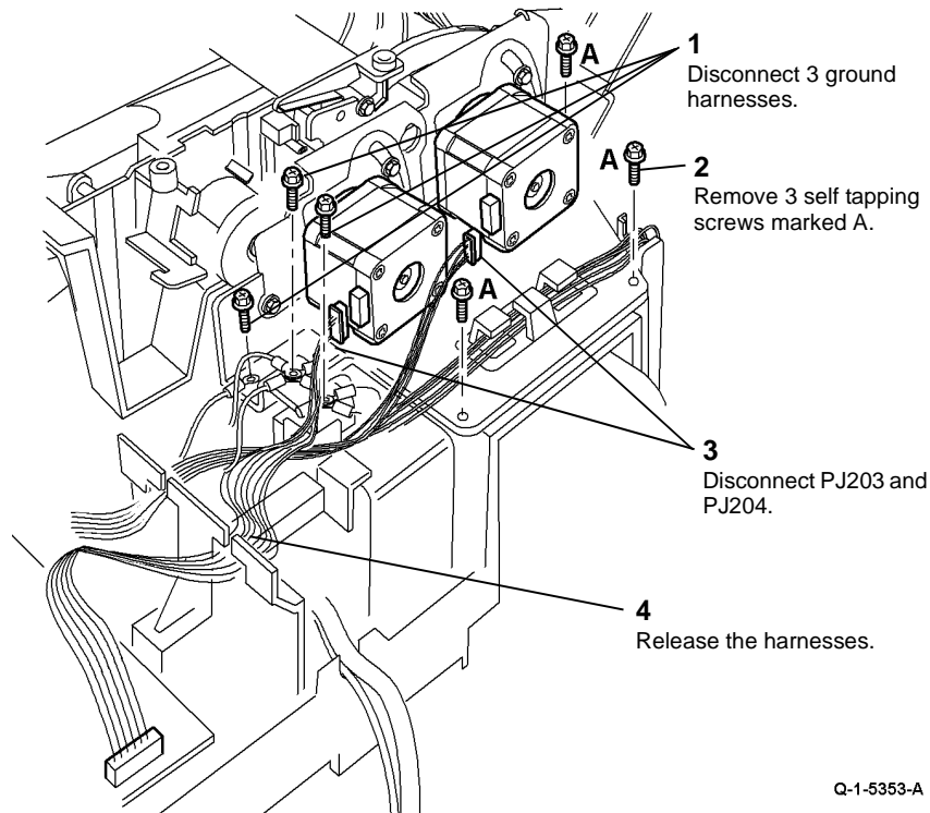
Figure 1 Drives assembly
