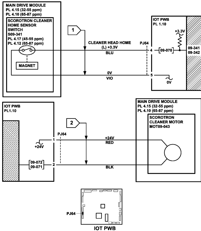
Figure 2 Circuit diagram
