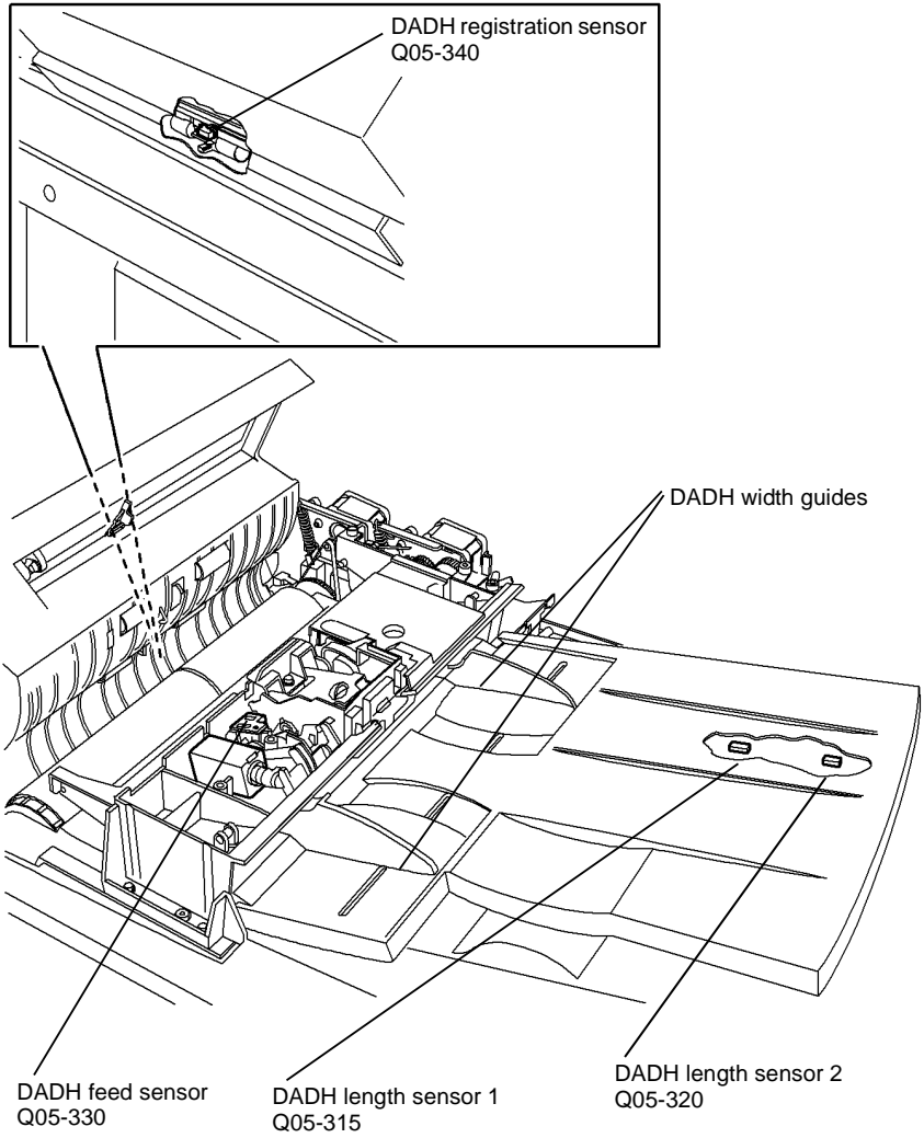
Figure 1 Component location
