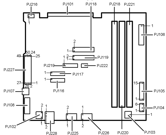
Figure 10 Image processing PWB
