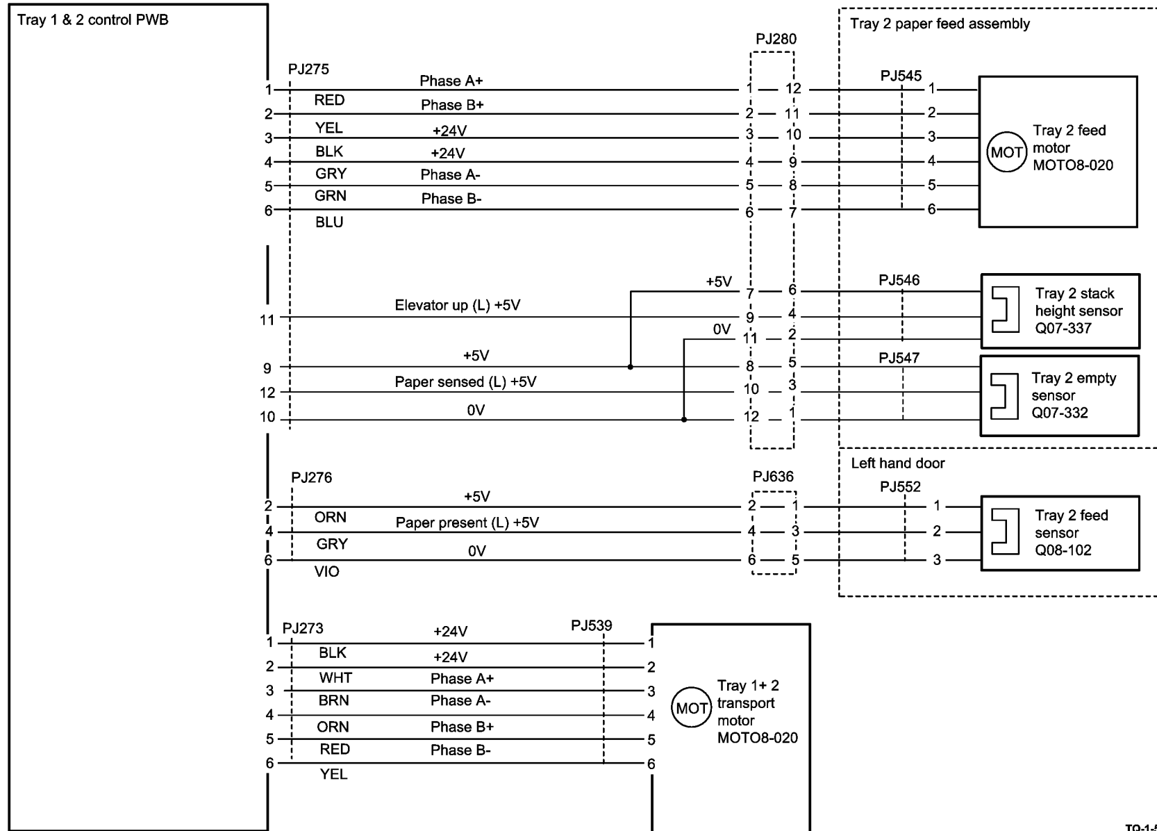
Figure 13 Wiring Diagram 13
