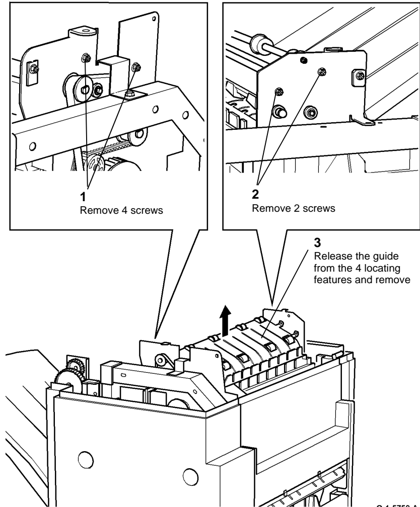
Figure 2 Removing guide
