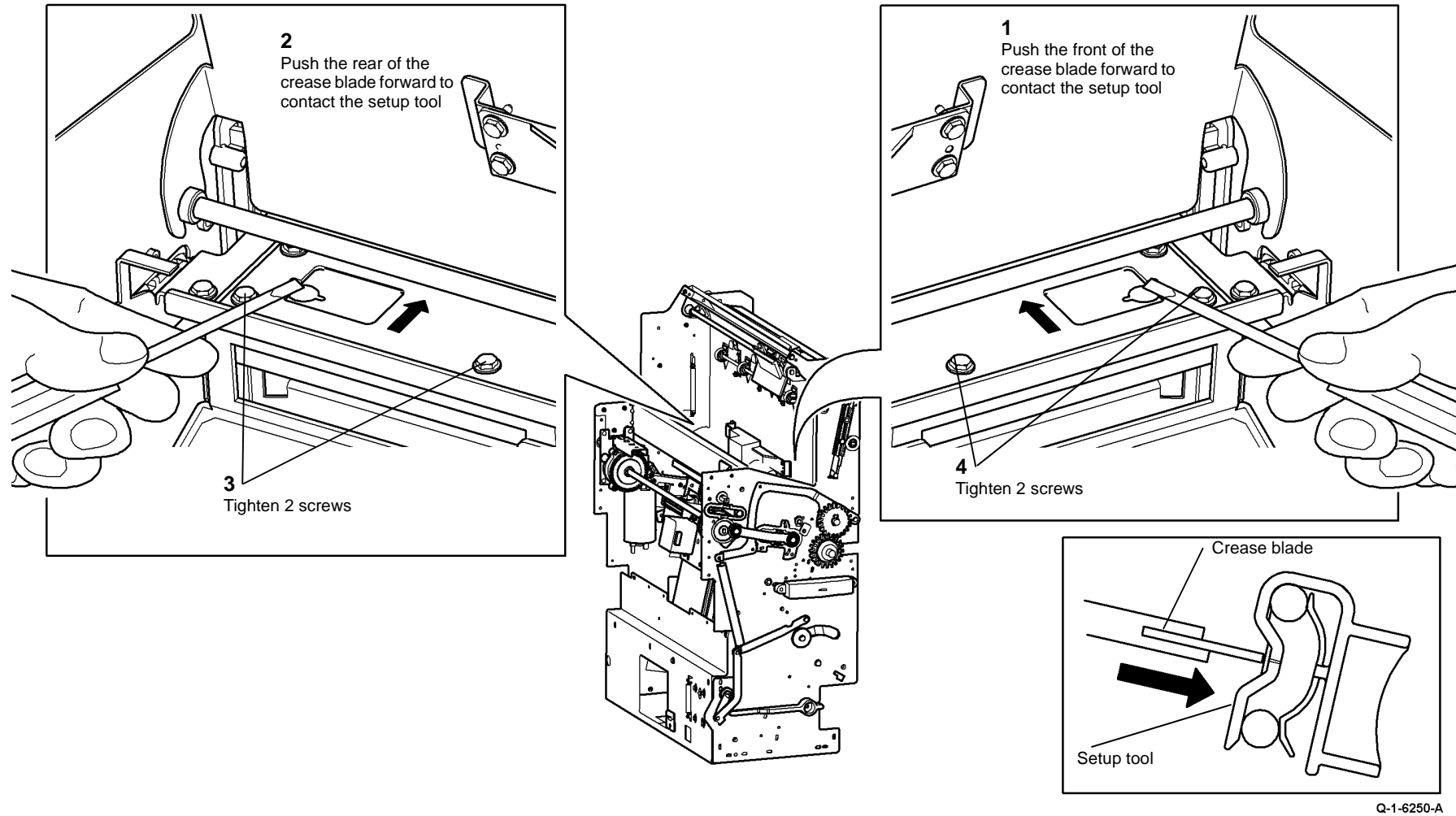
Figure 4 Blade positioning
