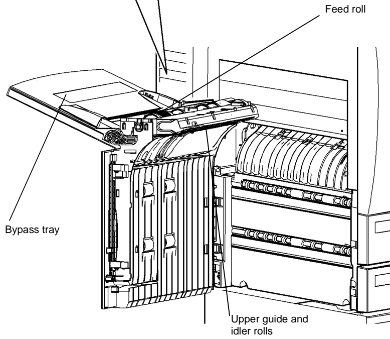
Figure 1 Component location
