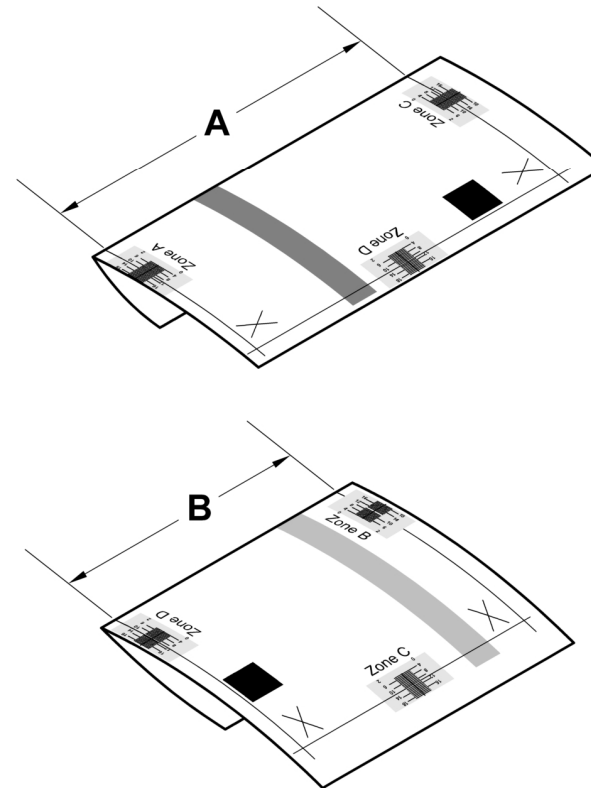
Figure 1 Magnification check
