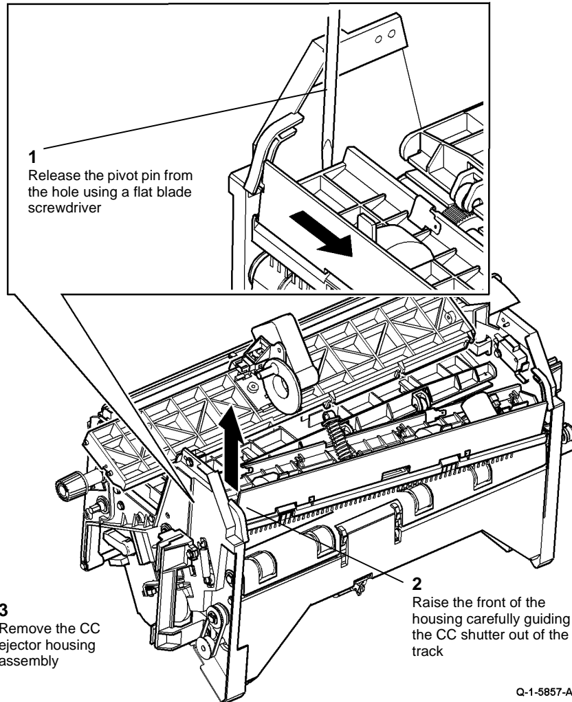
Figure 3 Housing removal
