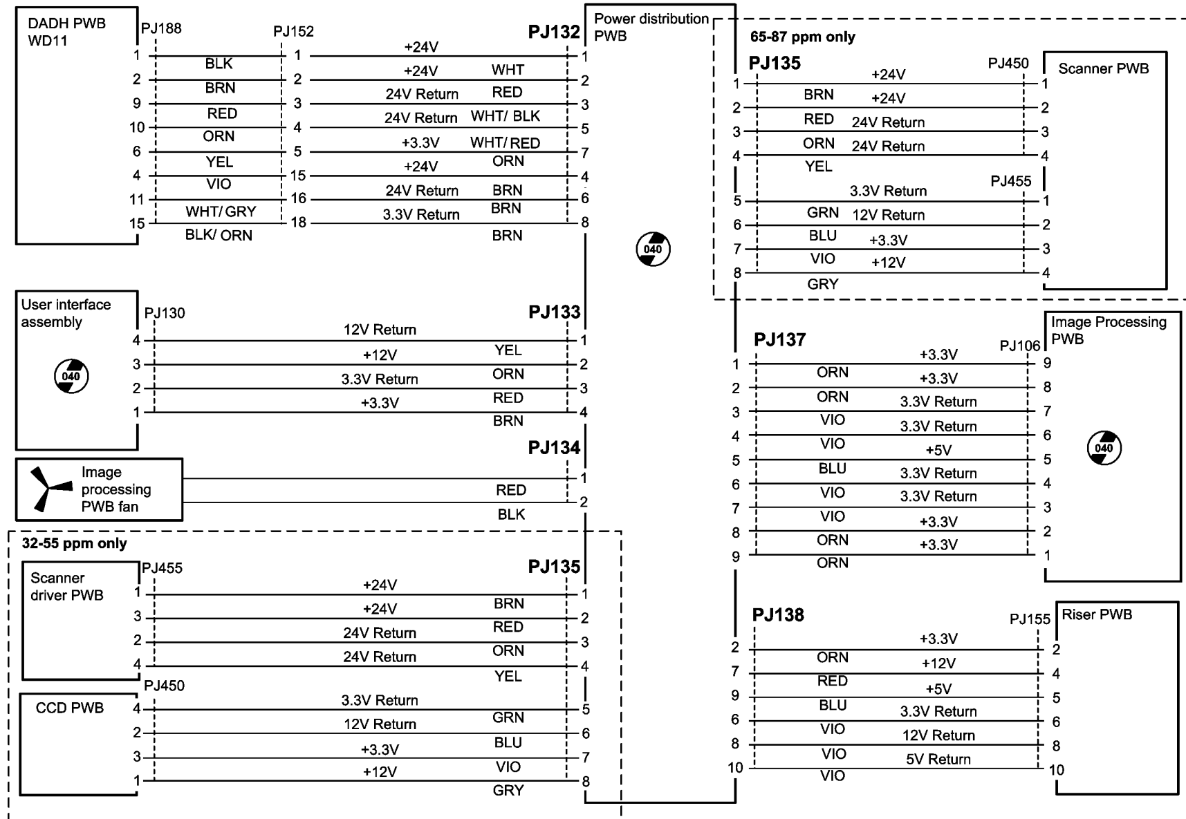
Figure 10 Wiring Diagram 10 (W/OTAG 040)
