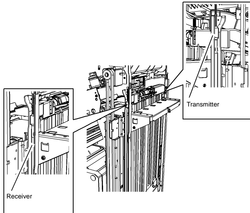
Figure 1 Stack height sensor removal
