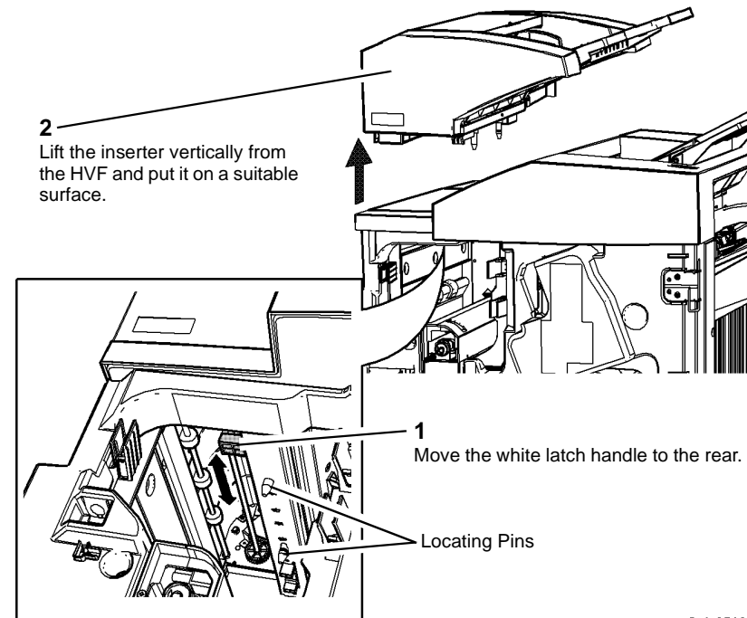
Figure 1 Inserter undocking
