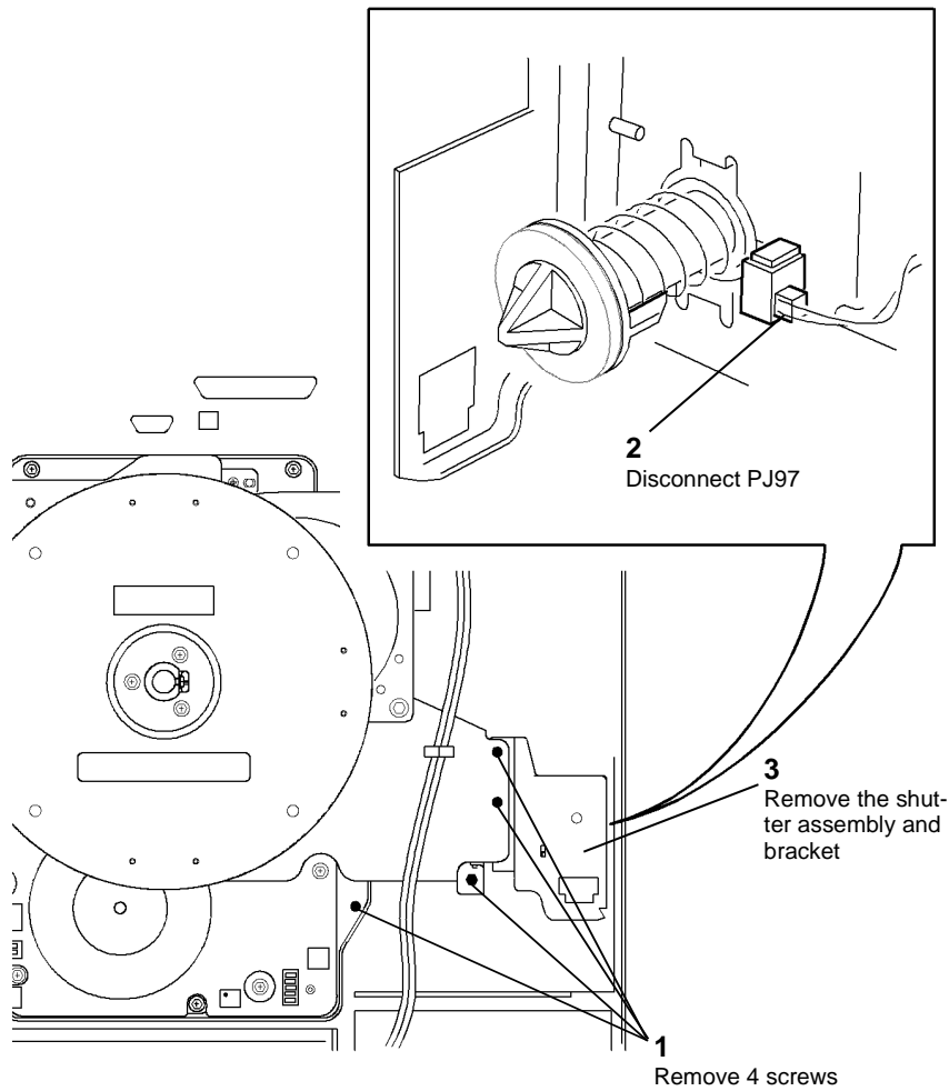
Figure 3 Remove shutter assembly
