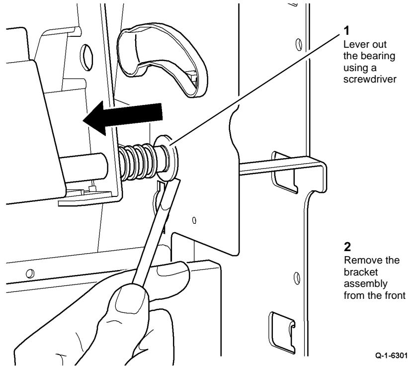
Figure 5 Assembly removal
