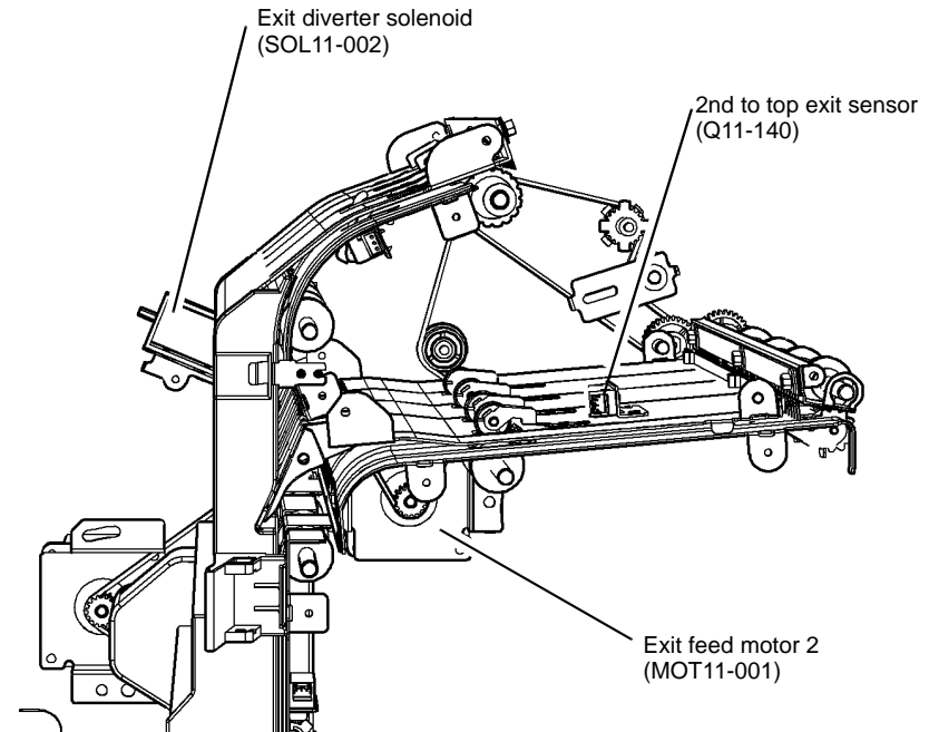
Figure 1 Component location
