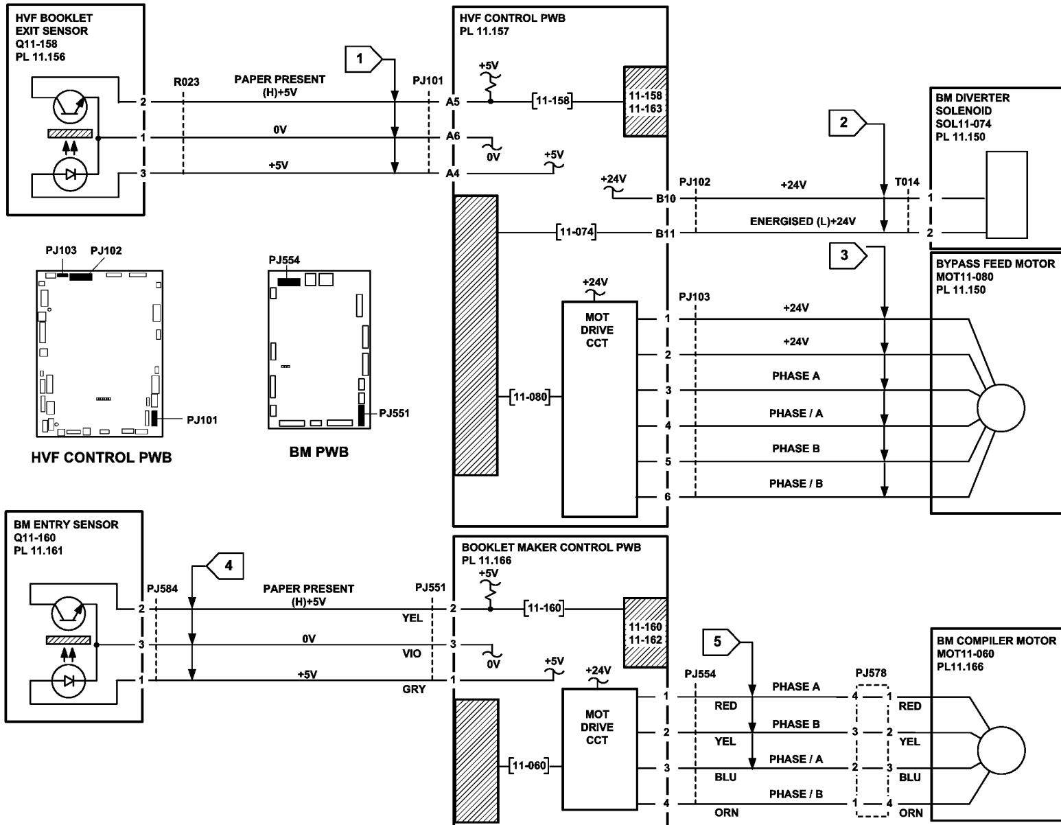
Figure 3 Circuit diagram
