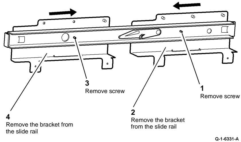
Figure 3 Remove the bracket from the slide rail
