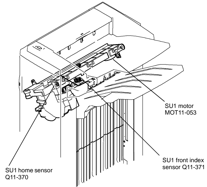
Figure 1 Component location
