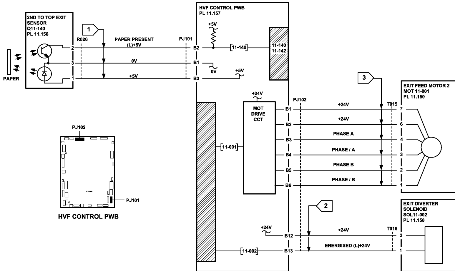
Figure 2 Circuit diagram
