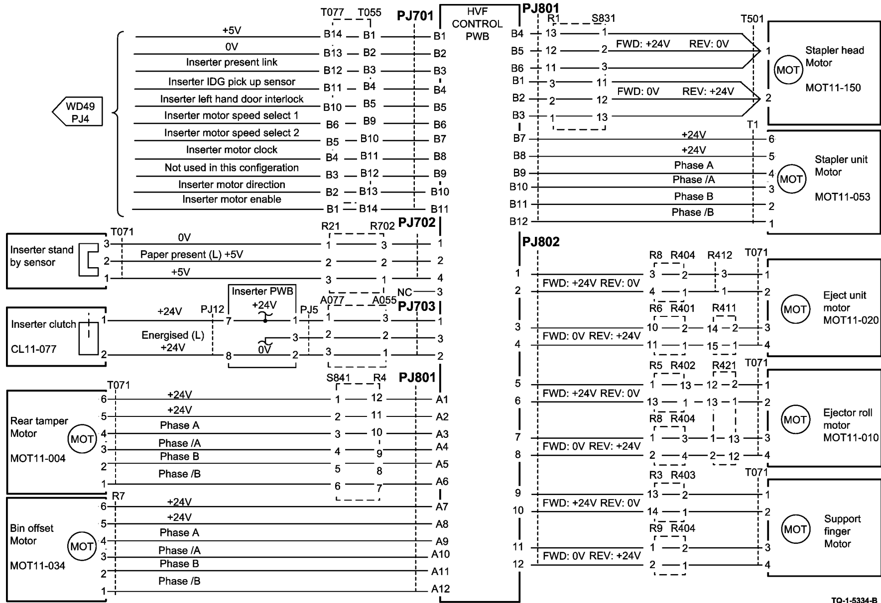
Figure 45 Wiring Diagram 45
