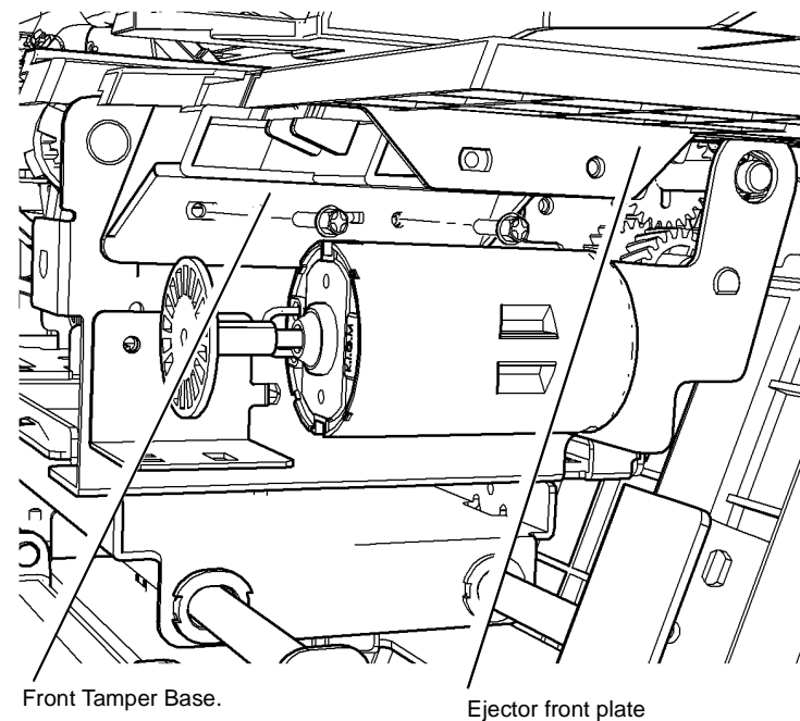
Figure 1 Ejector Front Plate
