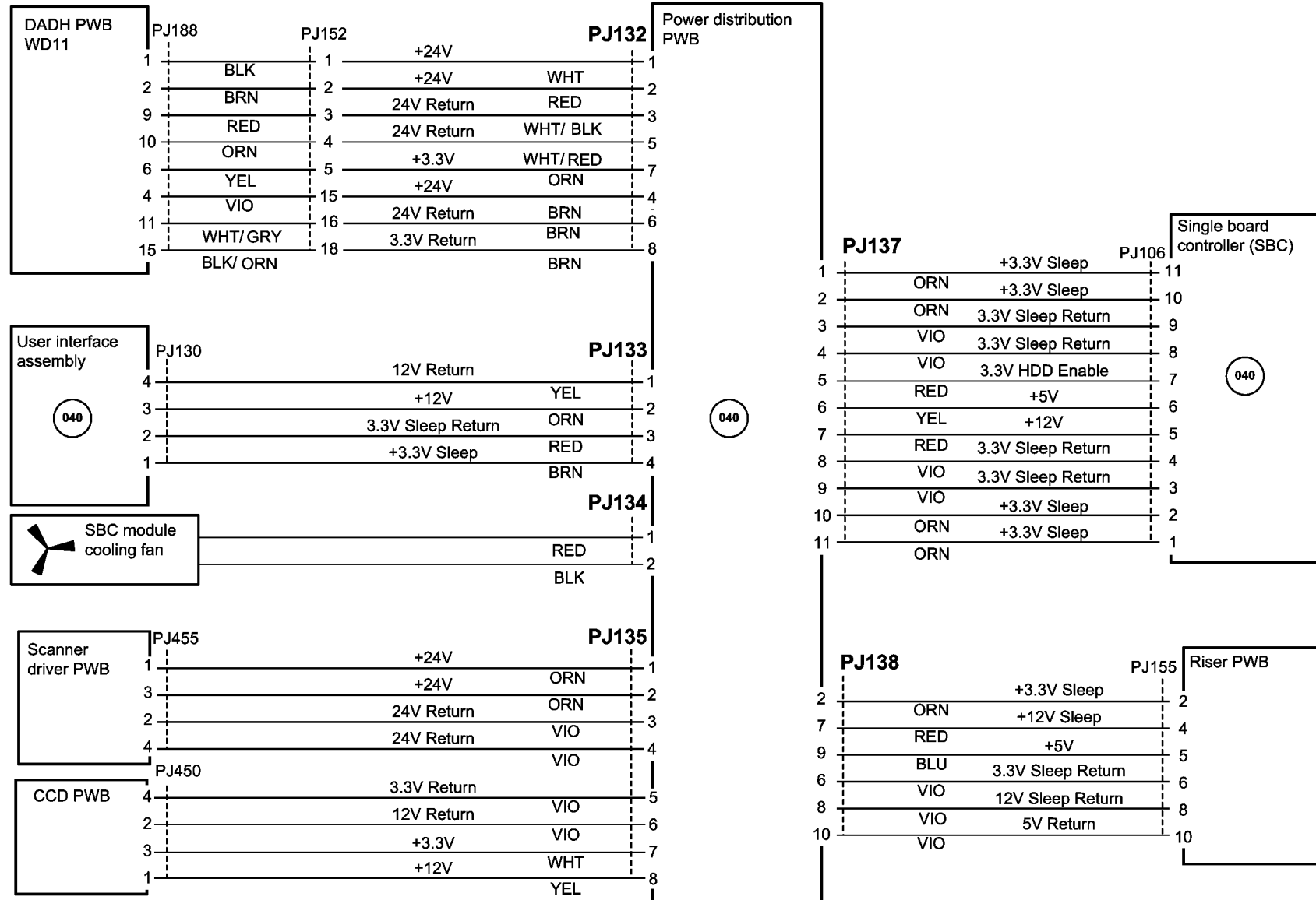
Figure 54 Wiring Diagram 54 (W/TAG 040)
