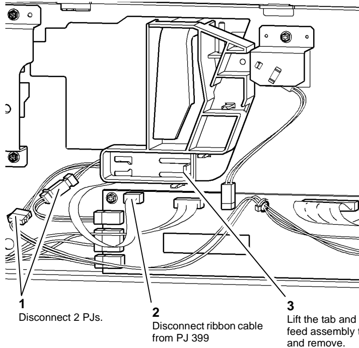
Figure 1 Tray 3 feed assembly
