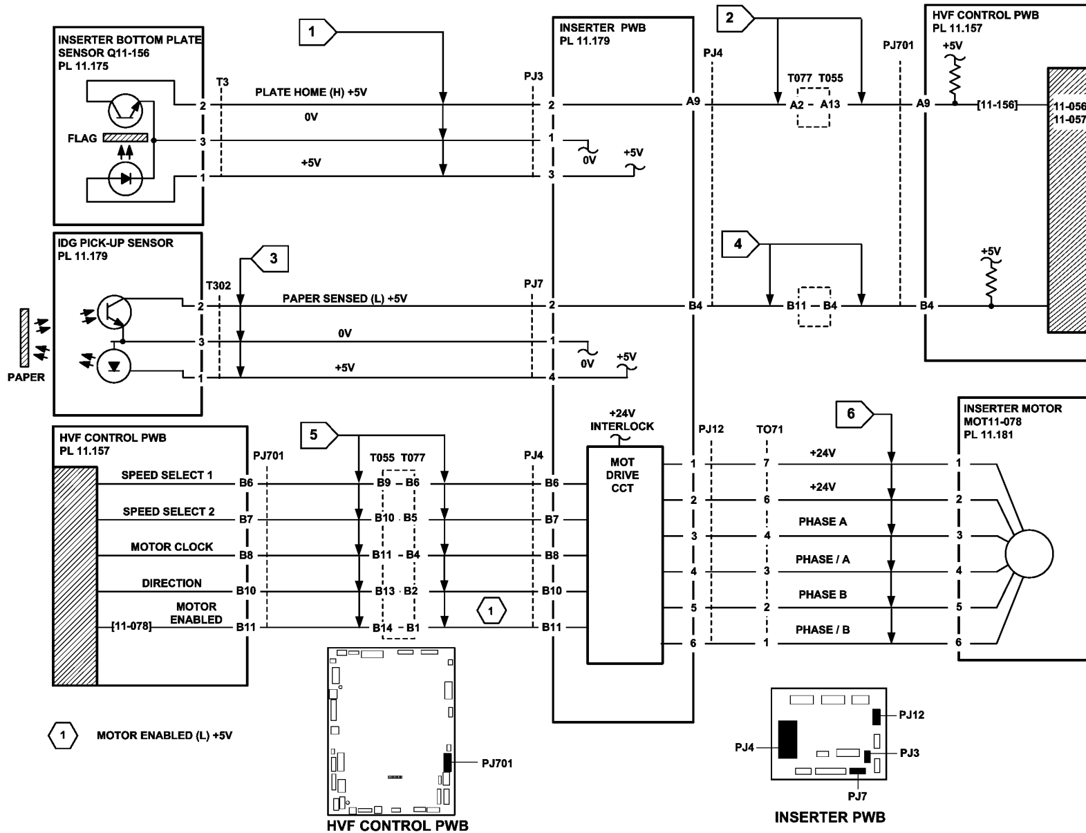
Figure 2 Circuit diagram
