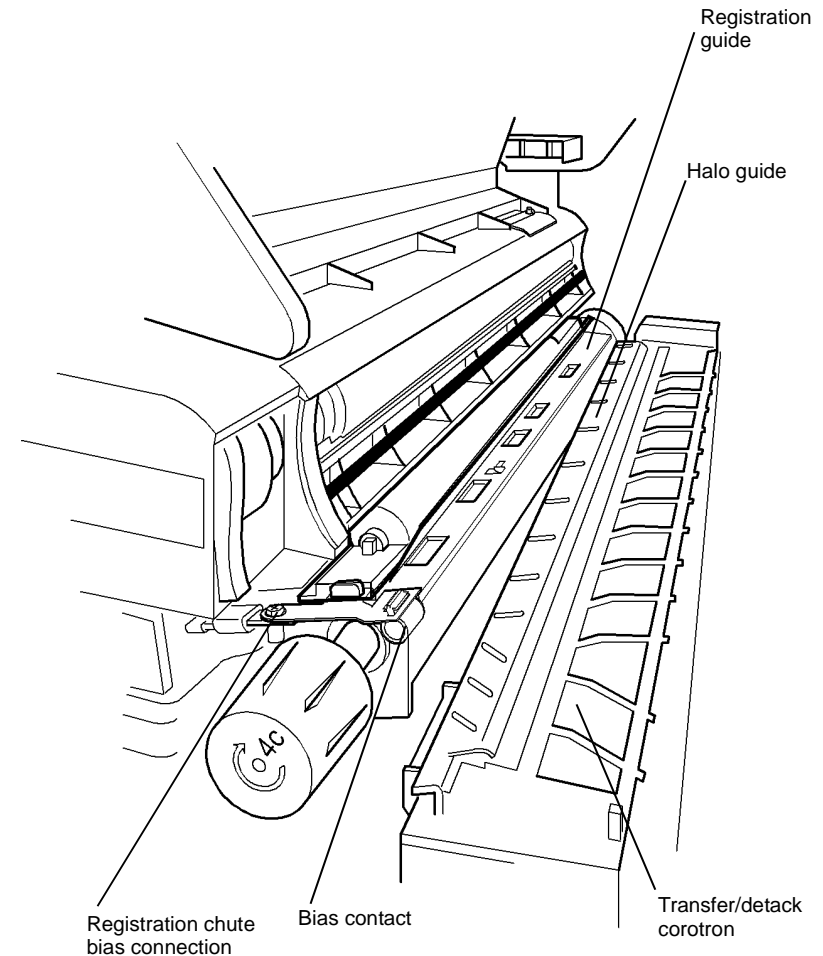
Figure 1 Component location
