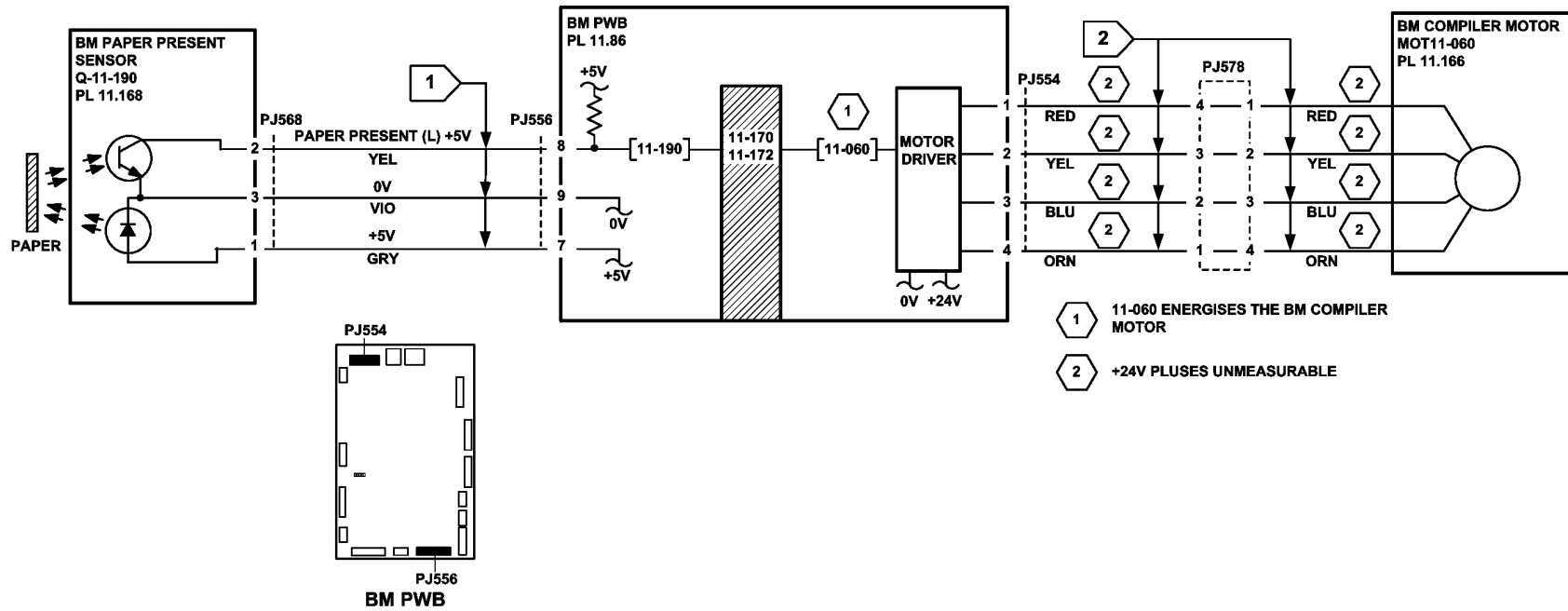
Figure 2 Circuit diagram
