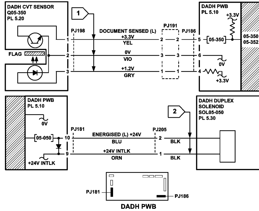
Figure 3 Circuit diagram
