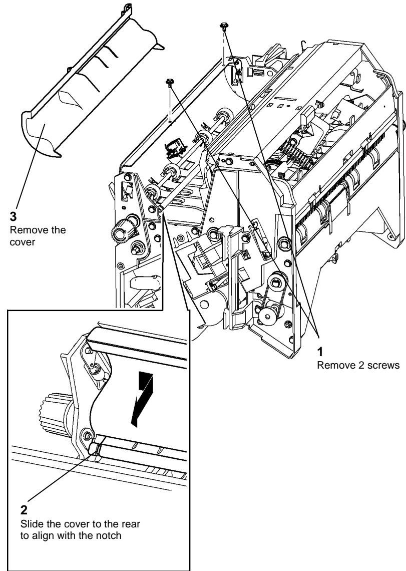
Figure 2 Cover removal
