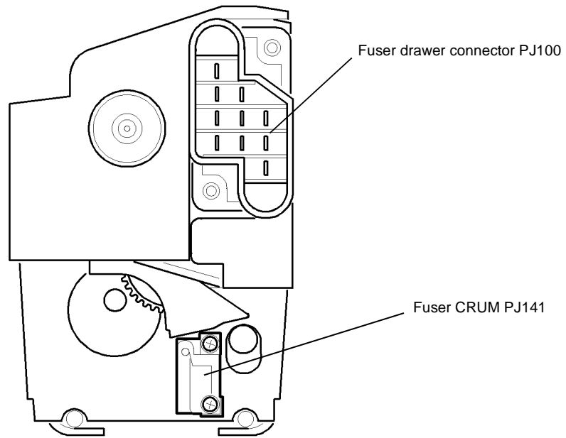
Figure 34 Fuser module
