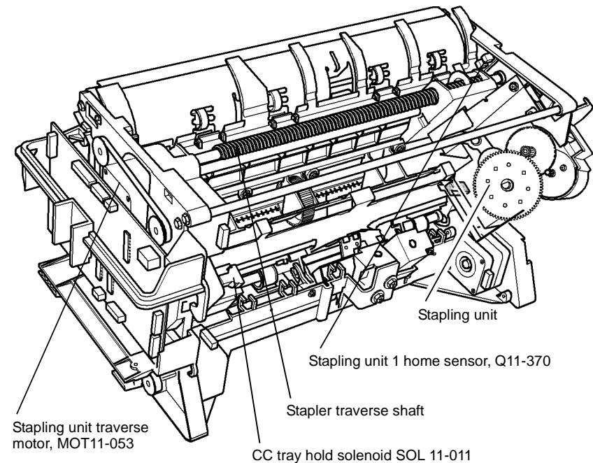
Figure 1 Component location
