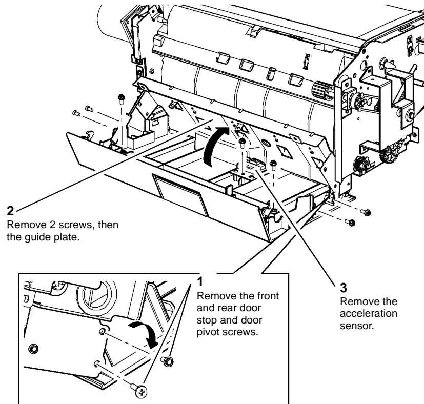
Figure 1 Sensor removal
