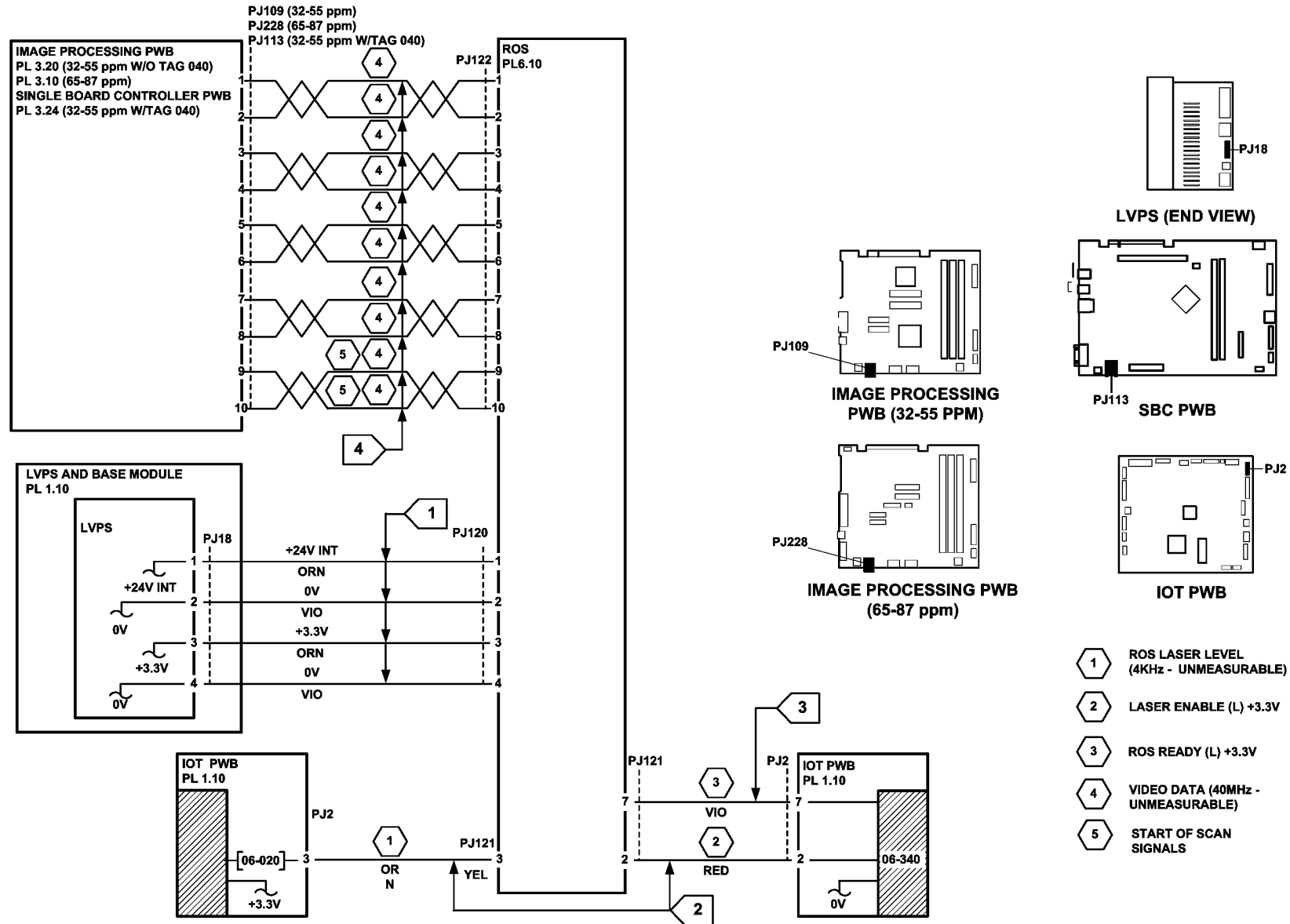
Figure 2 Circuit diagram
