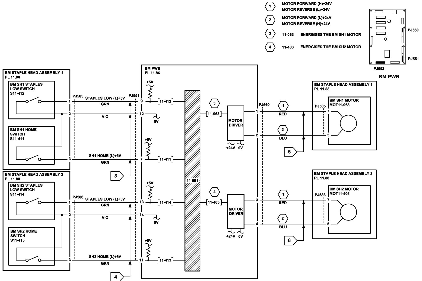
Figure 3 Circuit diagram
