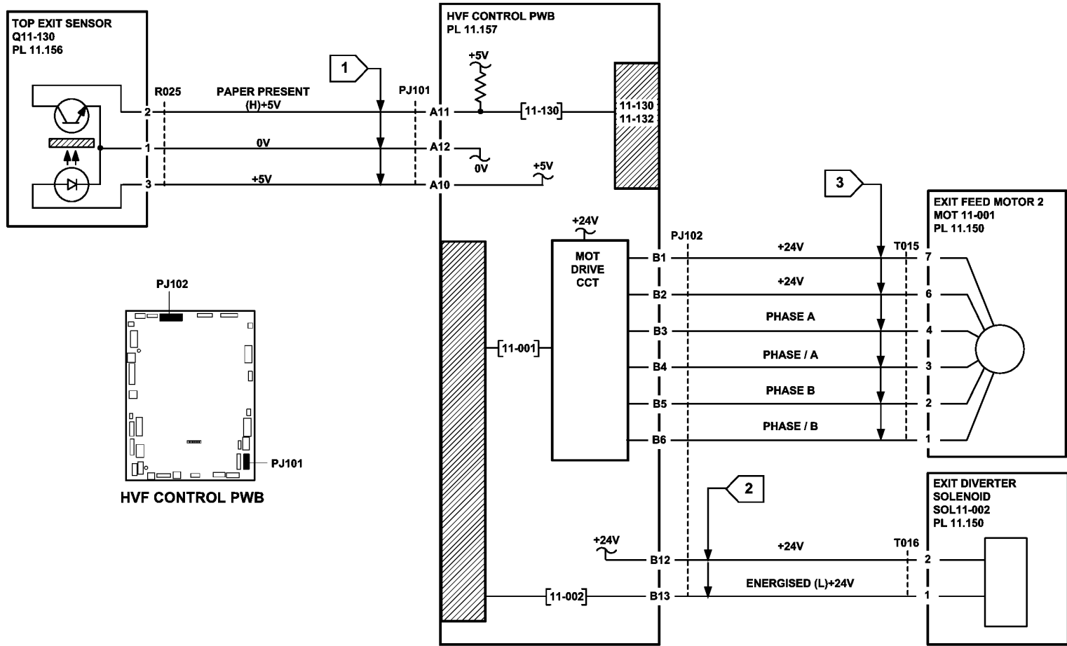
Figure 2 Circuit diagram
