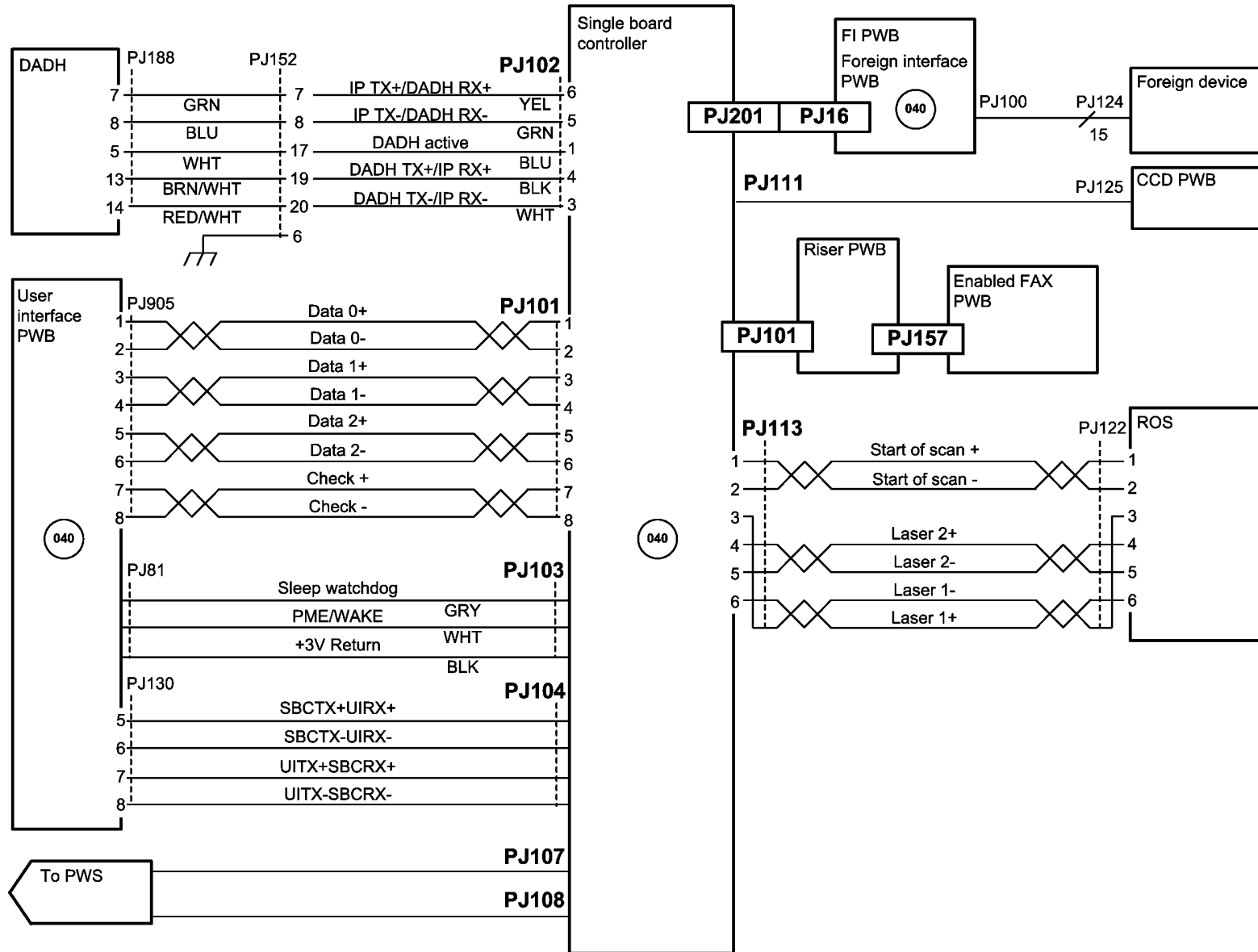
Figure 53 Wiring Diagram 53 (W/TAG 040)
