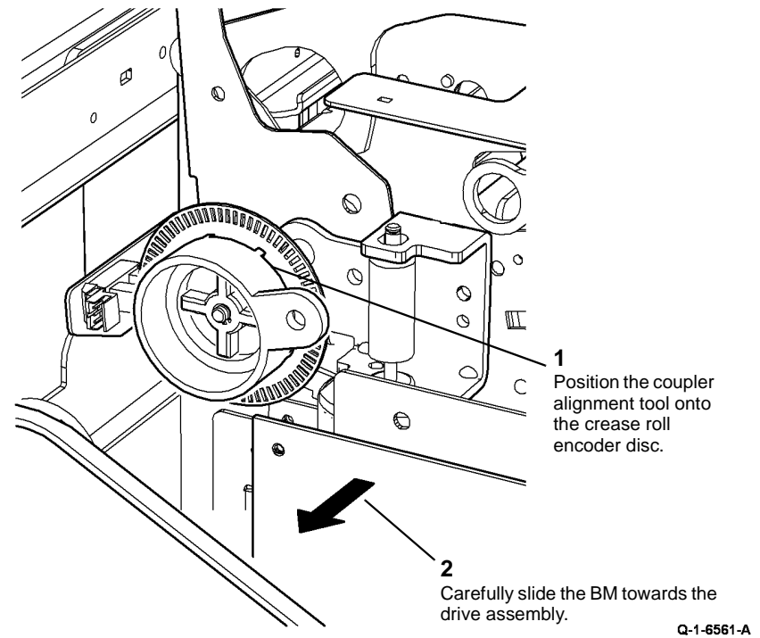
Figure 3 Centralise the alignment tool
