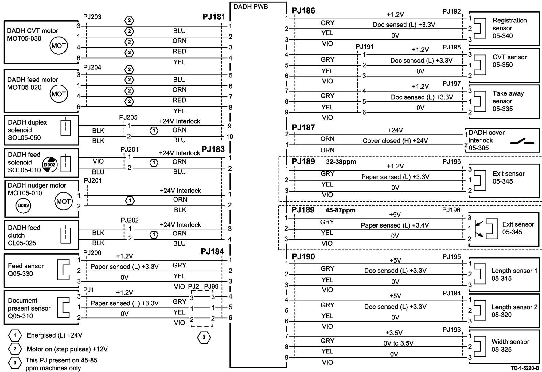
Figure 11 Wiring Diagram 11
