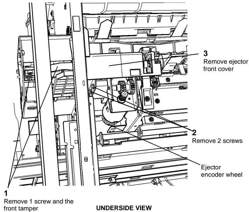
Figure 1 Front Tamper and Ejector Cover
