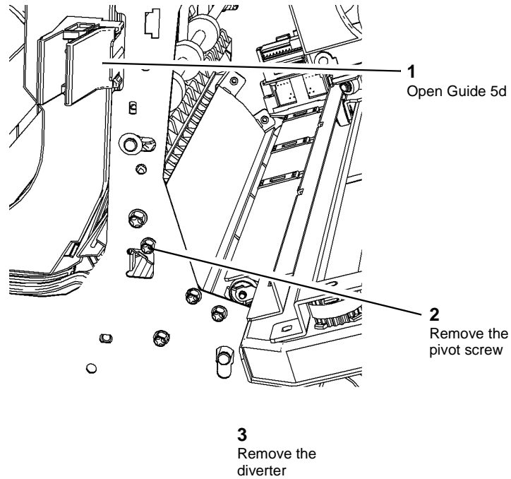
Figure 2 Diverter removal.
