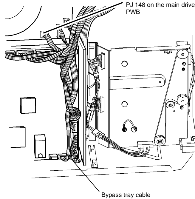
Figure 7 Bypass tray cable
