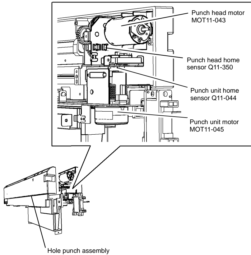
Figure 1 Component location
