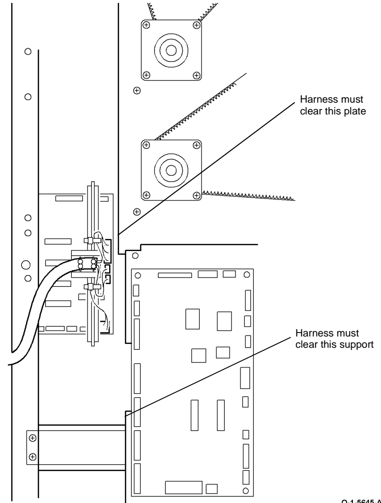
Figure 3 Harness position
