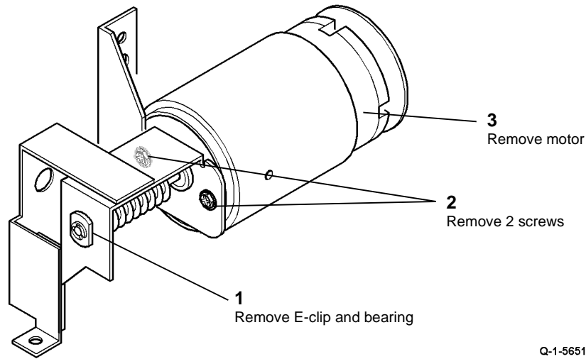
Figure 4 motor removal
