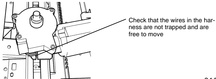
Figure 3 Harness position
