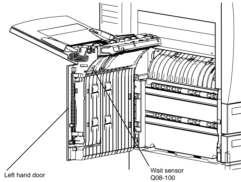
Figure 2 Component location
