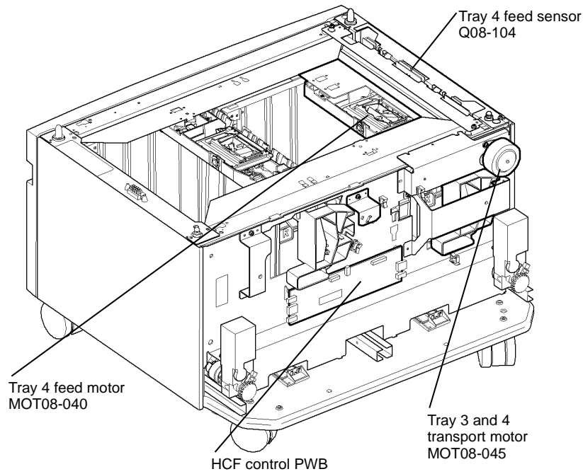
Figure 1 Component location
