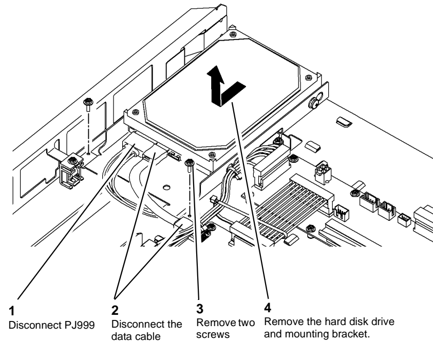
Figure 1 Hard disk drive removal
