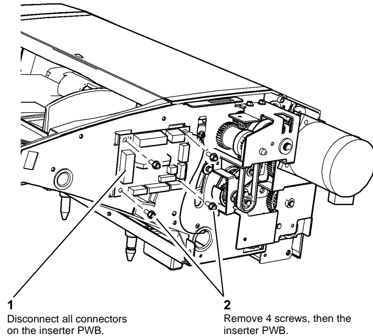
Figure 1 Inserter PWB
