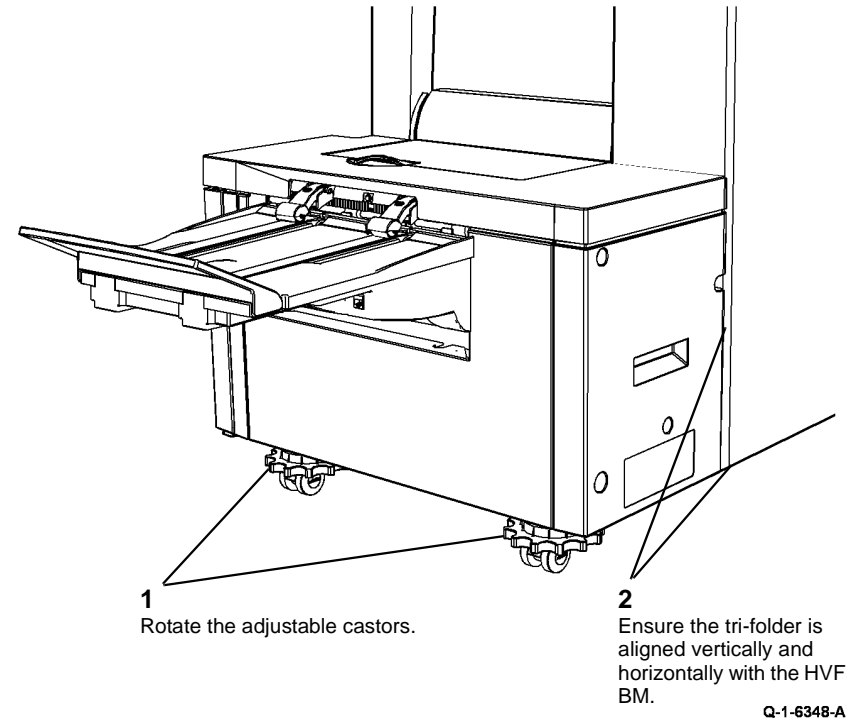
Figure 2 Tri-Folder to HVF BM alignment
