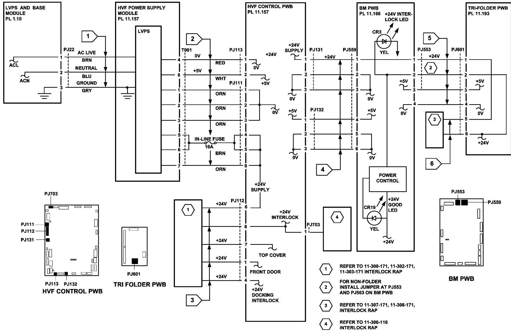
Figure 4 Circuit diagram
