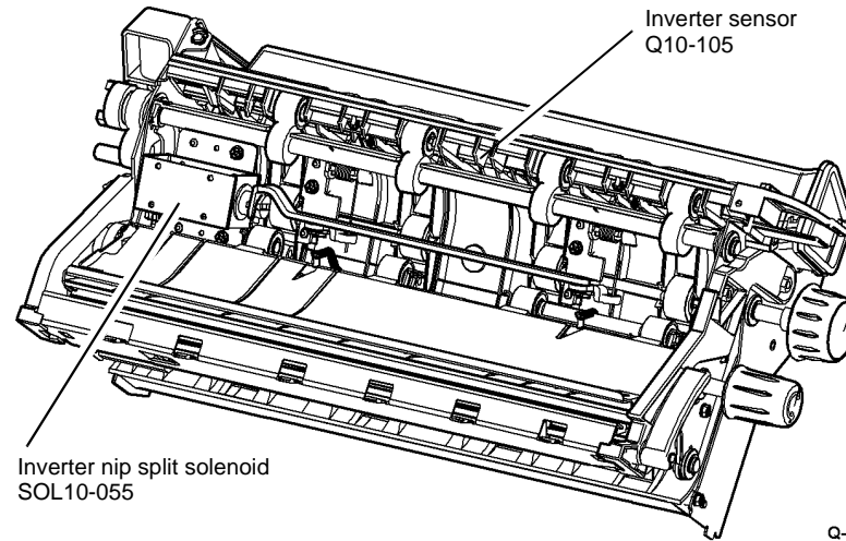
Figure 3 Inverter assembly
