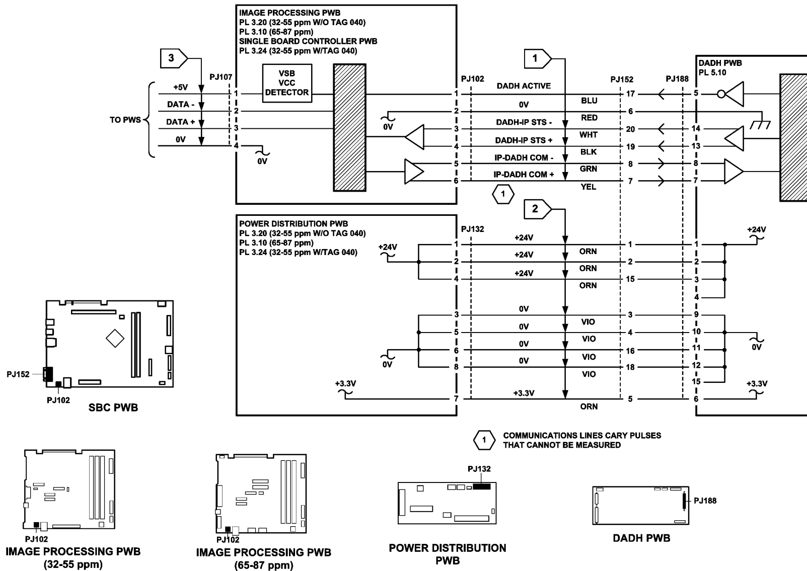
Figure 1 Circuit diagram
