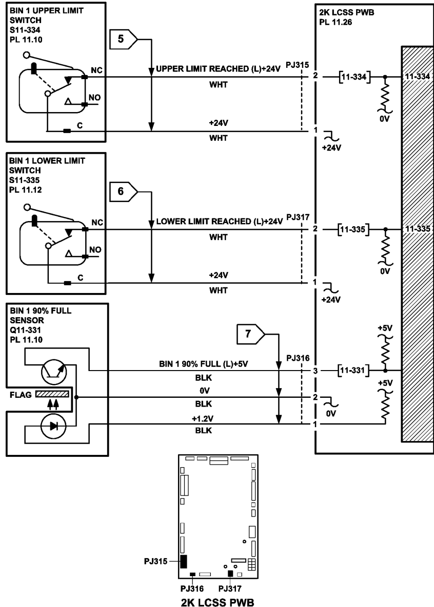
Figure 3 Circuit diagram
