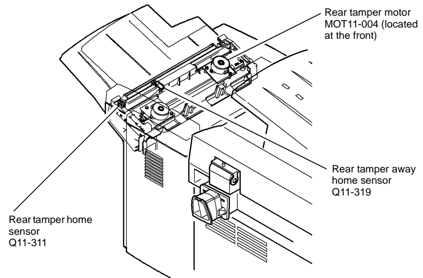
Figure 1 Component Location
