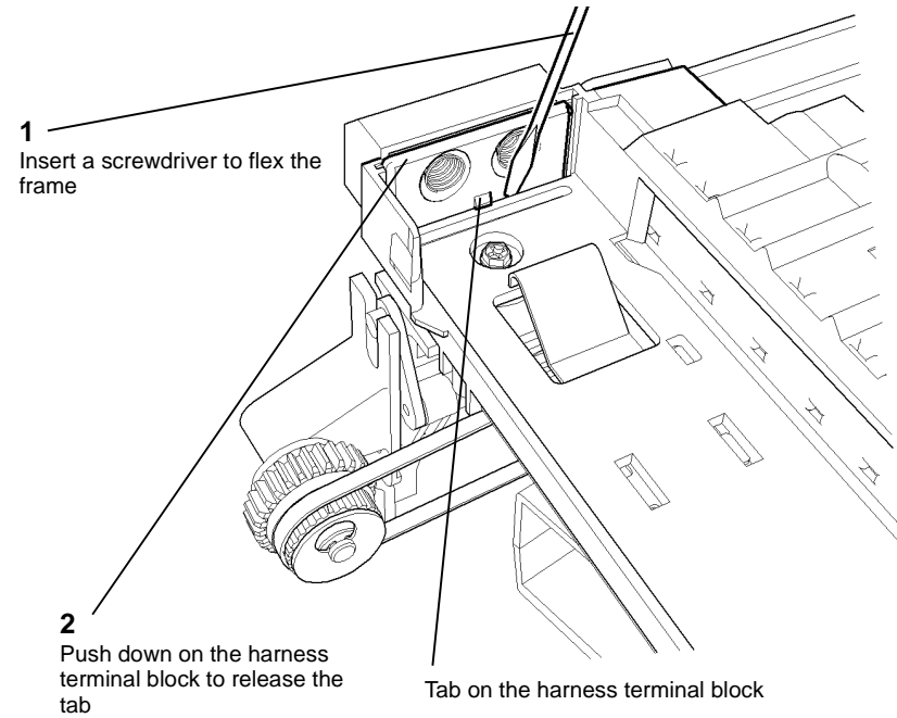
Figure 1 Transfer / detack harness
