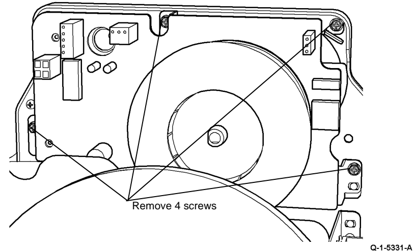
Figure 2 Main drive PWB
