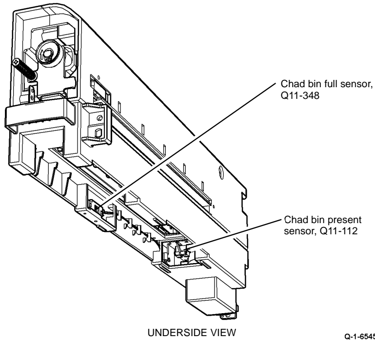
Figure 1 Component location
