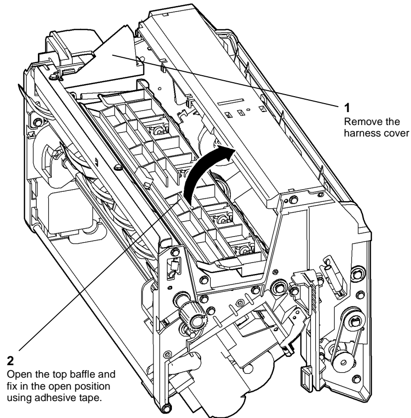
Figure 1 Improving access
