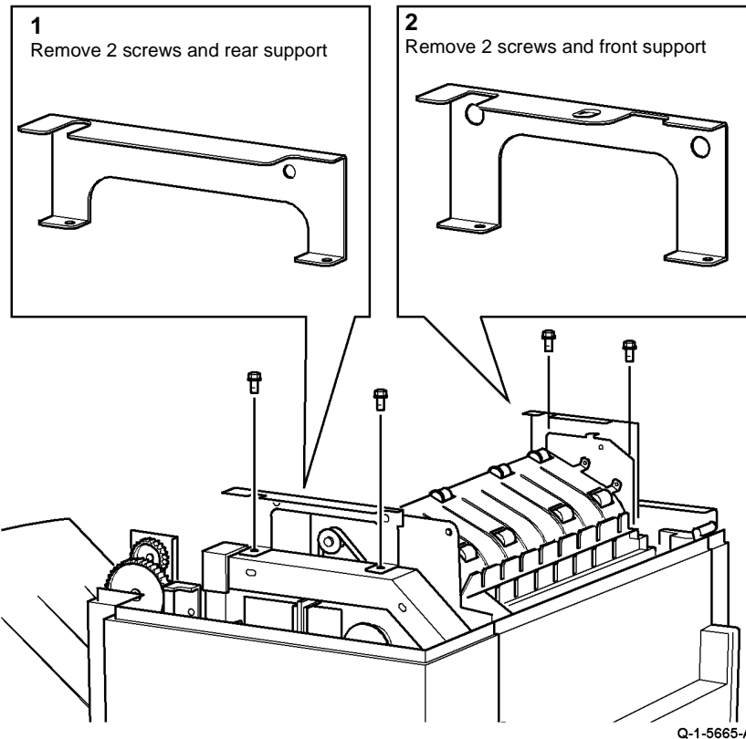
Figure 1 Removing supports
