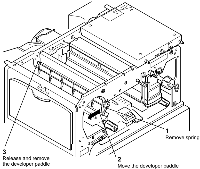
Figure 1 Developer paddle
