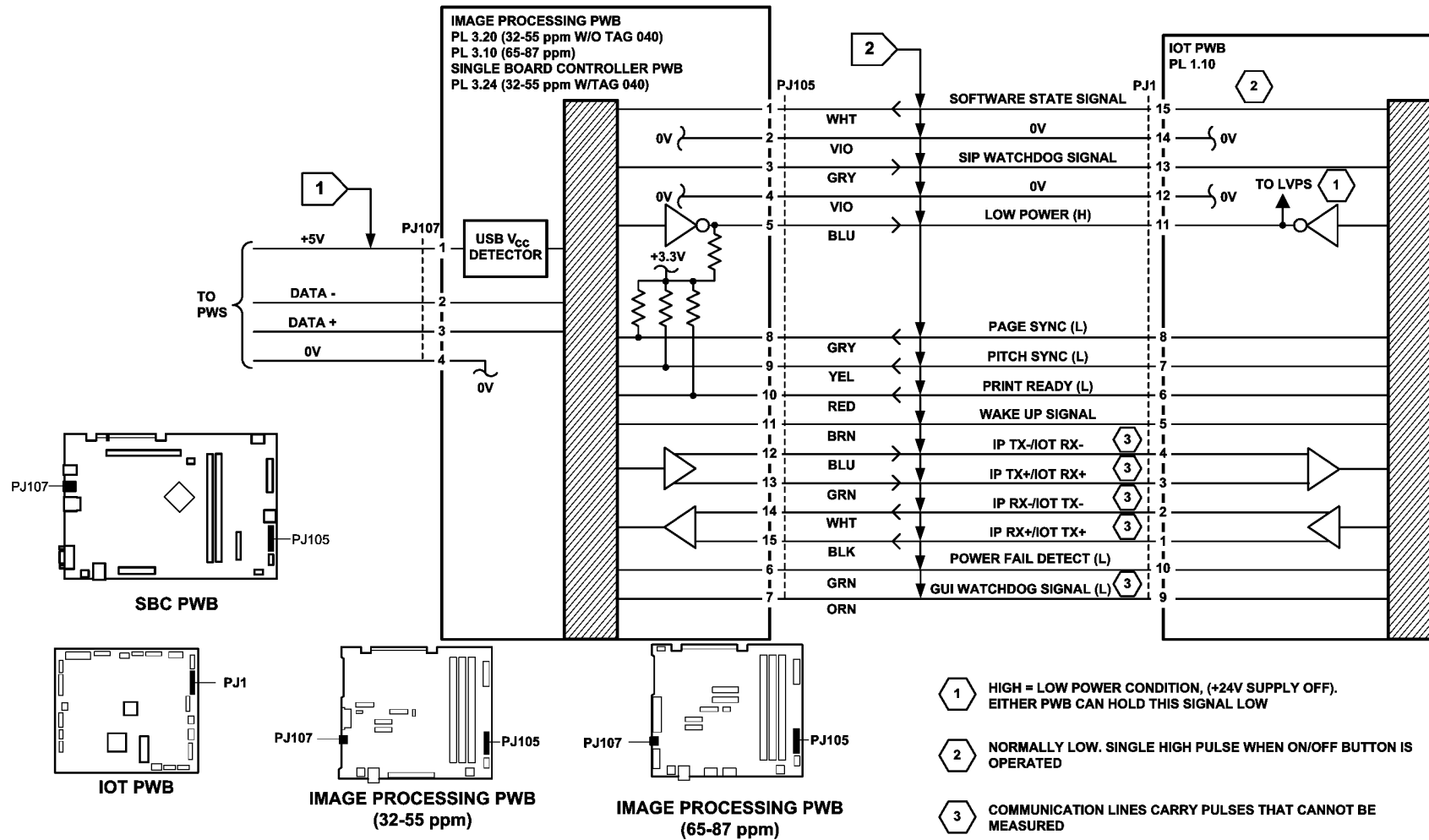
Figure 1 Circuit diagram
