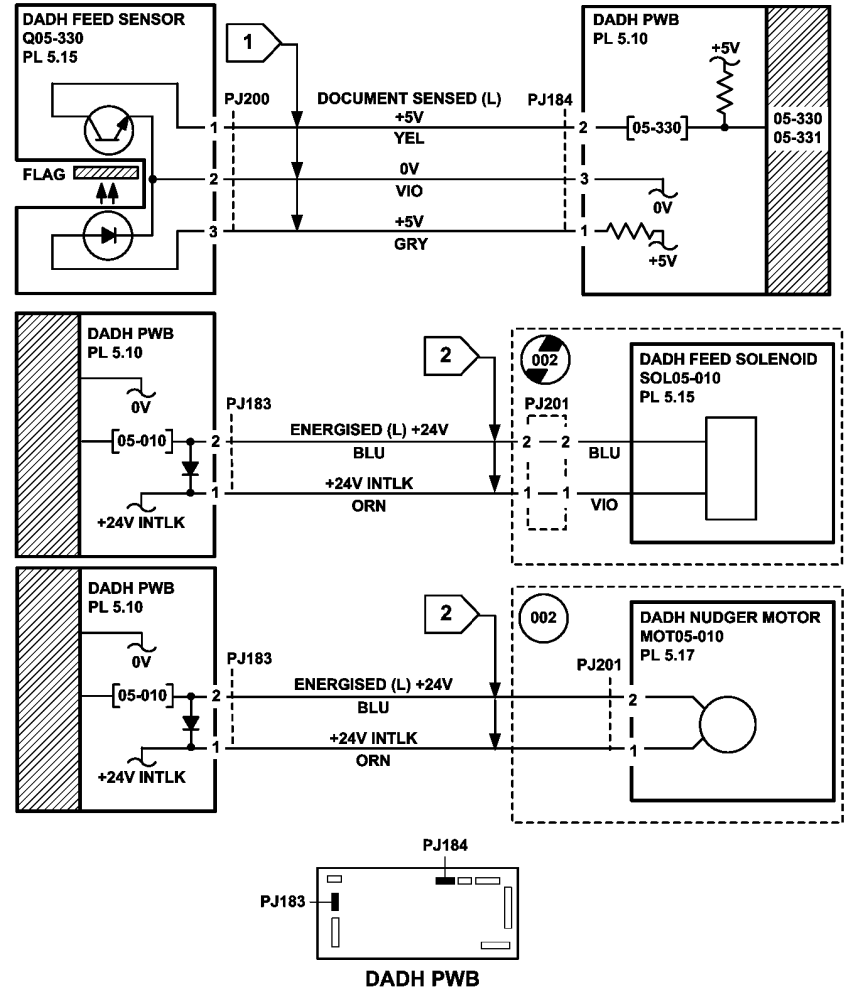
Figure 5 Circuit diagram
