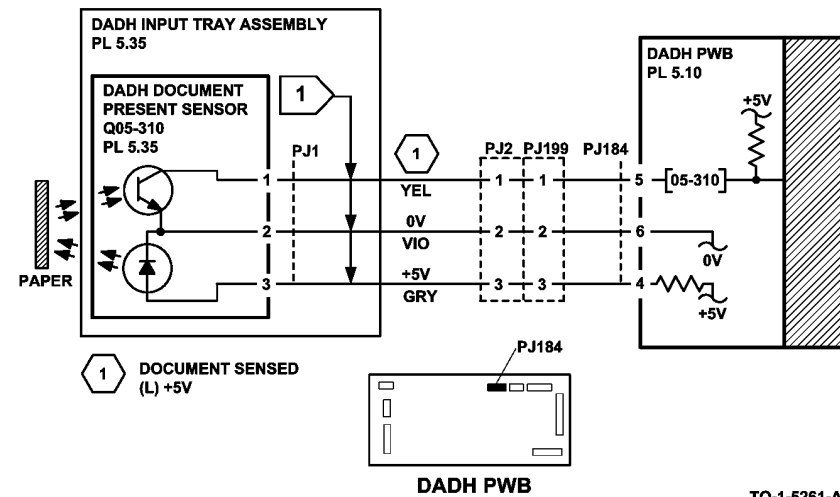
Figure 2 Circuit diagram
