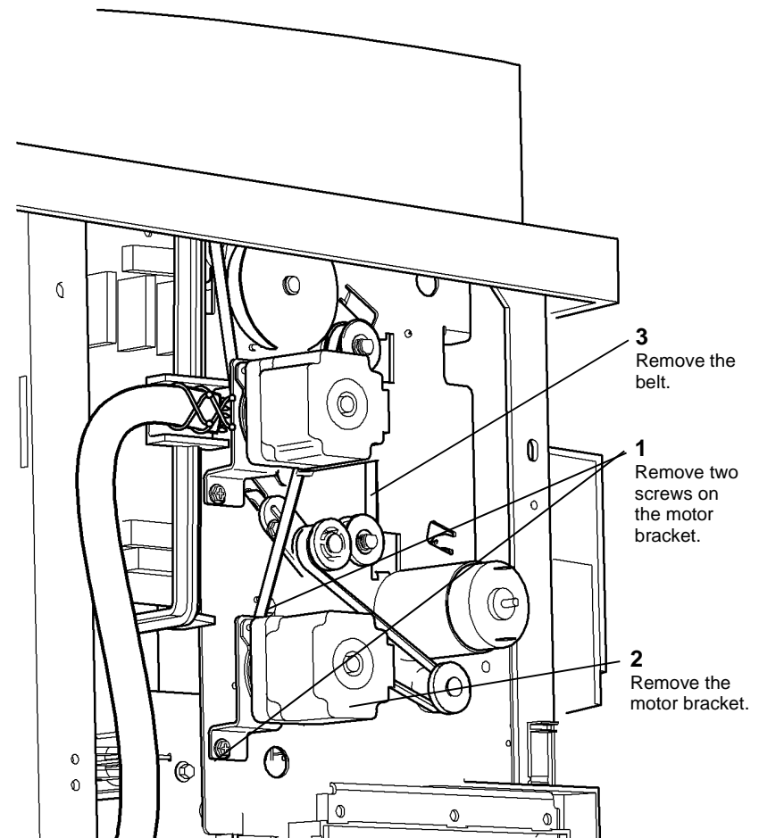
Figure 2 Belt removal
