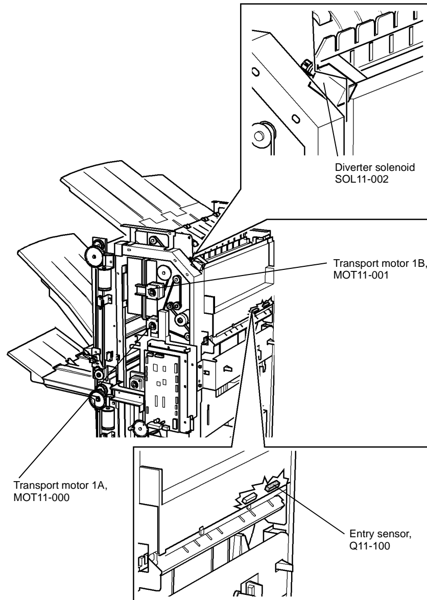
Figure 1 Component location
