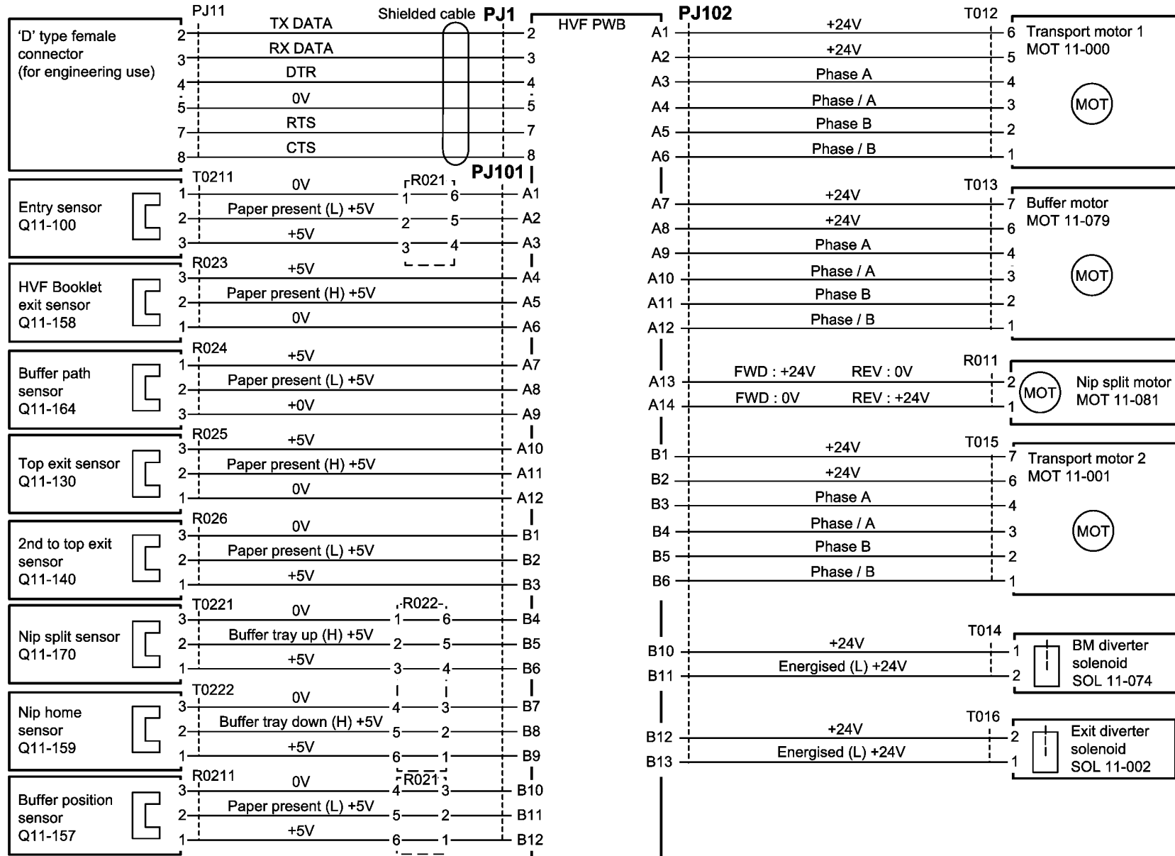
Figure 40 Wiring Diagram 40
