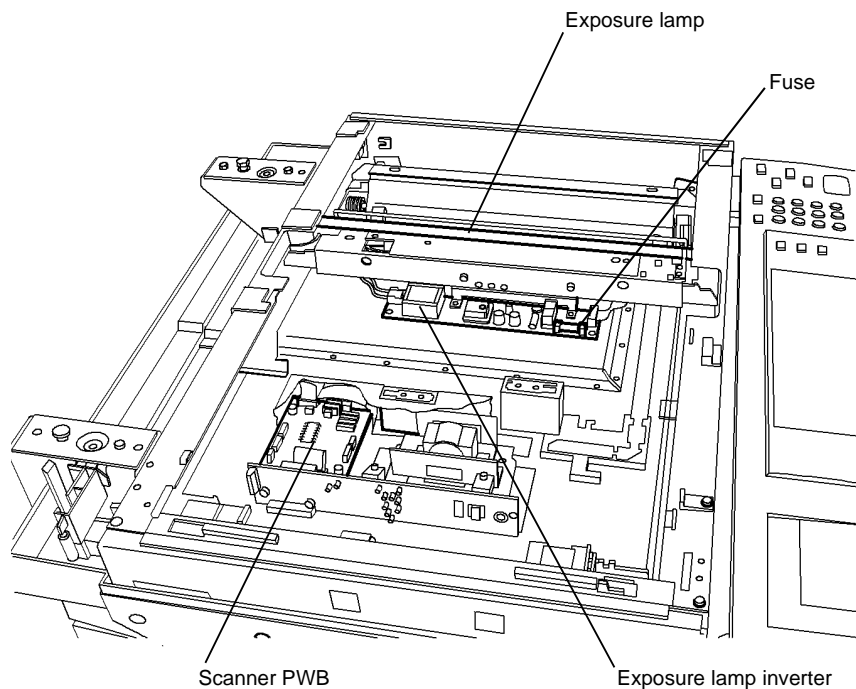
Figure 1 Exposure lamp, inverter and fuse.
