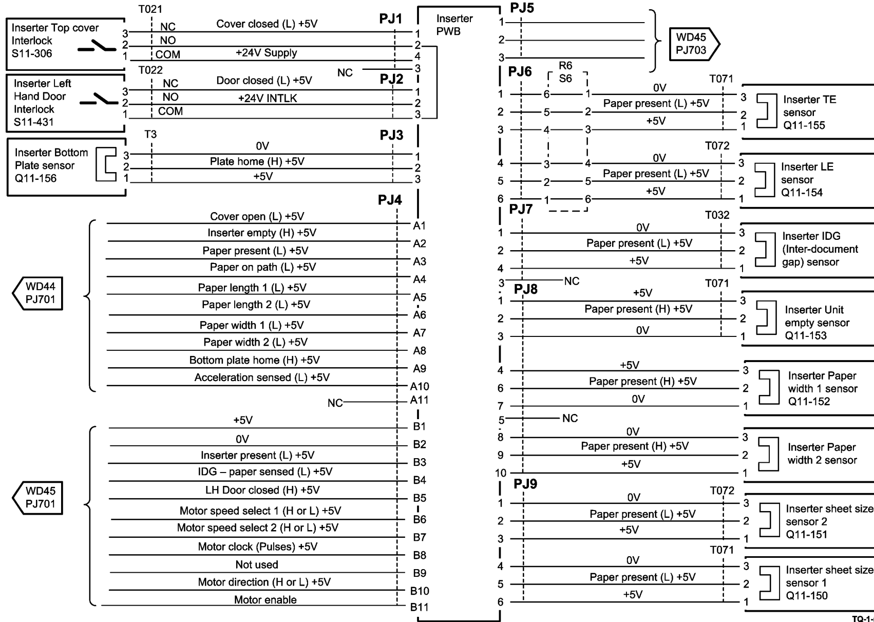
Figure 49 Wiring Diagram 49
