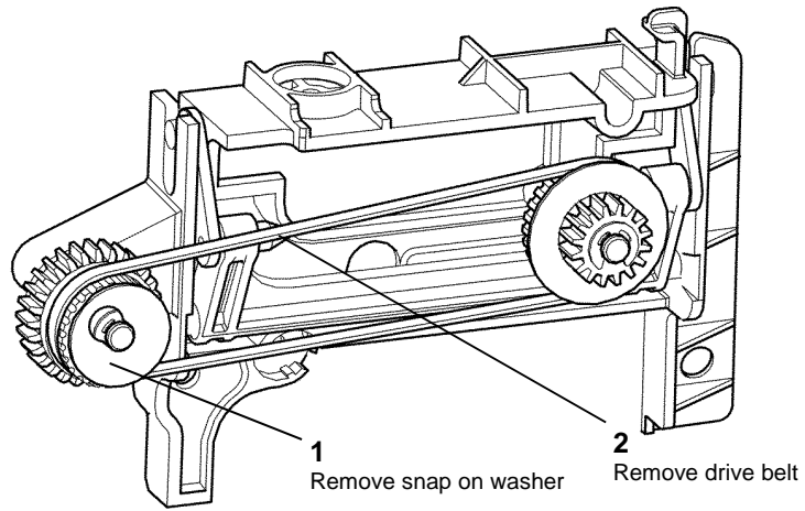
Figure 5 Remove the drive belt
