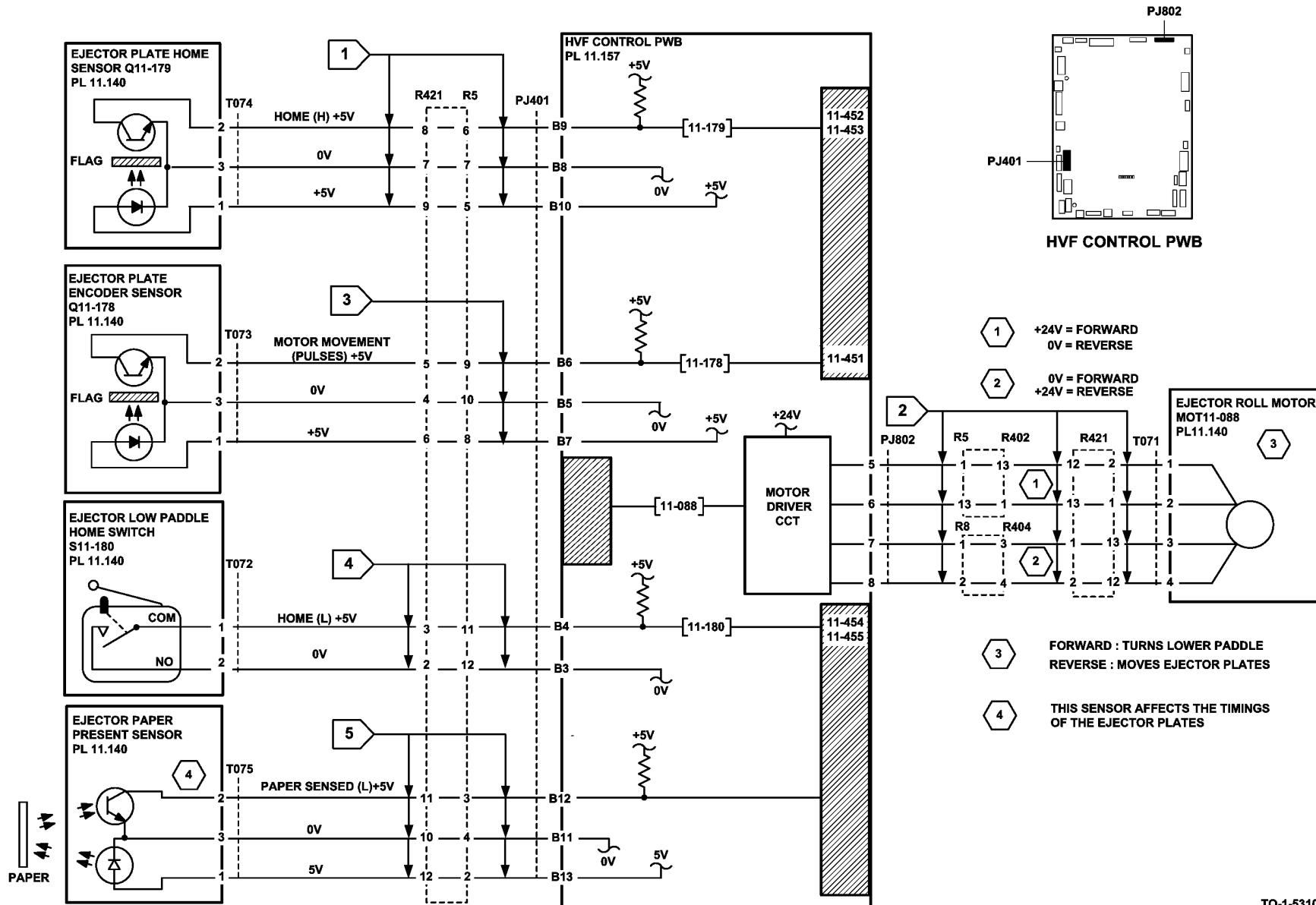
Figure 4 Circuit diagram
