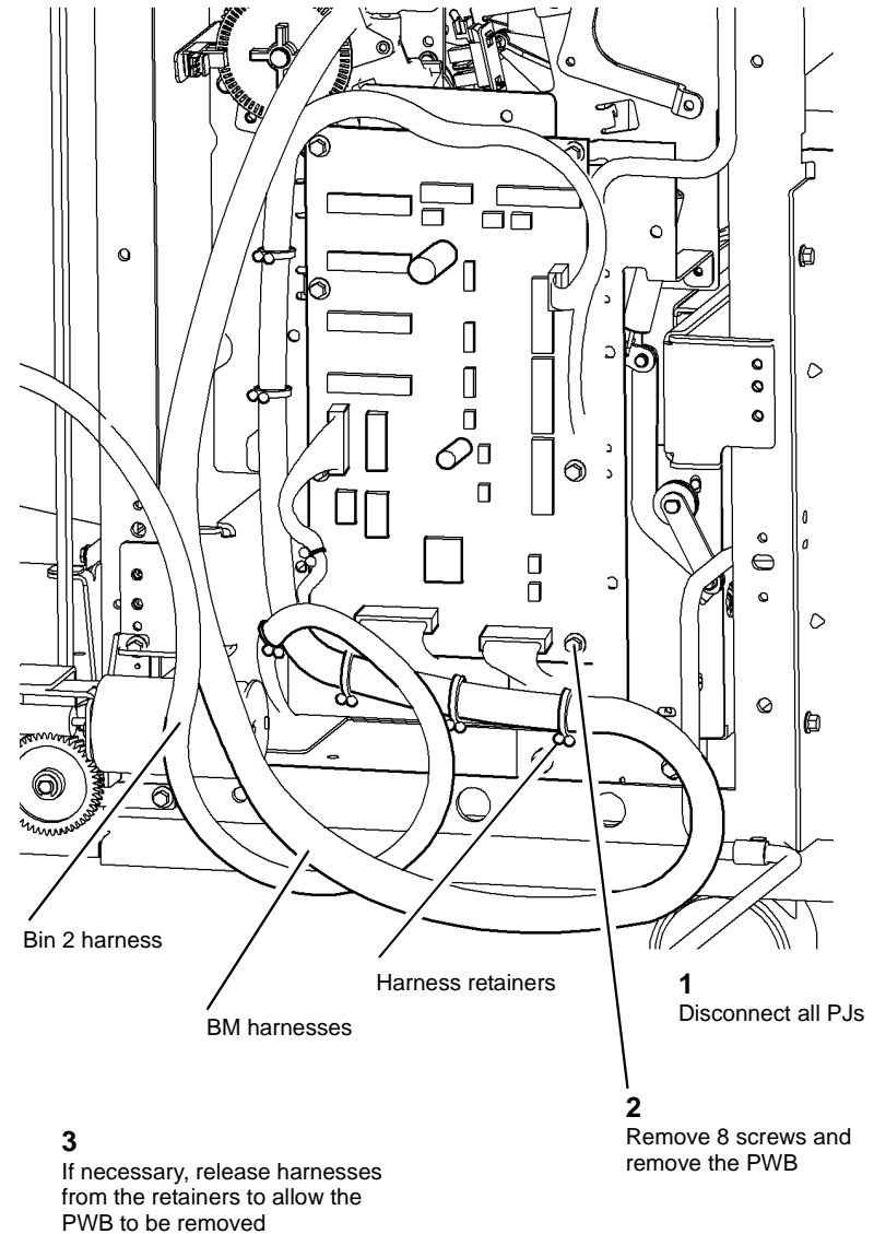
Figure 1 PWB removal
