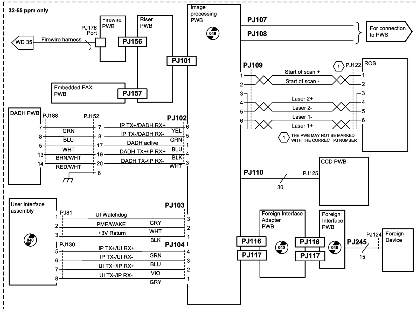
Figure 8 Wiring Diagram 8 (W/OTAG 040)
