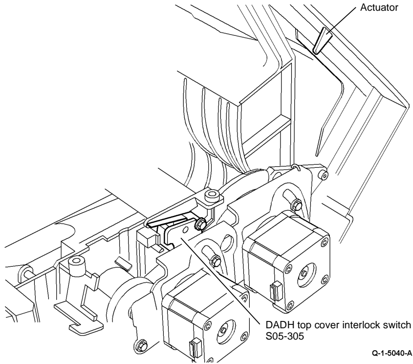
Figure 1 Component location
