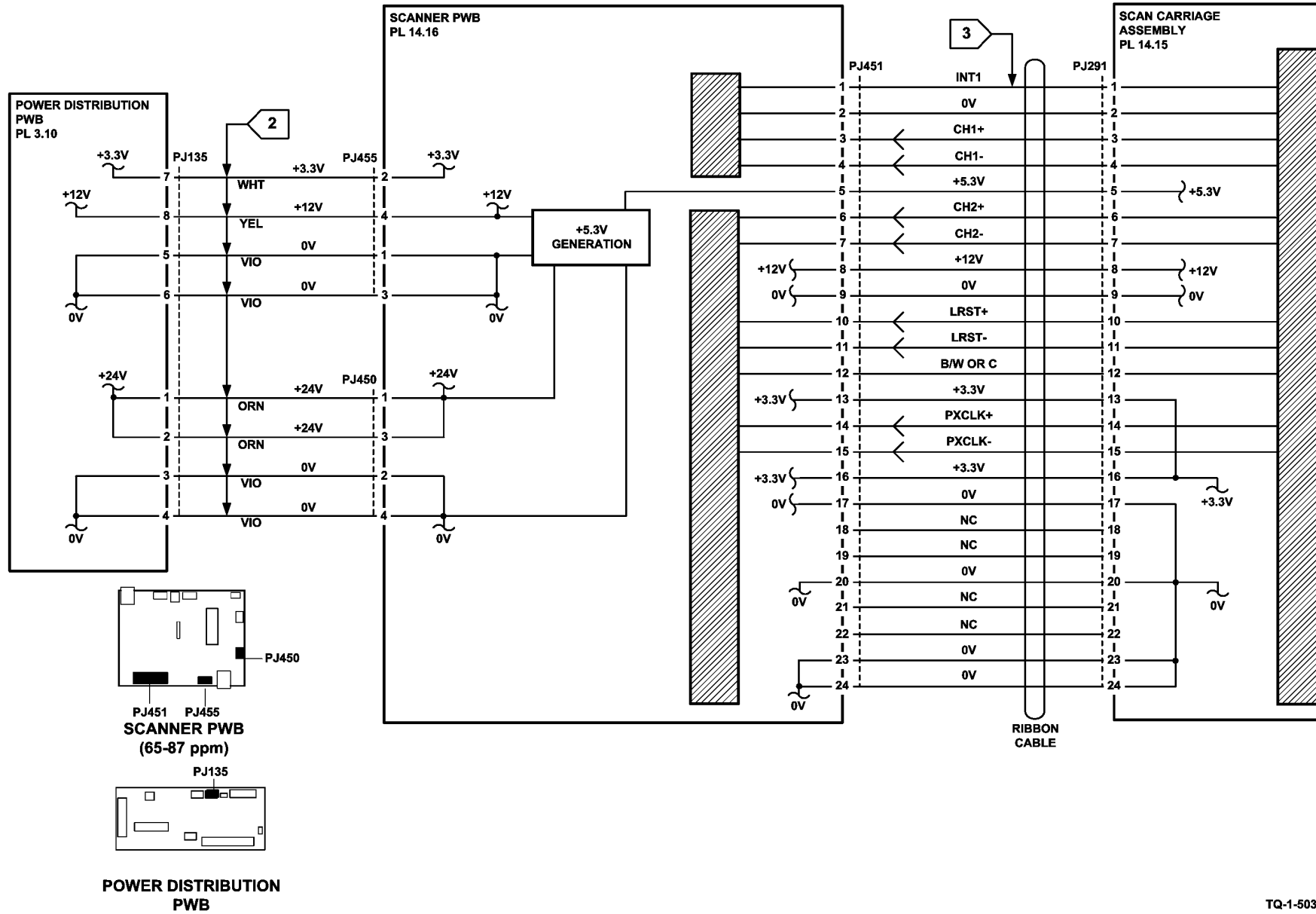
Figure 2 Circuit diagram
