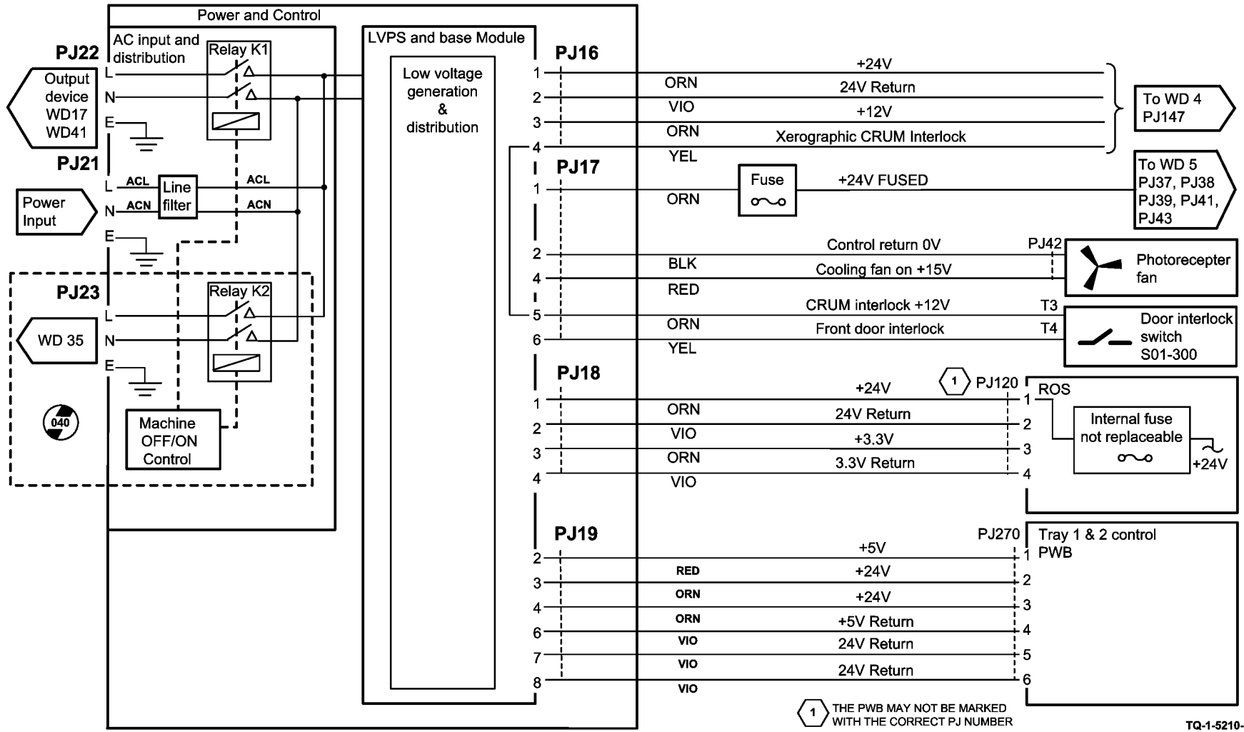
Figure 1 Wiring Diagram 1
