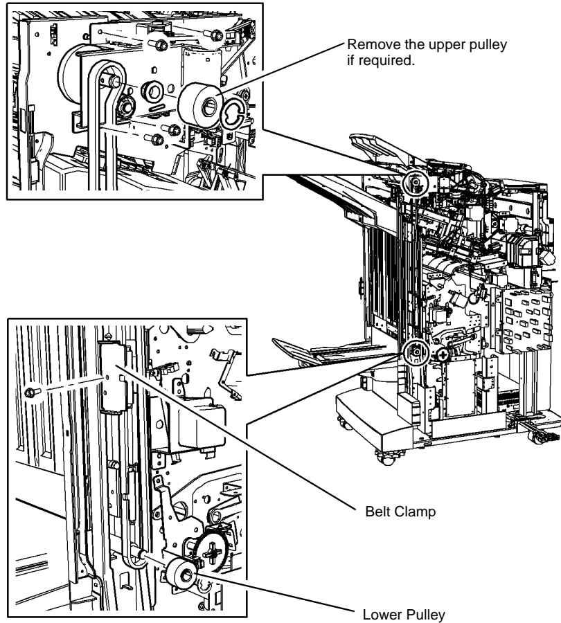
Figure 1 Stacker Driving Belts
