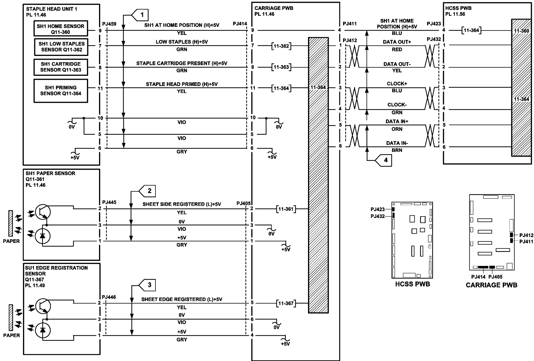
Figure 4 Circuit diagram
