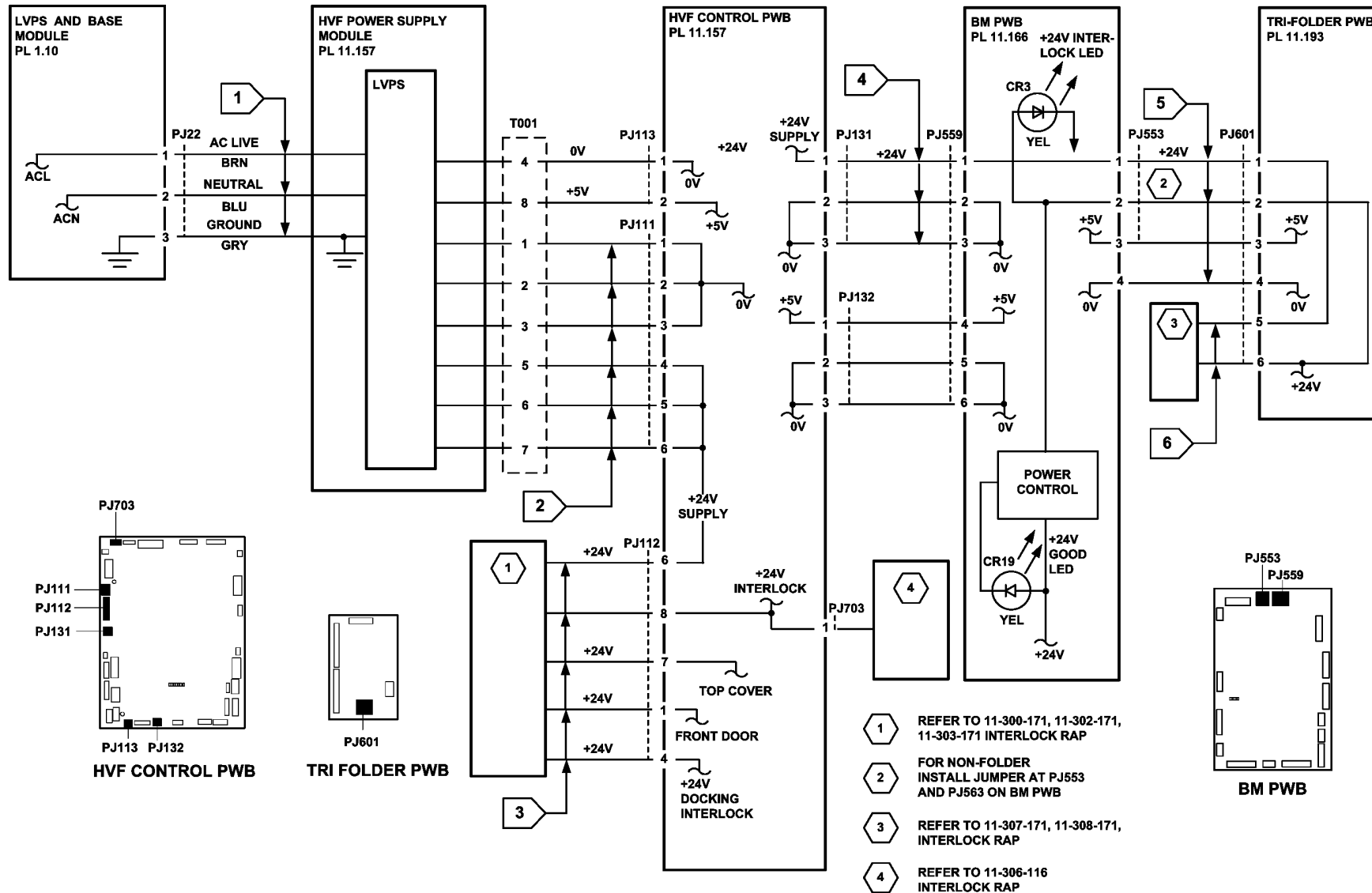
Figure 2 Circuit diagram
