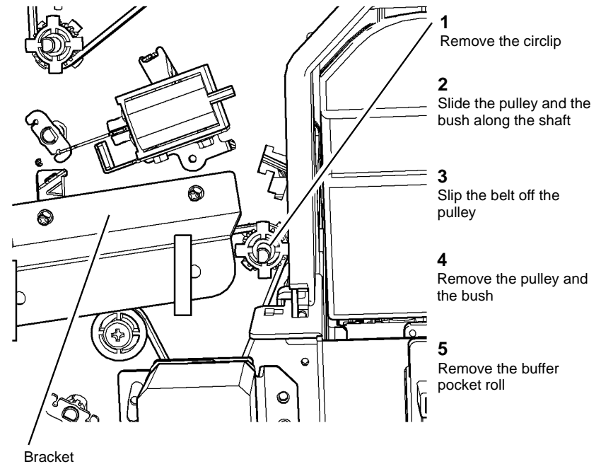
Figure 2 Buffer pocket roll removal.
