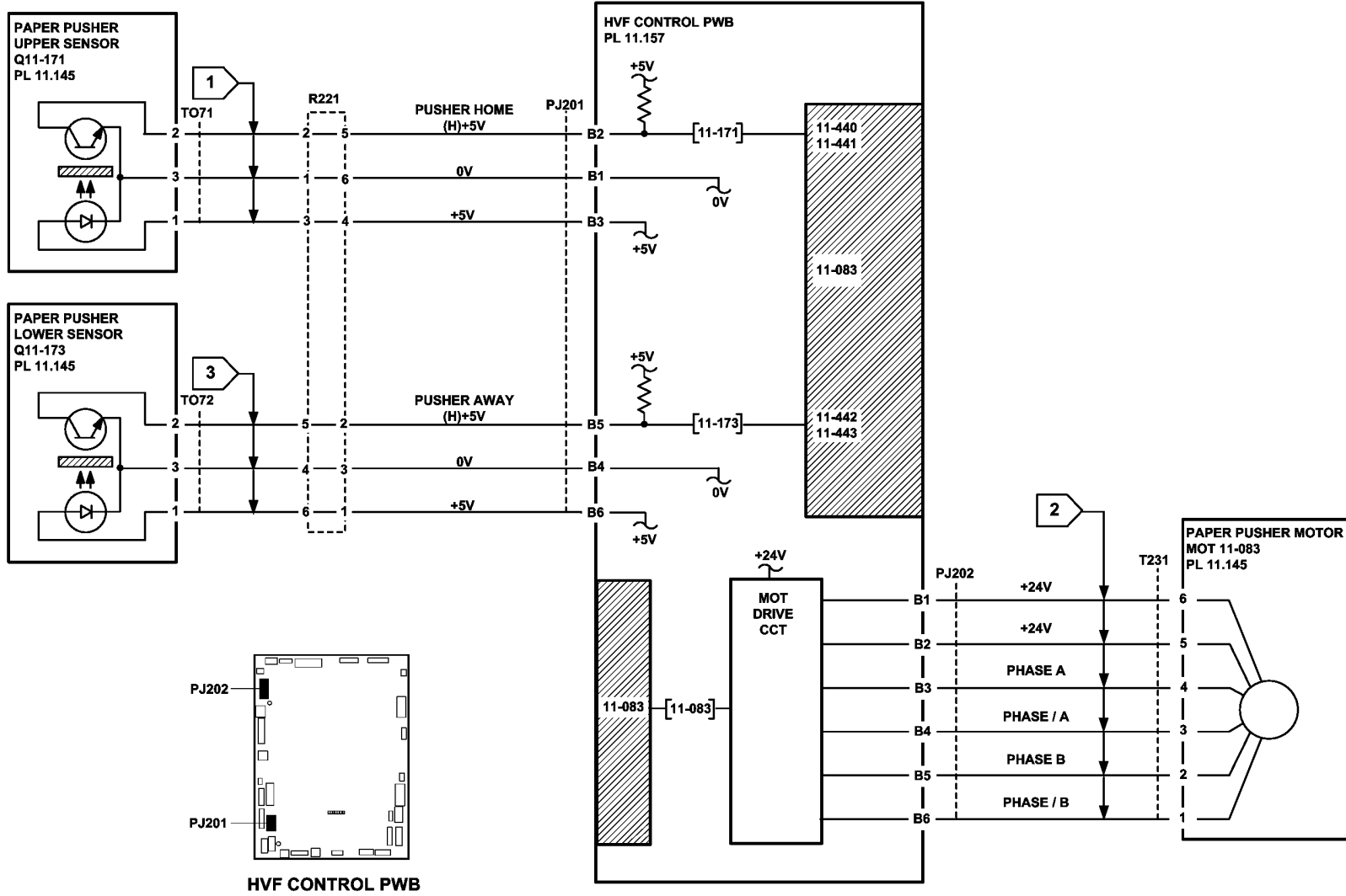
Figure 2 Circuit diagram
