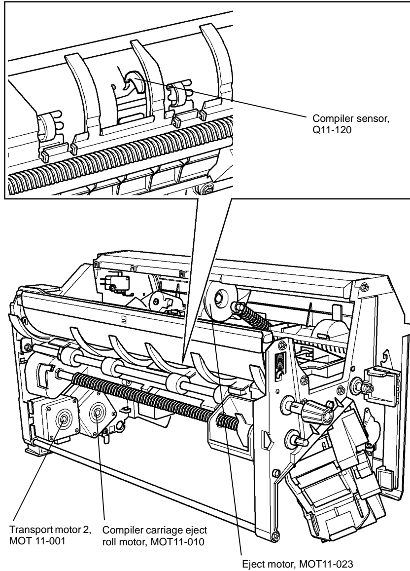
Figure 1 Component location
