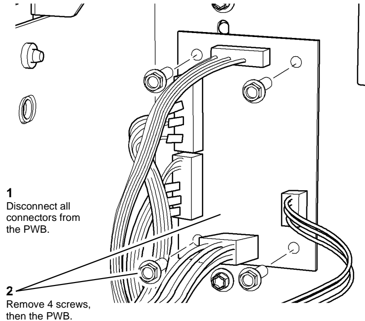
Figure 1 PWB removal
