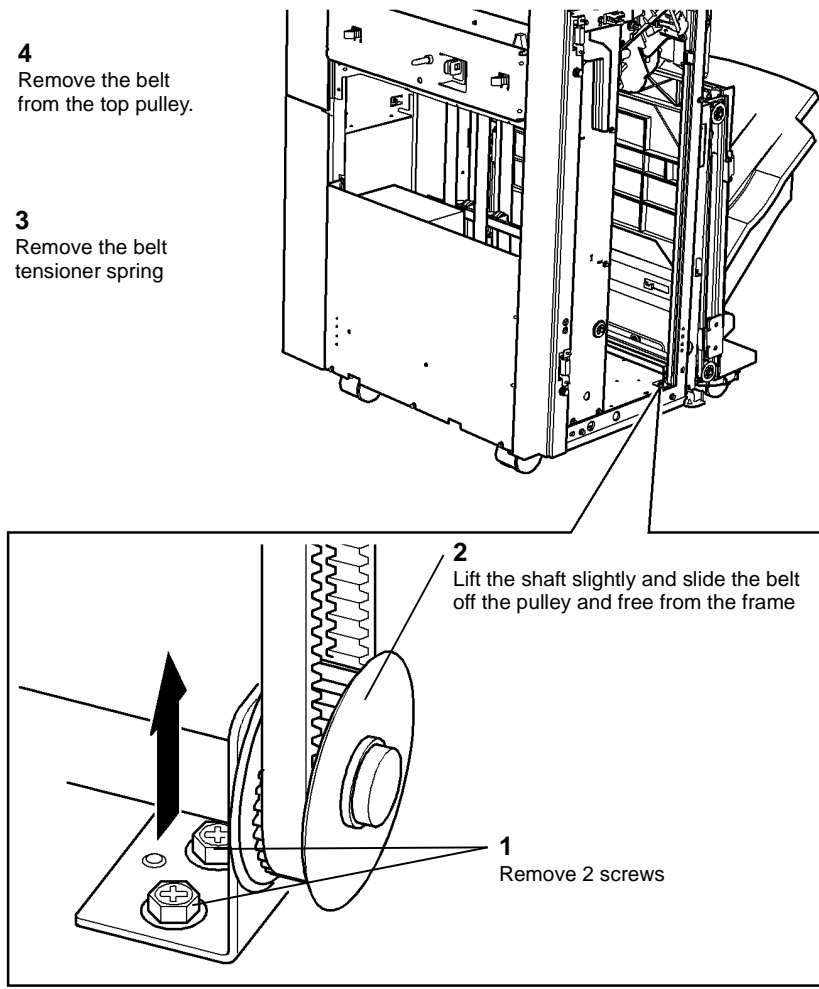
Figure 8 Releasing the belt
