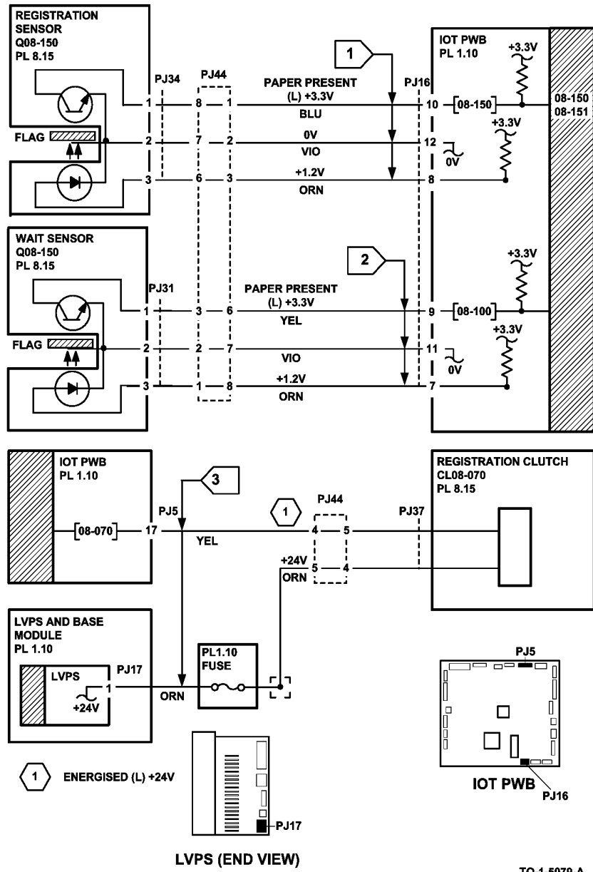
Figure 2 Circuit diagram
