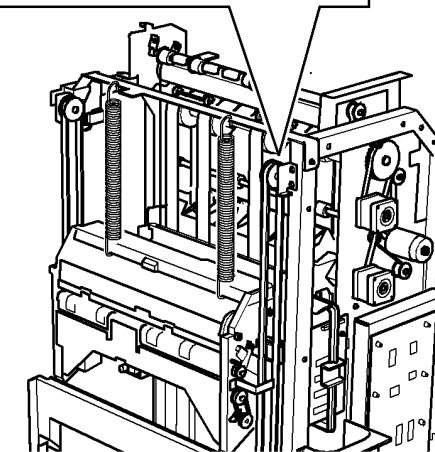
Figure 6 Releasing belts
