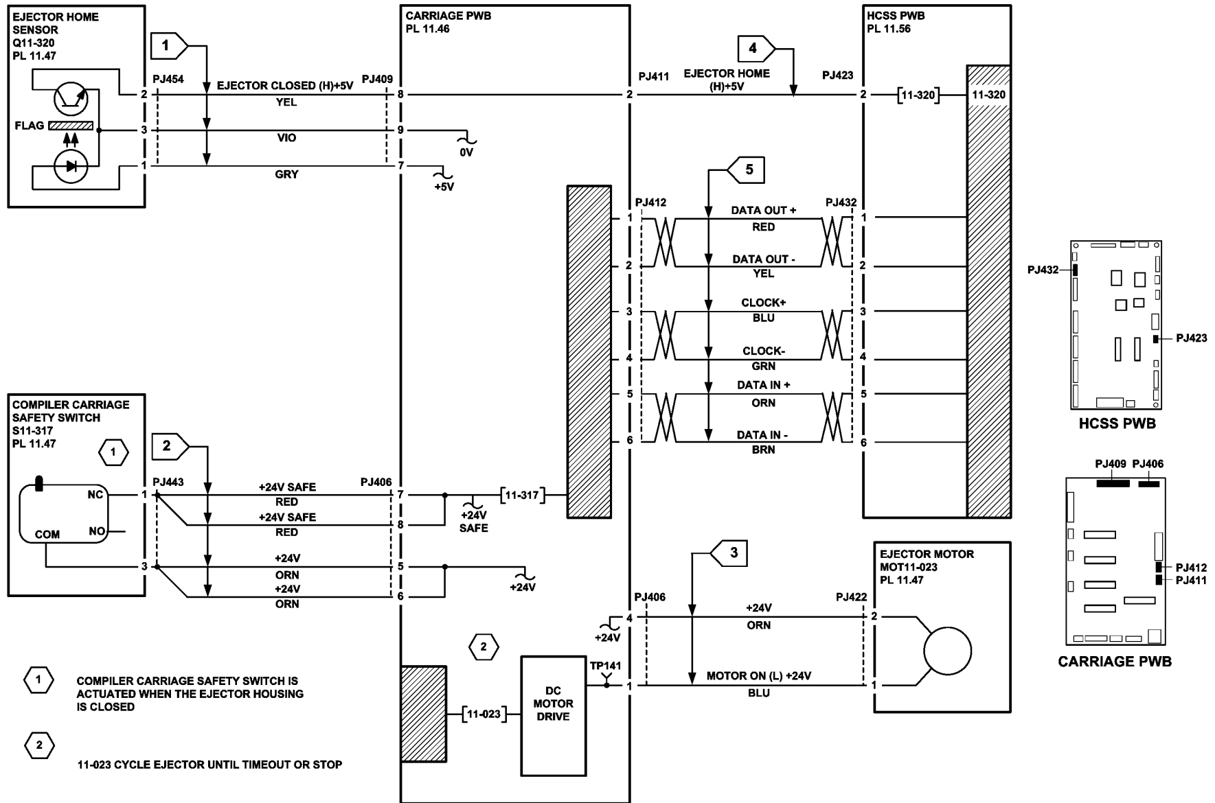
Figure 2 Circuit diagram
