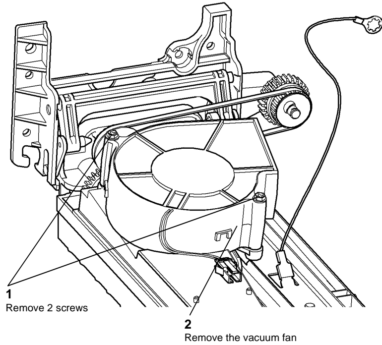
Figure 3 Remove vacuum fan
