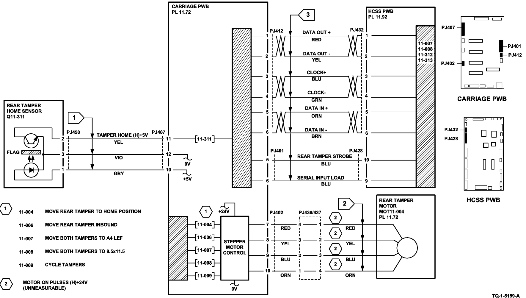
Figure 2 Circuit diagram
