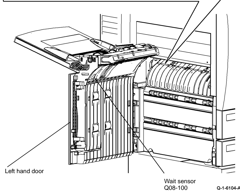
Figure 1 Component location
