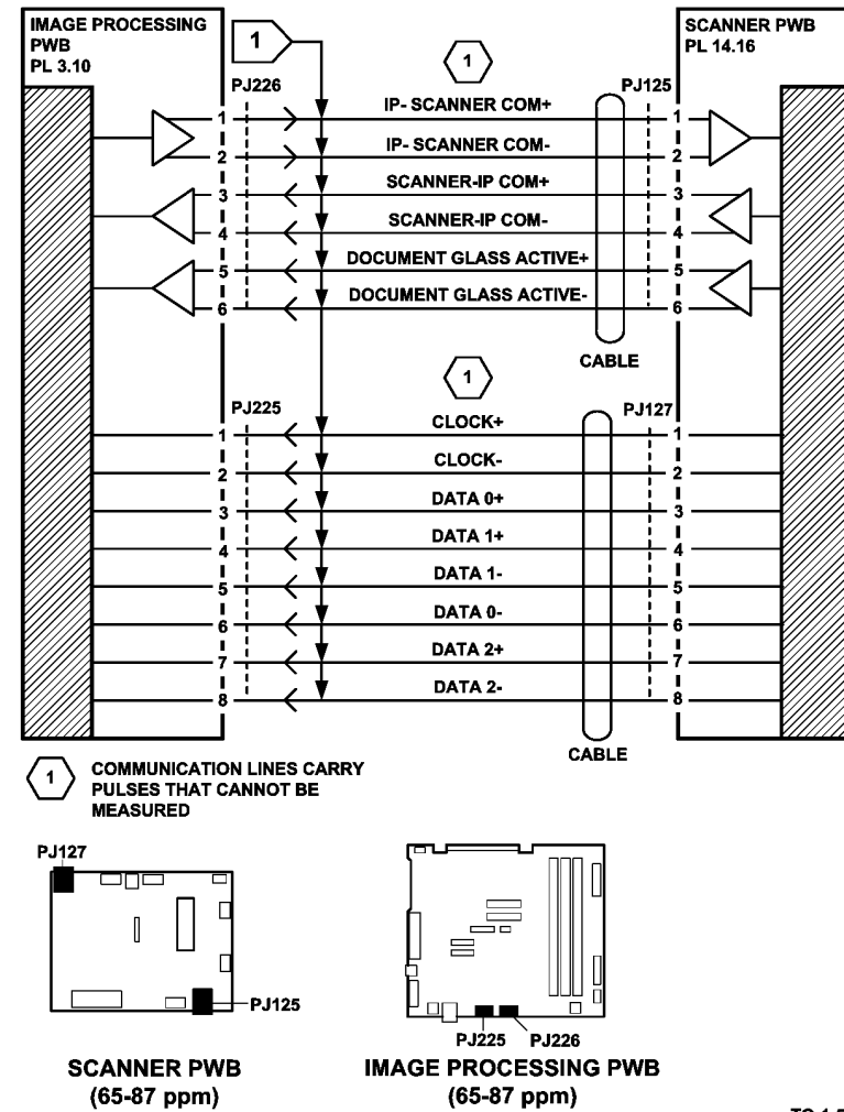
Figure 1 Circuit diagram
