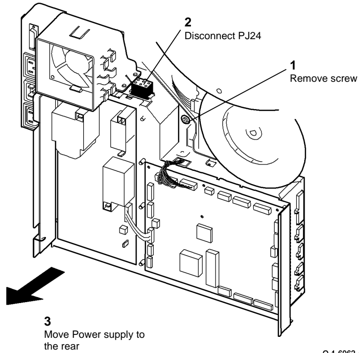
Figure 2 Power supply
