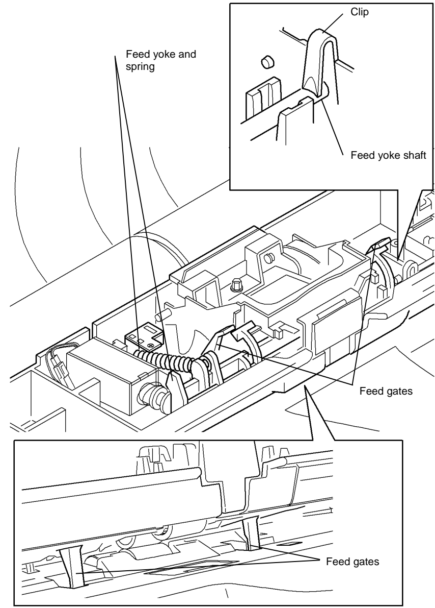
Figure 3 Component location W/OTAG D002
