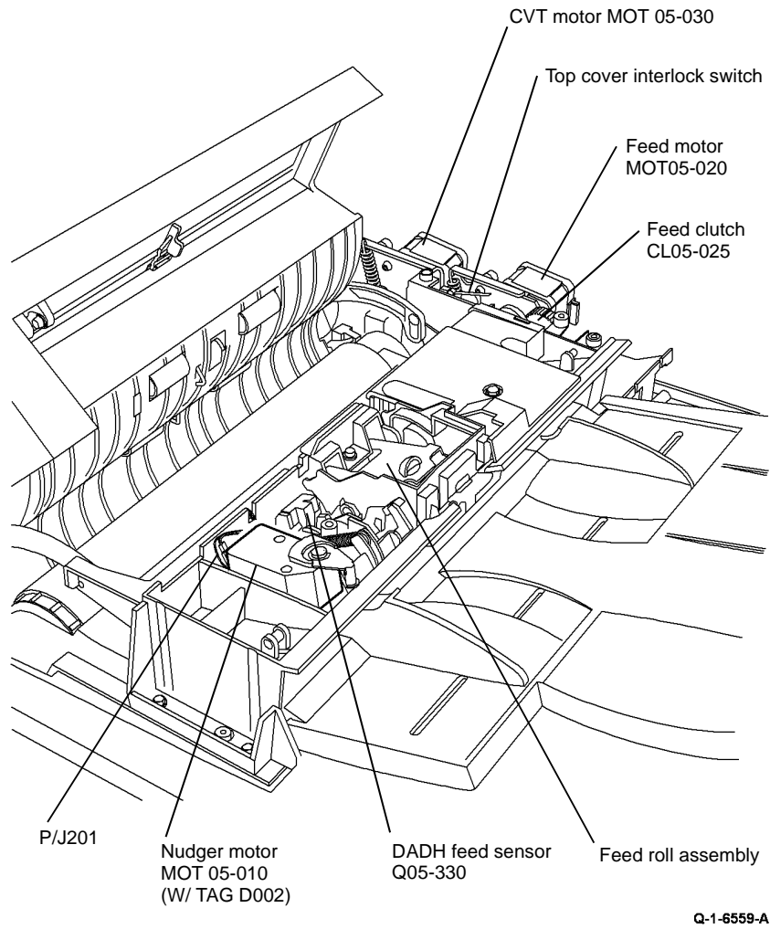
Figure 2 Component location W/TAG D002
