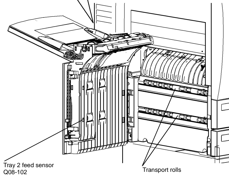
Figure 1 Component location
