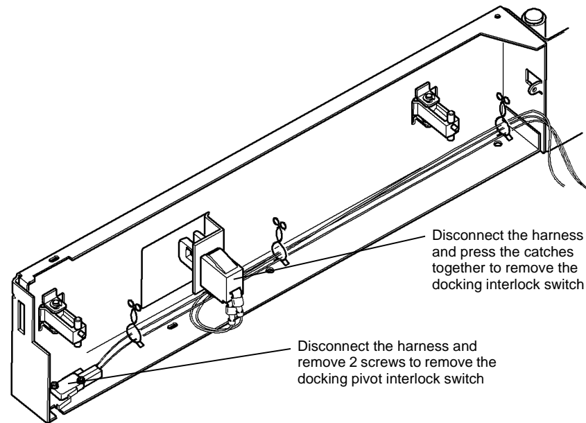
Figure 5 Switch removal
