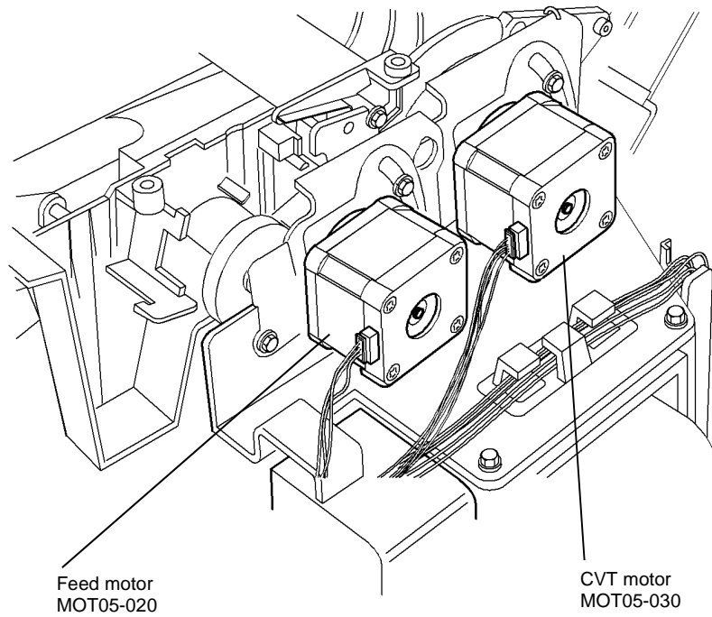
Figure 1 Component location
