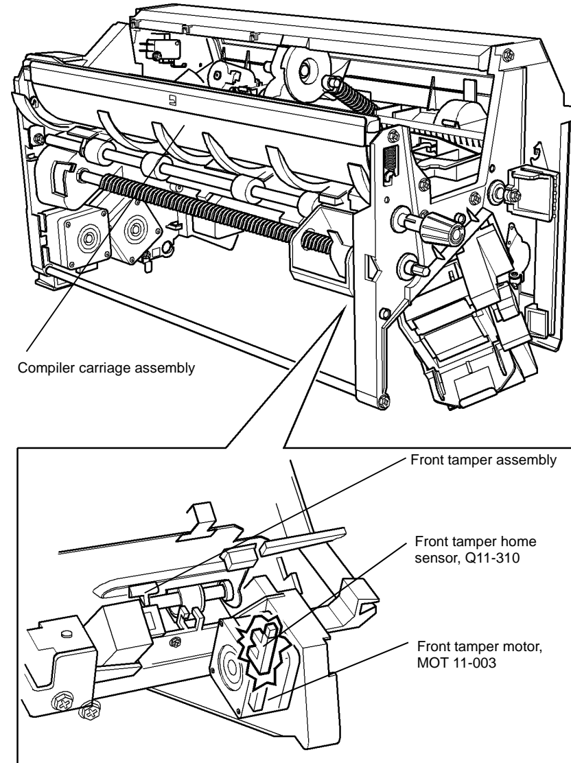
Figure 1 Component location
