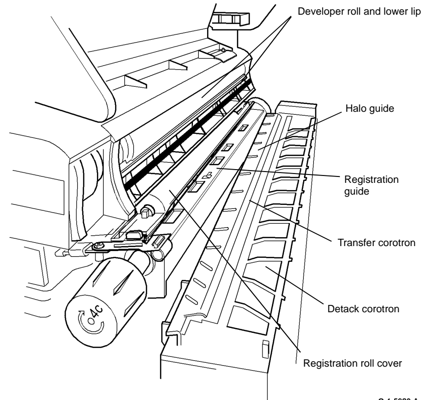
Figure 1 Component location
