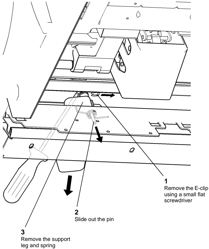
Figure 4 Leg and spring removal
