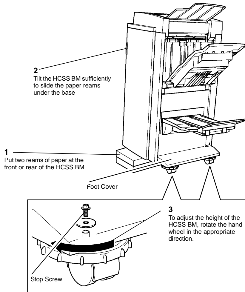
Figure 2 Adjustable castor
