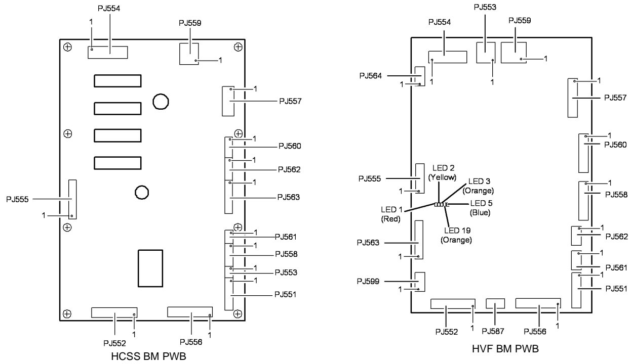
Figure 15 BM PWB
