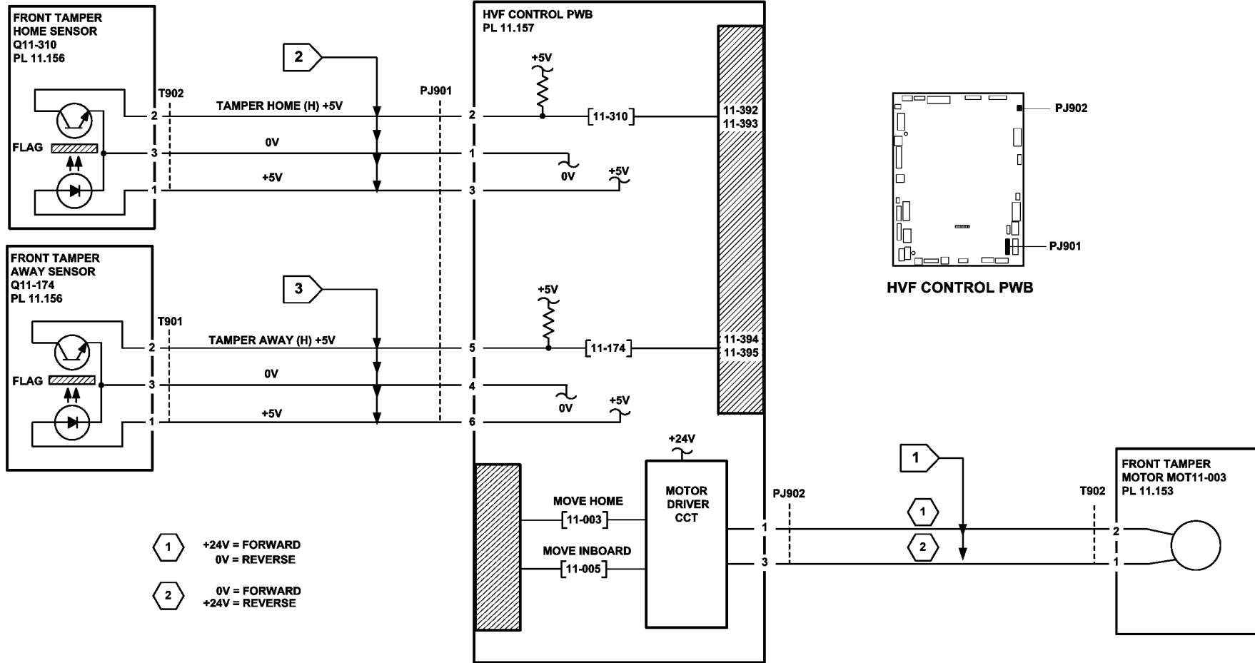
Figure 2 Circuit diagram
