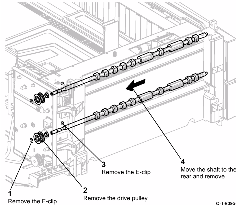
Figure 2 Remove the drive shaft
