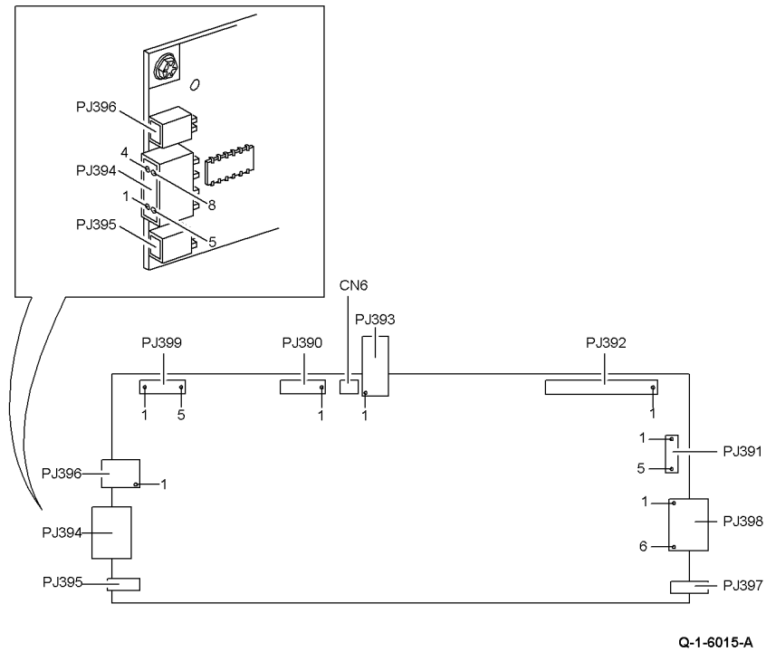
Figure 3 HCF control PWB
