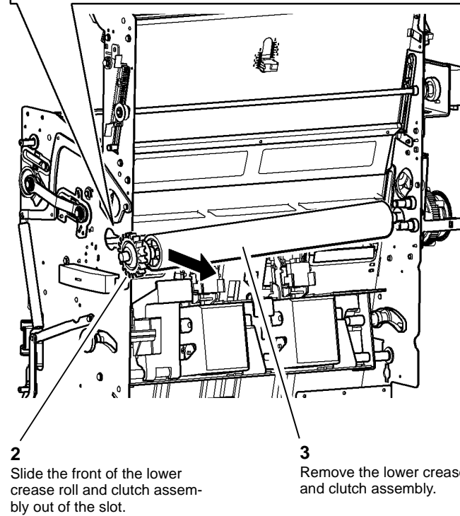
Figure 4 Lower crease roll and clutch removal
