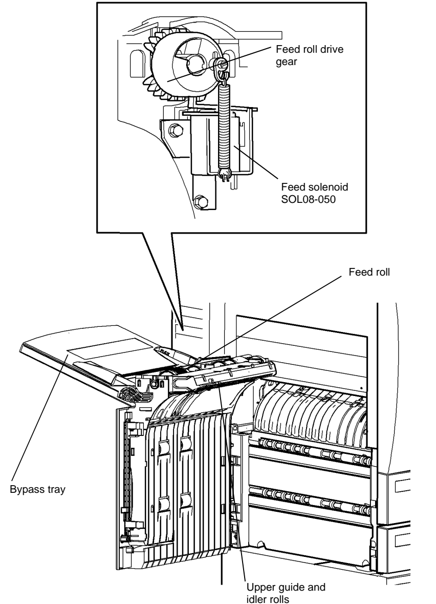
Figure 1 Component location
