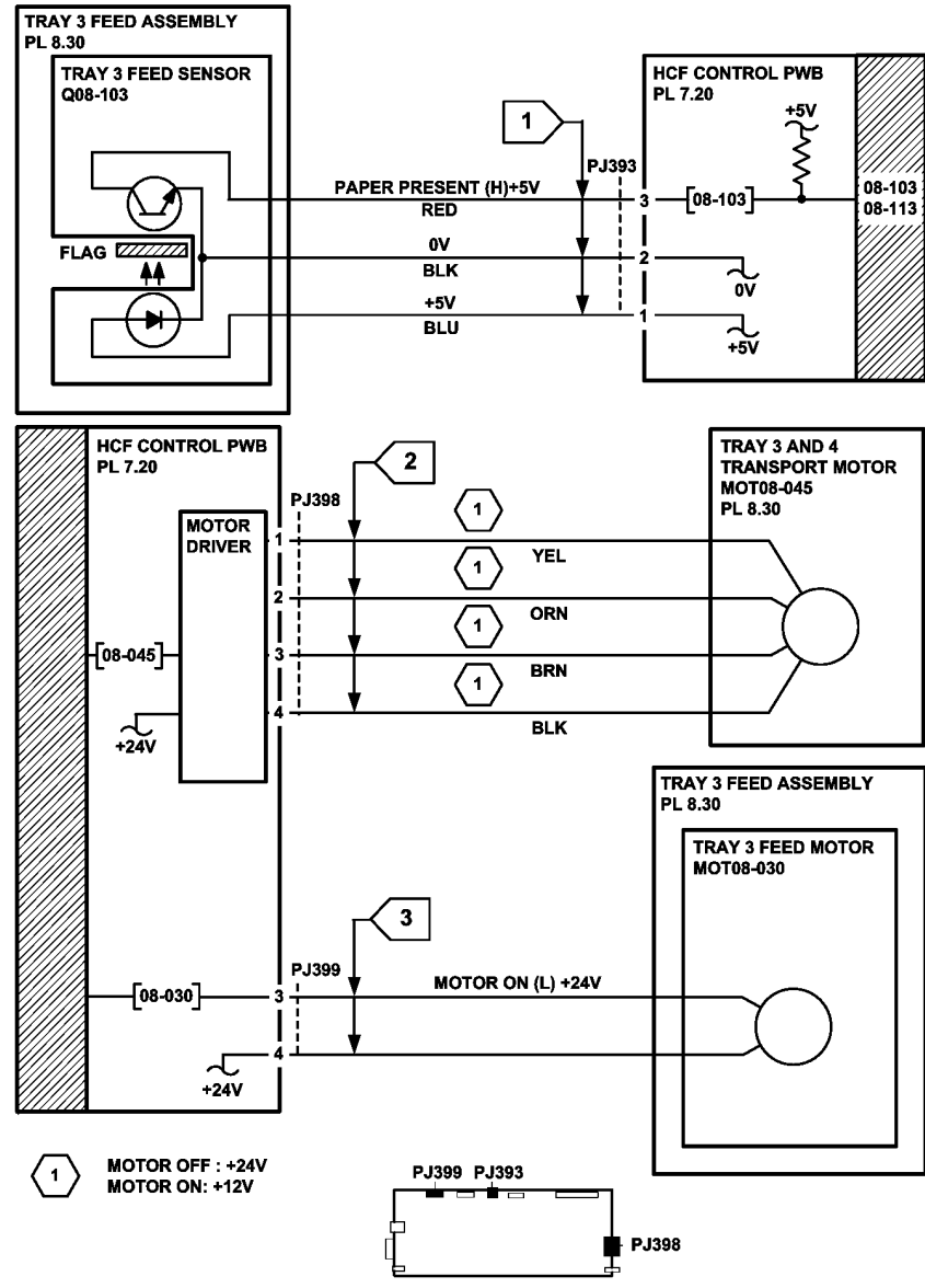
Figure 2 Circuit diagram
