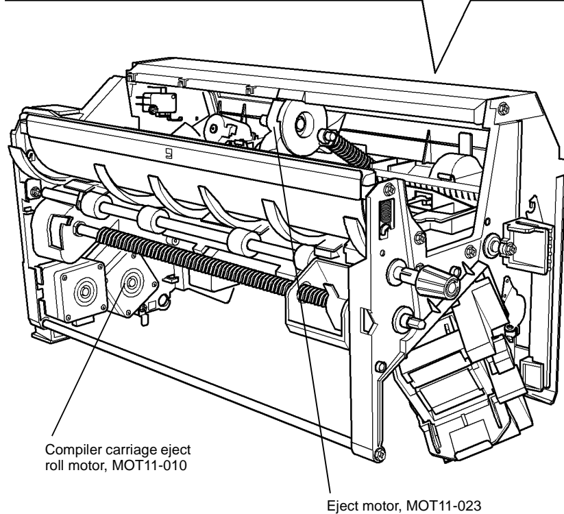
Figure 1 Component location
