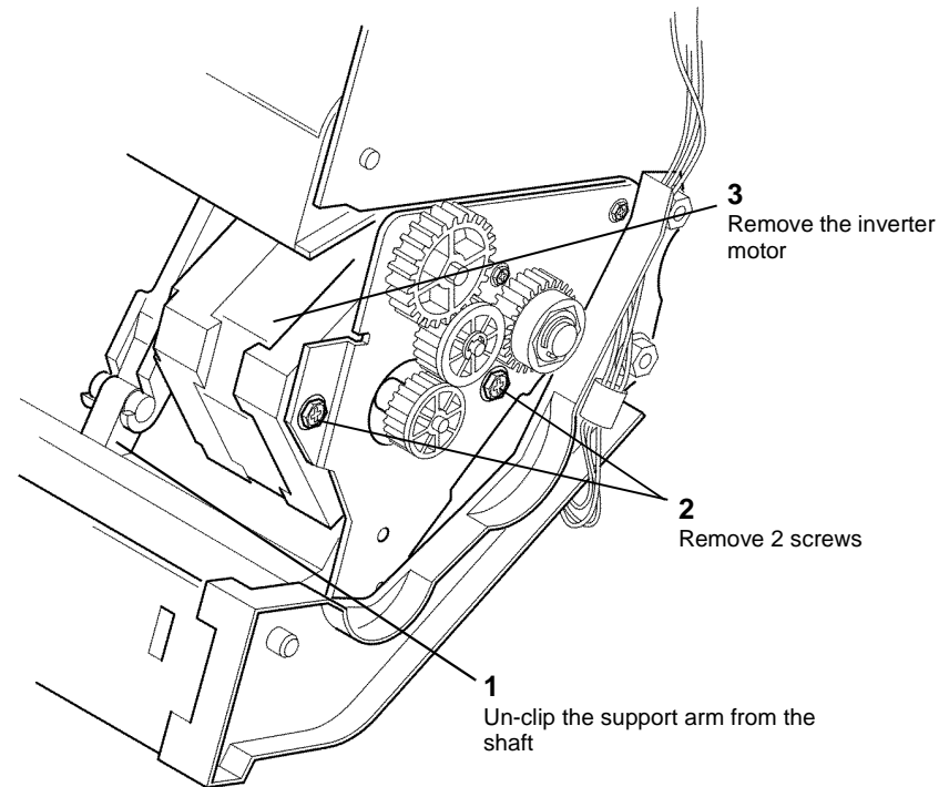
Figure 1 Inverter motor
