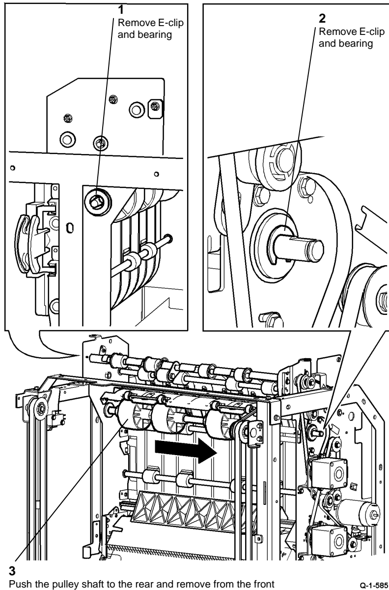
Figure 1 Pulley removal
