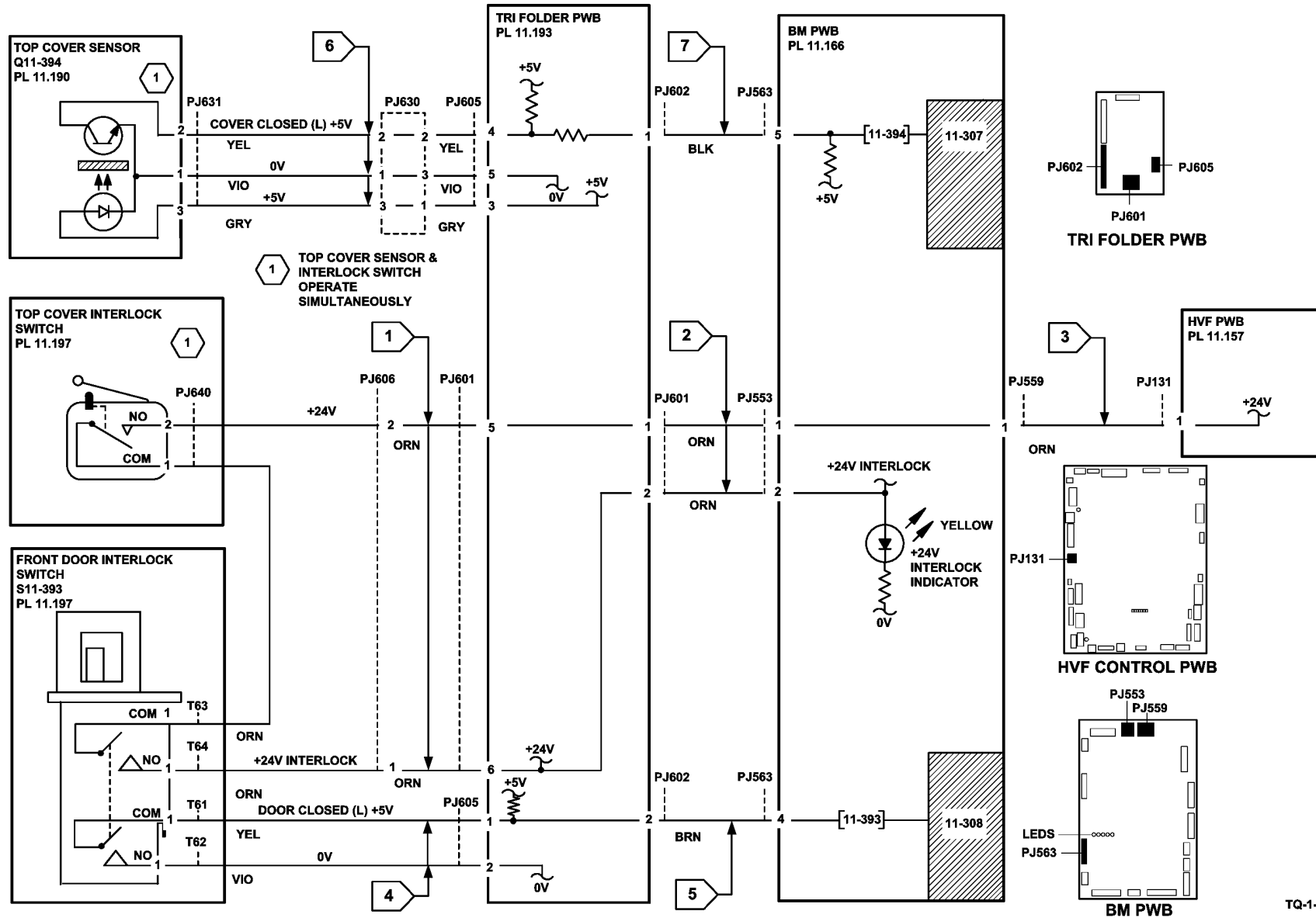
Figure 2 Circuit diagram
