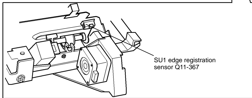
Figure 1 Component location
