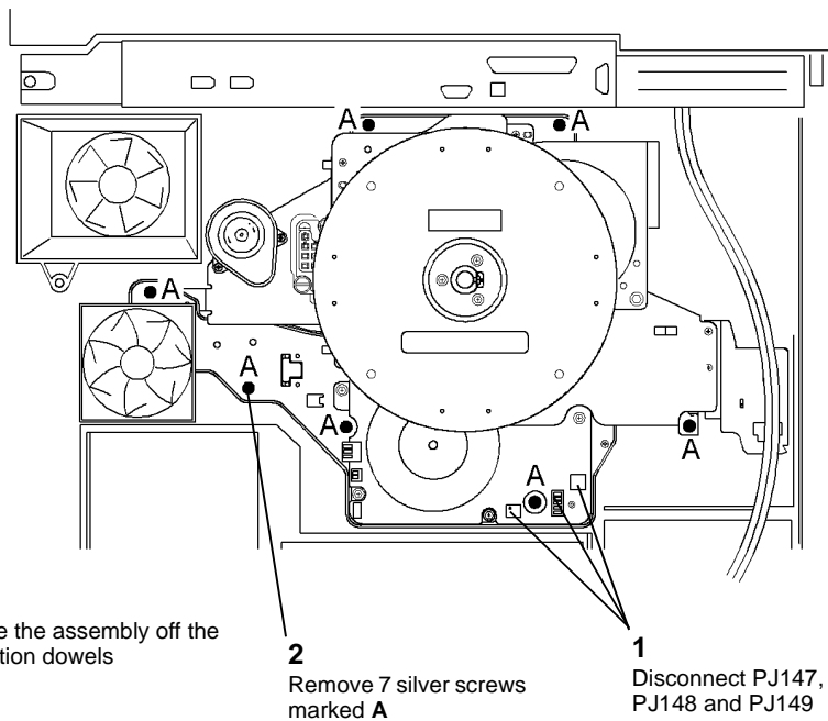
Figure 6 Main drive module
