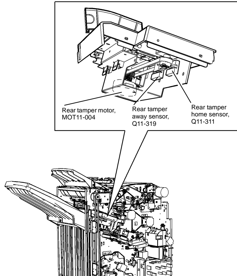
Figure 1 Component location
