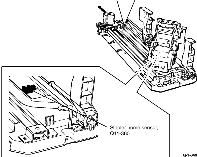
Figure 2 Component location
