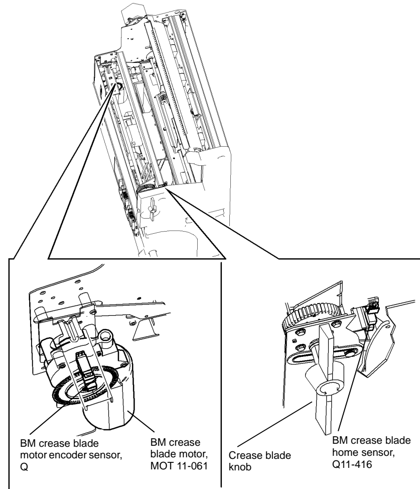
Figure 1 Component location
