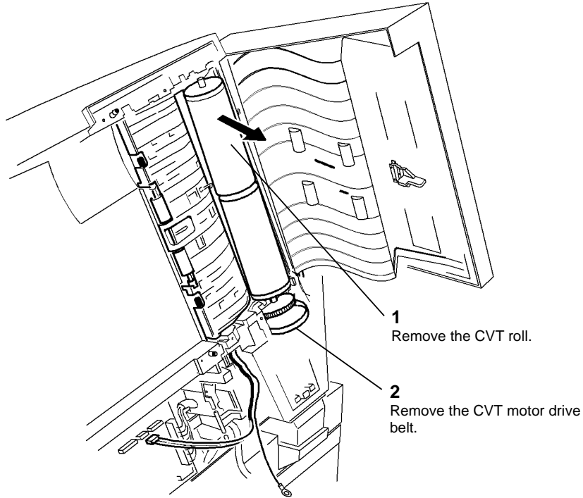
Figure 3 CVT roll
