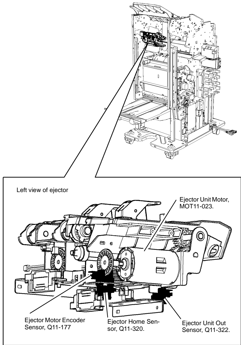
Figure 1 Component location
