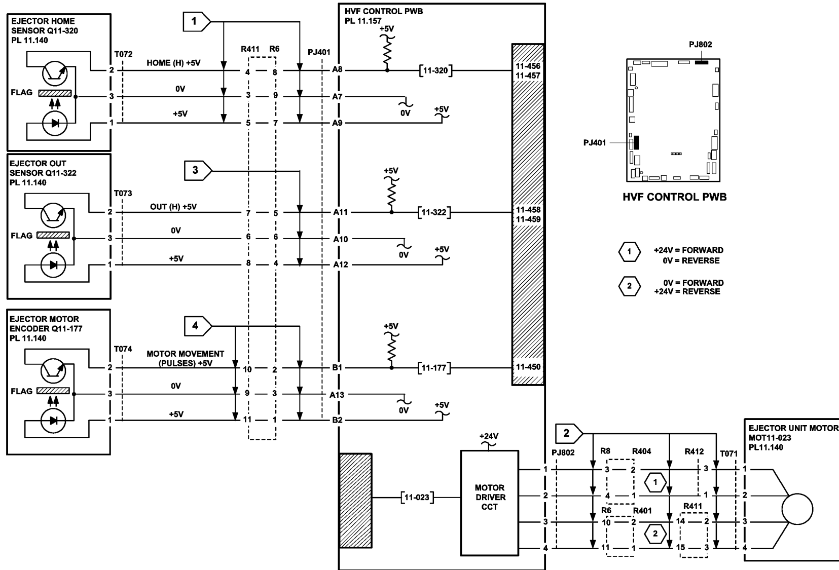
Figure 2 Circuit diagram
