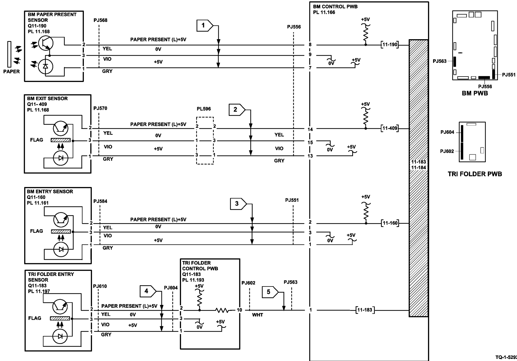
Figure 4 Circuit diagram
