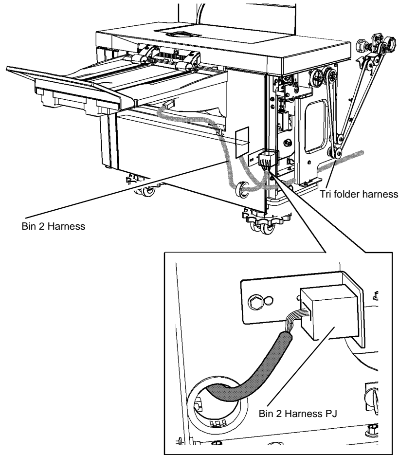
Figure 1 Harness removal
