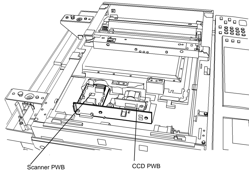
Figure 2 Component location
