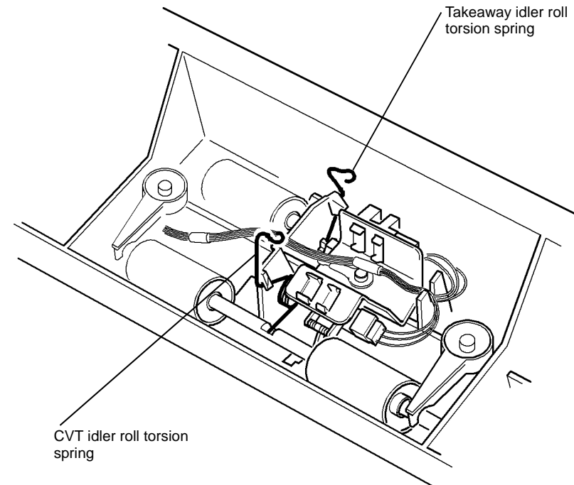
Figure 2 Torsion springs
