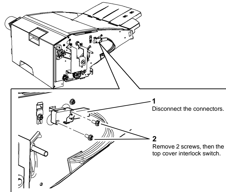
Figure 1 Switch removal
