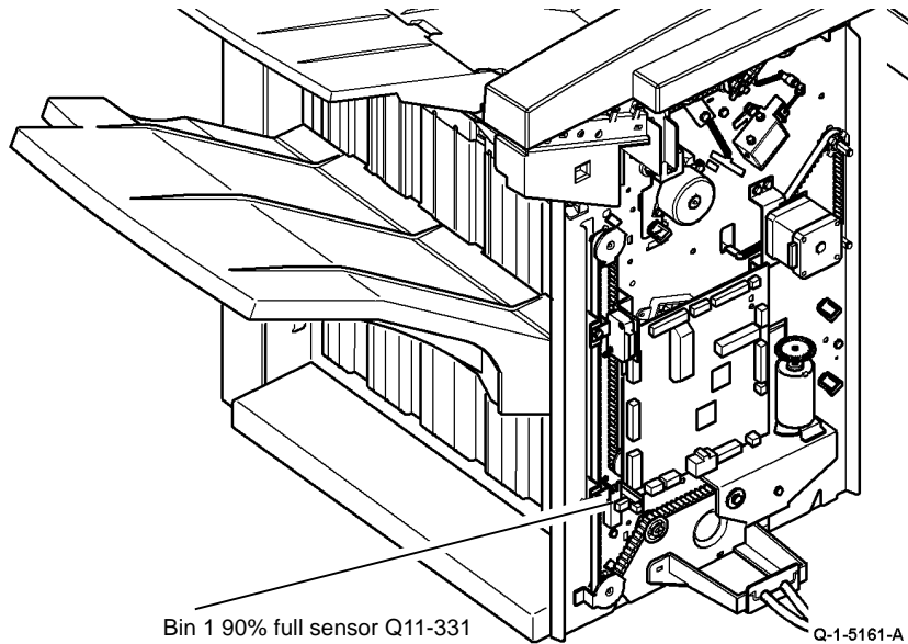
Figure 1 Component location
