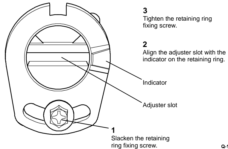
Figure 1 Initial calibration
