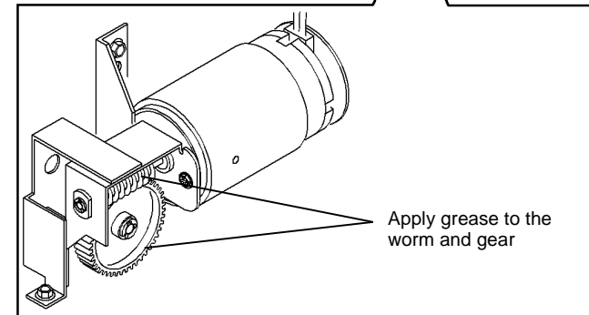
Figure 7 Worm and gear lubrication
