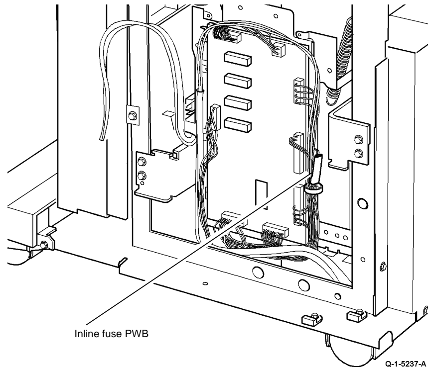
Figure 2 Component location
