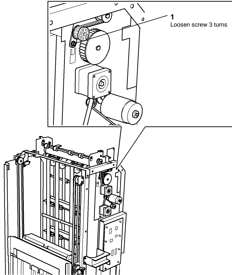
Figure 2 Belt tensioner
