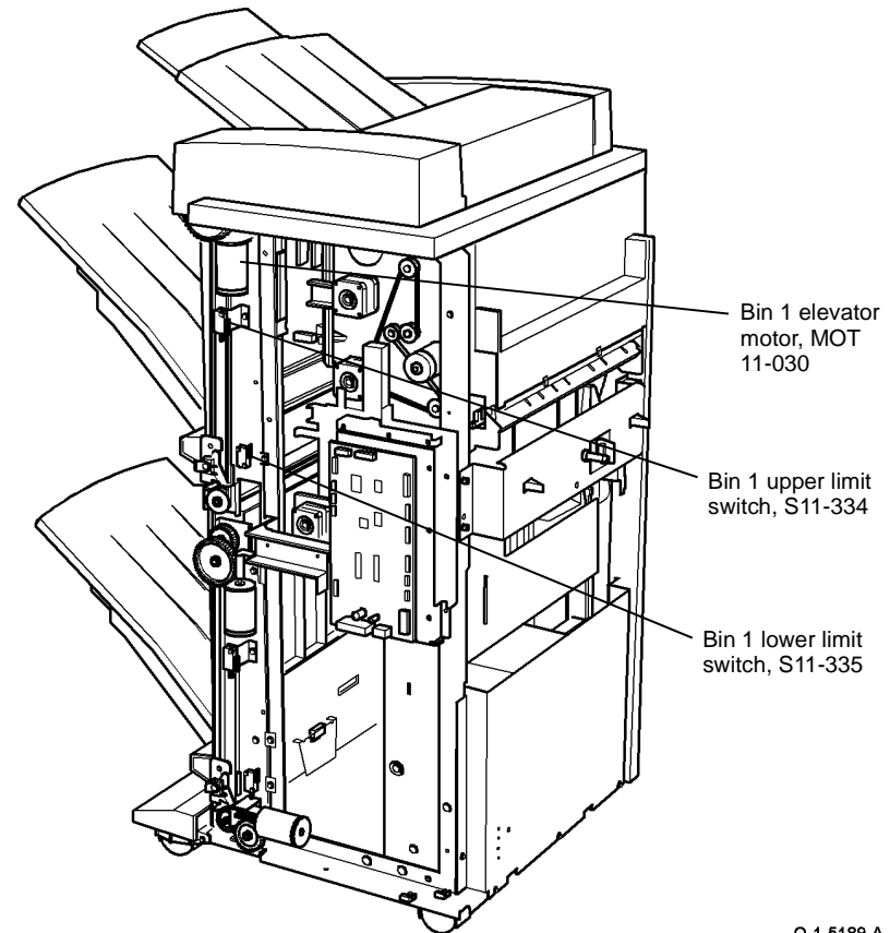
Figure 1 Component location
