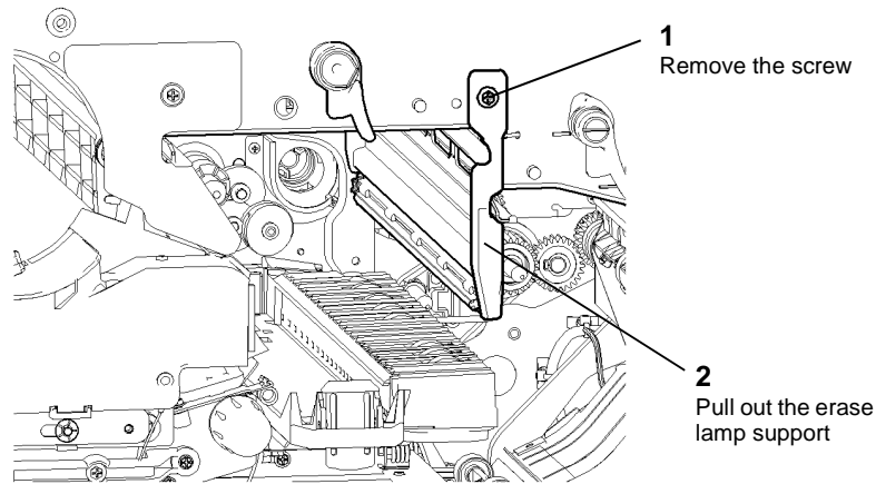
Figure 1 Erase lamp support
