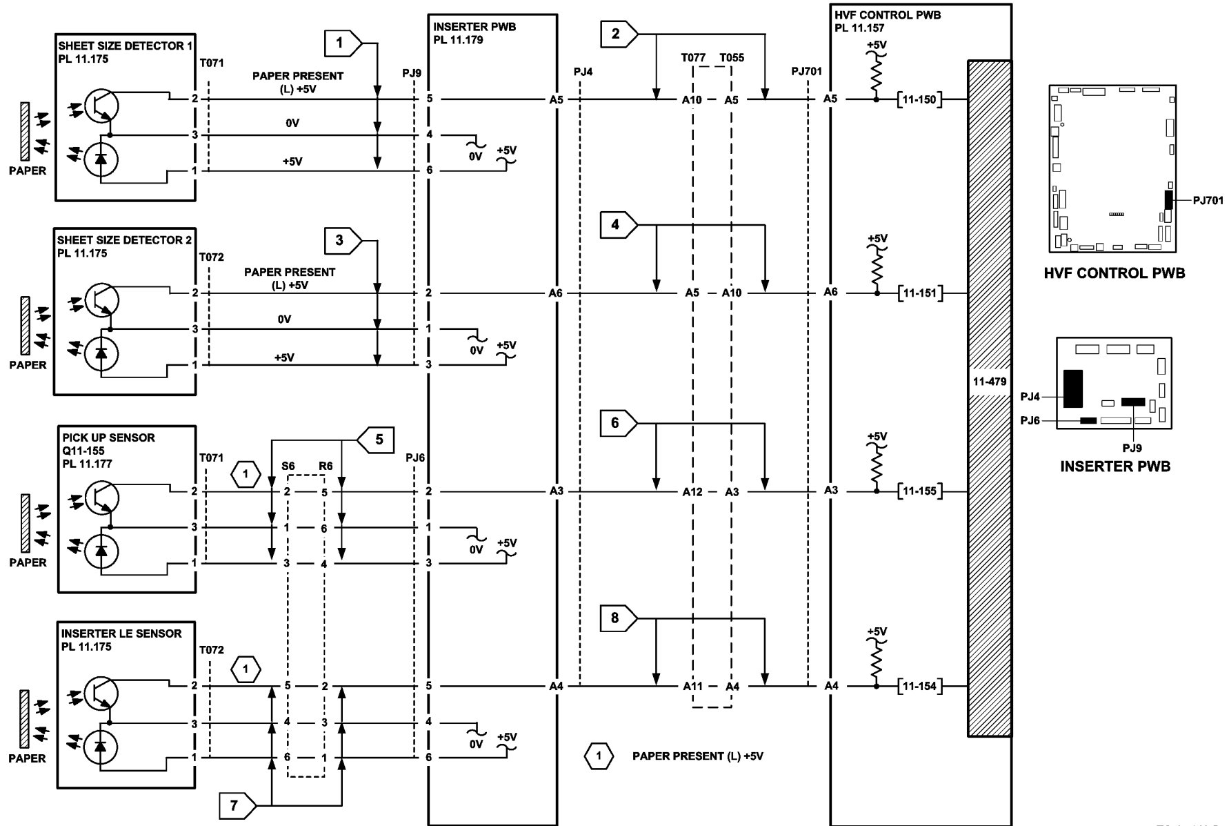
Figure 2 Circuit diagram
