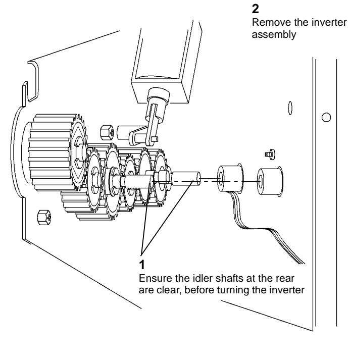
Figure 5 Remove Inverter assembly
