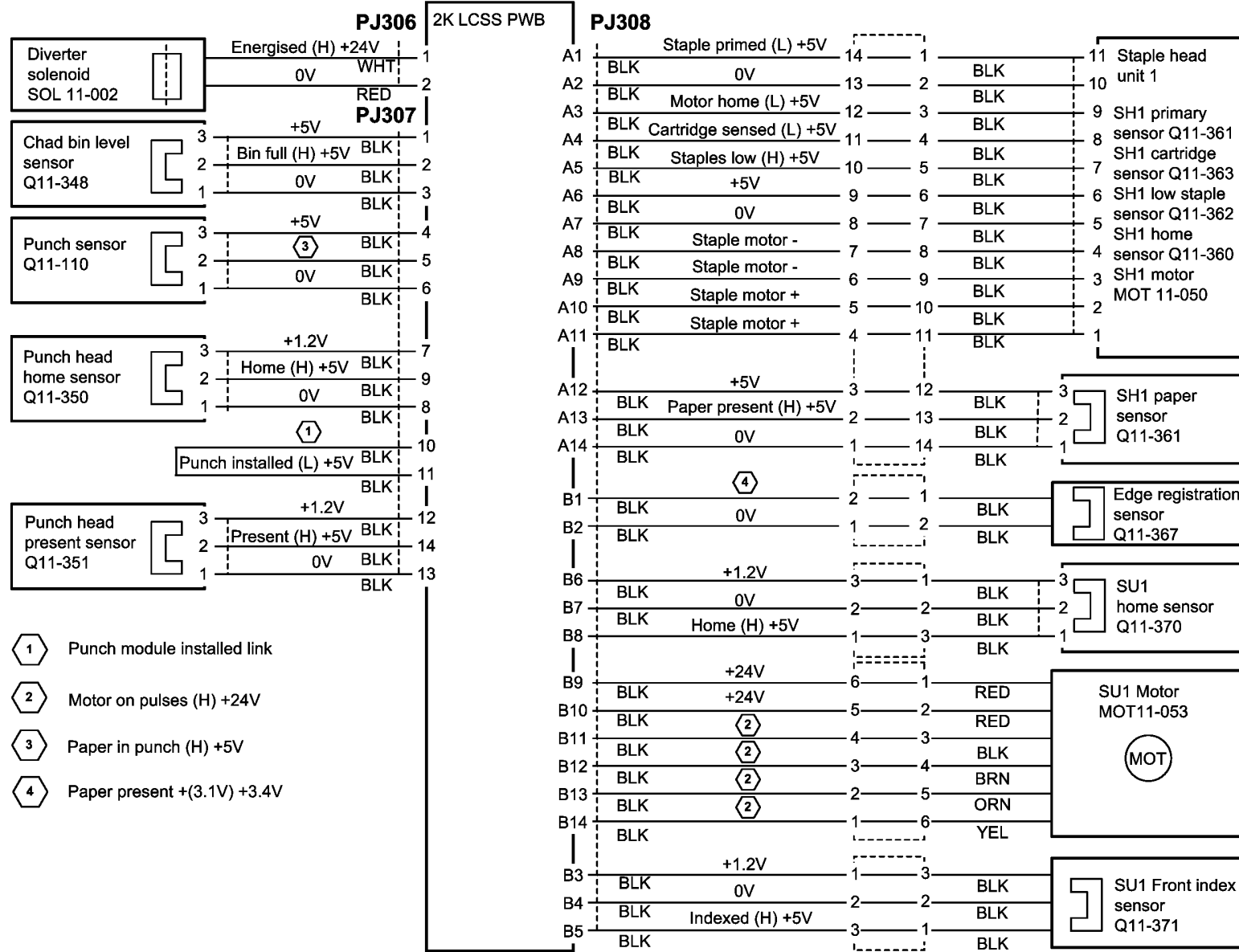
Figure 18 Wiring Diagram 18
