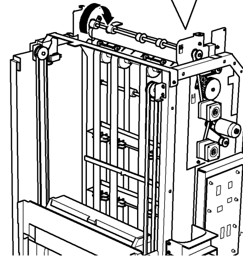
Figure 4 Belt drive
