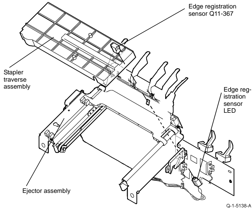
Figure 1 Component location
