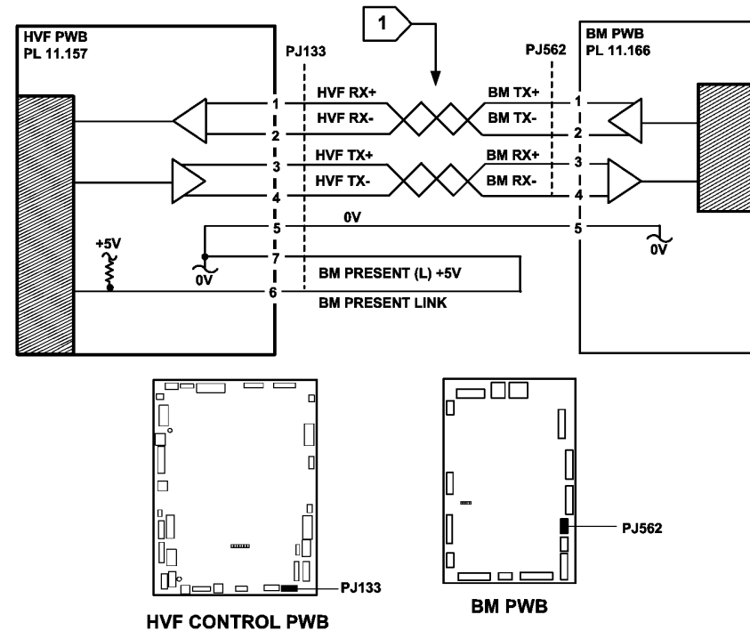
Figure 1 Circuit diagram
