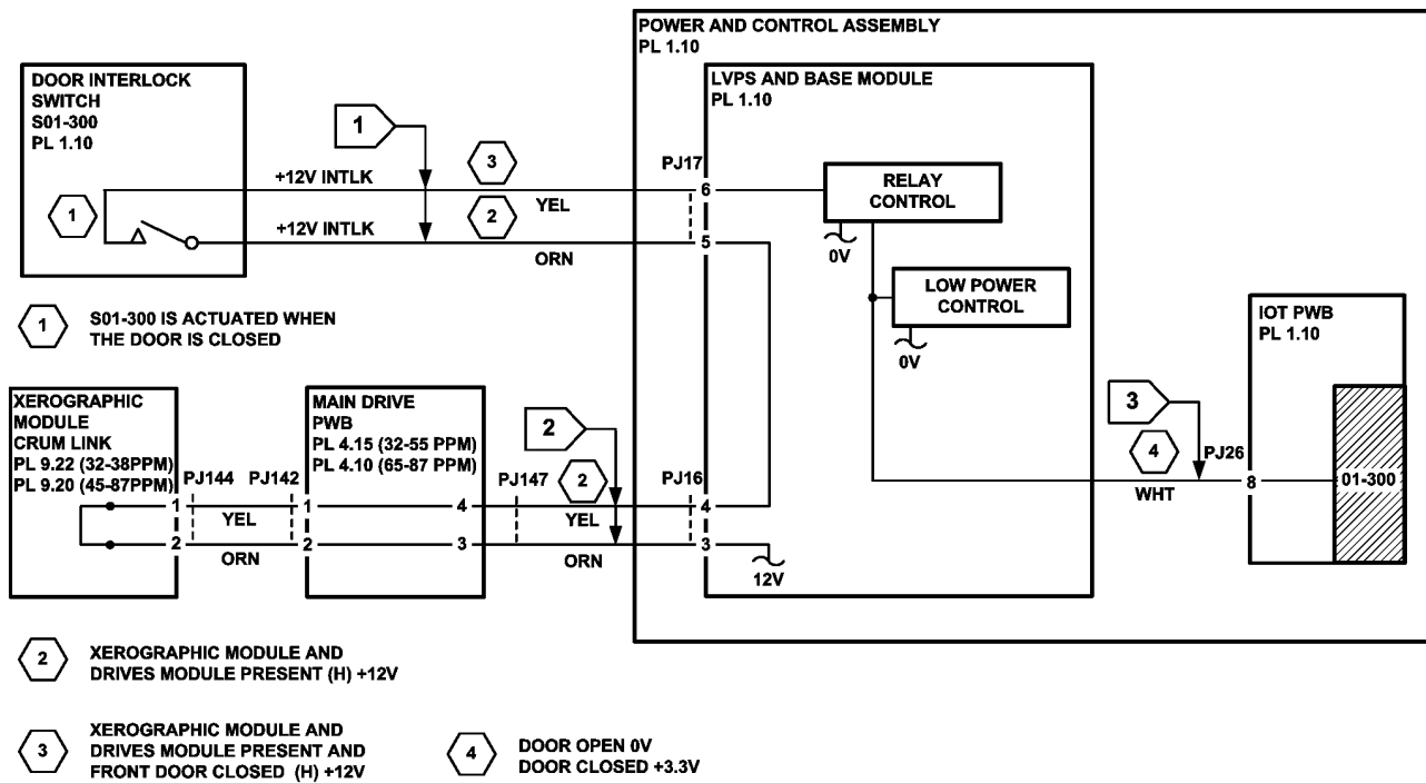
Figure 2 Circuit diagram
