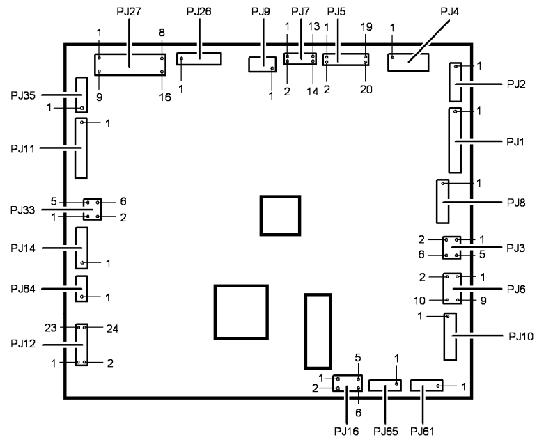
Figure 1 IOT PWB
