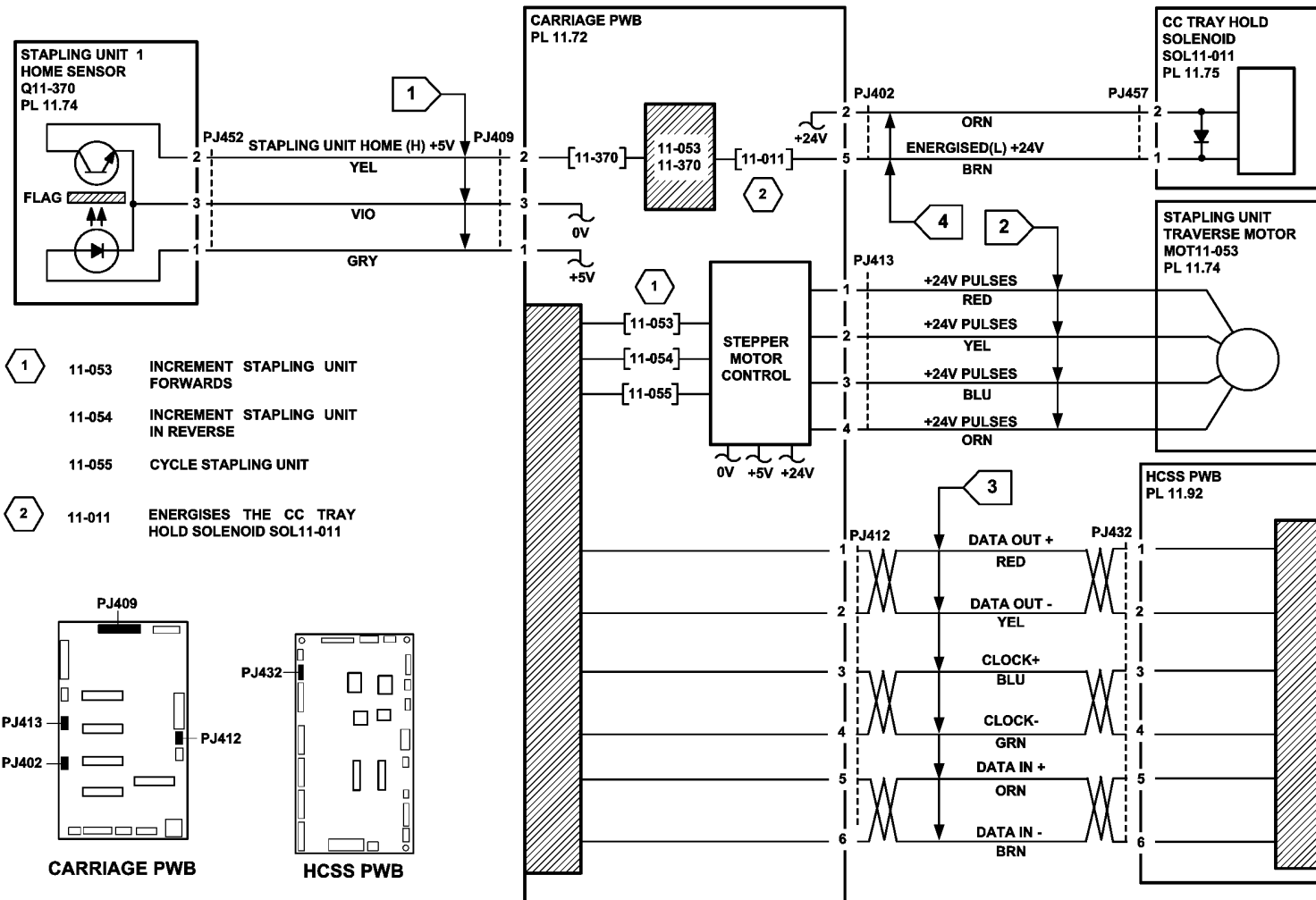
Figure 2 Circuit diagram
