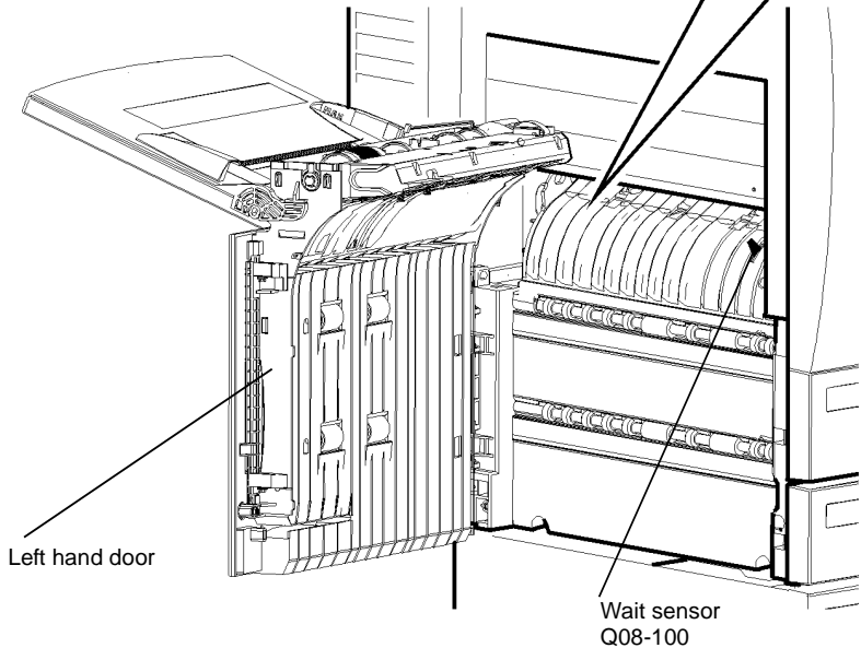
Figure 2 Component location
