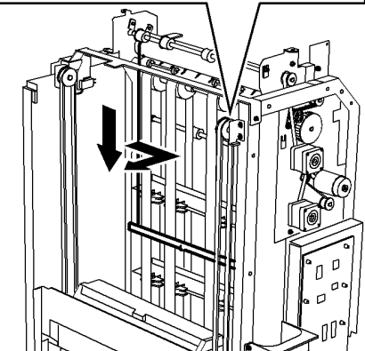
Figure 10 Spring tension
