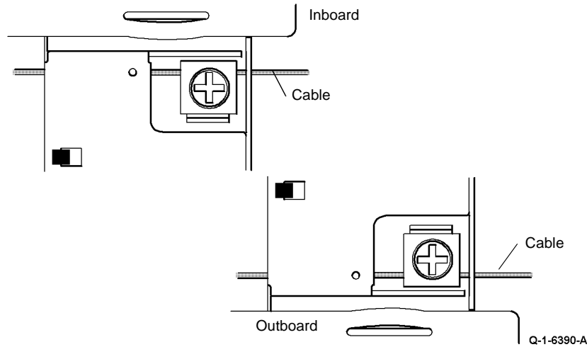
Figure 4 Cable clamps
