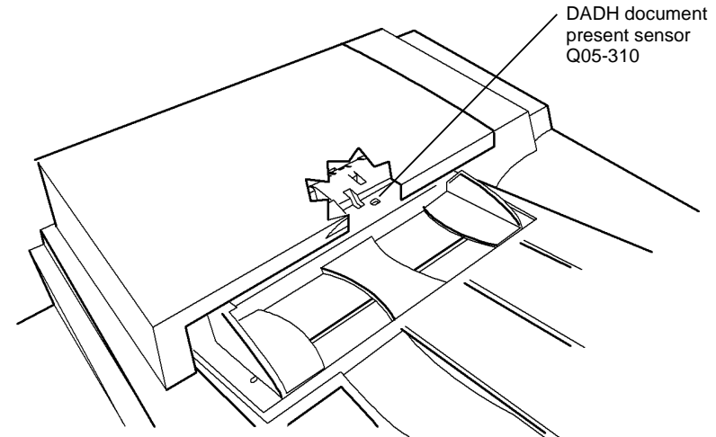
Figure 1 Component location
