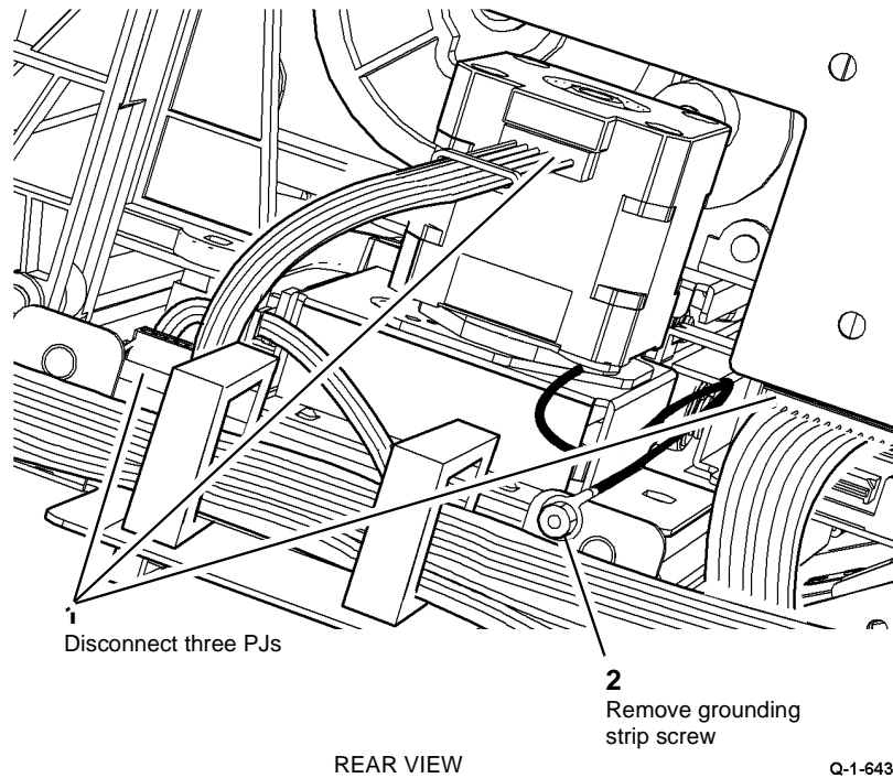
Figure 1 Disconnect PJs and remove screw
