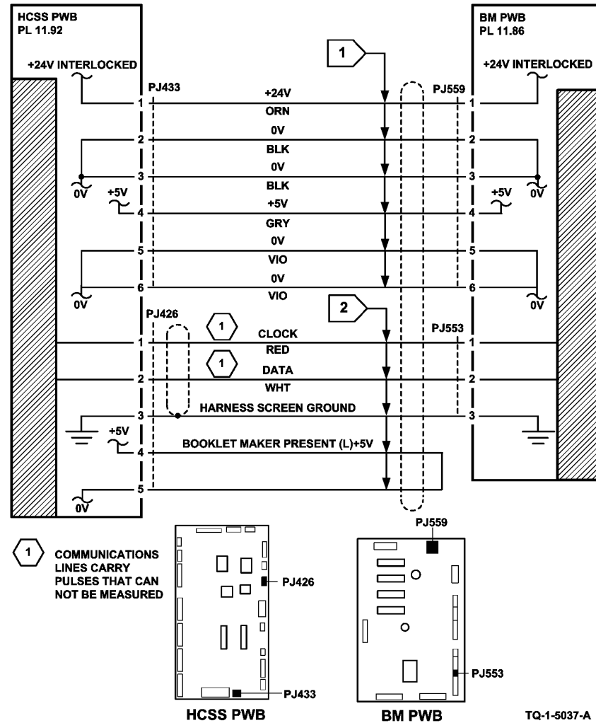
Figure 1 Circuit diagram
