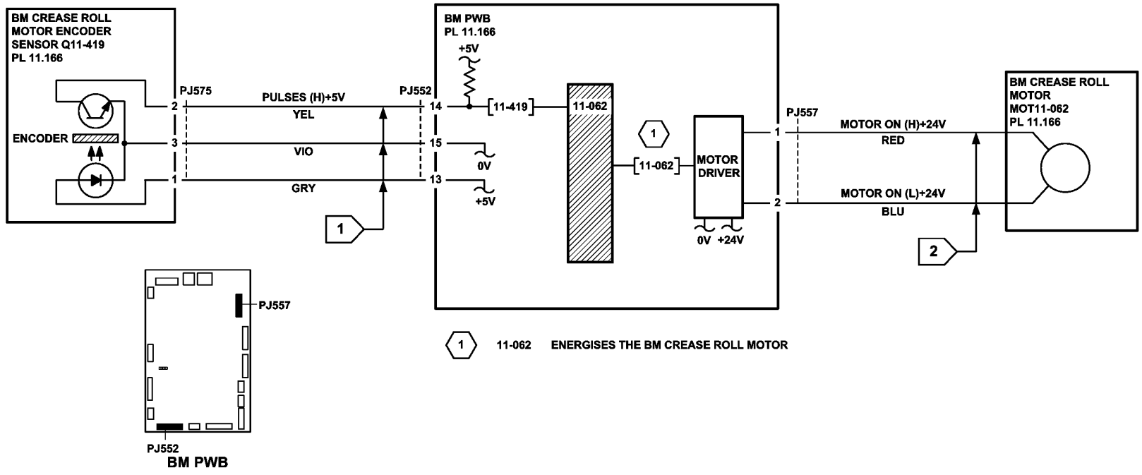
Figure 2 Circuit diagram
