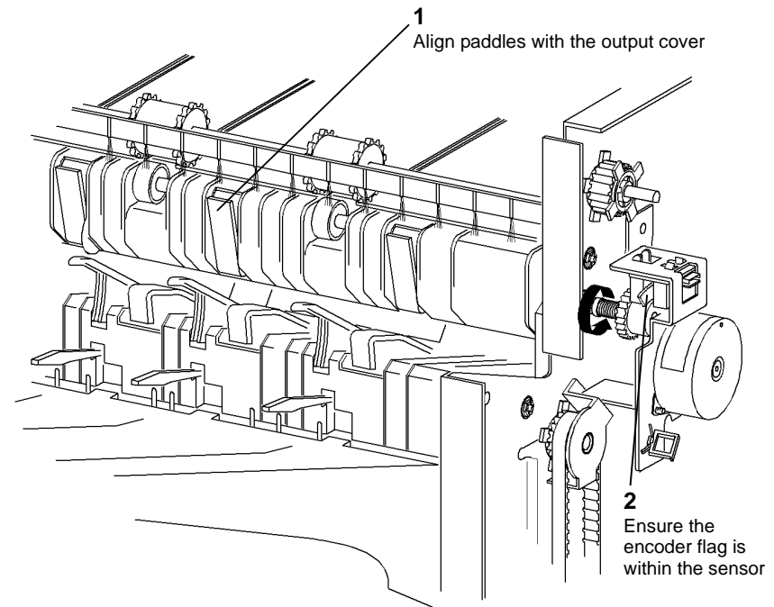
Figure 5 Paddle alignment
