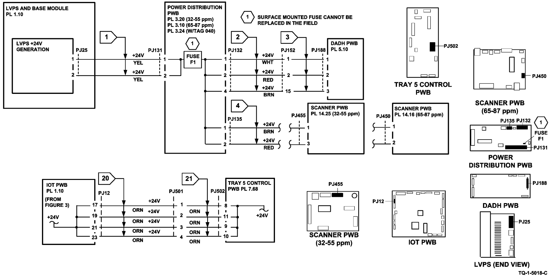
Figure 2 +24V distribution circuit diagram
