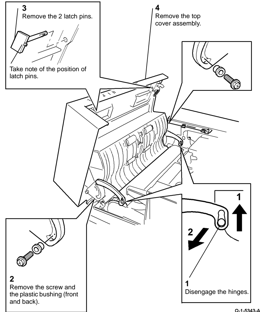
Figure 1 Top cover
