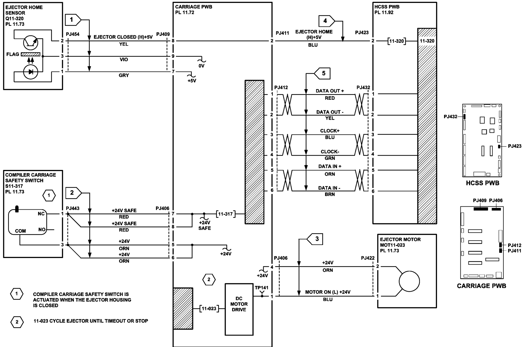
Figure 2 Circuit diagram
