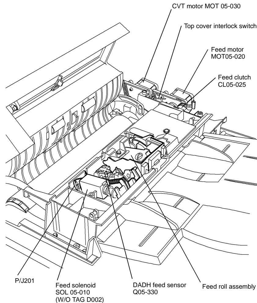
Figure 1 Component location W/OTAG D002
