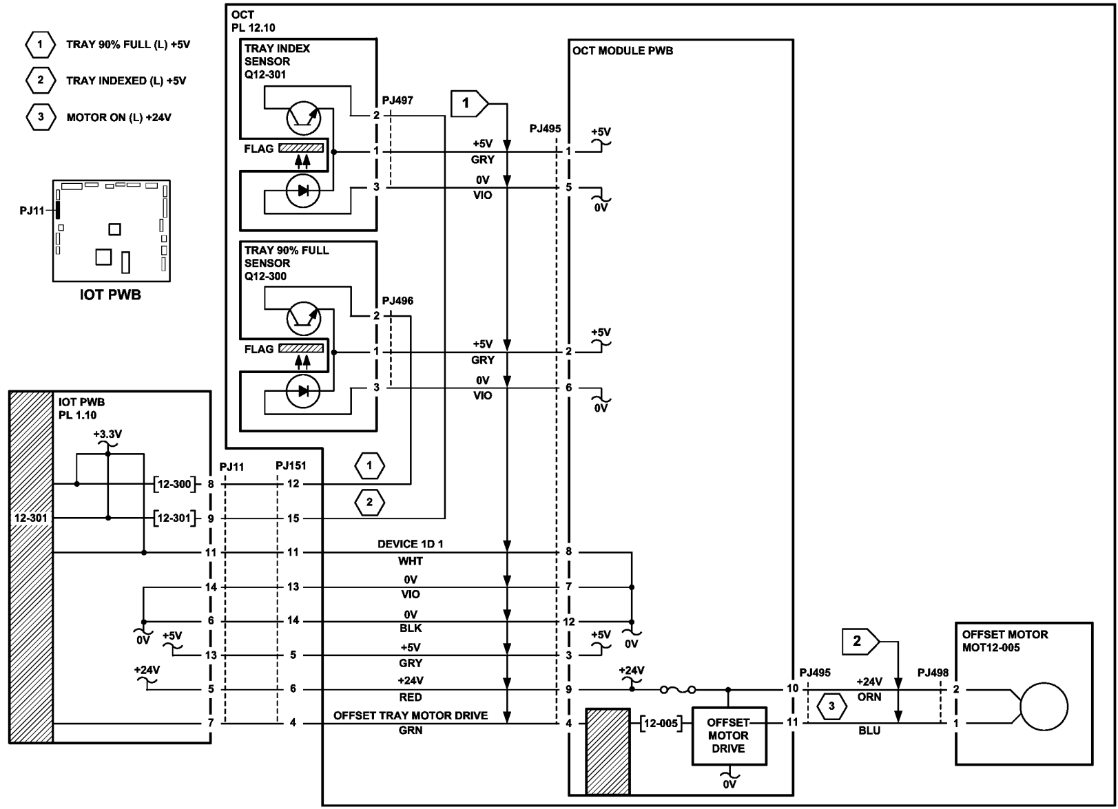
Figure 2 Circuit Diagram
