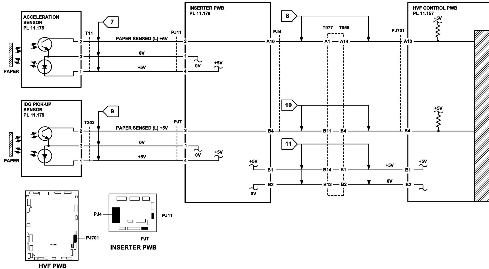
Figure 4 Circuit diagram
