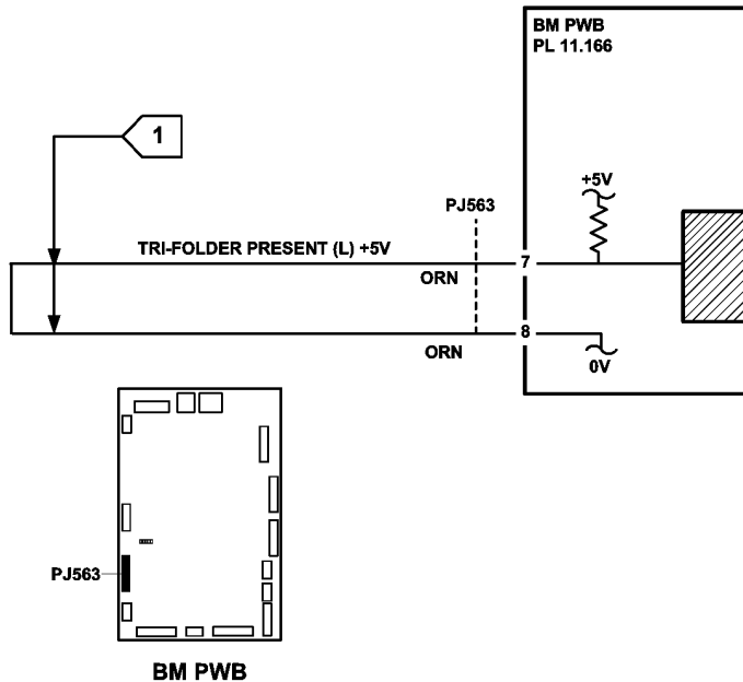
Figure 1 Circuit diagram
