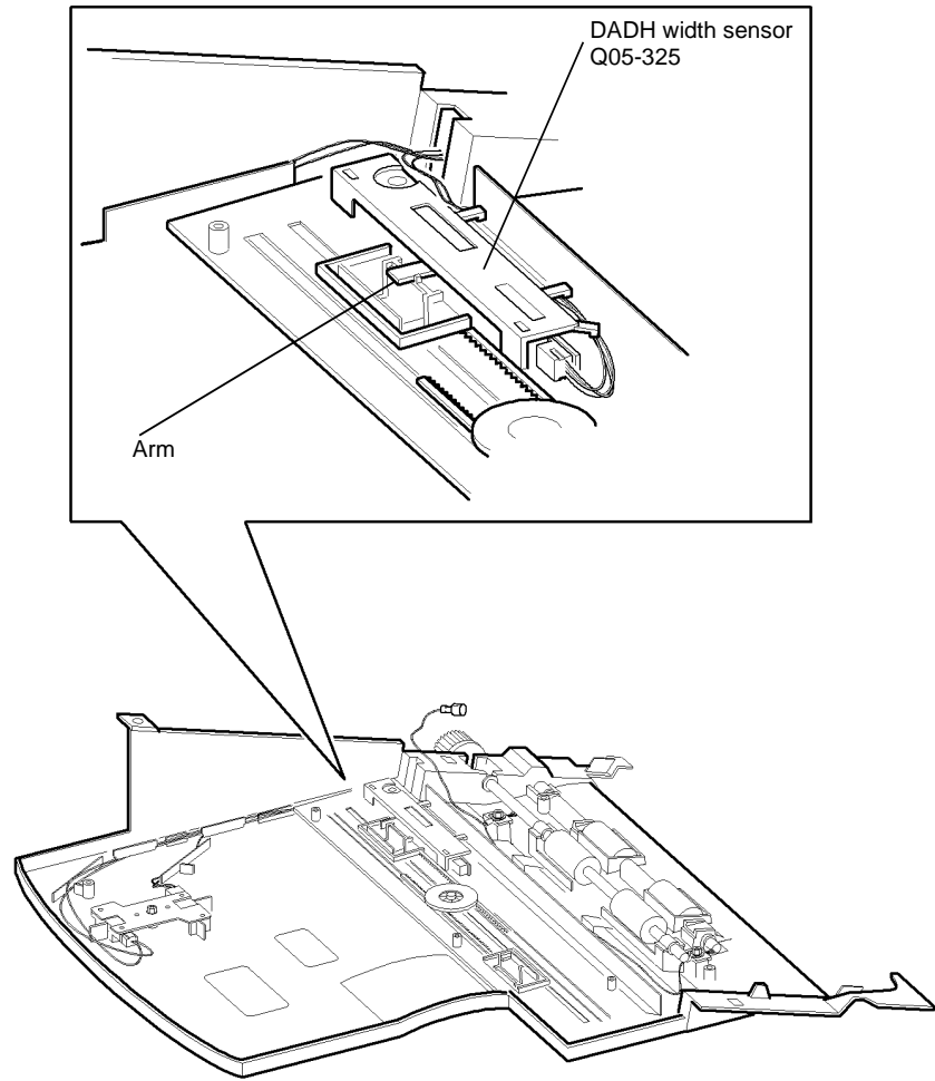
Figure 2 Component location
