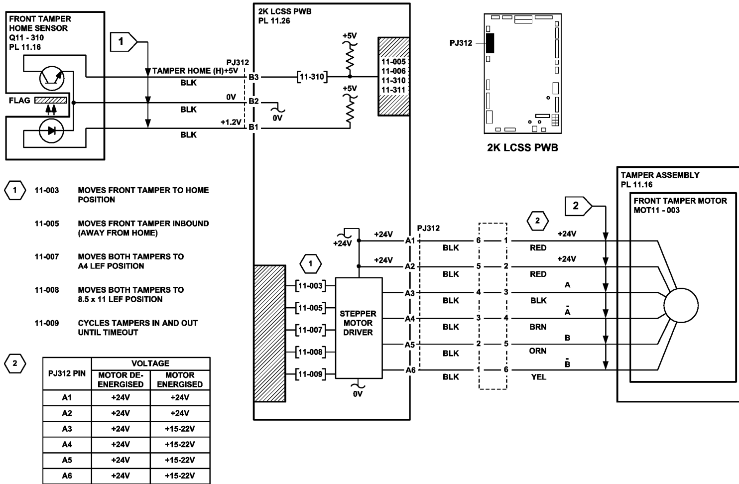
Figure 2 Circuit diagram
