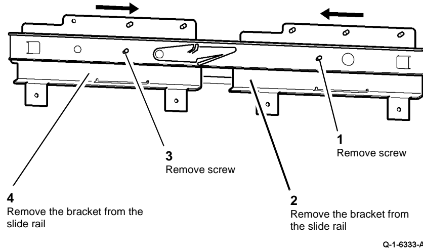
Figure 5 Remove the bracket from the slide rail
