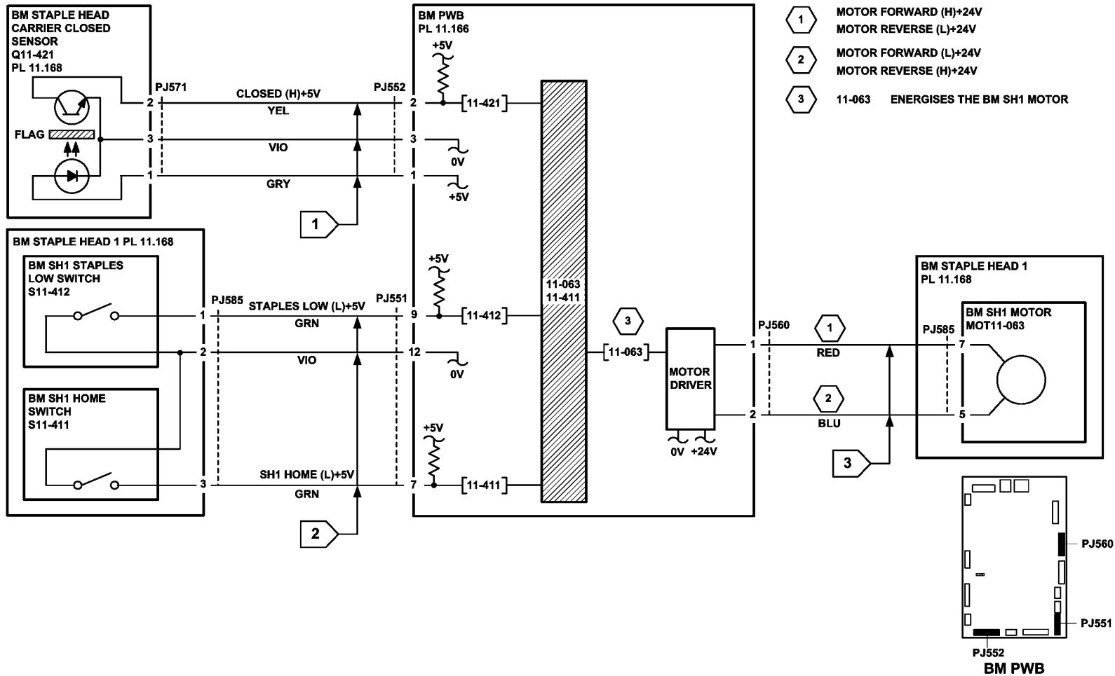
Figure 2 Circuit diagram
