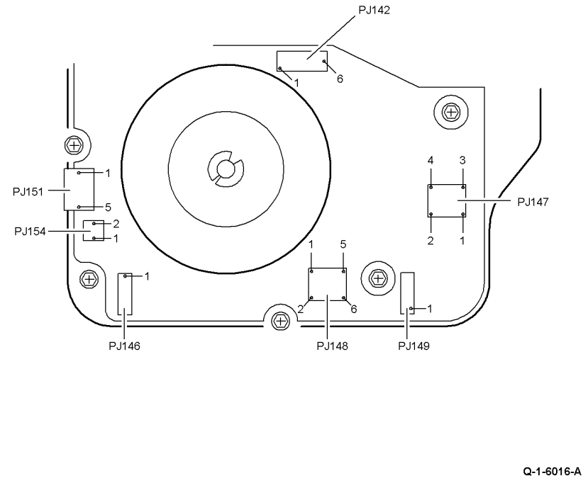
Figure 4 Main drive module
