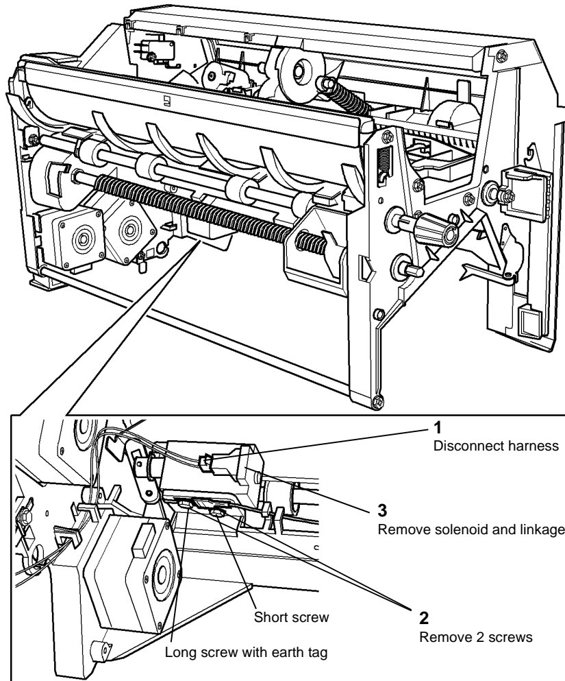
Figure 1 Solenoid removal
