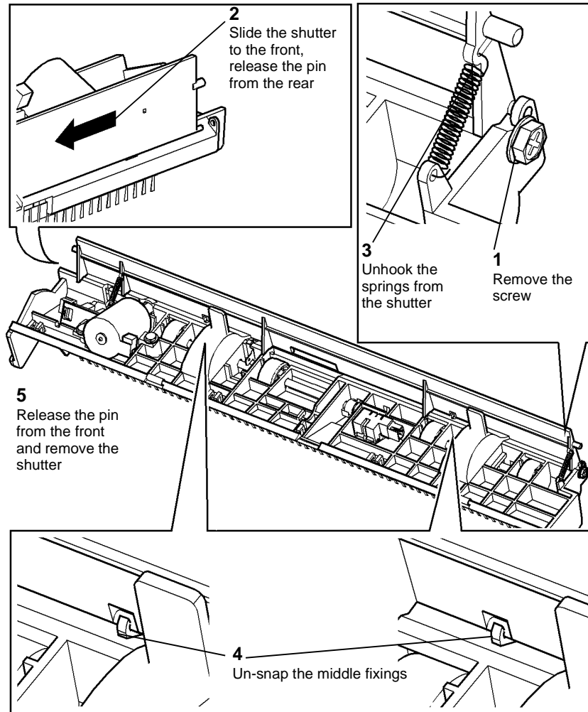
Figure 1 Shutter removal
