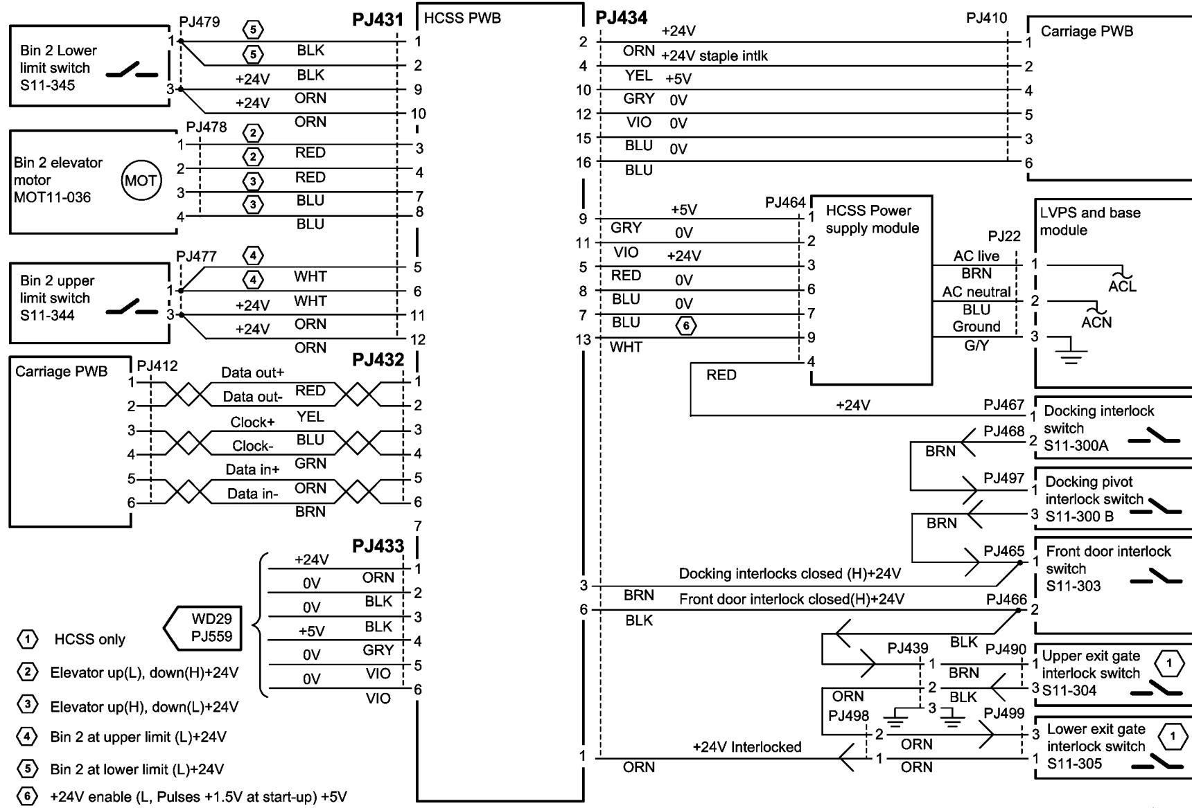
Figure 25 Wiring Diagram 25
