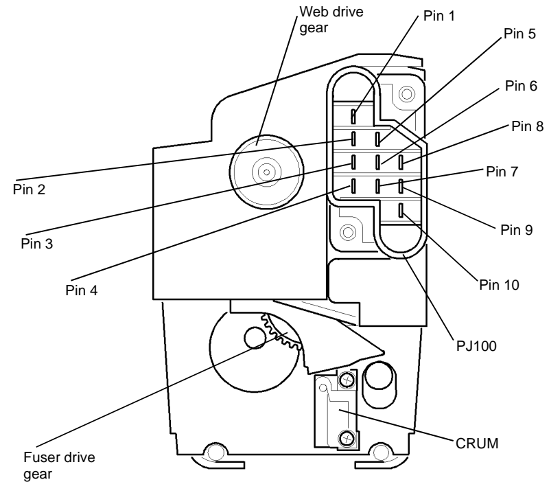
Figure 1 Component location
