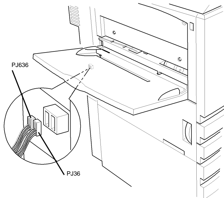
Figure 40 PJ36 and PJ636
