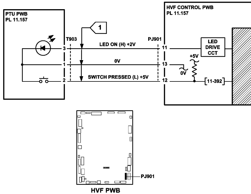
Figure 2 Circuit diagram
