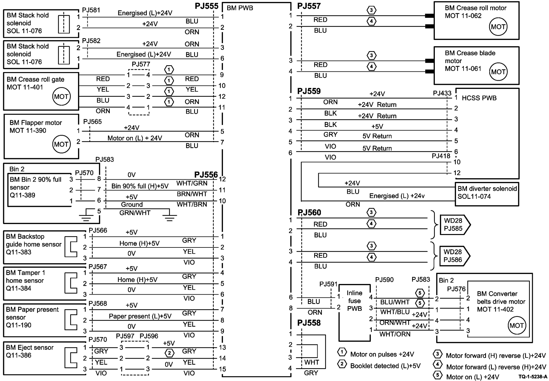
Figure 29 Wiring Diagram 29
