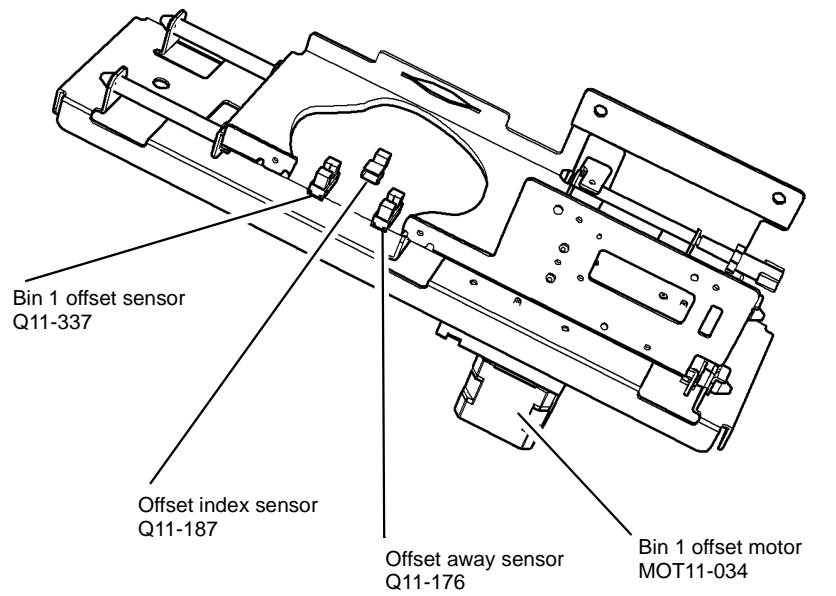
Figure 1 Component location
