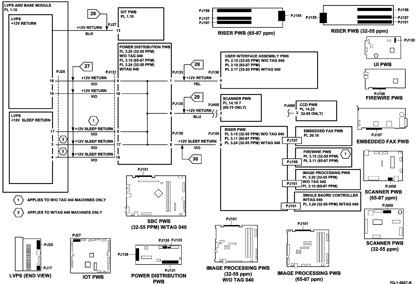
Figure 6 12V Return
