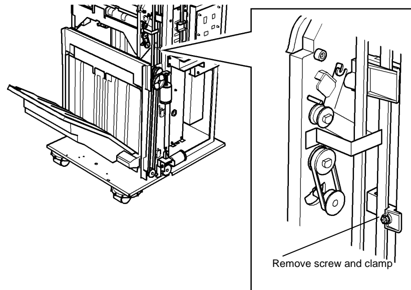
Figure 5 Clamp removal
