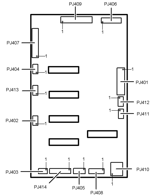
Figure 25 Carriage PWB
