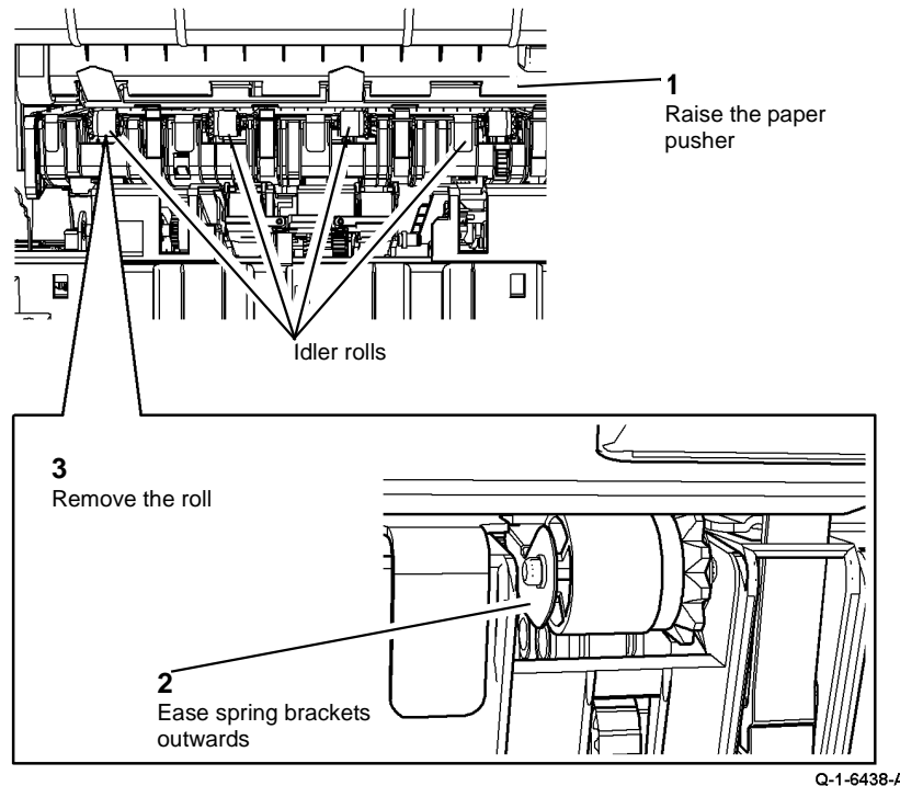
Figure 1 Paper pusher and idler rolls.
