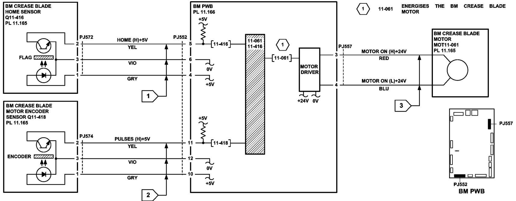
Figure 2 Circuit diagram
