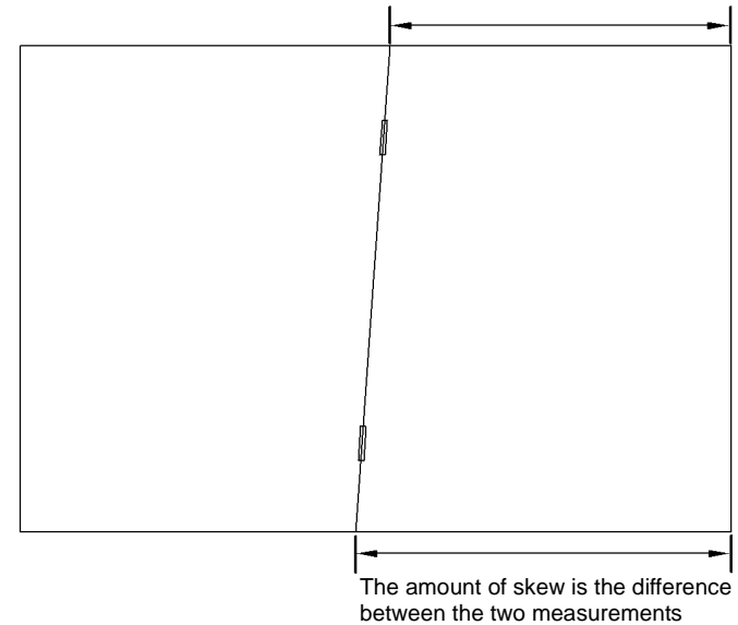
Figure 3 Booklet skew
