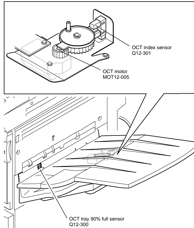
Figure 1 Component location
