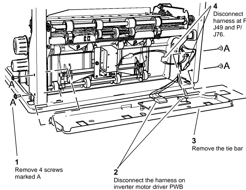
Figure 3 Tie bar
