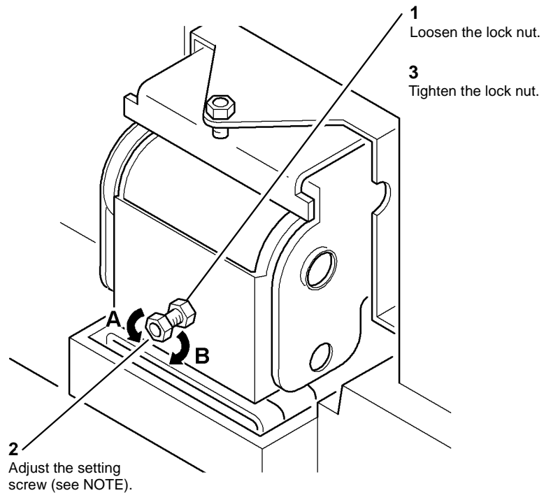
Figure 1 Skew adjustment
