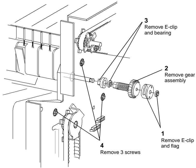
Figure 2 Rear preparation
