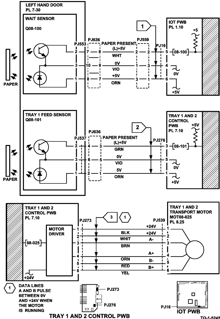
Figure 2 Circuit diagram
