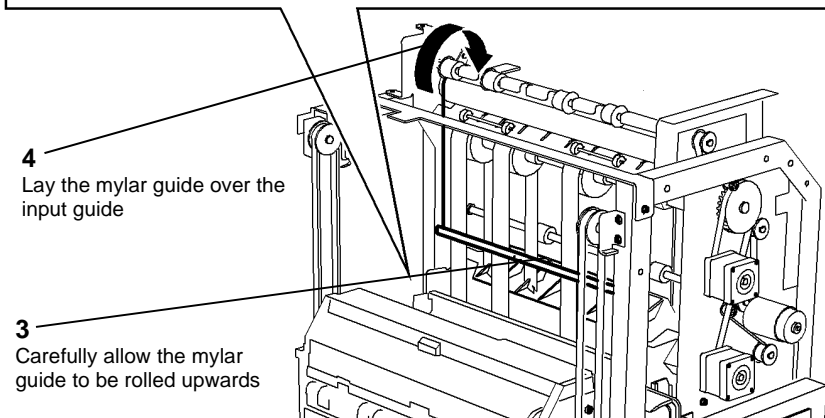
Figure 1 Mylar guide
