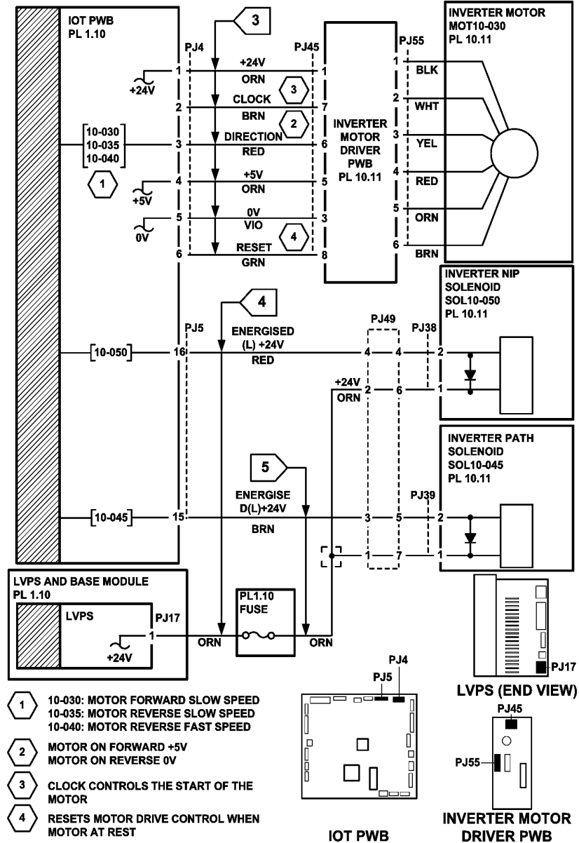
Figure 3 Circuit diagram
