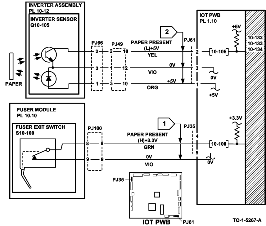
Figure 3 Circuit diagram
