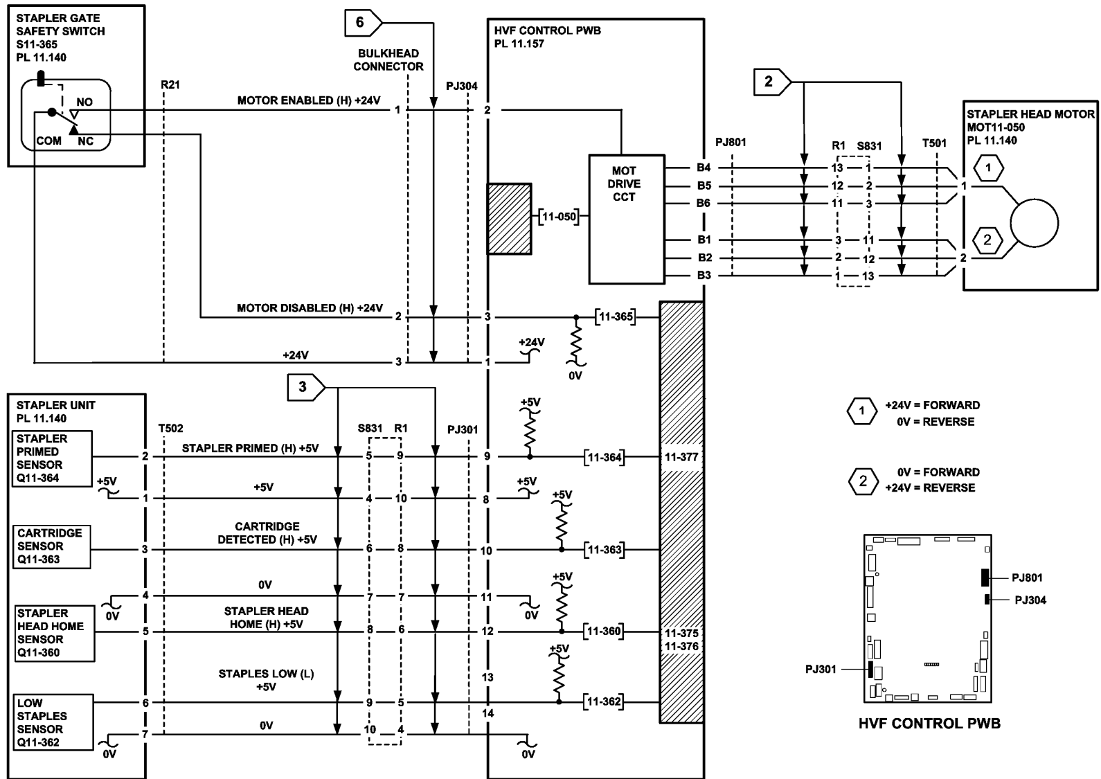
Figure 3 Circuit diagram
