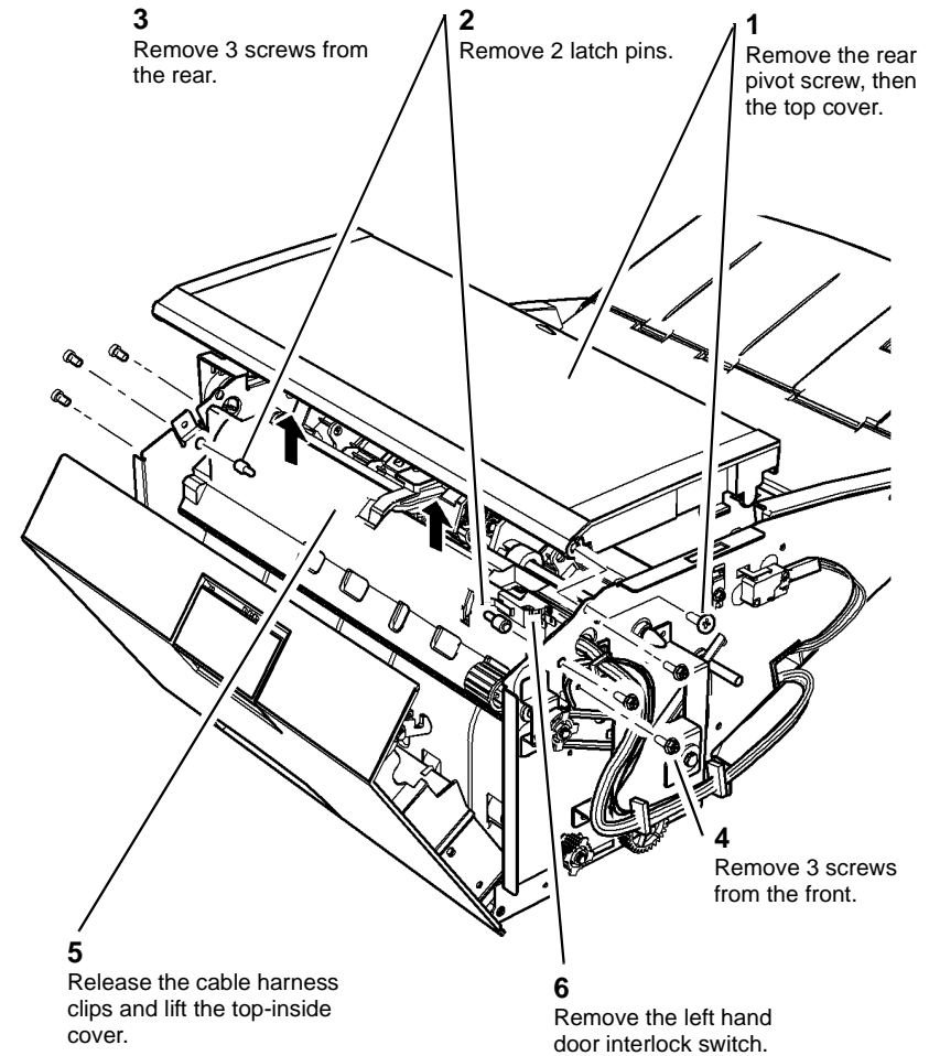
Figure 1 Switch removal
