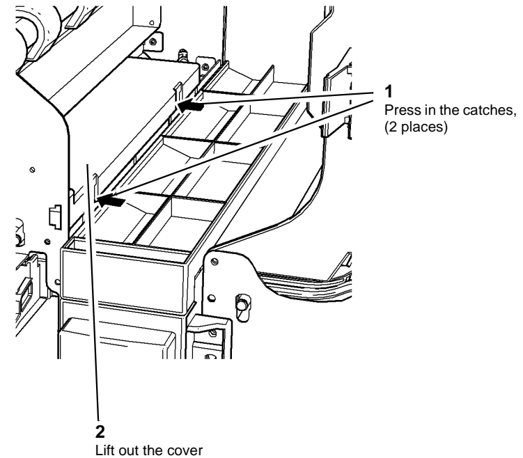
Figure 1 Cover removal.
