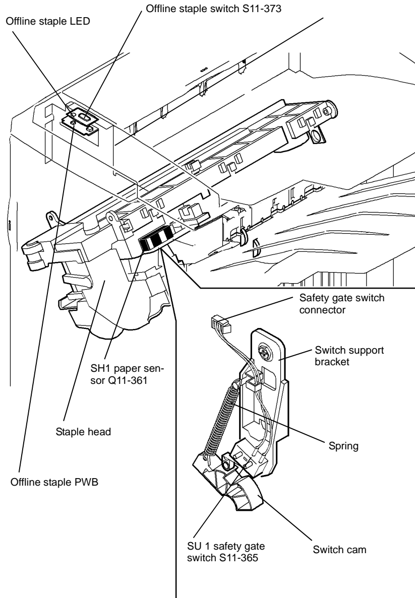
Figure 2 Component location
