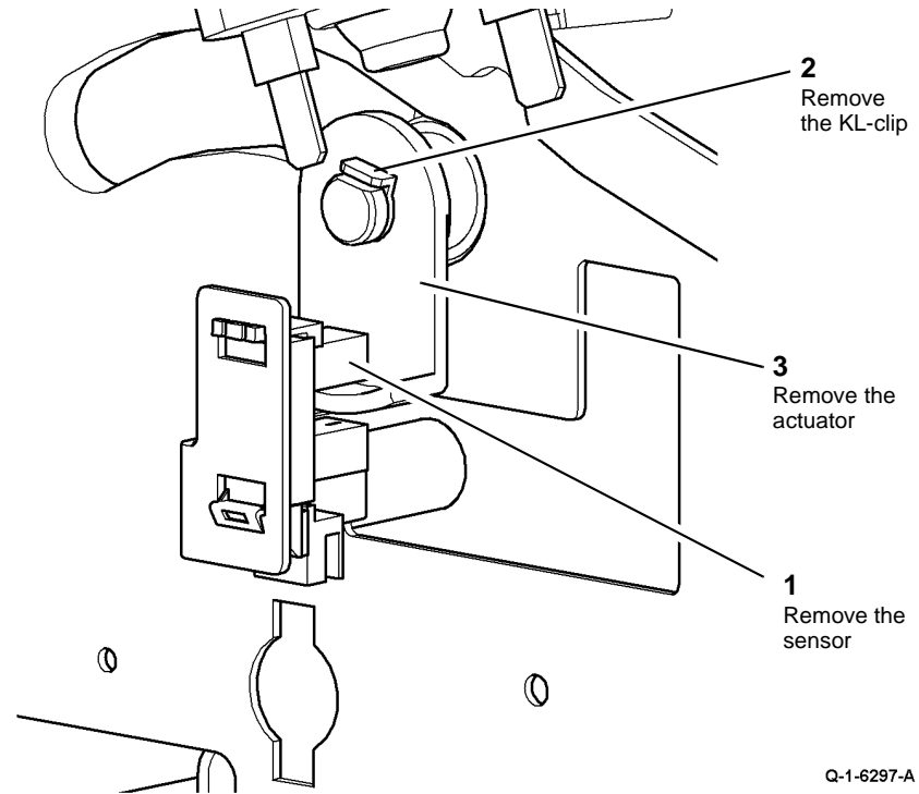
Figure 1 Actuator removal
