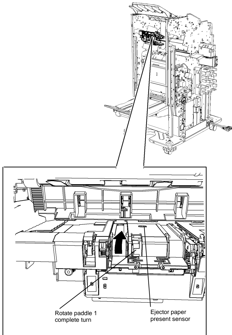
Figure 3 Component location
