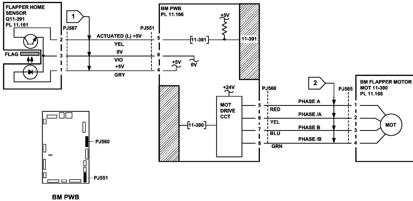
Figure 2 Circuit diagram
