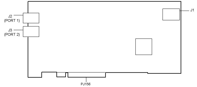
Figure 27 Firewire PWB
