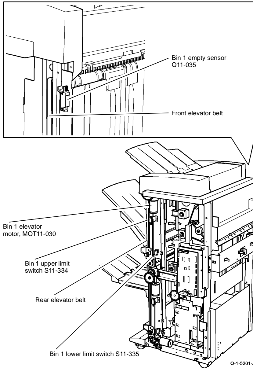
Figure 1 Component location
