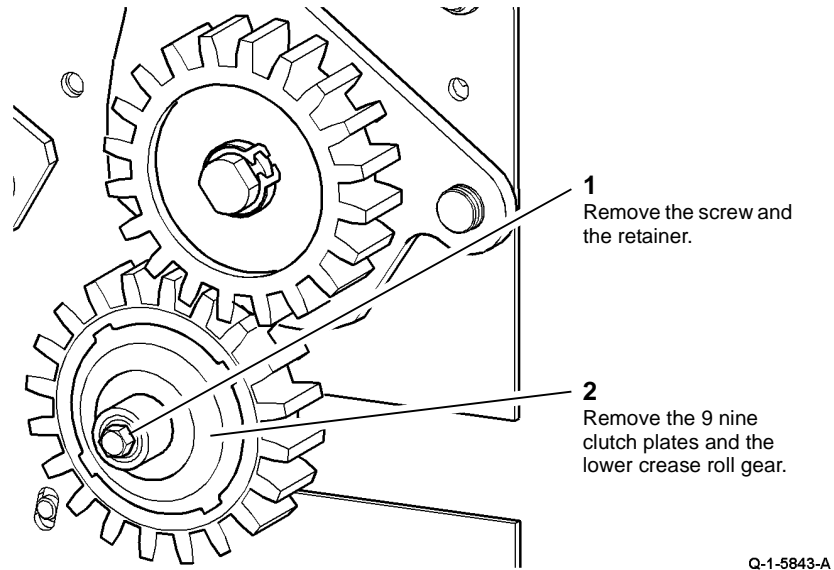
Figure 5 Clutch removal
