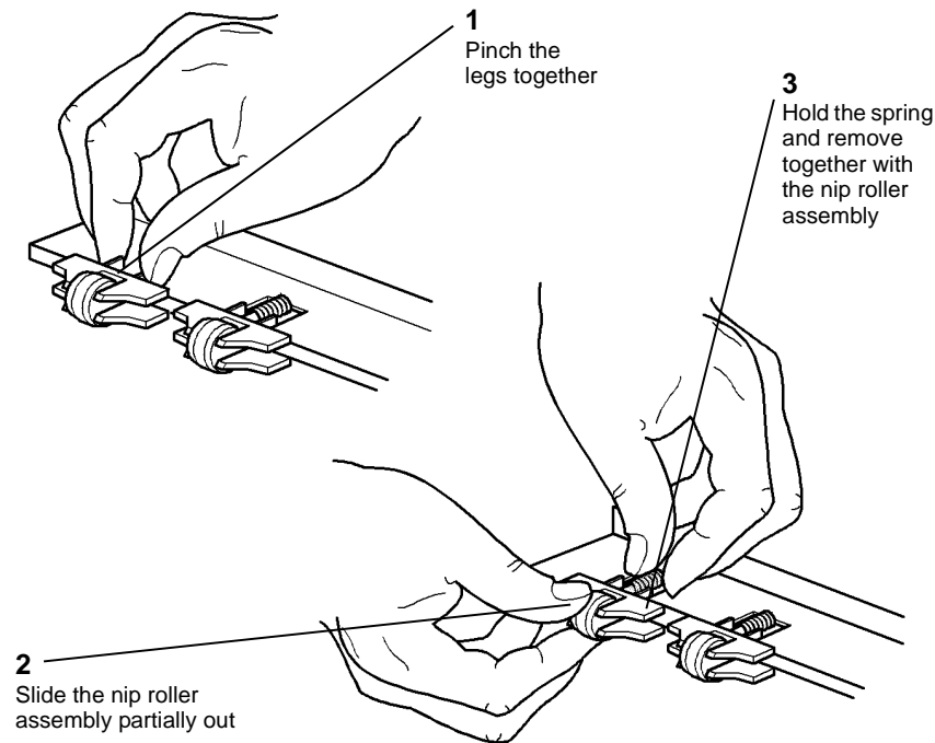
Figure 1 Roller removal
