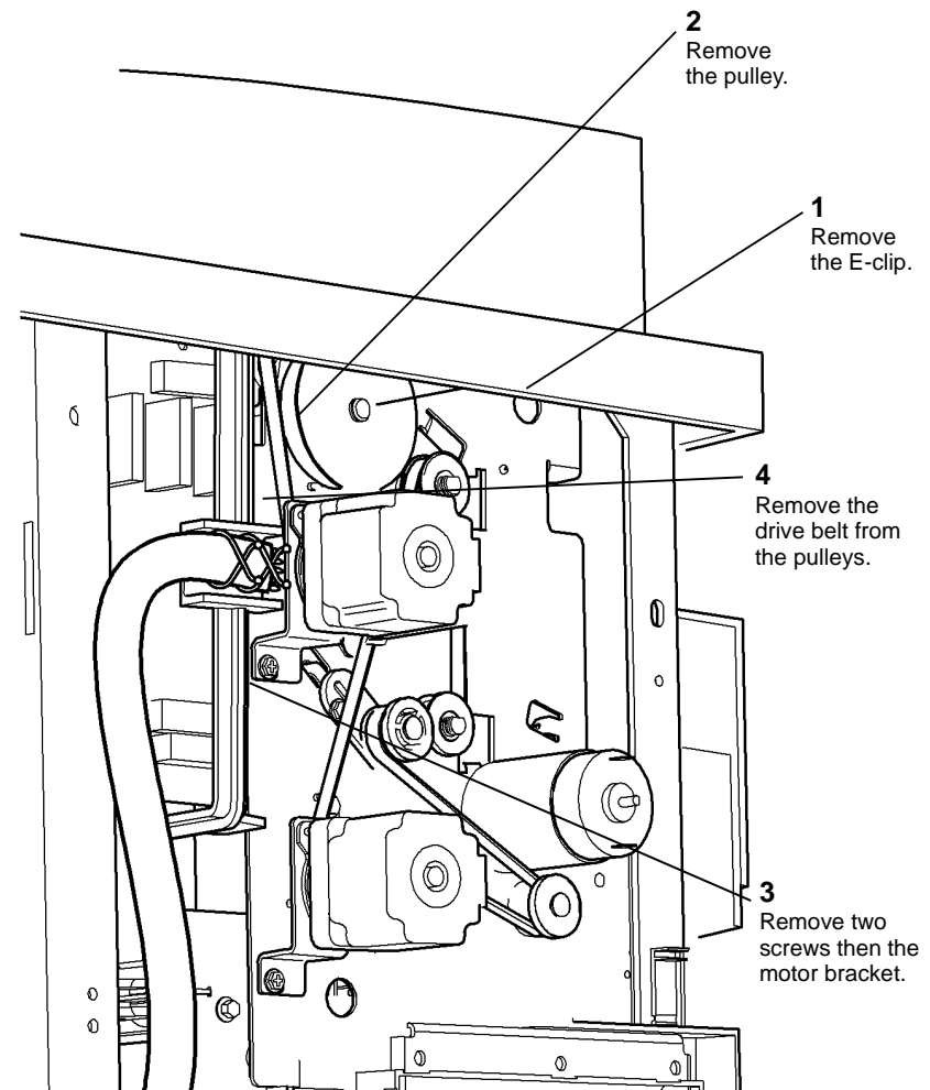
Figure 2 Belt removal
