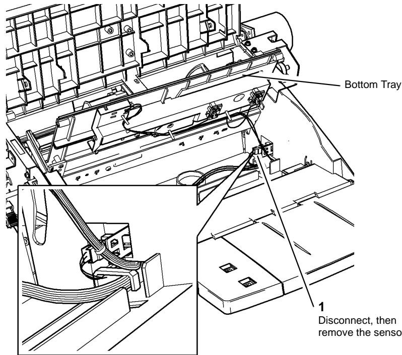
Figure 1 Sensor removal
