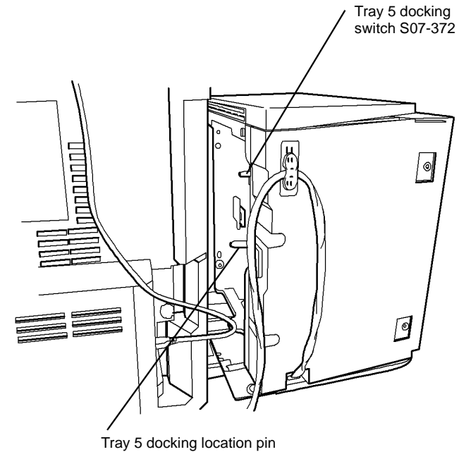
Figure 1 Component location
