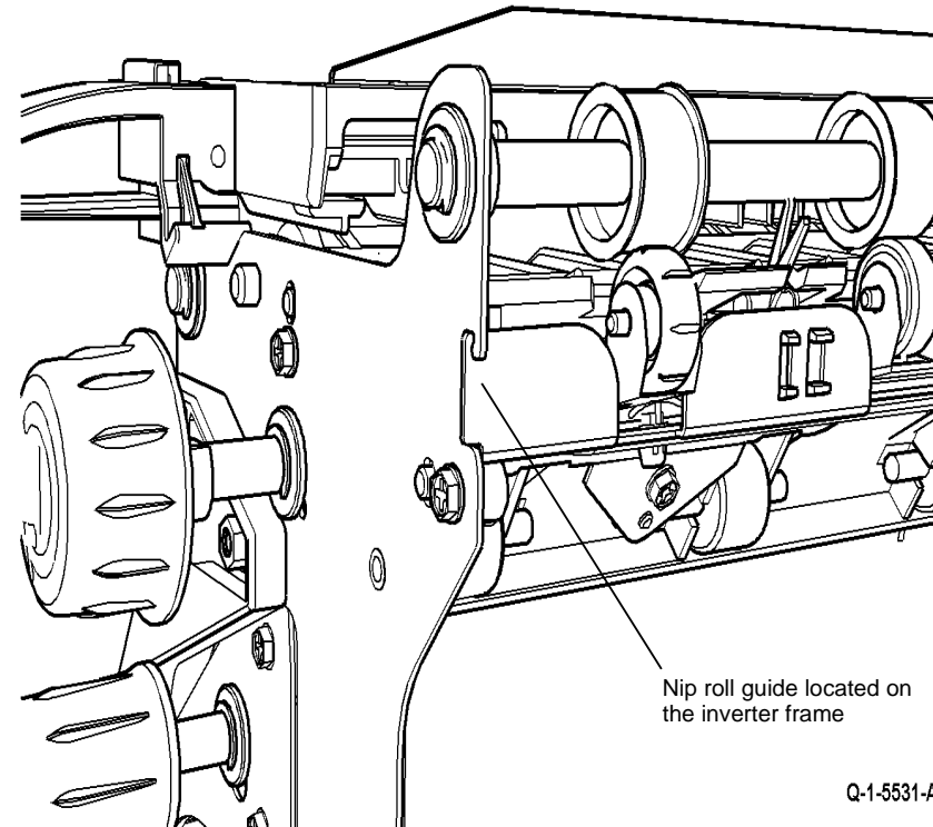
Figure 7 Nip roll guide
