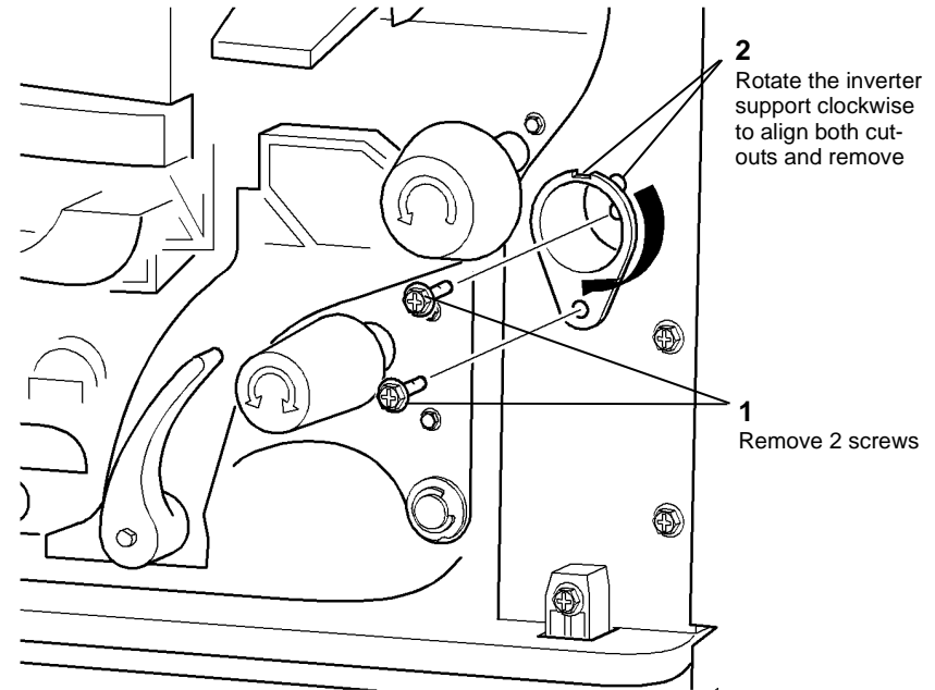
Figure 1 Inverter support
