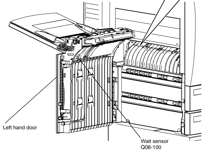
Figure 2 Component location
