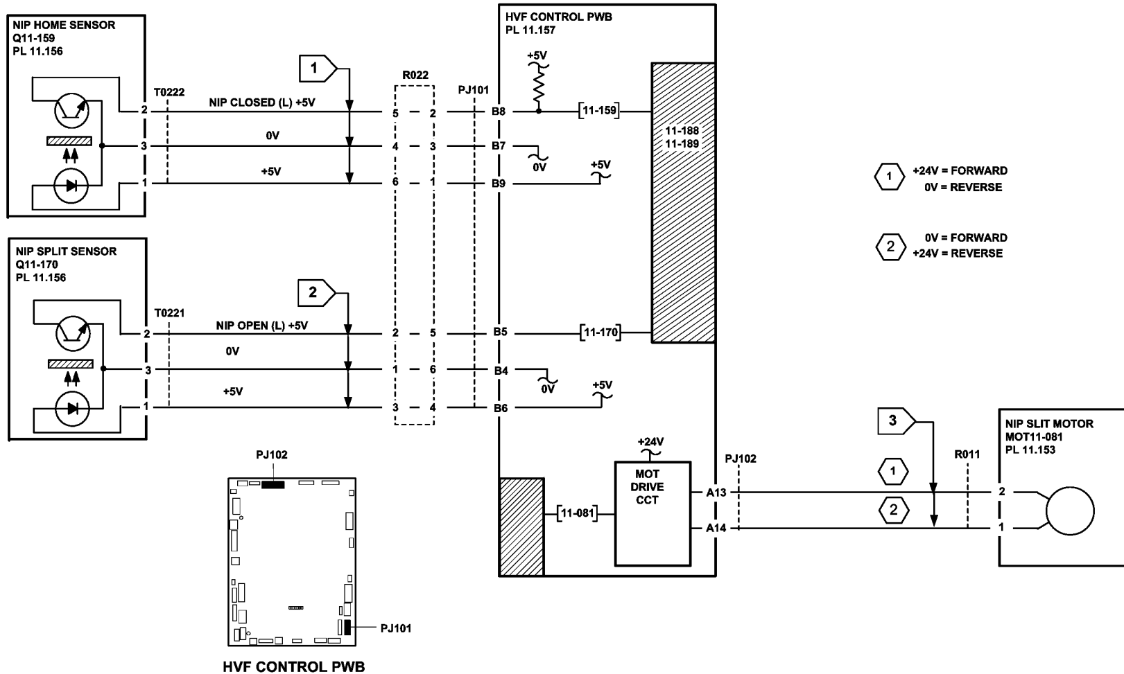
Figure 2 Circuit diagram
