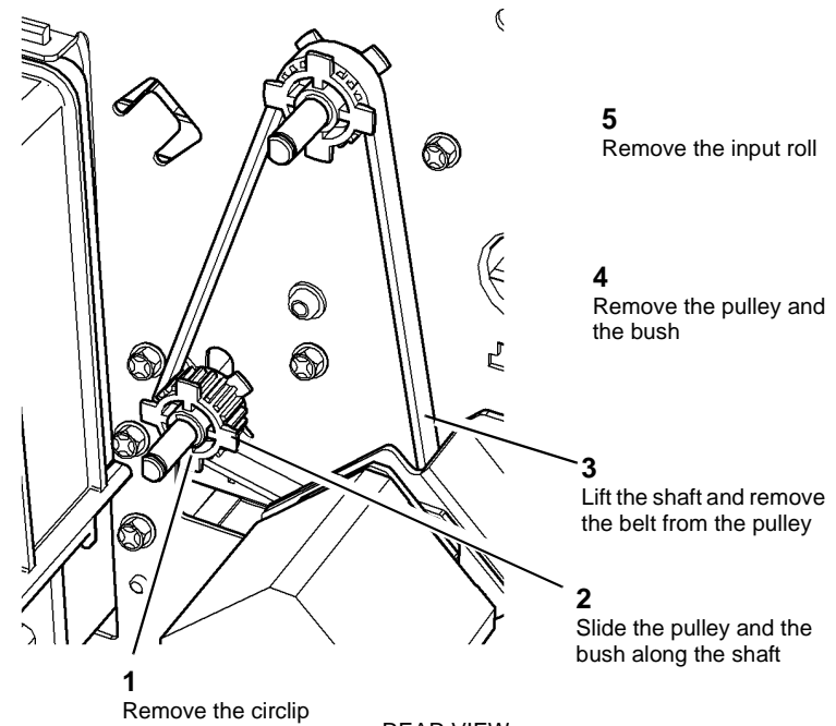
Figure 3 Input roll removal.
