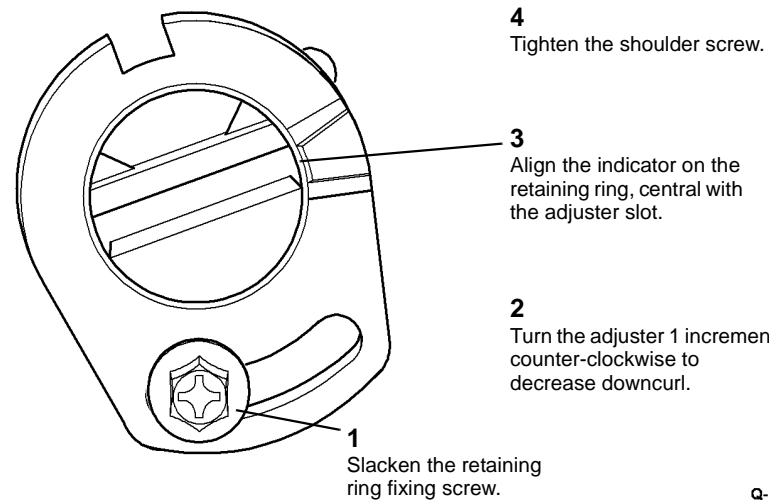
Figure 4 Decrease downcurl
