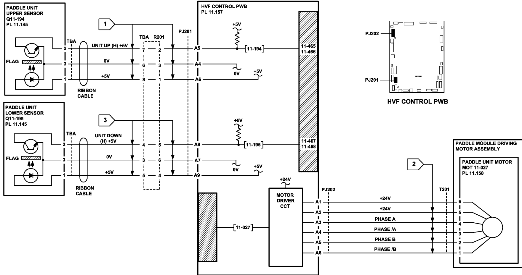
Figure 2 Circuit diagram
