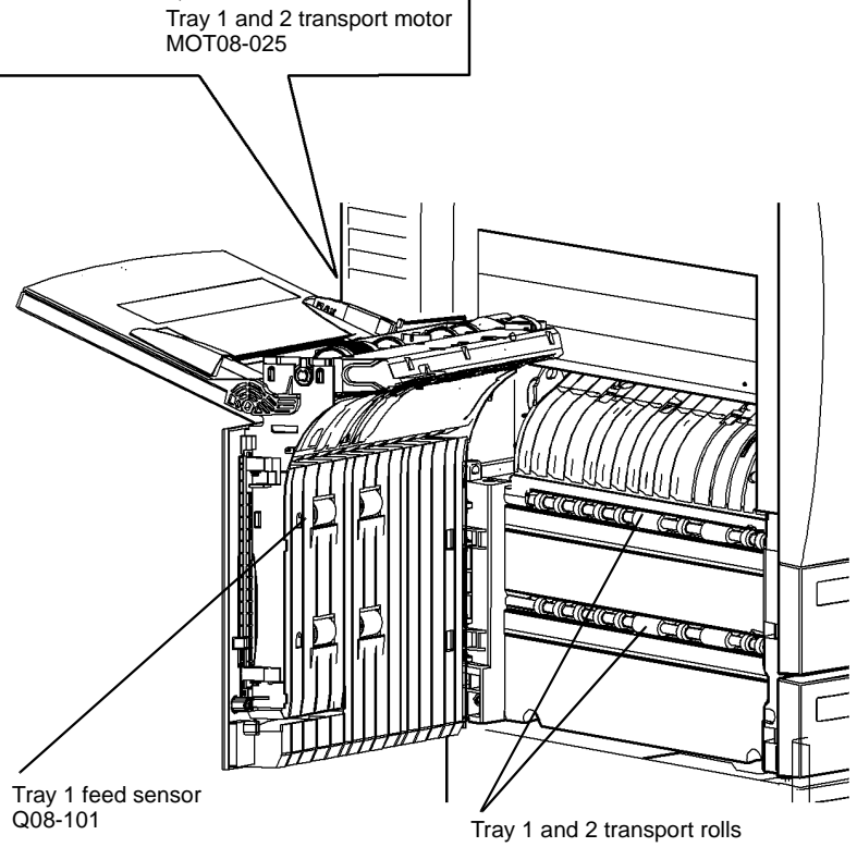
Figure 1 Component location
