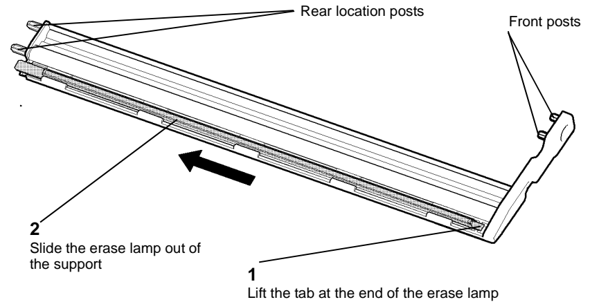
Figure 2 Remove the erase lamp
