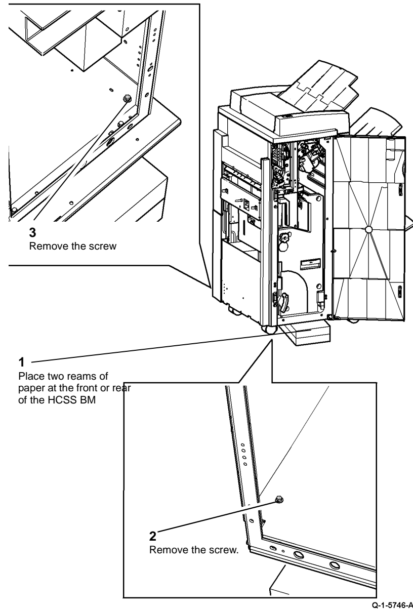
Figure 1 Removal of non-adjustable castors
