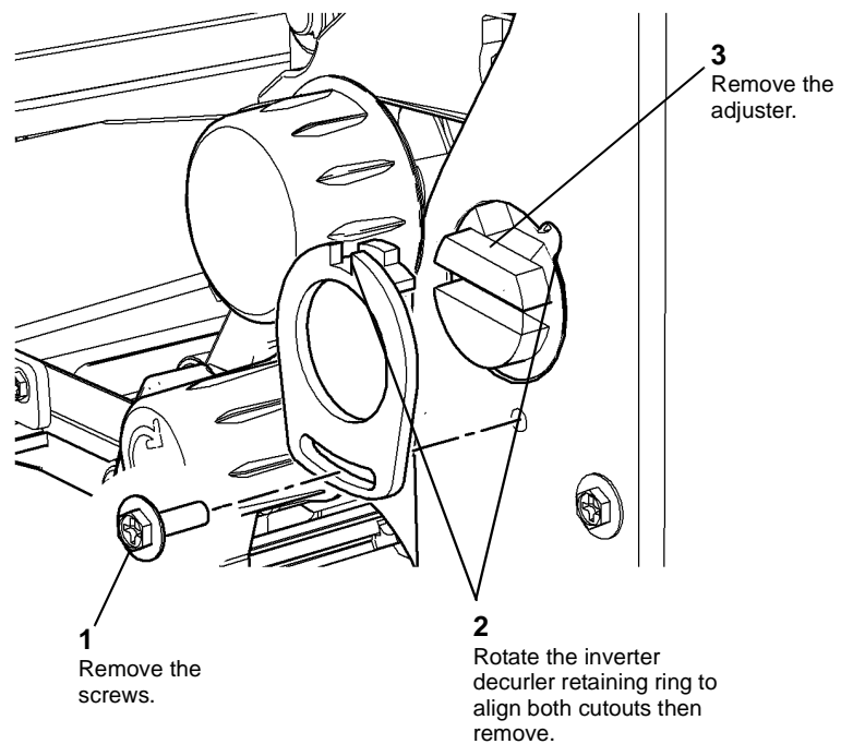
Figure 2 Adjuster and Retaining ring
