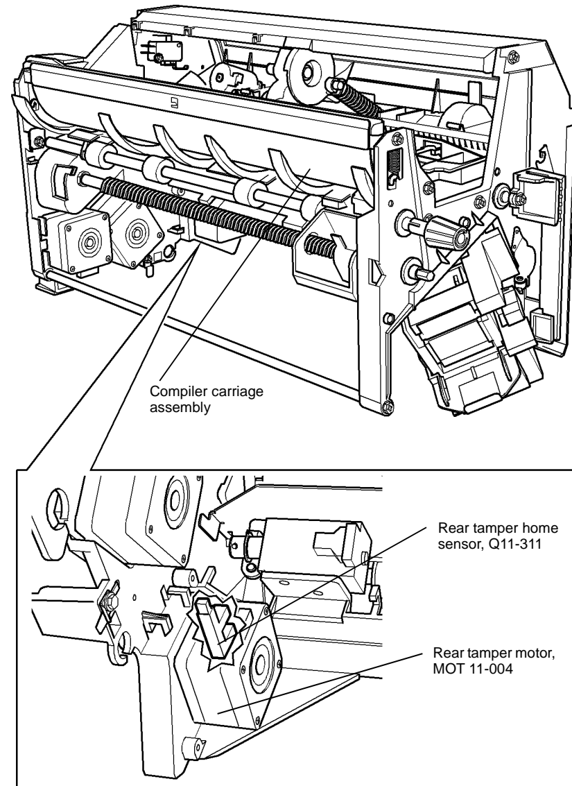
Figure 1 Component location
