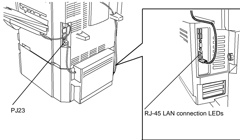
Figure 1 P/J23 and LAN connection location
