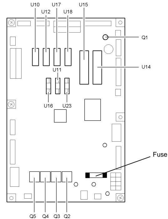
Figure 1 2K LCSS PWB components
