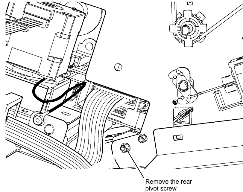
Figure 1 Rear pivot screw removal.
