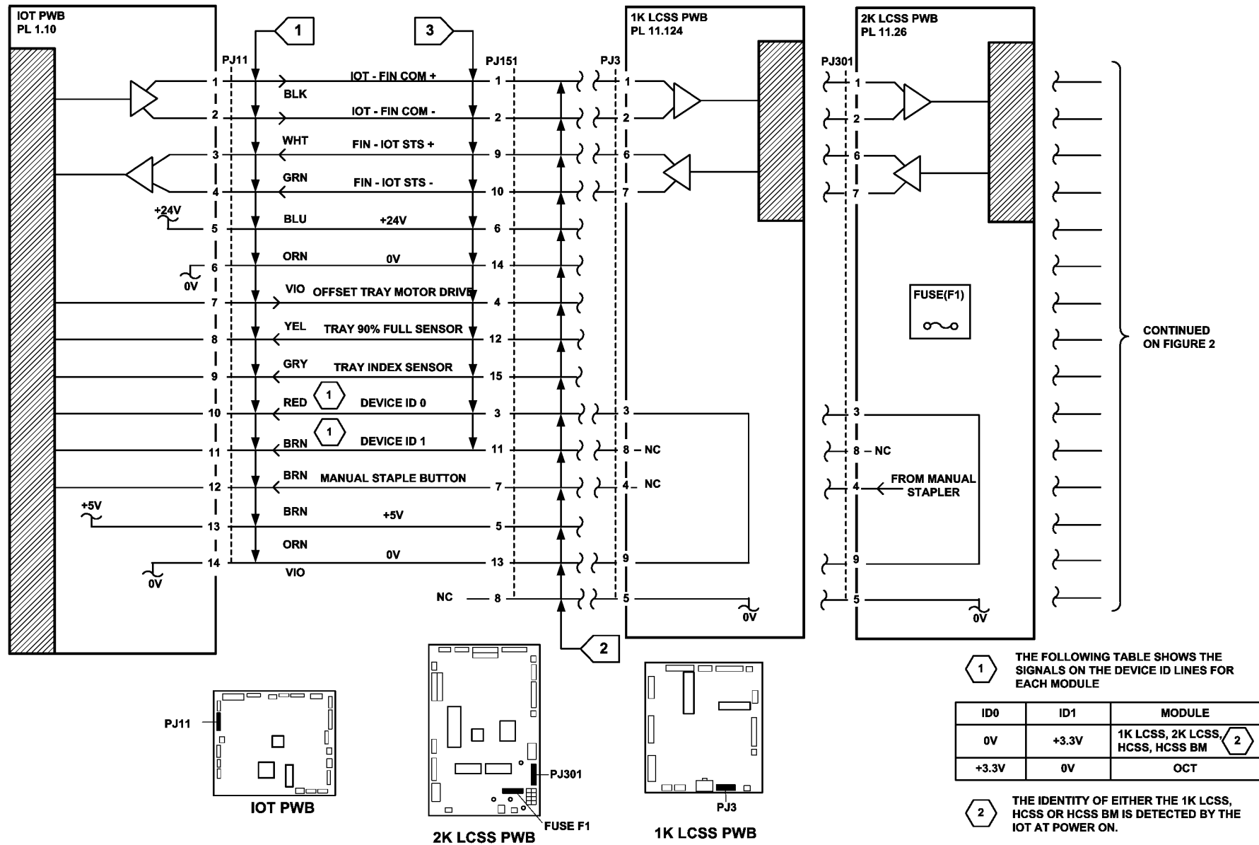
Figure 1 Circuit diagram
