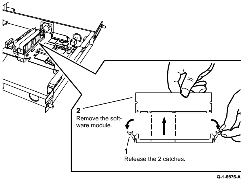
Figure 1 Software module removal W/OTAG 040
