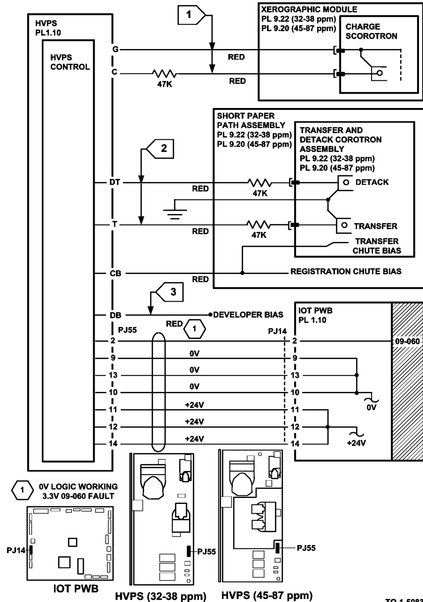
Figure 5 Circuit diagram
