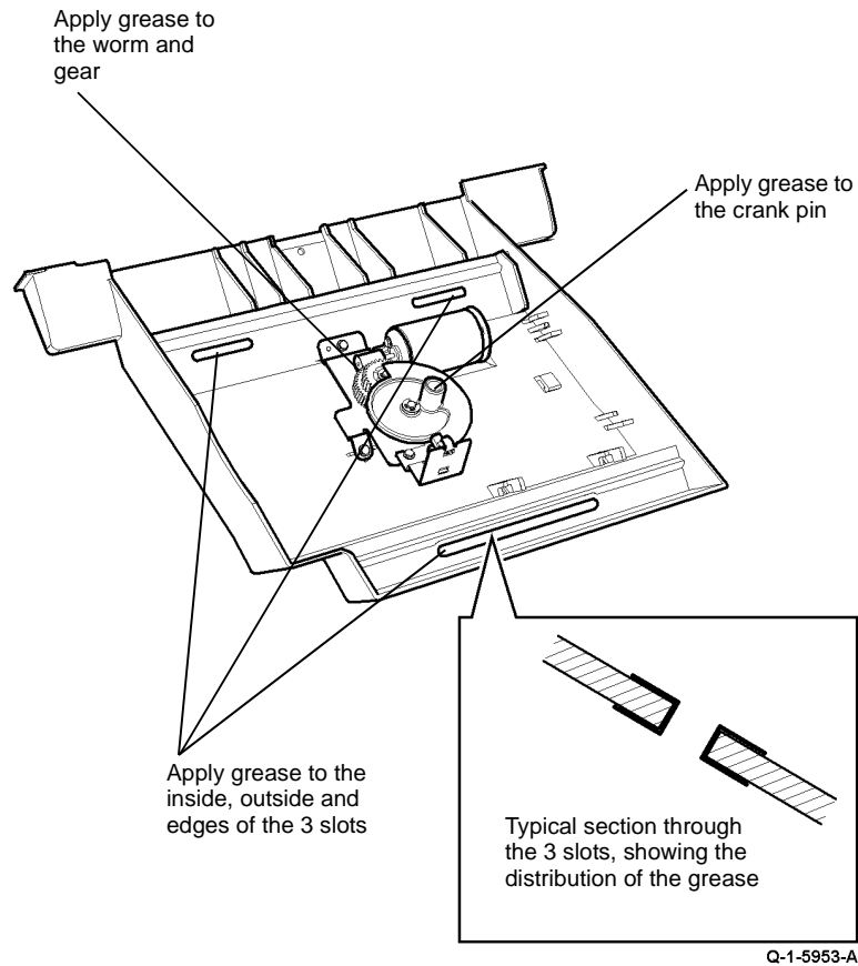
Figure 12 Tray lubrication
