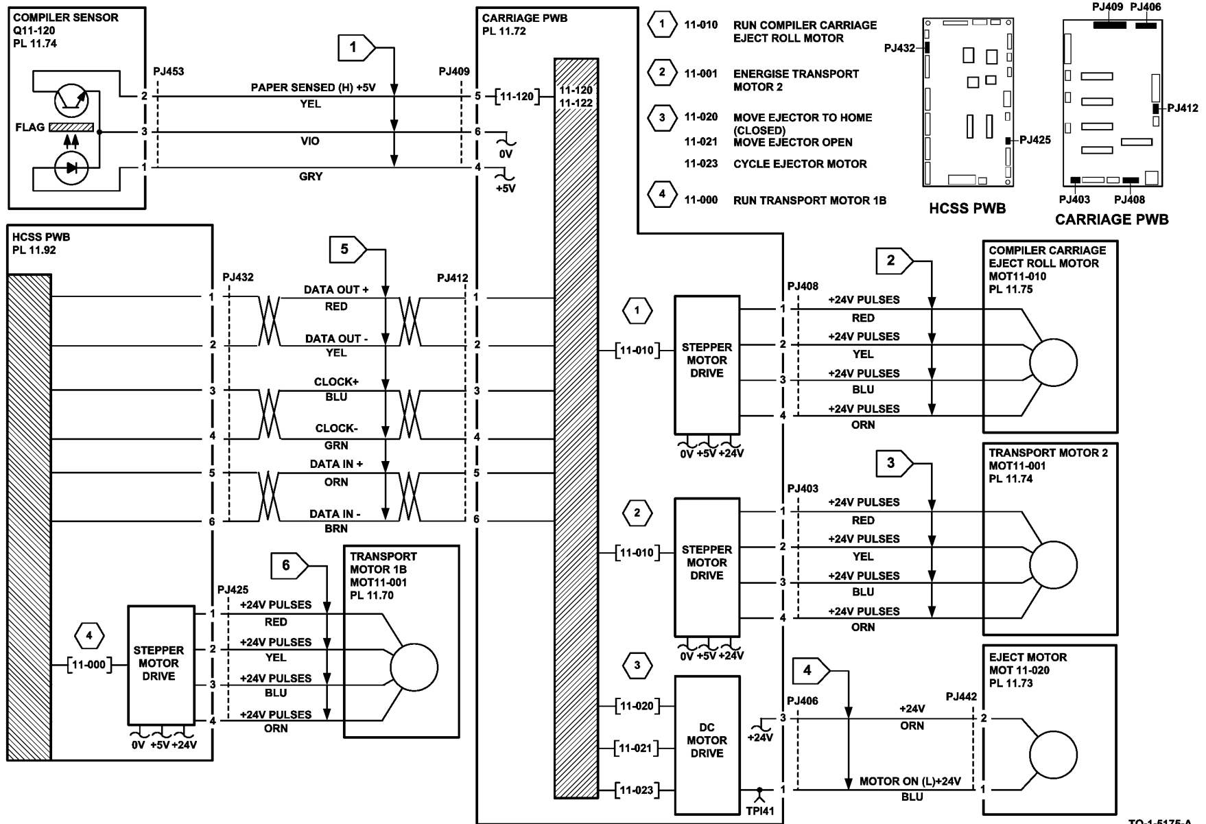
Figure 3 Circuit diagram
