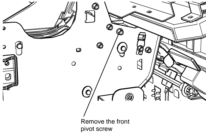
Figure 2 Front pivot screw removal.
