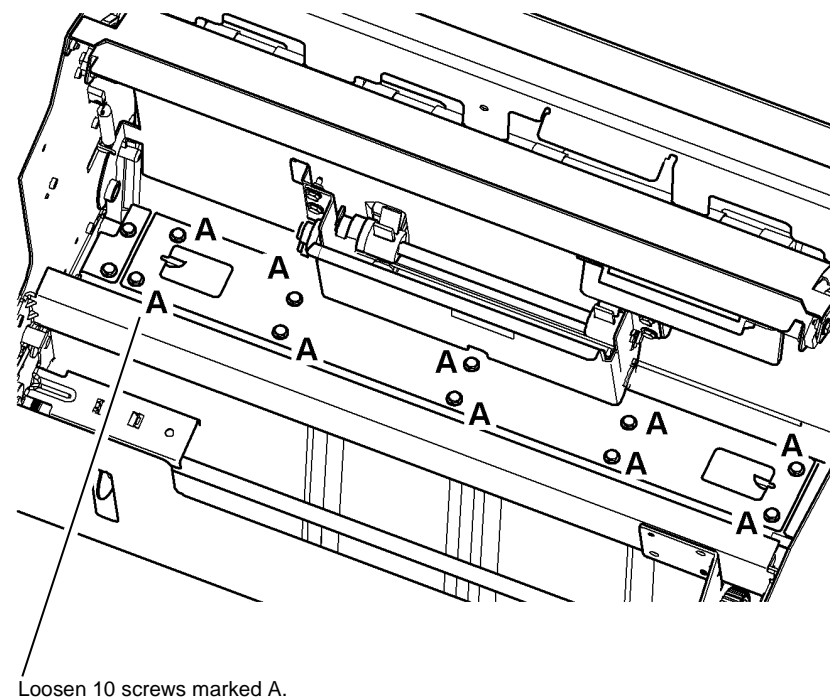
Figure 3 Blade loosening
