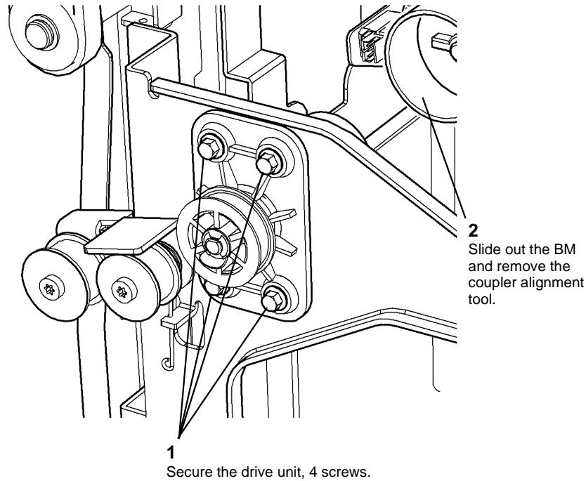
Figure 6 Secure the drive unit
