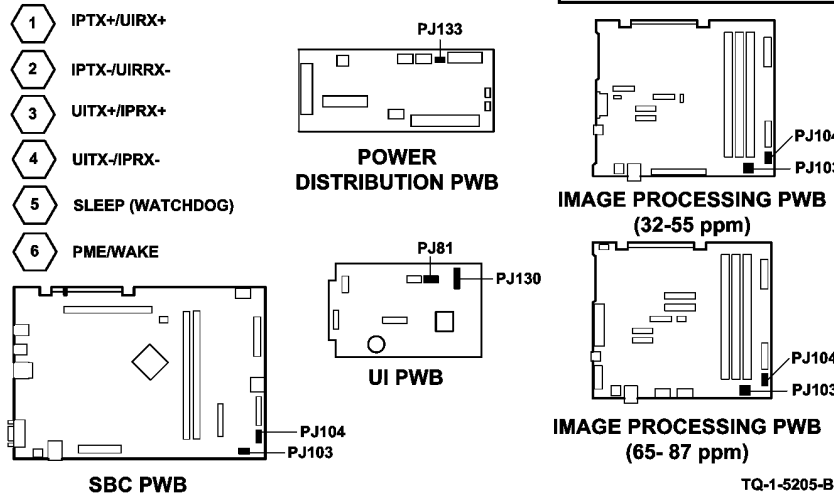
Figure 2 Circuit diagram
