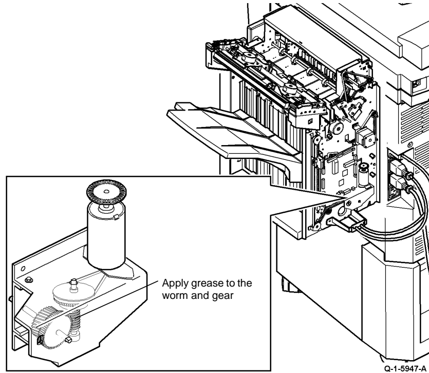
Figure 8 Lower vertical slides
