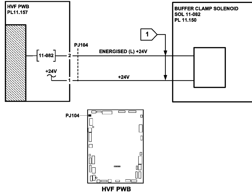
Figure 2 Circuit diagram
