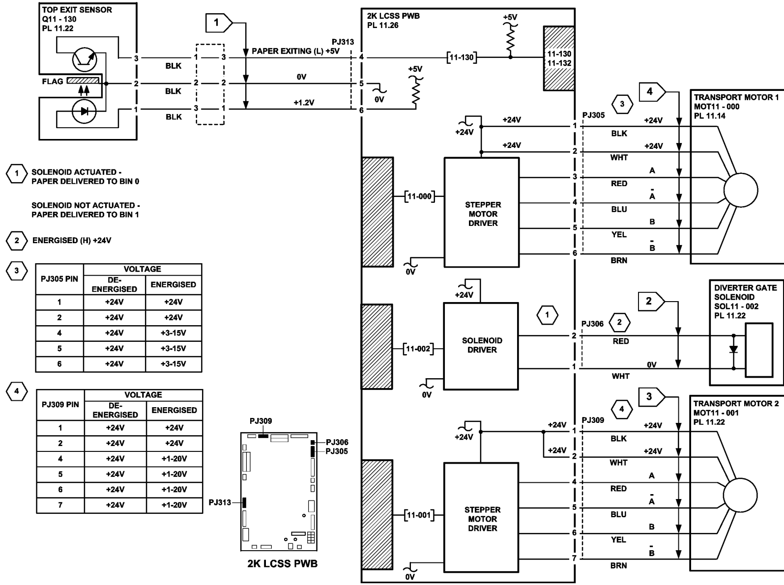
Figure 2 Circuit diagram
