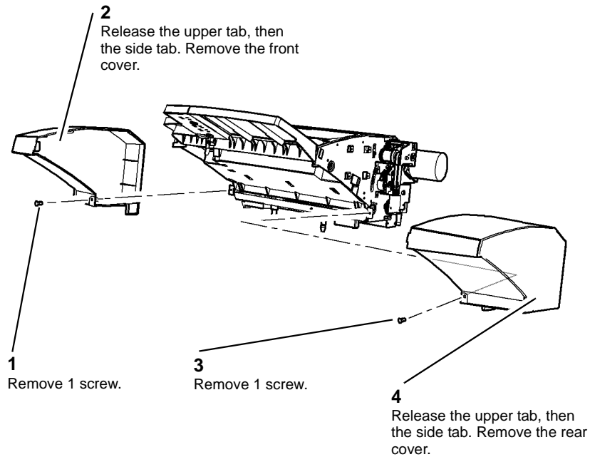
Figure 1 Covers removal
