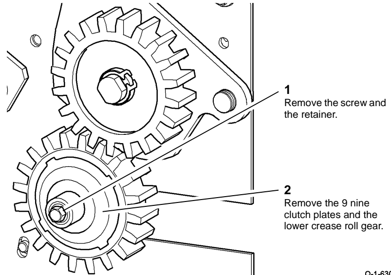
Figure 5 Clutch removal
