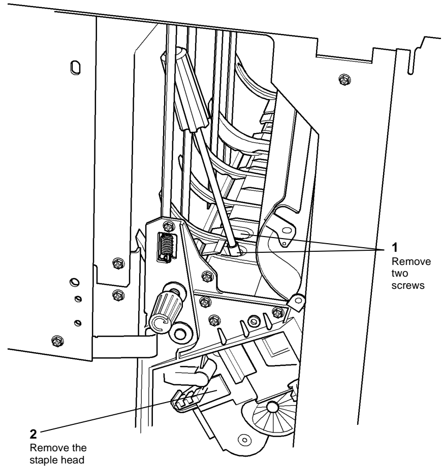
Figure 3 Staple head removal
