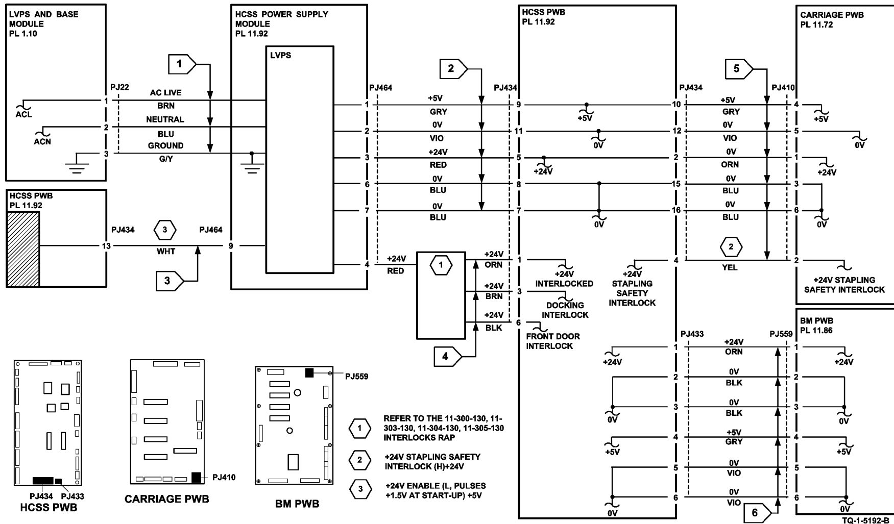
Figure 2 Circuit diagram
