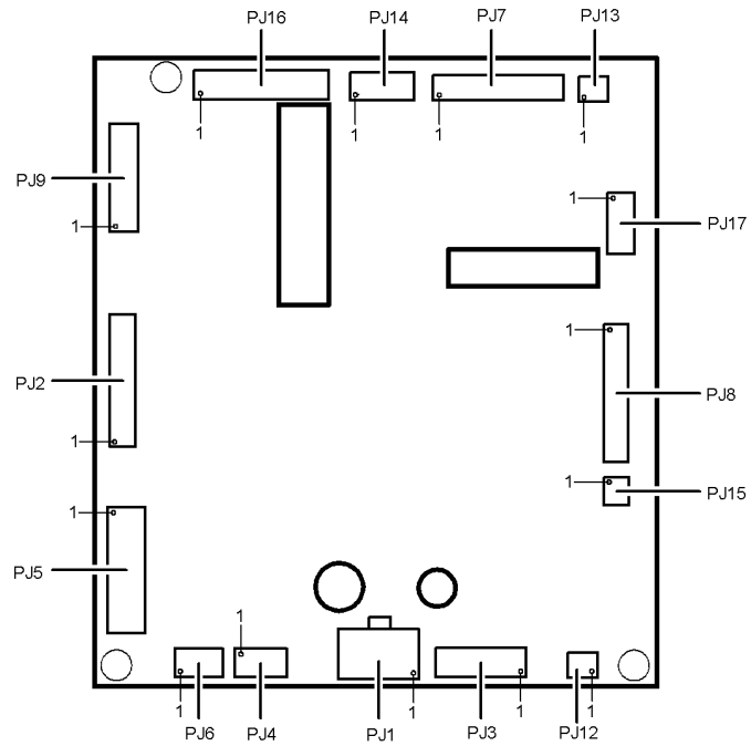
Figure 32 1K LCSS PWB
