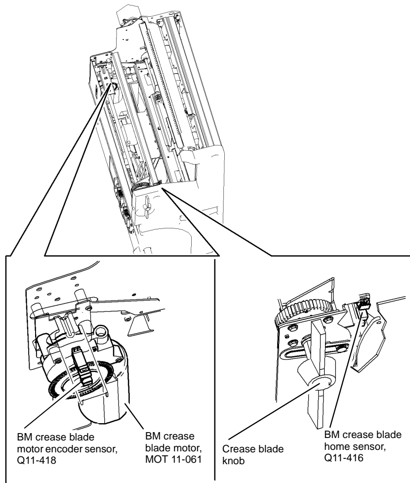
Figure 1 Component location
