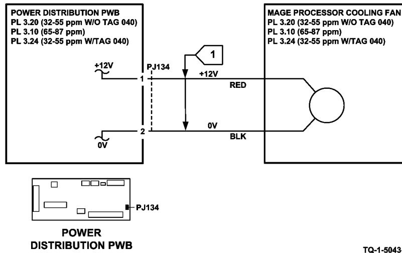
Figure 1 Circuit diagram
