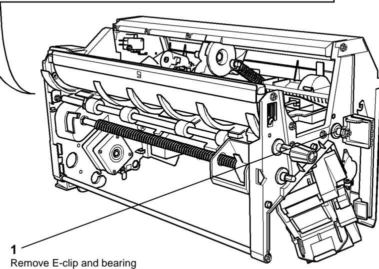
Figure 1 Preparation
