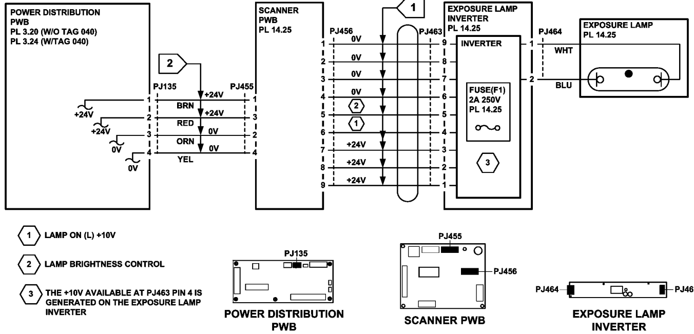
Figure 2 Circuit diagram
