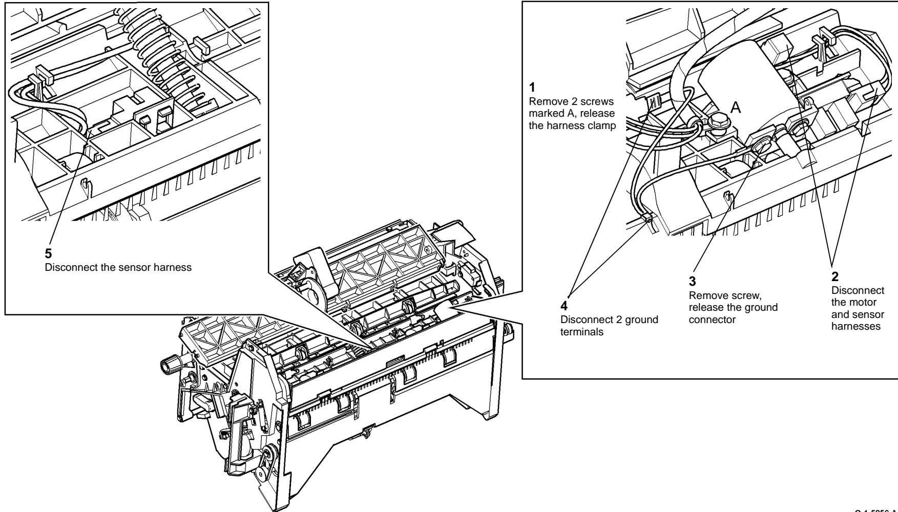
Figure 2 Preparation
