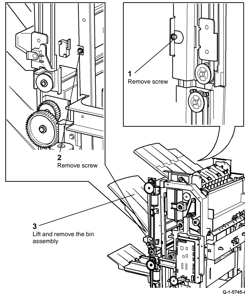
Figure 1 Bin 1 assembly removal
