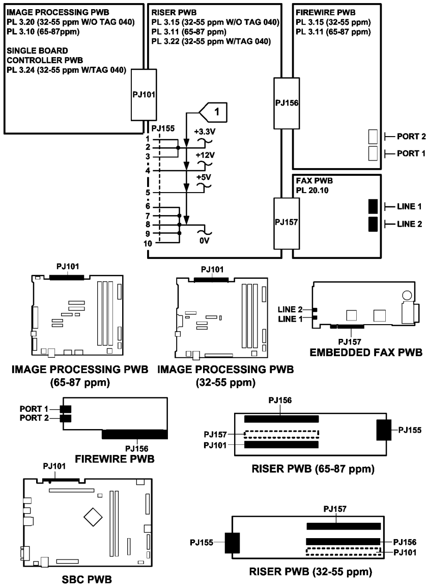
Figure 2 Circuit diagram
