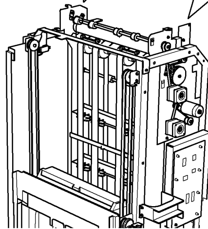
Figure 3 Bearing removal
