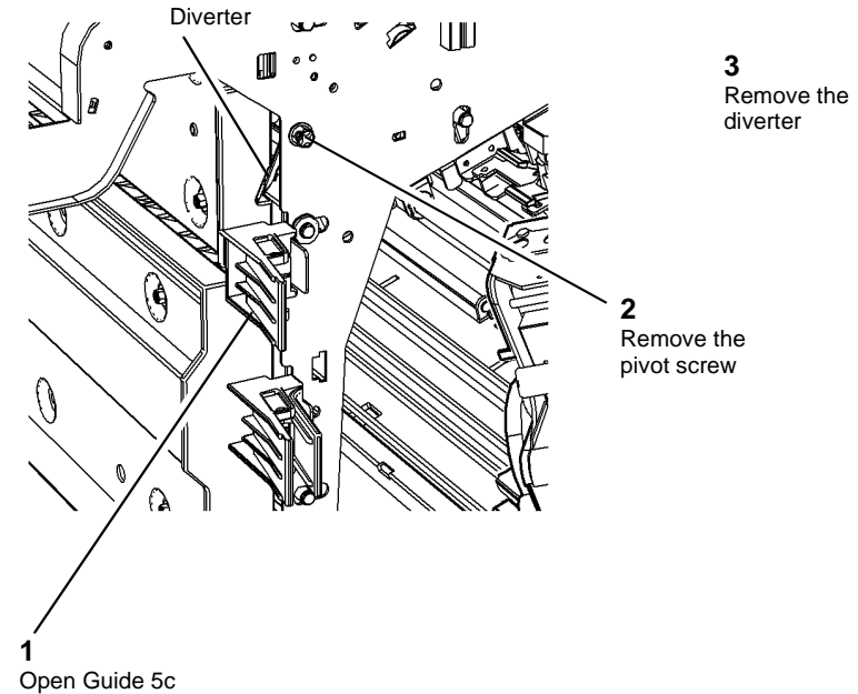
Figure 2 Diverter removal
